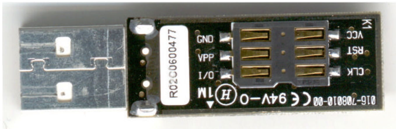
Internal board, smart card connector side
