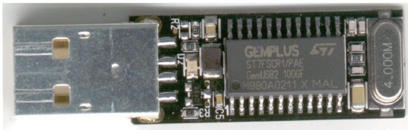
Internal board, smart card connector removed
