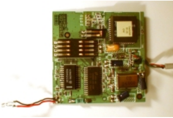
3 – Internal board, Component side
