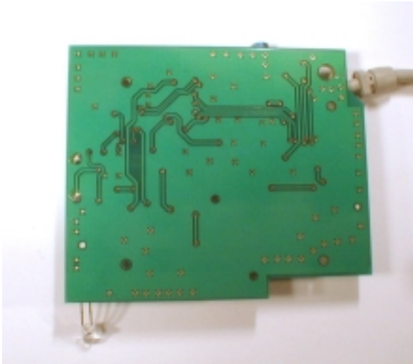
4 – Internal board, Foil side
