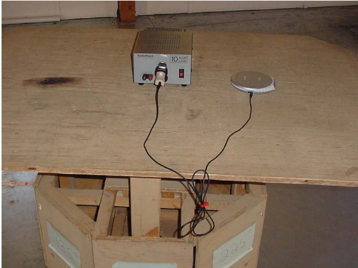
Radiated Test setup Front
