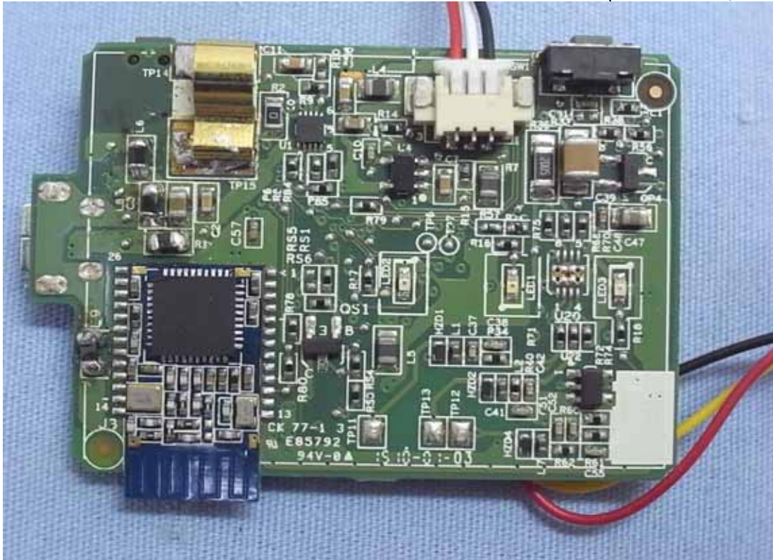
Figure 13 Internal View (Main Board, Front View)
