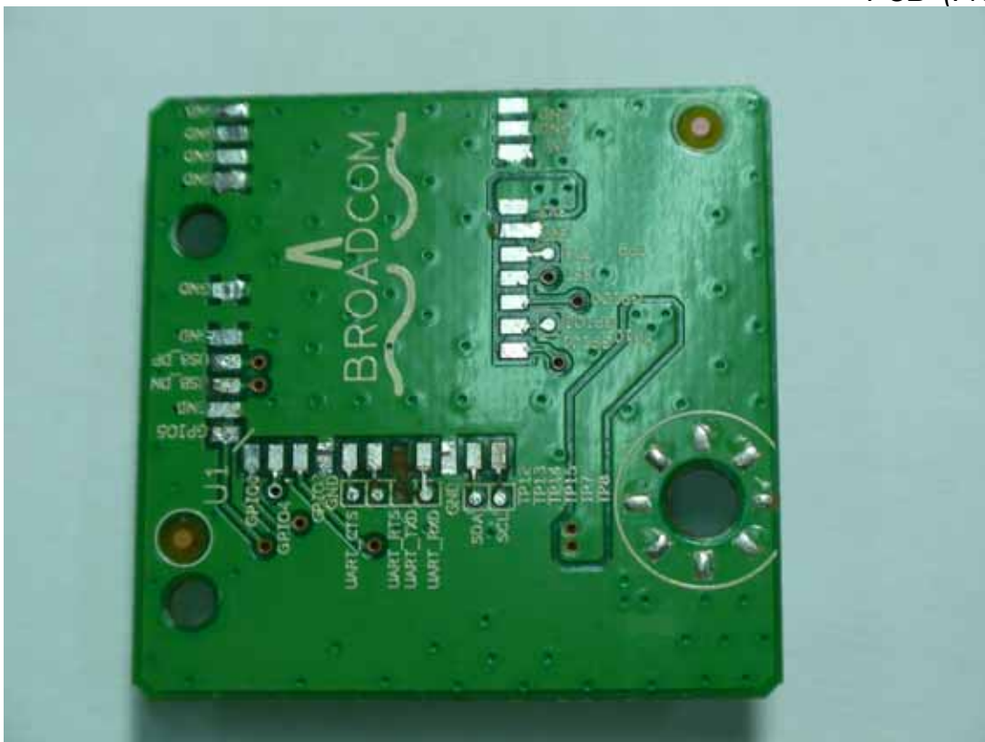
Photo 3 PCB (Front View)
