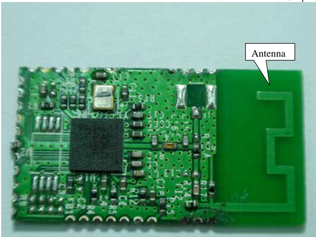
Photo 6 PCB (Front View)
