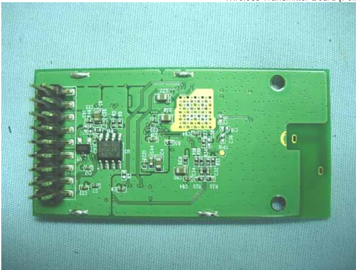
Figure 9 Wireless Transmitter Board (Foil Side)
