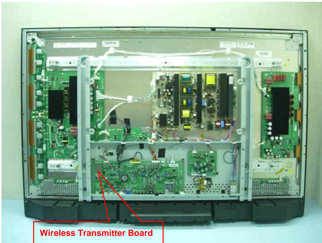
Figure 7 Internal View
