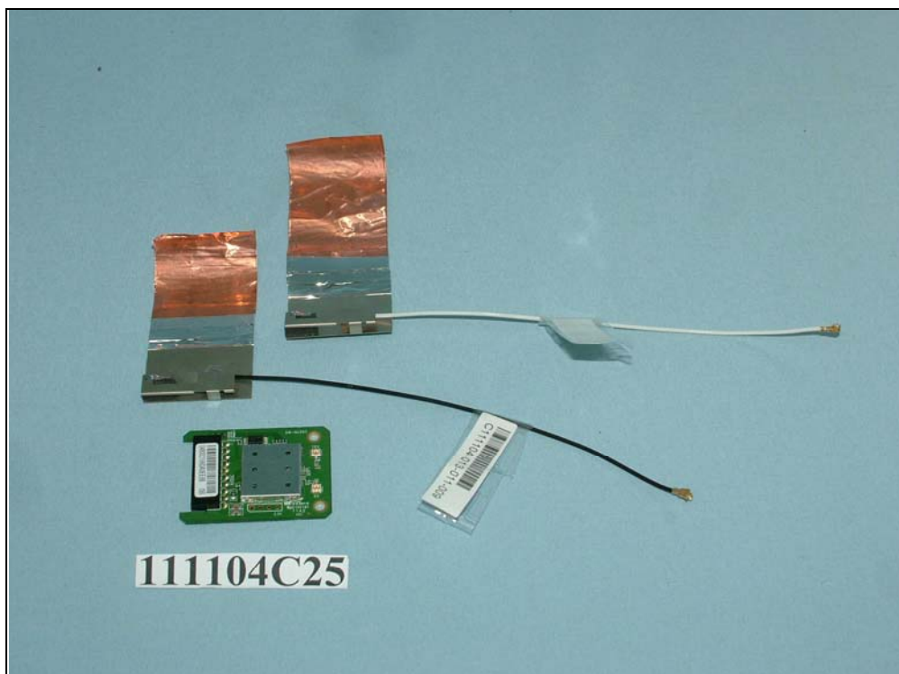
EUT with antenna item 1
