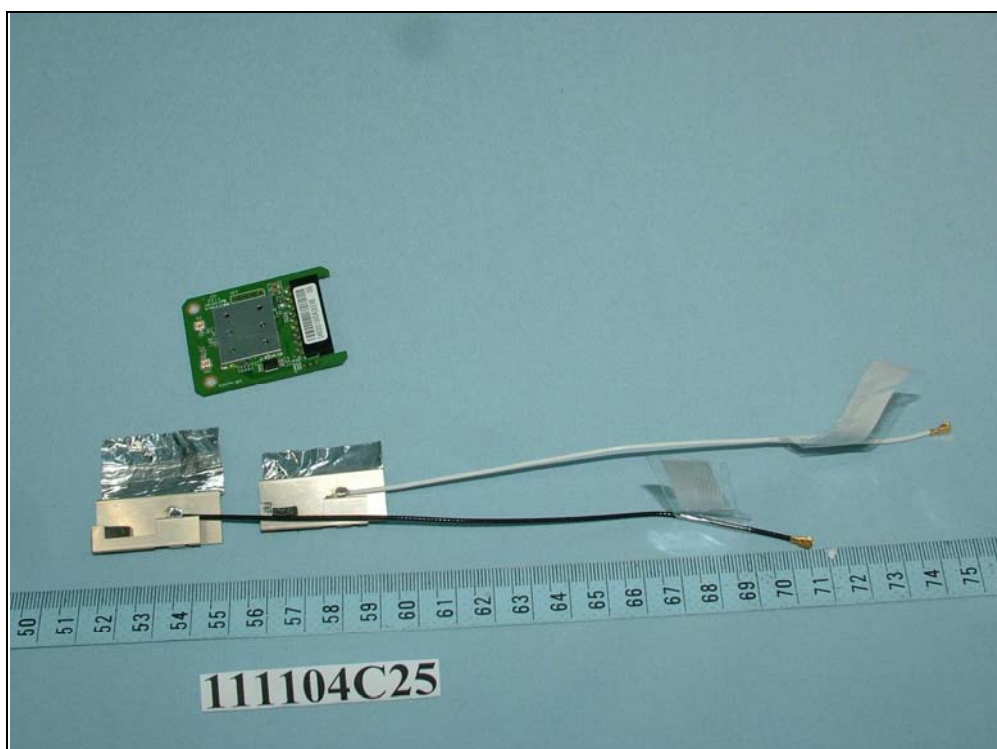
EUT with antenna item 2
