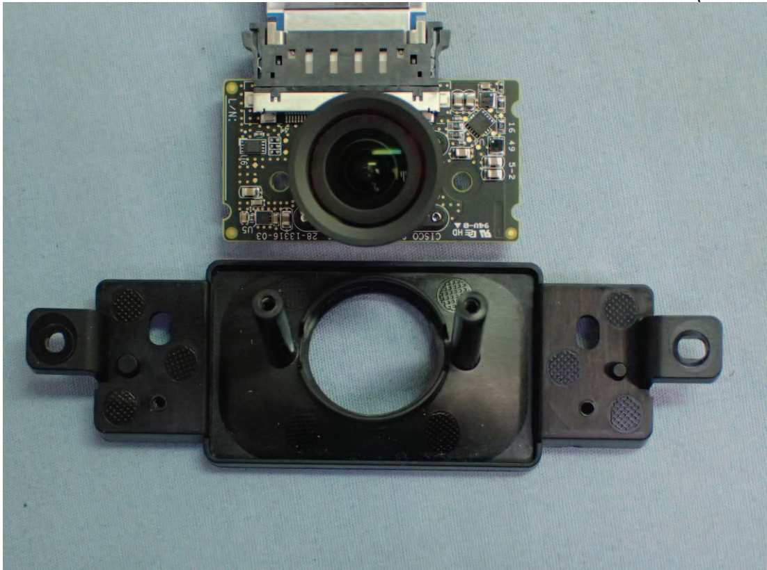
Figure 11 Internal View (Sensor Board)
