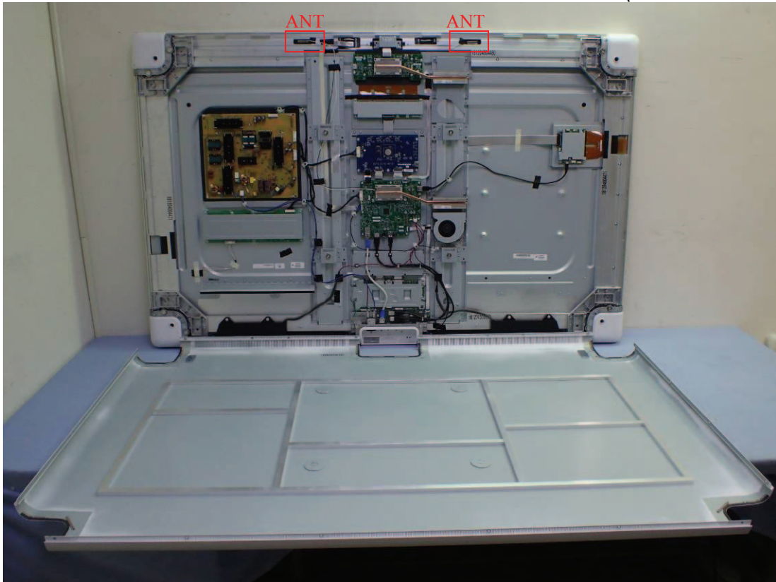
Figure 6 Internal View (Removed Back Cover)
