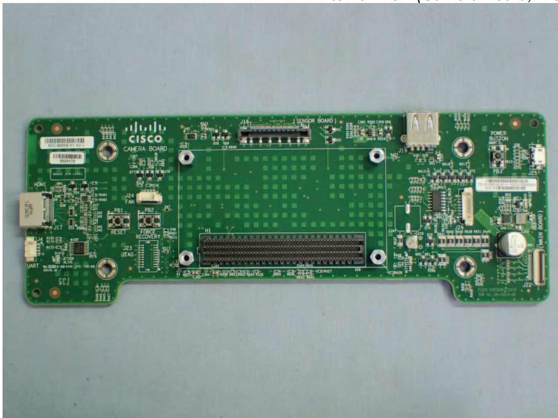
Figure 13 Internal View (Camera Board, Front View)
