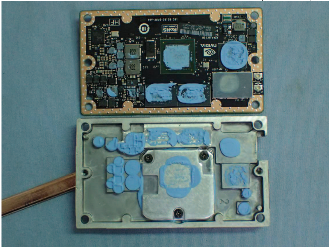
Figure 16 Internal View (TX1 Board, Front View)
