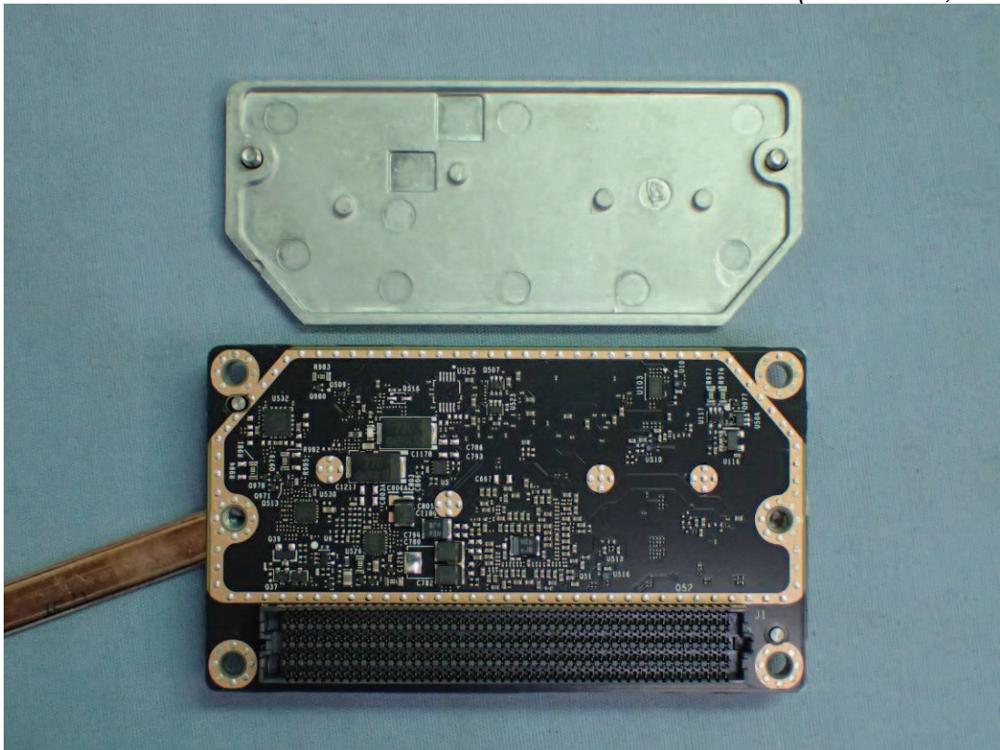
Figure 15 Internal View (TX1 Board, Back View)
