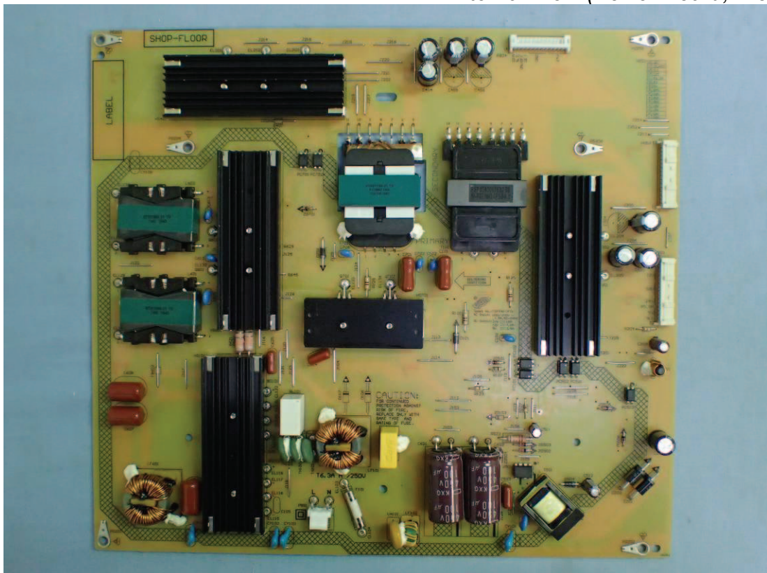
Figure 17 Internal View (Power Board, Front View)
