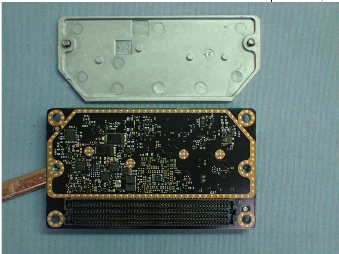
Figure 31 Internal View (RF Module, Back View)
