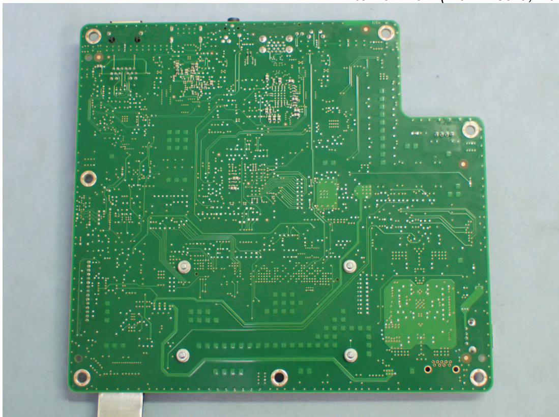
Figure 29 Internal View (Main Board, Back View)
