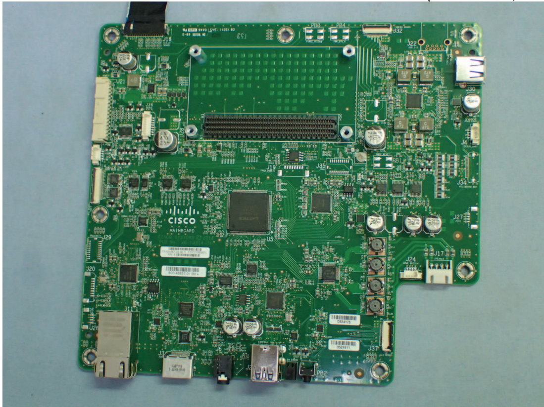
Figure 28 Internal View (Main Board, Front View)
