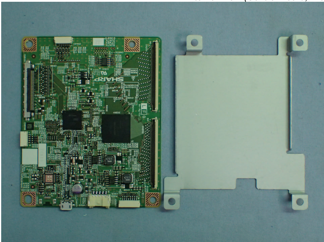
Figure 35 Internal View (Control Board, Front View)
