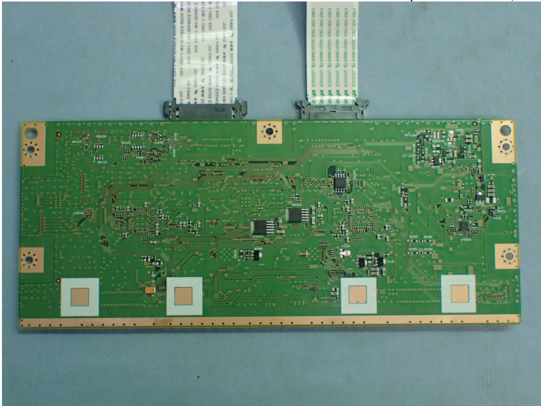
Figure 34 Internal View (Control Board, Back View)
