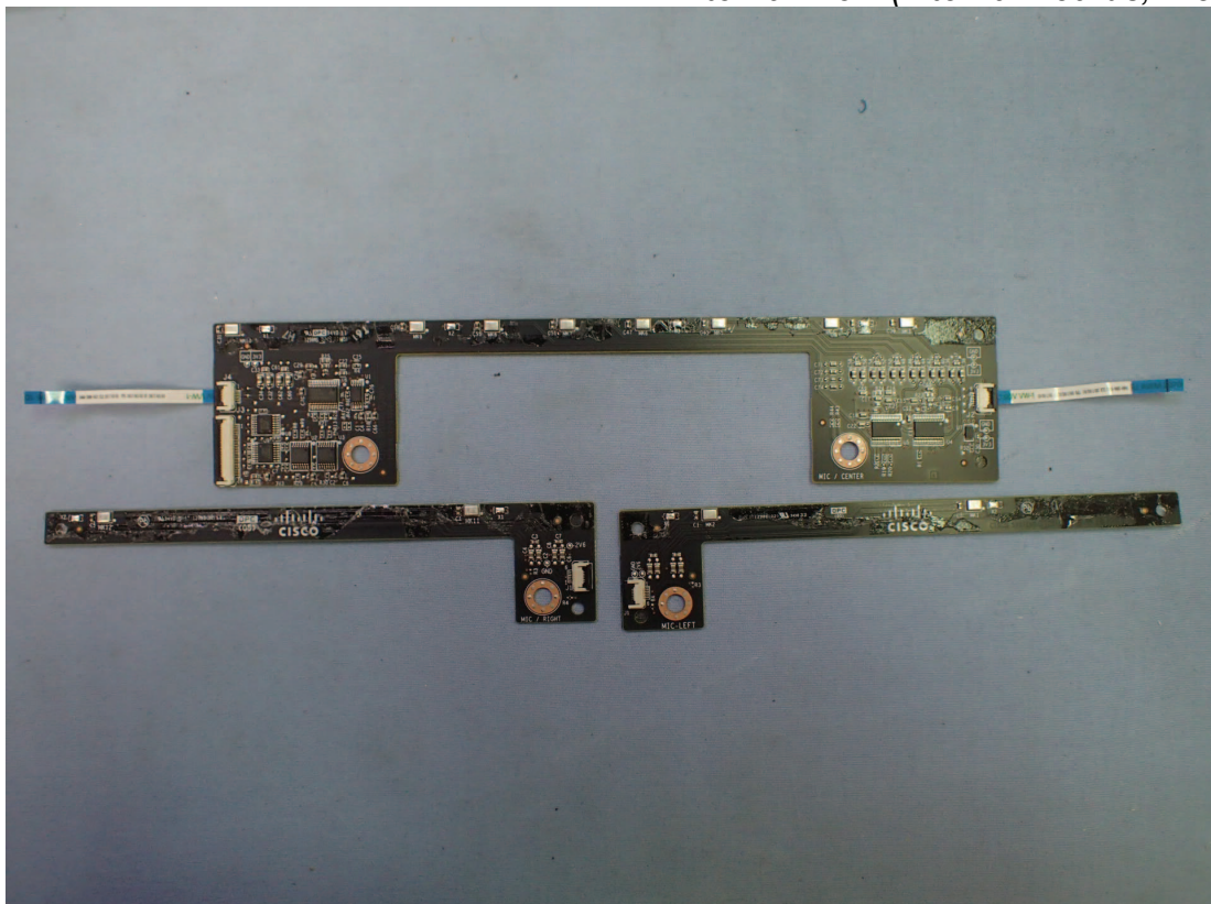
Figure 37 Internal View (Internal Boards, Front View)
