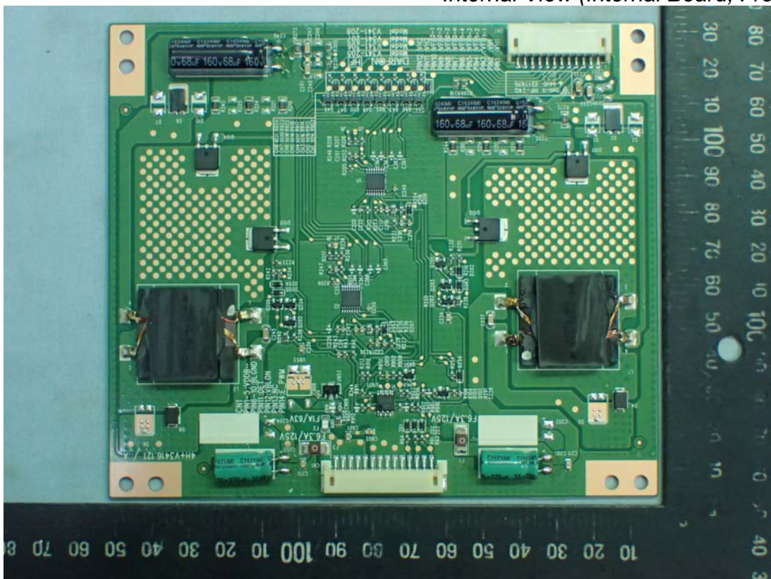
Figure 29 Internal View (Internal Board, Front View)
