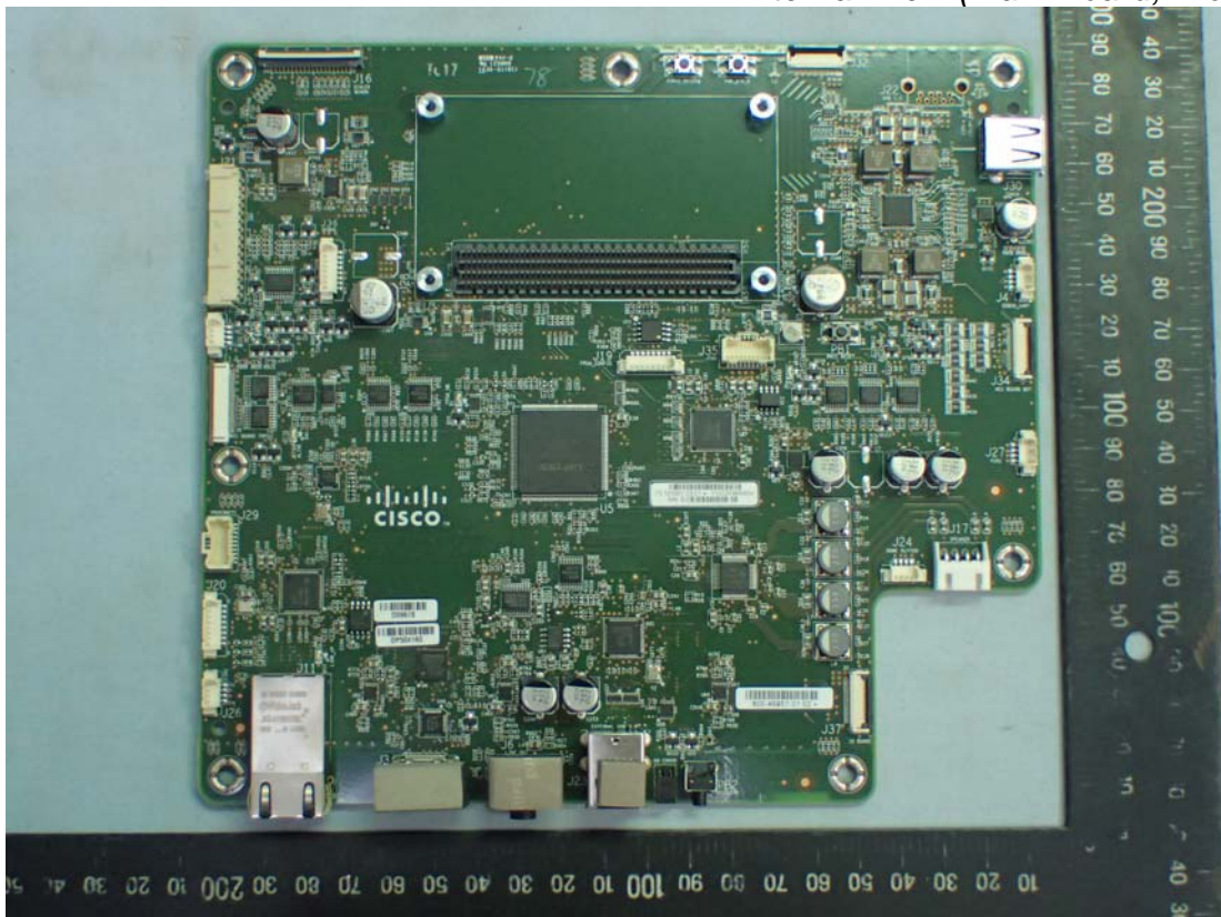
Figure 37 Internal View (Main Board, Front View)
