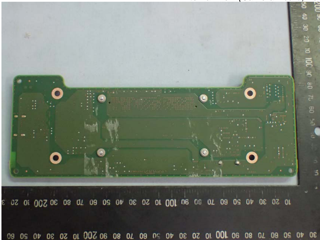
Figure 19 Internal View (Camera Board, Back View)
