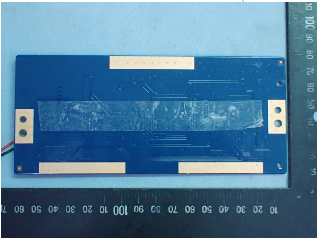
Figure 25 Internal View (T-Com Board, Back View)
