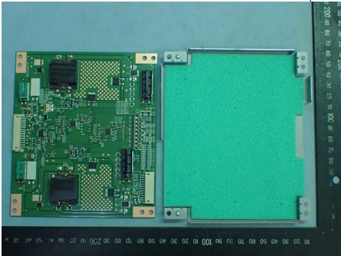
Figure 28 Internal View (Internal Board)
