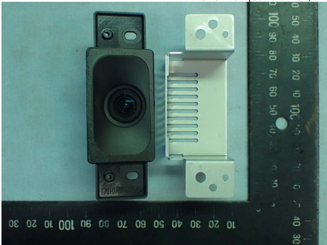
Figure 33 Internal View (Camera View, Front View)
