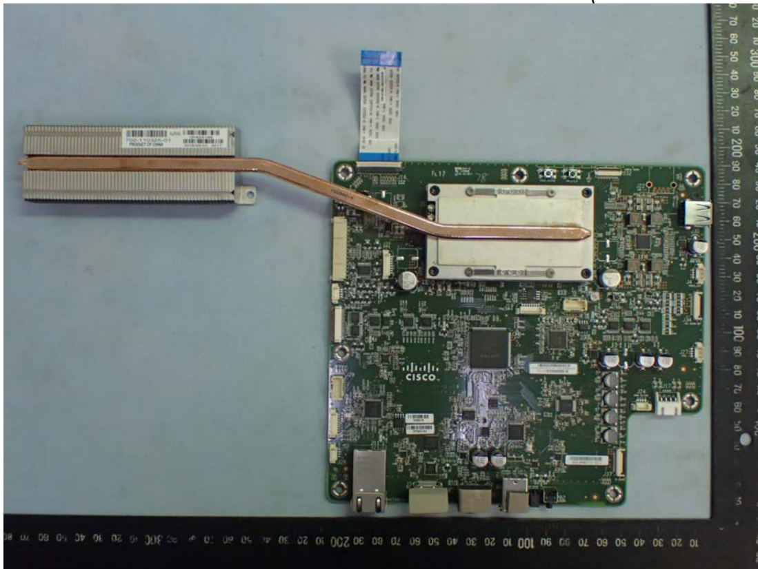
Figure 36 Internal View (Main Board & Heat Sink)
