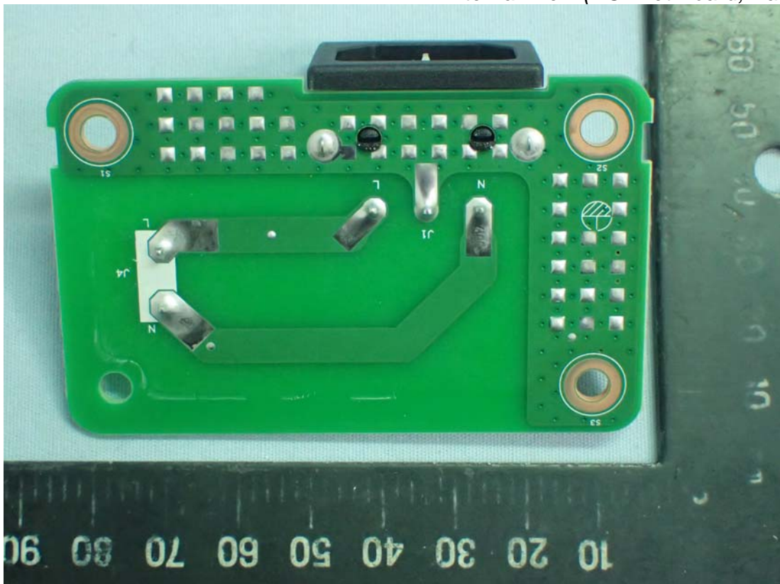
Figure 15 Internal View (AC Inlet Board, Back View)
