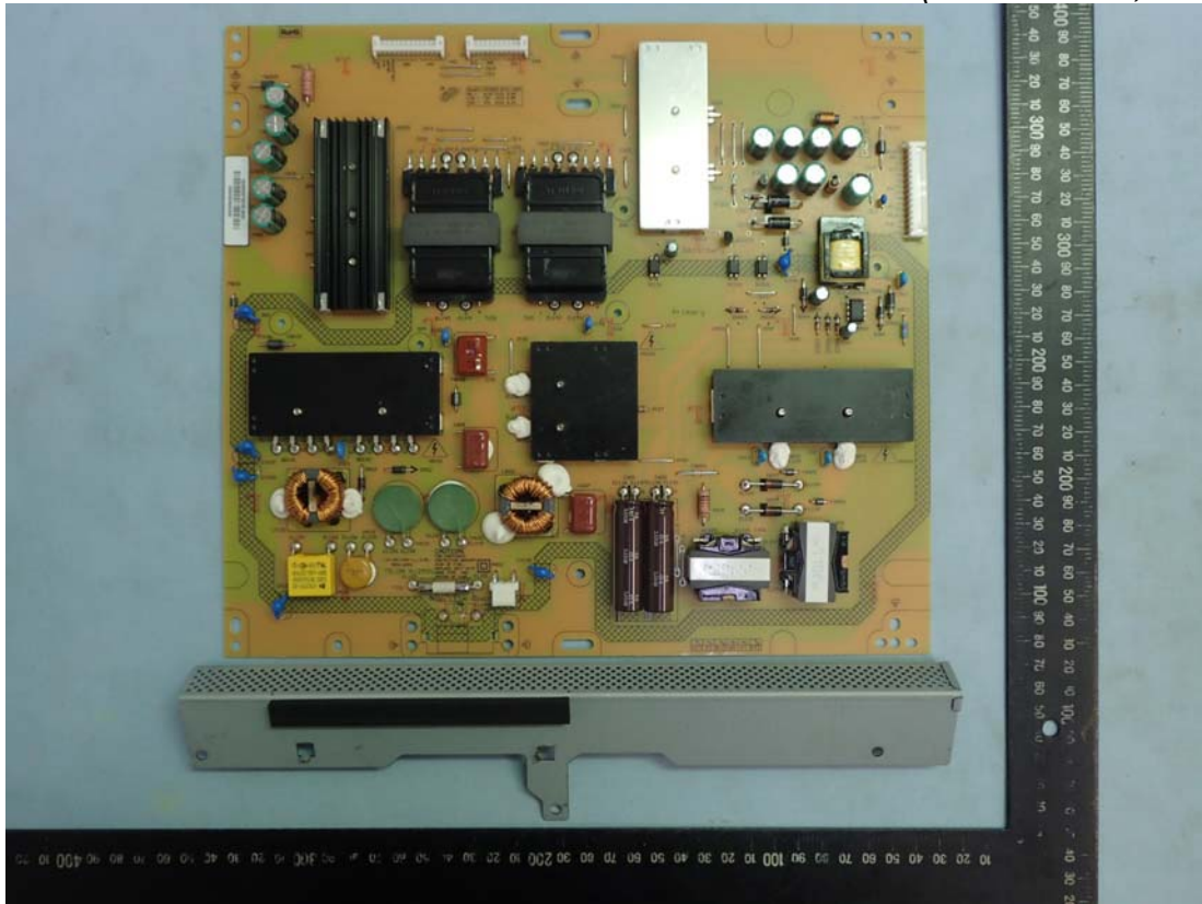
Figure 10 Internal View (Power Board, Front View)
