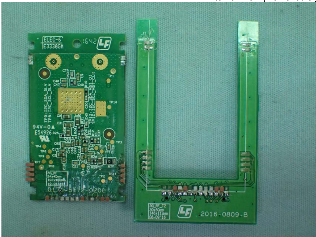
Internal View (Removed Jig Board)
