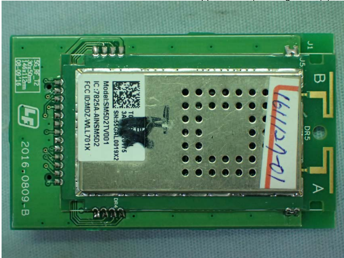
Figure 2 General Appearance (With Jig Board) (Back View)
