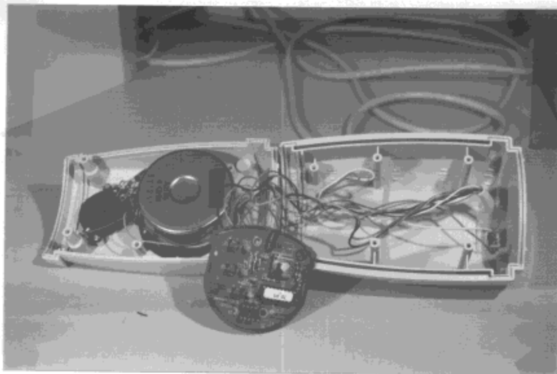
Figure 12.6 Partially Disassembled, Speaker Opened
