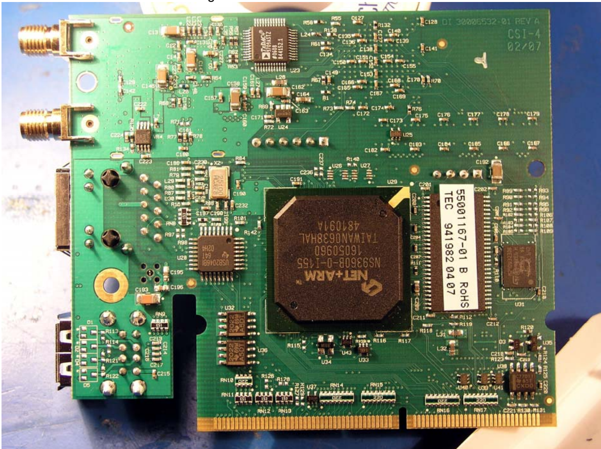
Digi ConnectCore Wi9C Solder Side
