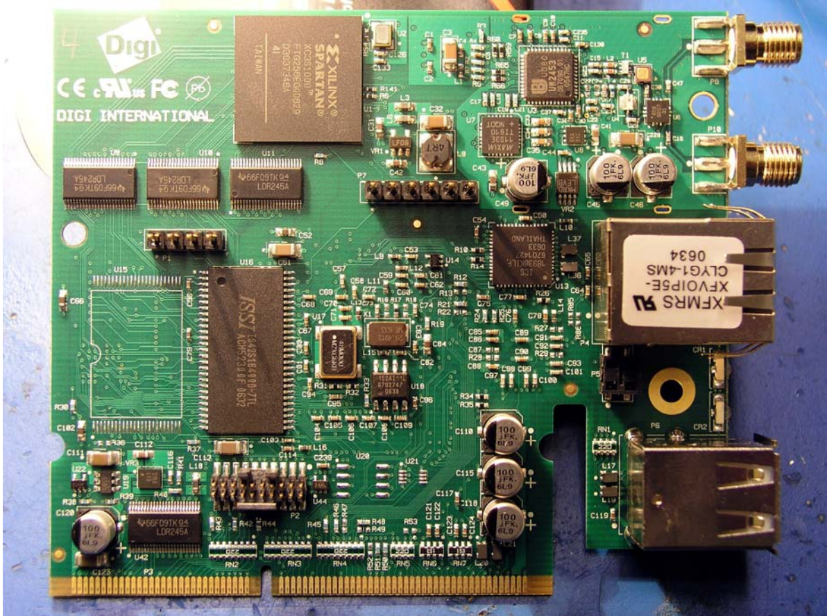
Digi ConnectCore Wi9C Comp Side
