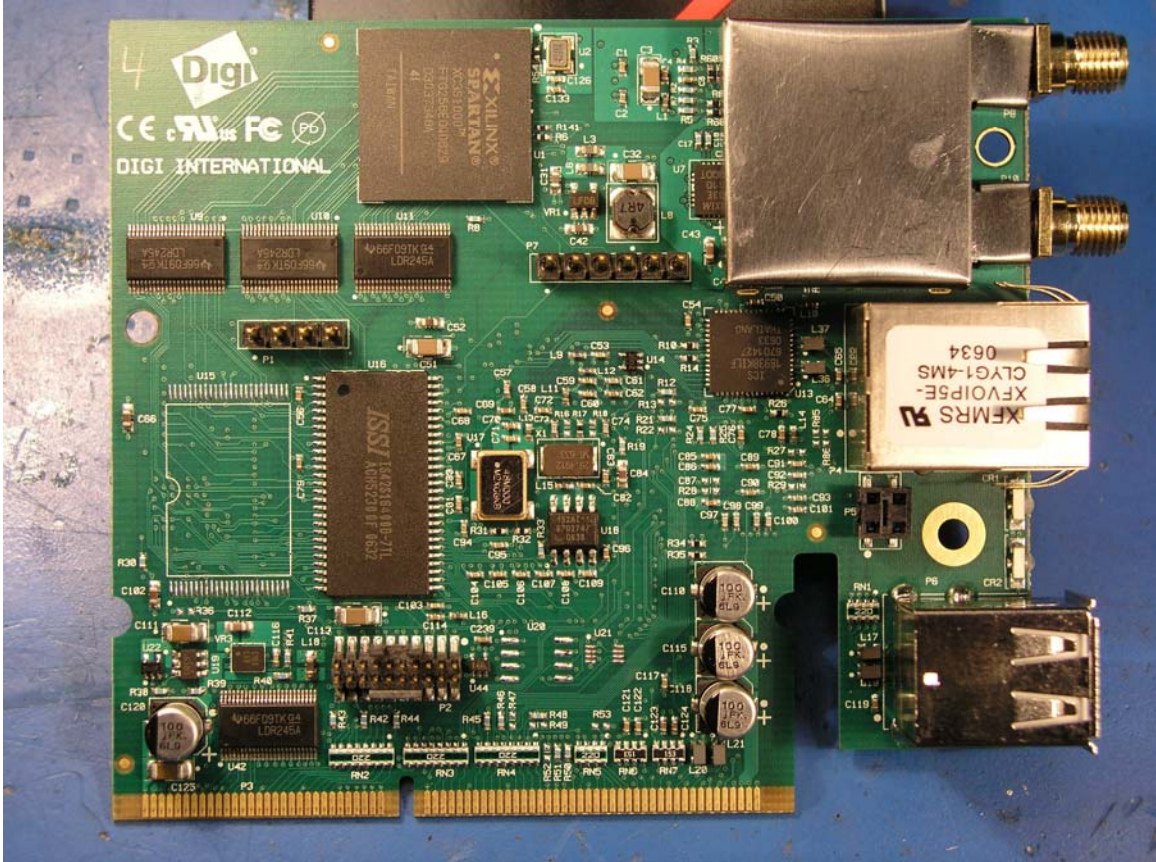
Digi ConnectCore Wi9C Shield Rear
