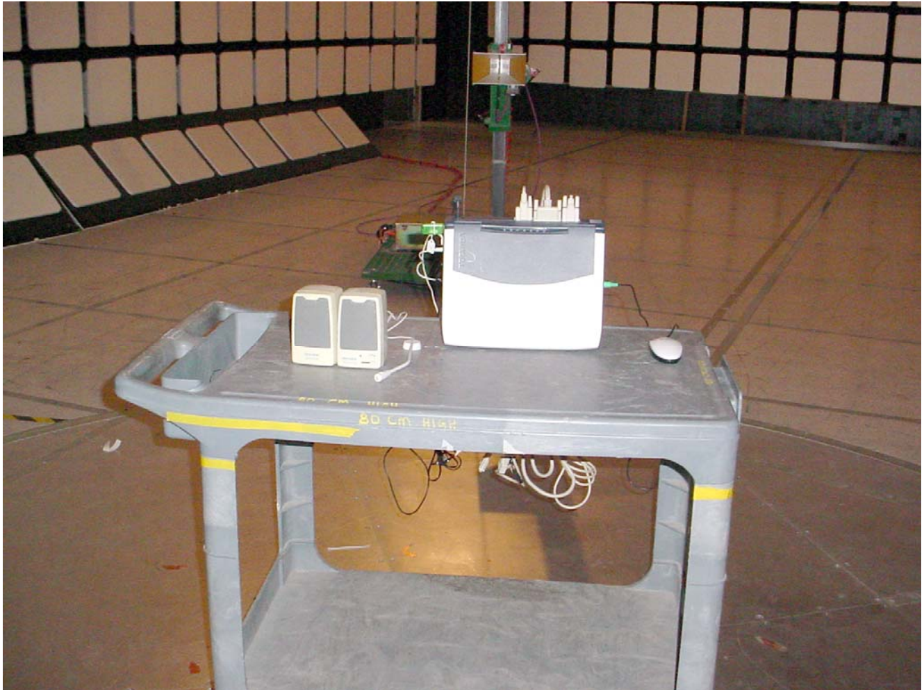
Radiated Emissions @ 3 m EUT Orientation: Orthogonal Position 2
