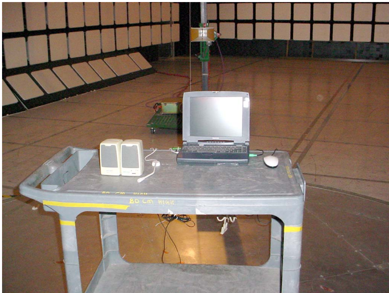
Radiated Emissions @ 3 m EUT Orientation: Orthogonal Position 1
