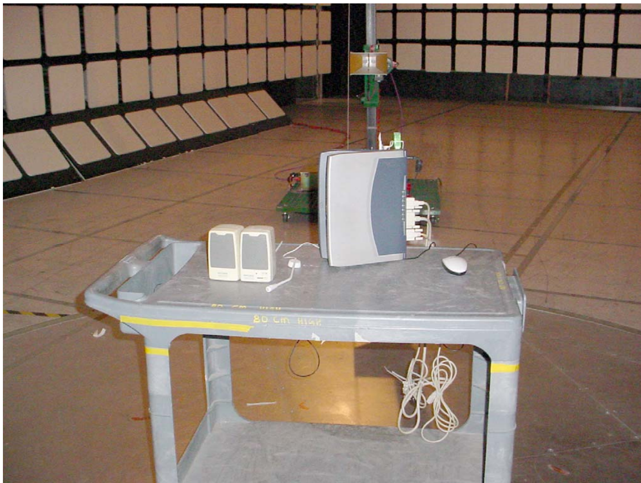
Radiated Emissions @ 3 m EUT Orientation: Orthogonal Position 3
