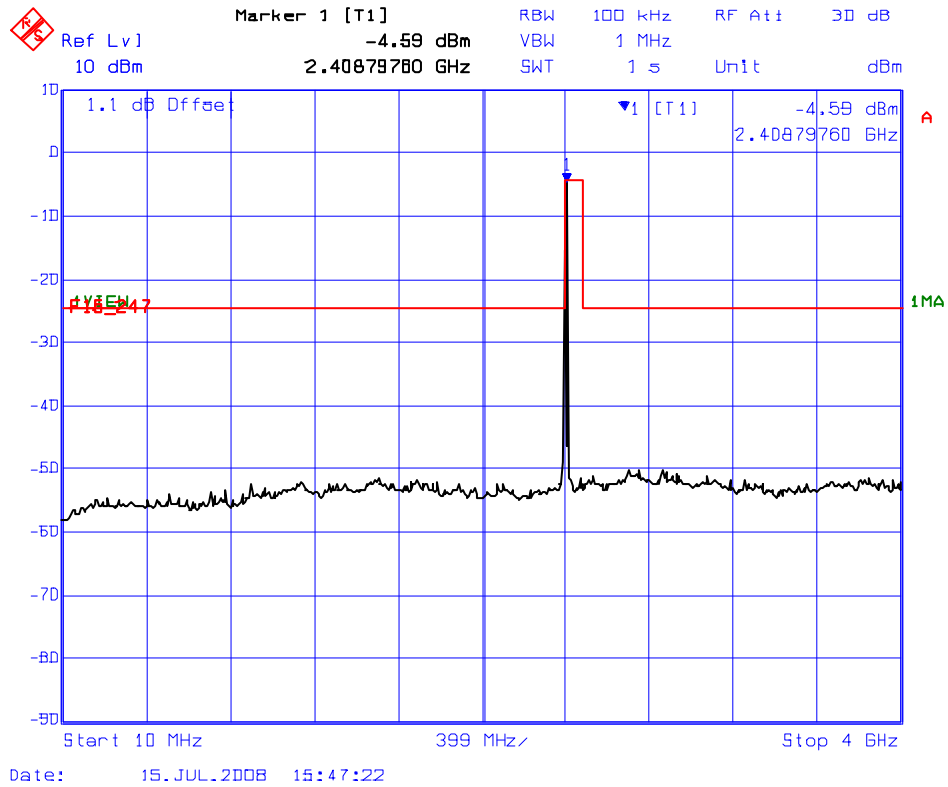
Plot 6.8.5.2.1(i) Spurious RF Conducted Emissions Transmitter Frequency: 2405 MHz
