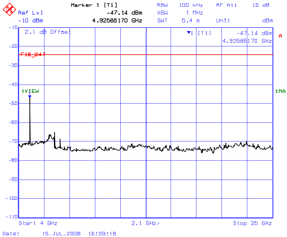
Plot 6.8.5.2.3(ii) Spurious RF Conducted Emissions Transmitter Frequency: 2480 MHz
