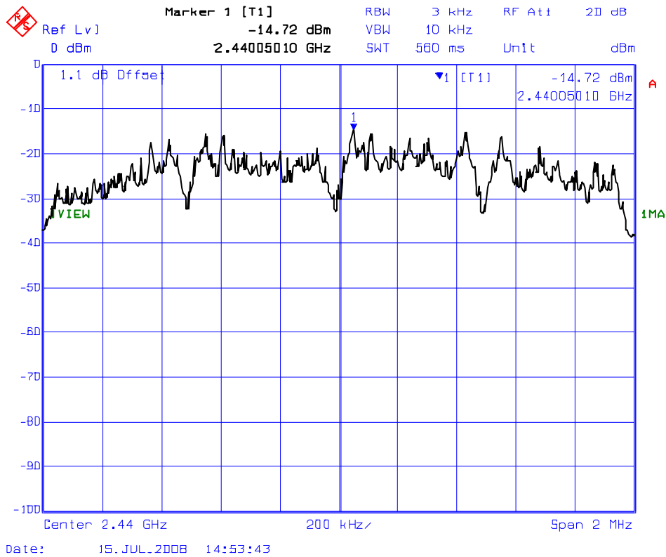
Plot 6.10.5.2 Power Spectral Density Frequency: 2440 MHz
