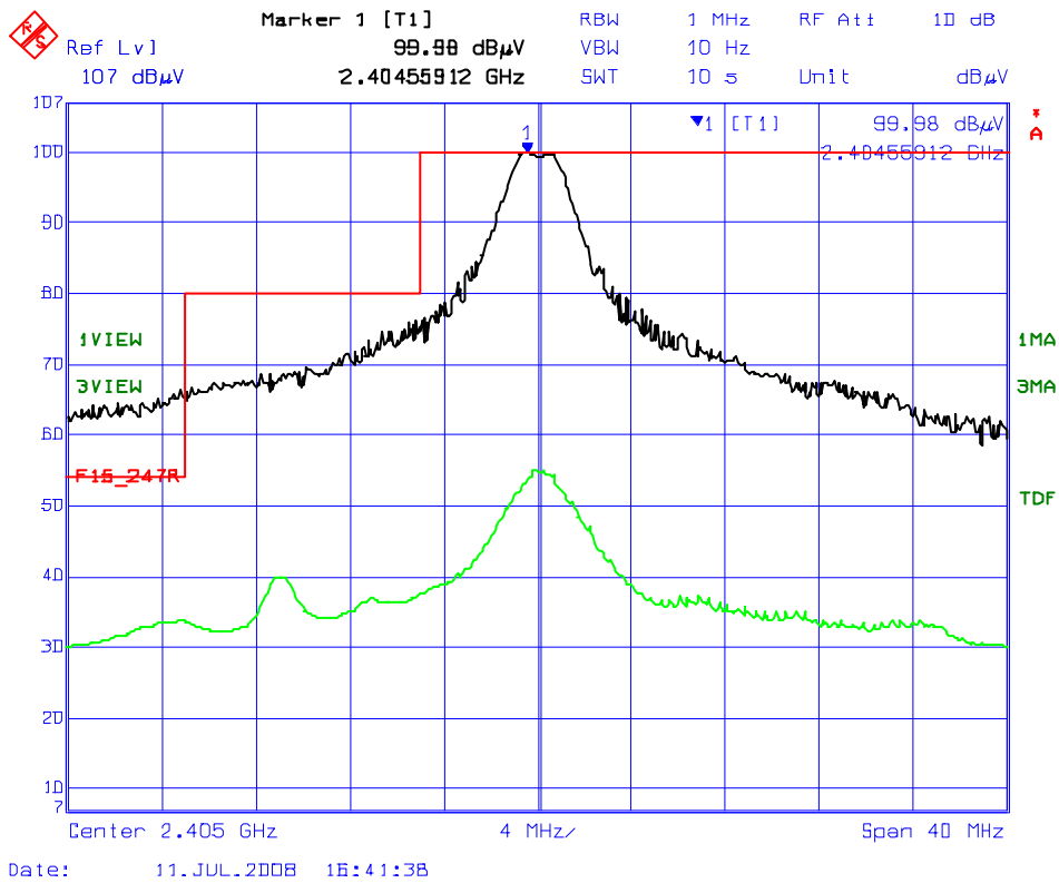
Plot 6.9.5.1 Band-Edge RF Radiated Emissions @ 3 m Low End of Frequency Band Rx Antenna Orientation: Horizontal
