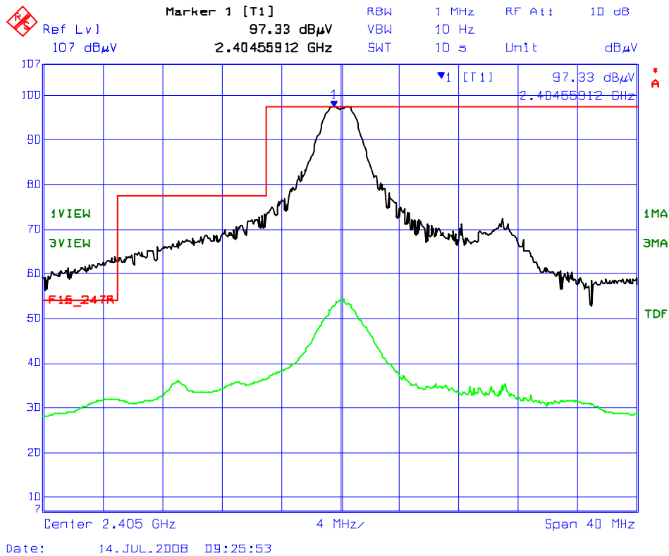
Plot 6.9.5.2 Band-Edge RF Radiated Emissions @ 3 m Low End of Frequency Band Rx Antenna Orientation: Vertical
