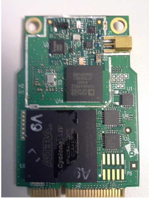
Internal Top
