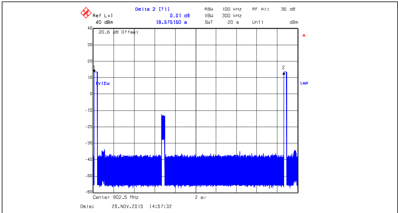
Plot 5.3.4.49. Time of Occupancy, 902.5 MHz XB0, Data Rate at 10 kbps Average time of occupancy = 20 \times (T_{on}) / (T_{total}) = 20 \times 0.3006012s / 18.5752s = 0.3237s < 0.4s
