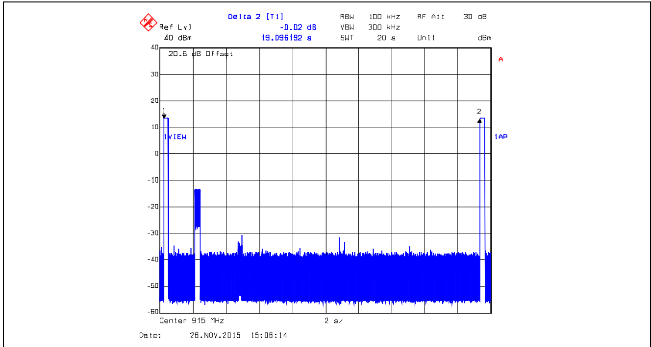
Plot 5.3.4.51. Time of Occupancy, 915 MHz XB0, Data Rate at 10 kbps Average time of occupancy = 20 \times (T_{on}) / (T_{total}) = 20 \times 0.3006012s / 19.0962s = 0.3148s < 0.4s
