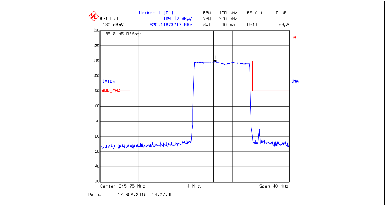
Plot 5.5.4.2.52. Band-Edge RF Radiated Emissions at 3 m, Vertical Polarization Pseudorandom Hopping Mode, Low End of Frequency Band, 915.75 MHz, XTCA1, Data Rate at 105kbps
