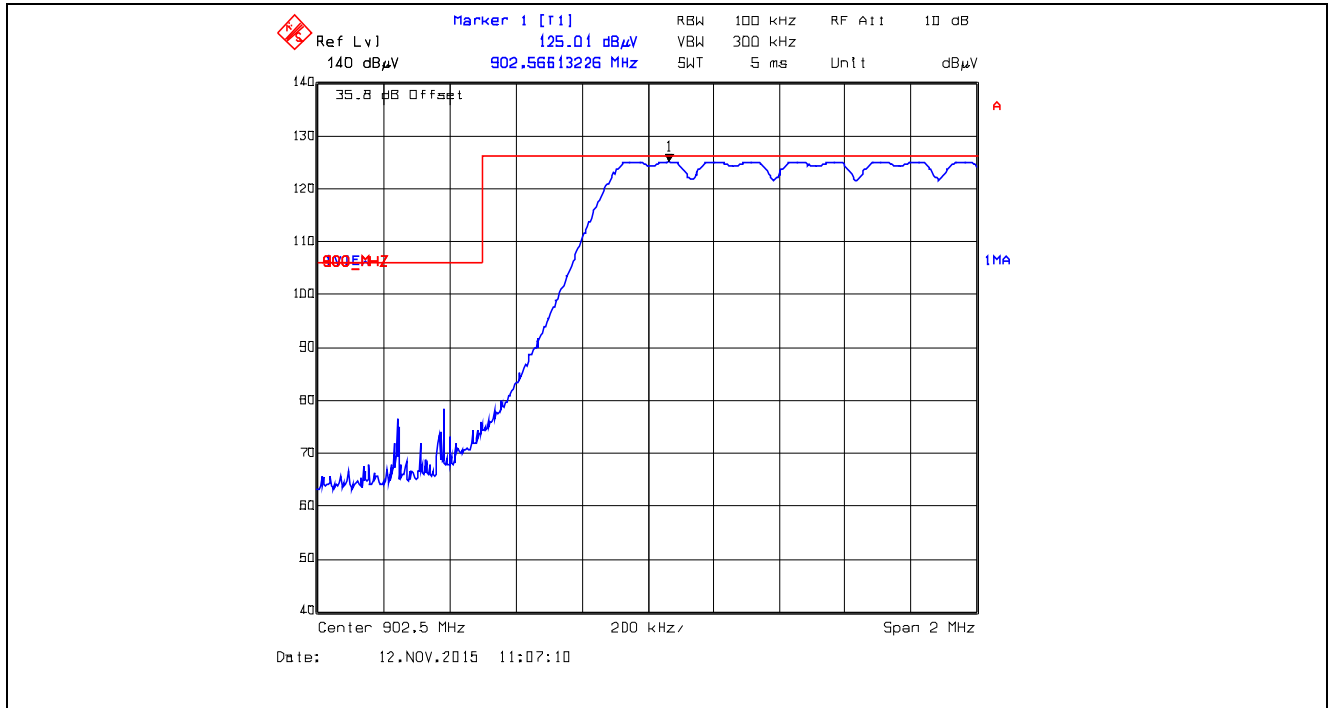
Plot 5.5.4.5.2.12. Band-Edge RF Radiated Emissions at 3 m, Vertical Polarization Pseudorandom Hopping Mode, Low End of Frequency Band, 902.5 MHz, XB1, Data Rate at 110 kbps
