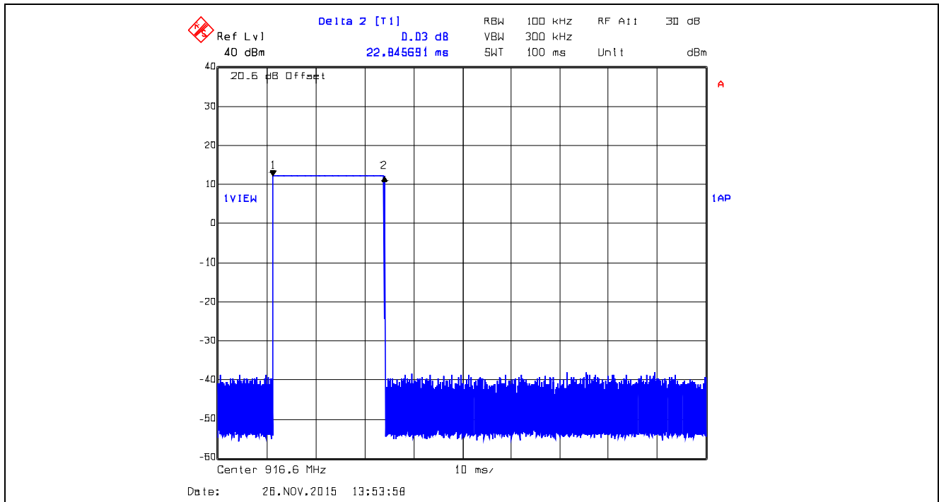
Plot 5.3.4.74. Time of Occupancy, 916.6 MHz, XTC1, Data Rate at 125 kbps Dwell Time @ 916.6 MHz = 22.8457 ms
