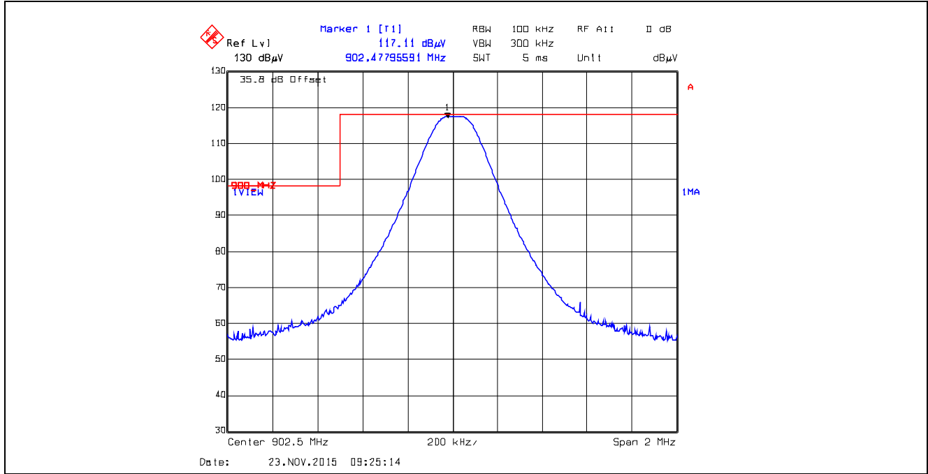
Plot 5.5.4.4.2.1. Band-Edge RF Radiated Emissions at 3 m, Horizontal Polarization Single Frequency Mode, Low End of Frequency Band, 902.5 MHz, XB0, Data Rate at 10 kbps
