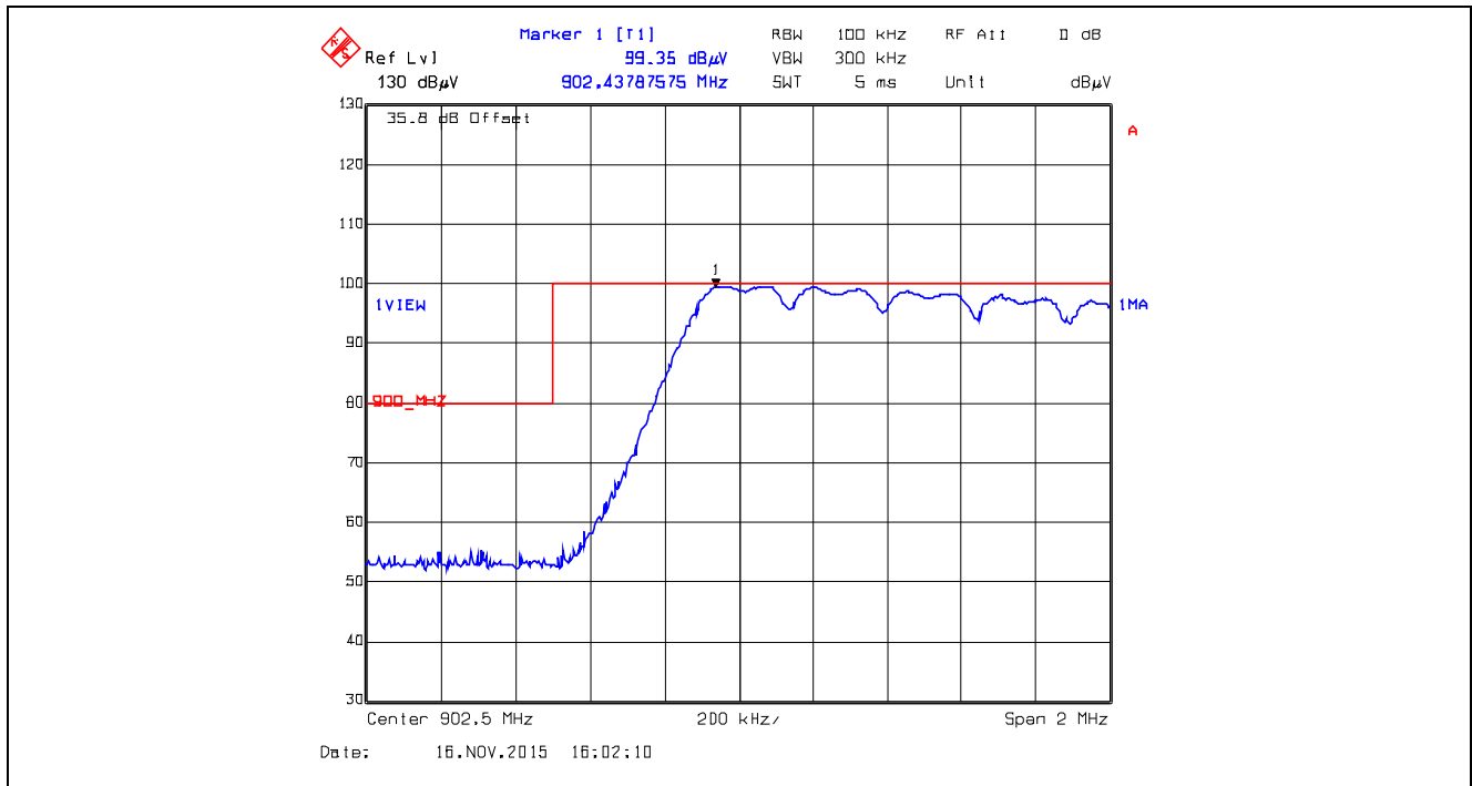
Plot 5.5.4.2.2.10. Band-Edge RF Radiated Emissions at 3 m, Horizontal Polarization Pseudorandom Hopping Mode, Low End of Frequency Band, 902.5 MHz, XB1, Data Rate at 110 kbps
