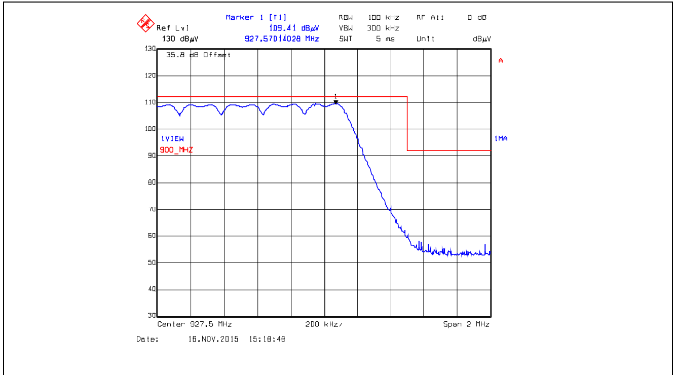
Plot 5.5.4.2.16. Band-Edge RF Radiated Emissions at 3 m, Vertical Polarization Pseudorandom Hopping Mode, High End of Frequency Band, 927.5 MHz, XBX1, Data Rate at 110 kbps
