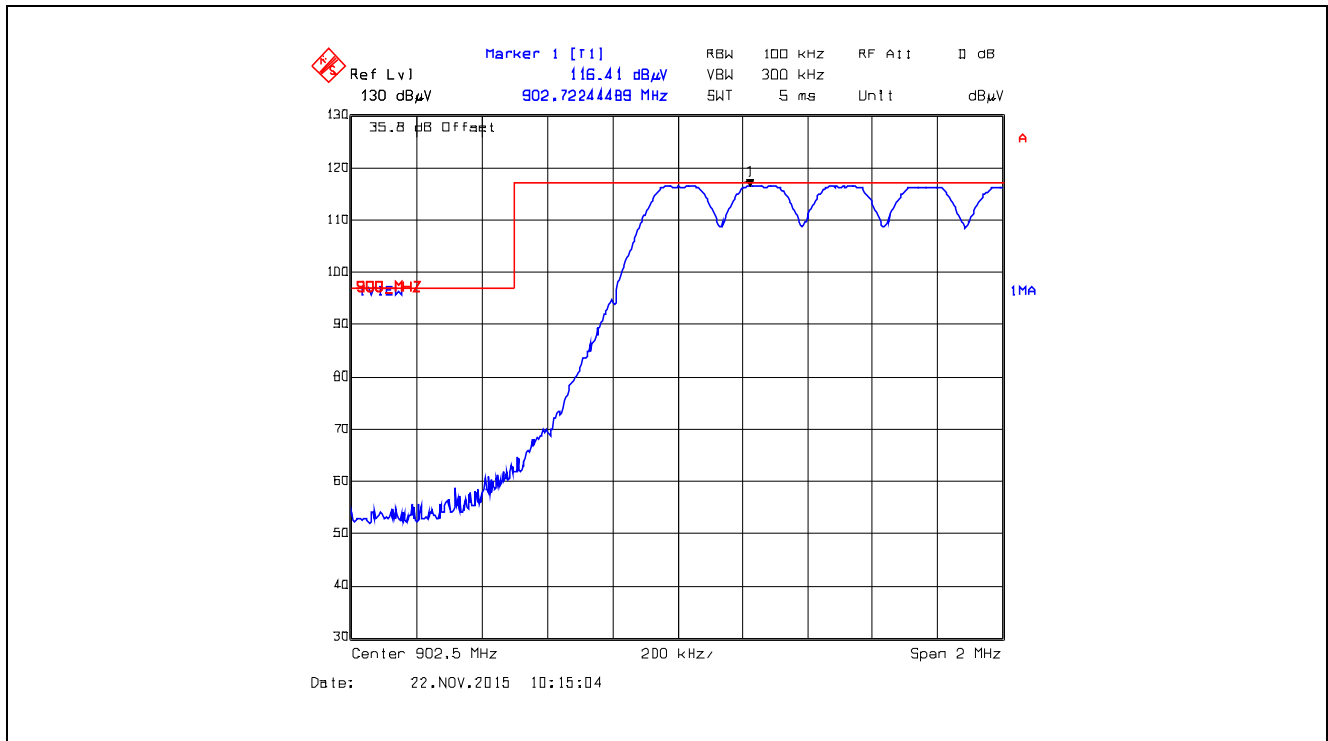
Plot 5.5.4.4.2.4. Band-Edge RF Radiated Emissions at 3 m, Vertical Polarization Pseudorandom Hopping Mode, Low End of Frequency Band, 902.5 MHz, XB0, Data Rate at 10 kbps
