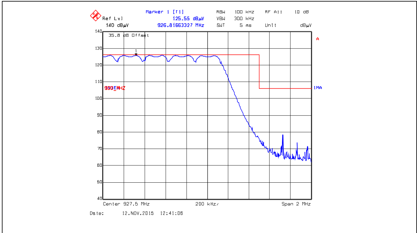
Plot 5.5.4.5.2.16. Band-Edge RF Radiated Emissions at 3 m, Vertical Polarization Pseudorandom Hopping Mode, High End of Frequency Band, 927.5 MHz, XB1, Data Rate at 110 kbps
