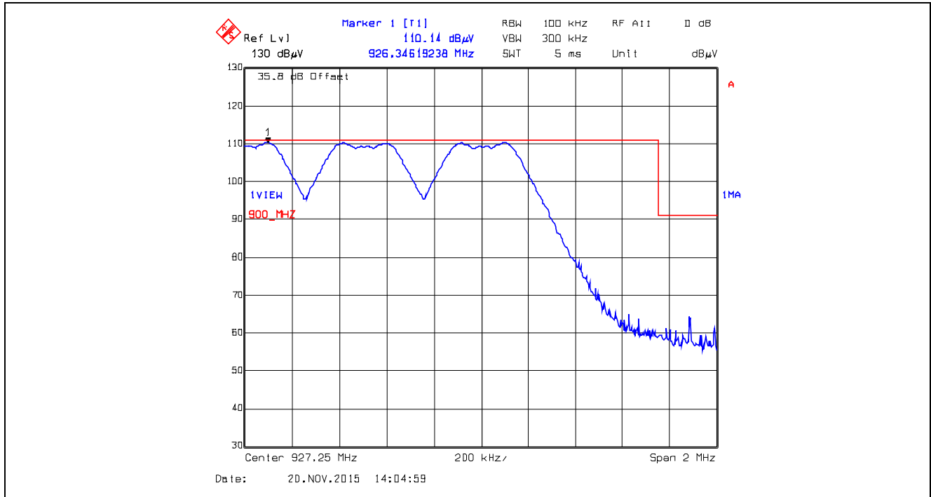
Plot 5.5.4.1.2.22. Band-Edge RF Radiated Emissions at 3 m, Horizontal Polarization Pseudorandom Hopping Mode, High End of Frequency Band, 927.25 MHz, XB2, Data Rate at 250 kbps
