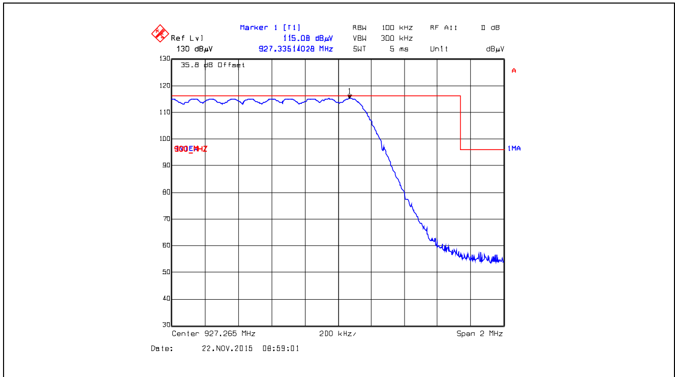
Plot 5.5.4.4.28. Band-Edge RF Radiated Emissions at 3 m, Vertical Polarization Pseudorandom Hopping Mode, High End of Frequency Band, 927.265 MHz, XTCA0, Data Rate at 10 kbps
