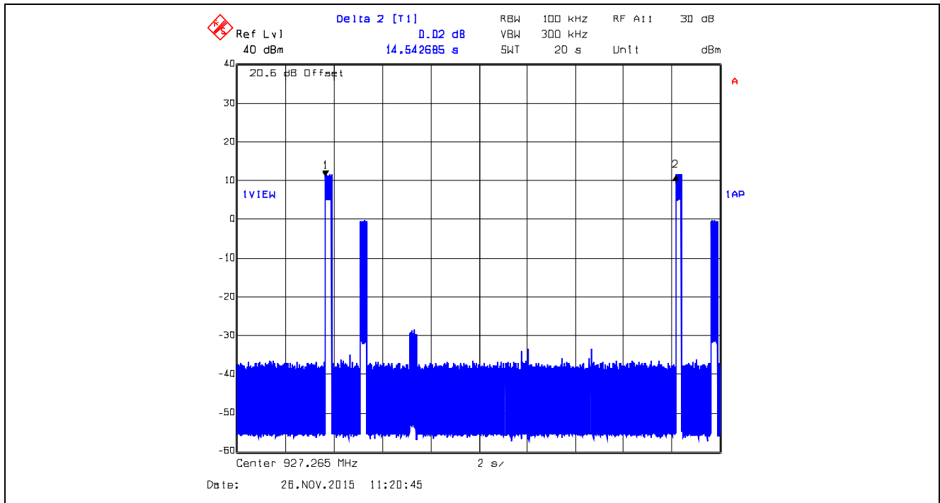
Plot 5.3.4.83. Time of Occupancy, 927.265 MHz XTCA0, Data Rate at 10 kbps Average time of occupancy = 20 \times (T_{on}) / (T_{total}) = 20 \times 0.2729459s / 14.5427s = 0.3754s < 0.4s
