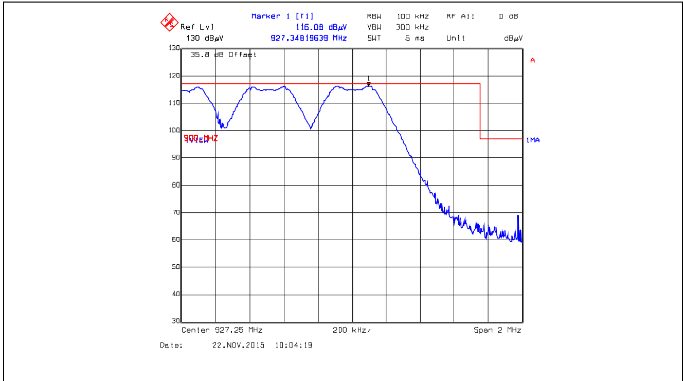
Plot 5.5.4.4.24. Band-Edge RF Radiated Emissions at 3 m, Vertical Polarization Pseudorandom Hopping Mode, High End of Frequency Band, 927.25 MHz, XB2, Data Rate at 250 kbps
