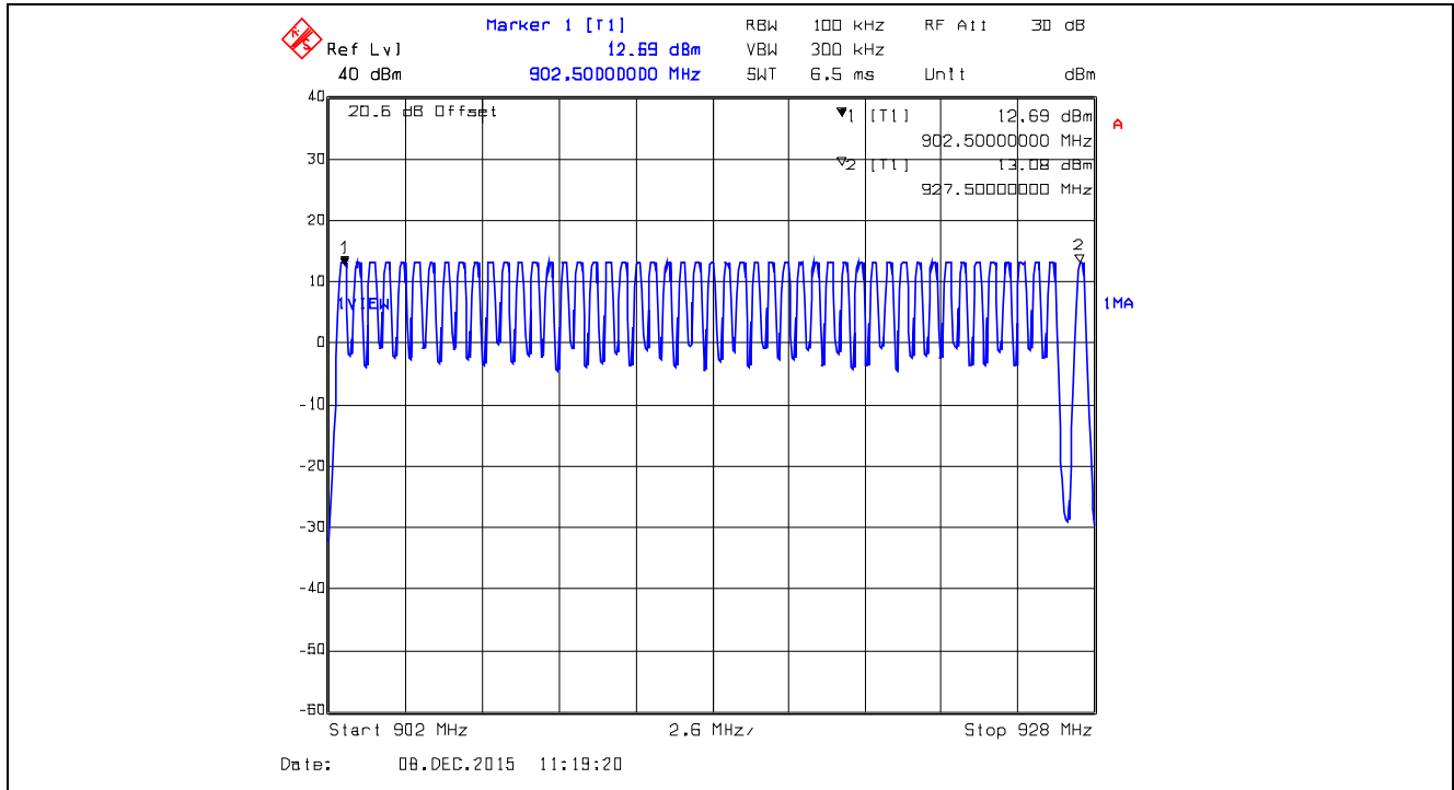
Plot 5.3.4.30. Number of Hopping Frequencies, XB1, Data Rate at 110 kbps 50 Hopping Channels from 902 – 928 MHz
