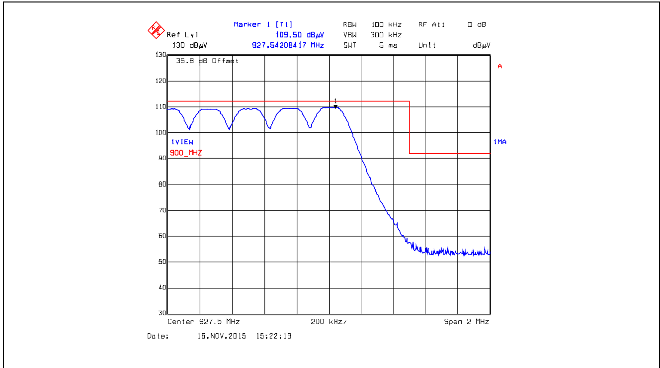
Plot 5.5.4.2.8. Band-Edge RF Radiated Emissions at 3 m, Vertical Polarization Pseudorandom Hopping Mode, High End of Frequency Band, 927.5 MHz, XBX0, Data Rate at 10 kbps
