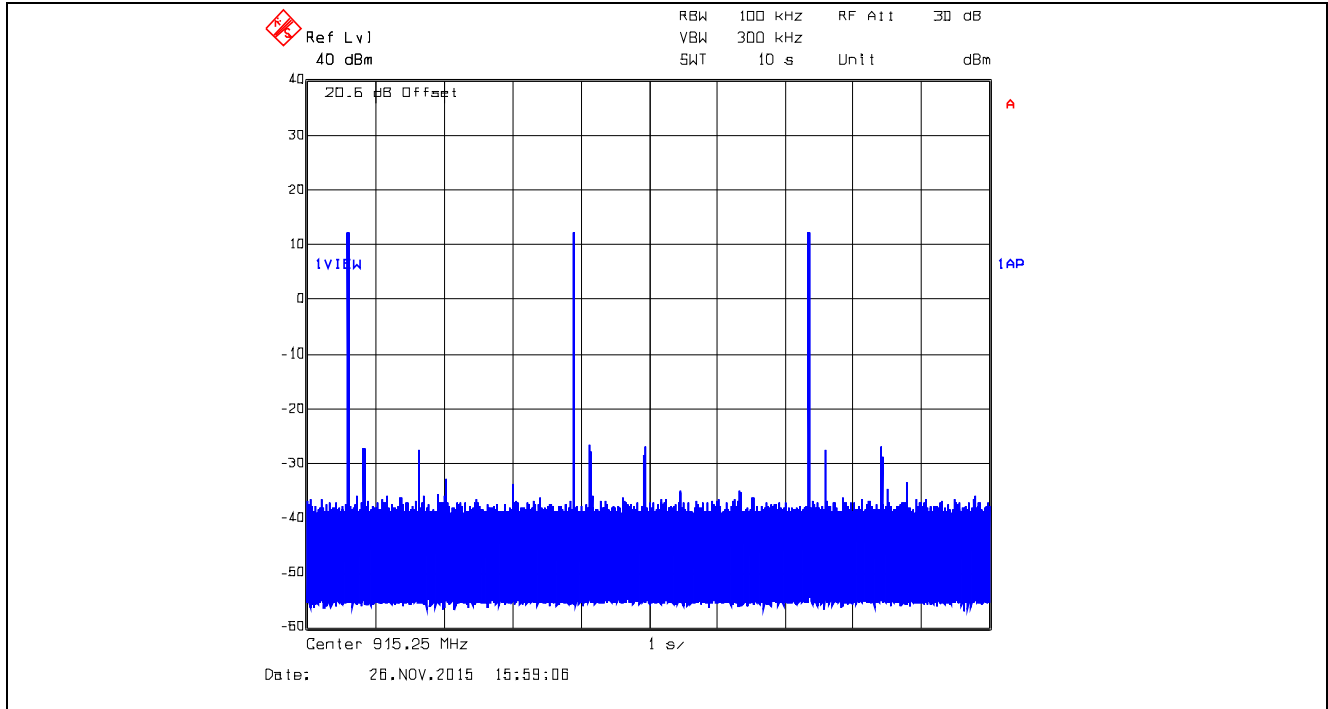
Plot 5.3.4.63. Time of Occupancy, 915.25 MHz, XB2, Data Rate at 250 kbps Average time of occupancy = (Dwell Time) x (number of hops) = 15.4309 ms x 3 = 46.2927 ms < 0.4 sec within 10 sec
