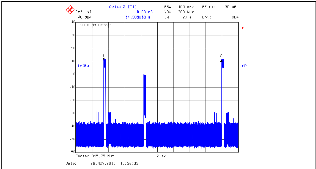
Plot 5.3.4.79. Time of Occupancy, 915.75 MHz XTCA0, Data Rate at 10 kbps Average time of occupancy = 20 \times (T_{on}) / (T_{total}) = 20 \times 0.2729459s / 14.5090s = 0.3762s < 0.4s
