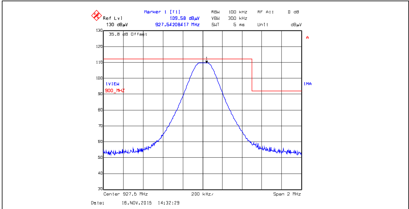
Plot 5.5.4.2.7. Band-Edge RF Radiated Emissions at 3 m, Vertical Polarization Single Frequency Mode, High End of Frequency Band, 927.5 MHz, XBX0, Data Rate at 10 kbps
