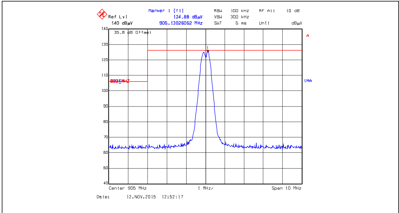
Plot 5.5.4.5.27. Band-Edge RF Radiated Emissions at 3 m, Vertical Polarization Single Frequency Mode, Low End of Frequency Band, 905.0 MHz, XTC0, Data Rate at 10 kbps
