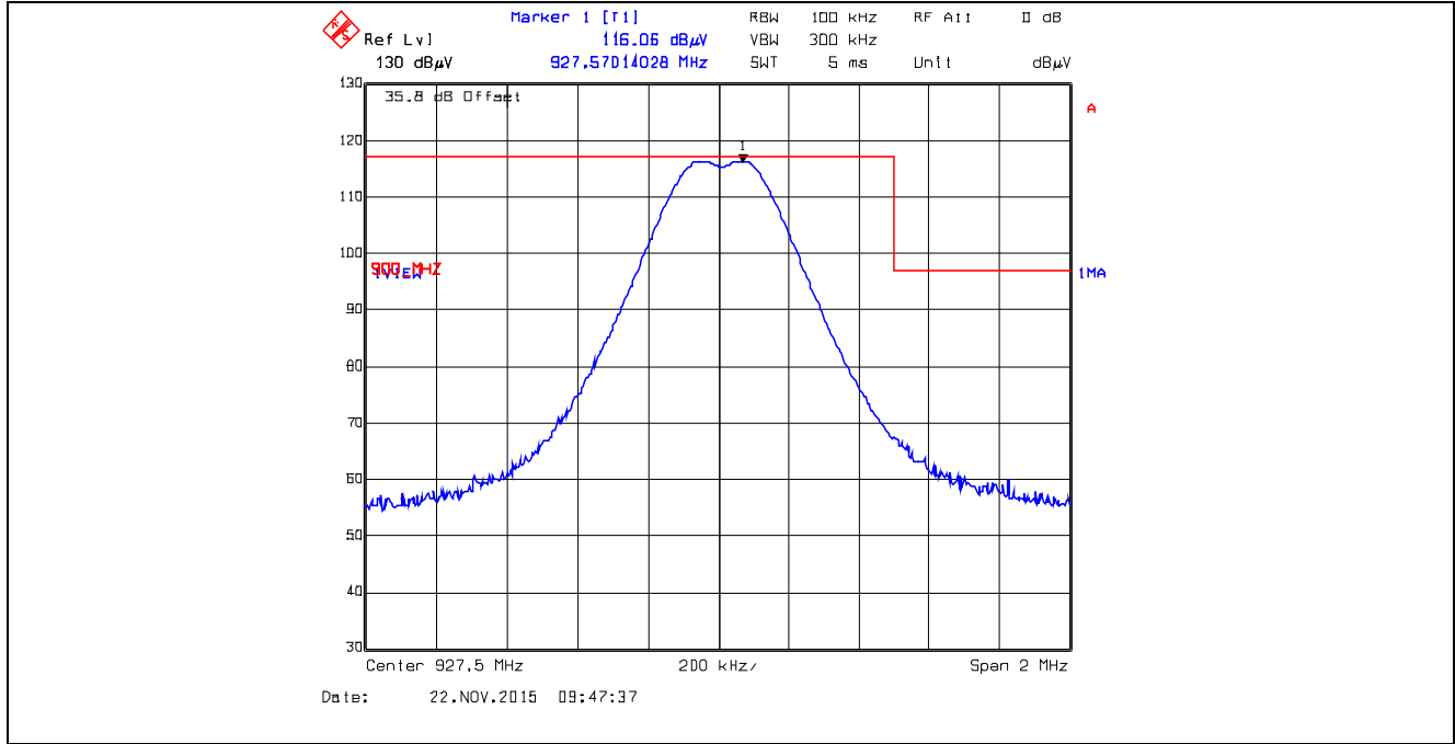
Plot 5.5.4.4.2.15. Band-Edge RF Radiated Emissions at 3 m, Vertical Polarization Single Frequency Mode, High End of Frequency Band, 927.5 MHz, XB1, Data Rate at 110 kbps
