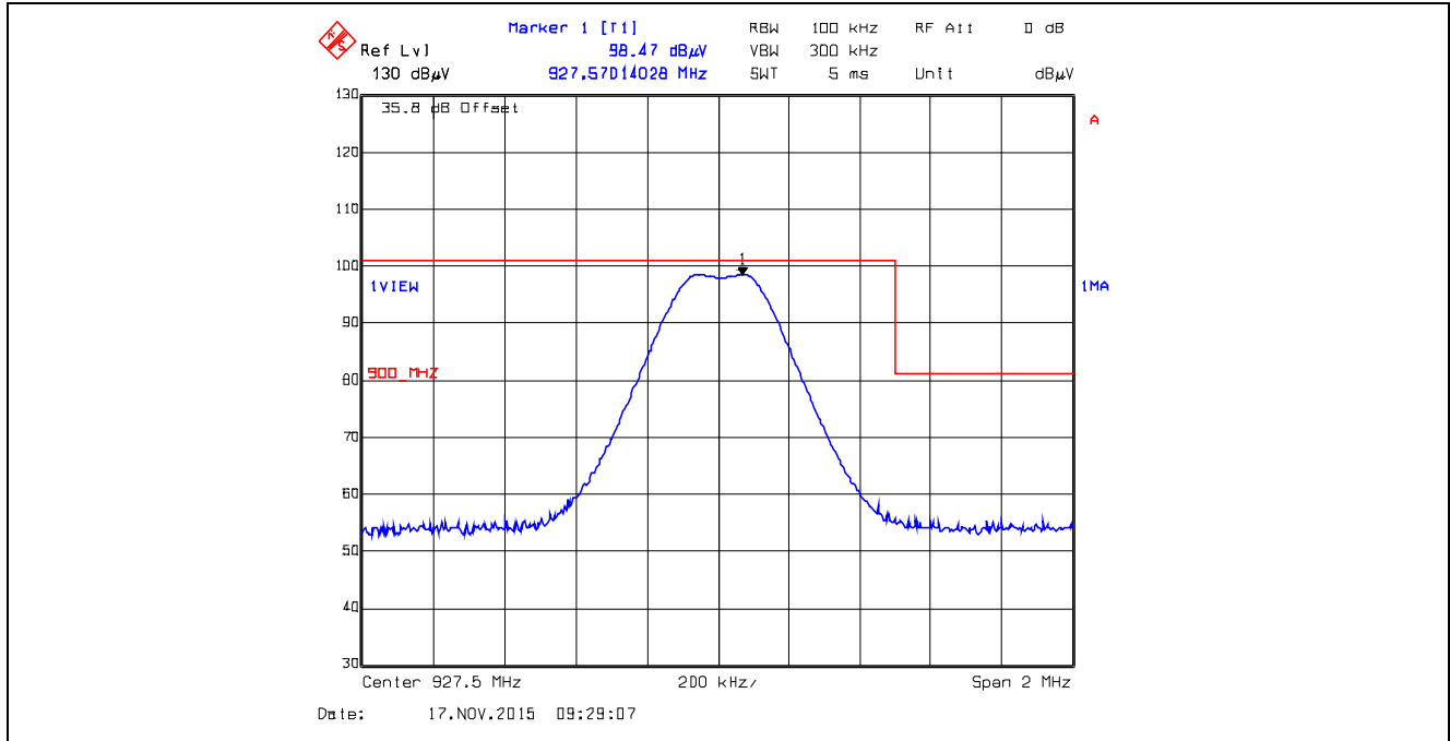
Plot 5.5.4.2.2.13. Band-Edge RF Radiated Emissions at 3 m, Horizontal Polarization Single Frequency Mode, High End of Frequency Band, 927.5 MHz, XB1, Data Rate at 110 kbps
