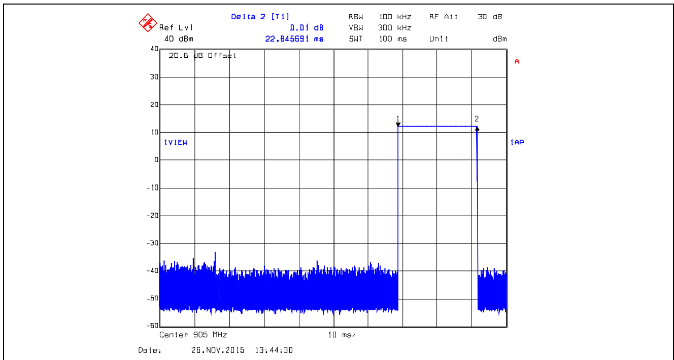
Plot 5.3.4.72. Time of Occupancy, 905 MHz, XTC1, Data Rate at 125 kbps Dwell Time @ 905 MHz = 22.8457 ms
