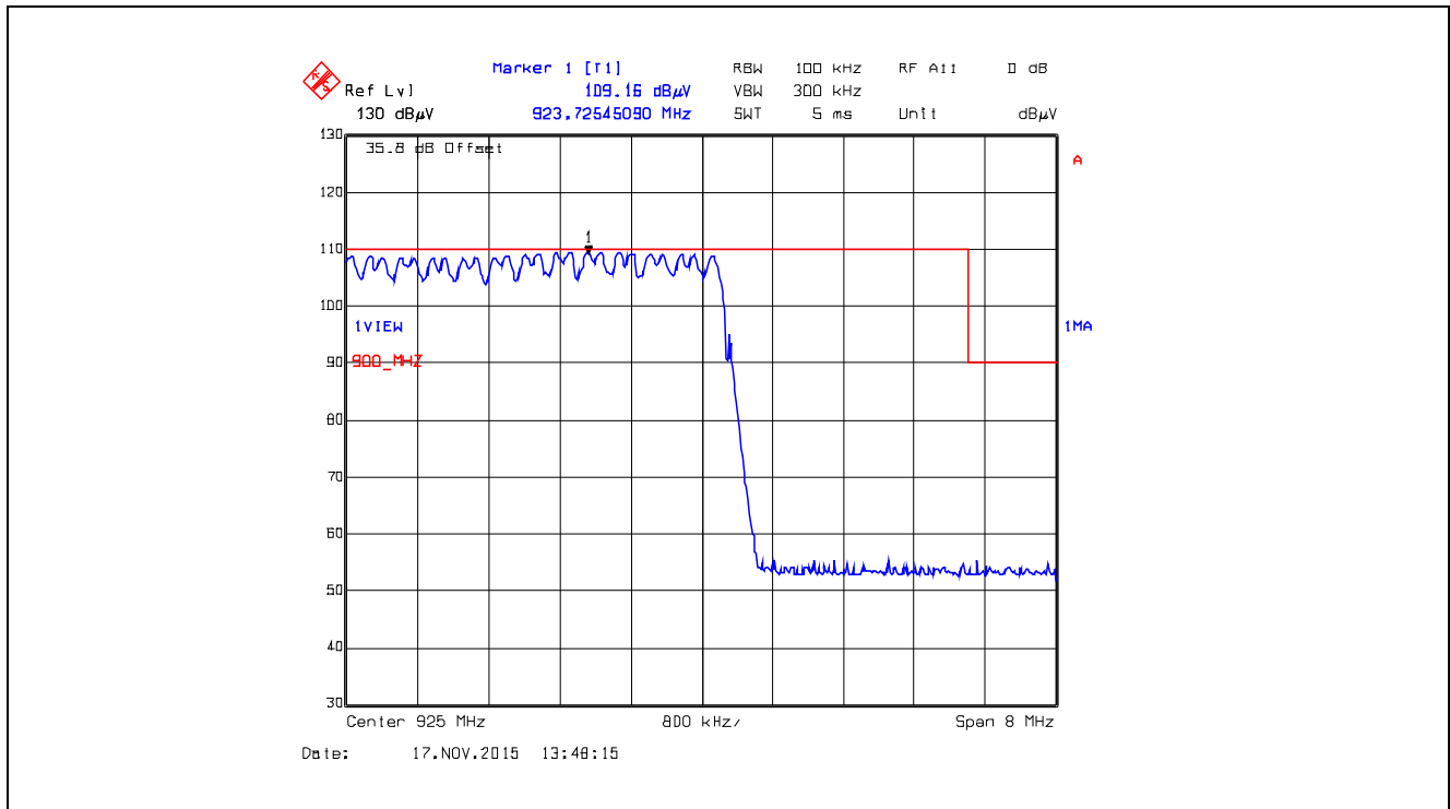
Plot 5.5.4.2.32. Band-Edge RF Radiated Emissions at 3 m, Vertical Polarization Pseudorandom Hopping Mode, High End of Frequency Band, 925.0 MHz, XTC0, Data Rate at 10 kbps
