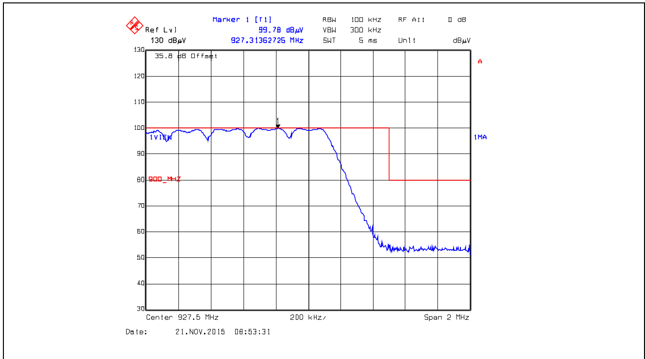
Plot 5.5.4.3.2.14. Band-Edge RF Radiated Emissions at 3 m, Horizontal Polarization Pseudorandom Hopping Mode, High End of Frequency Band, 927.5 MHz, XB1, Data Rate at 110 kbps
