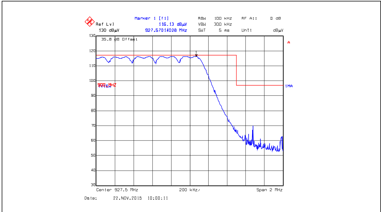
Plot 5.5.4.4.2.16. Band-Edge RF Radiated Emissions at 3 m, Vertical Polarization Pseudorandom Hopping Mode, High End of Frequency Band, 927.5 MHz, XB1, Data Rate at 110 kbps
