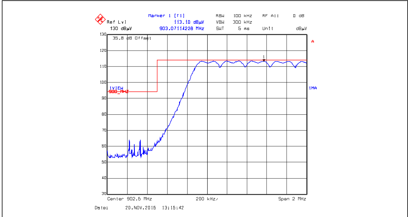
Plot 5.5.4.1.2.12. Band-Edge RF Radiated Emissions at 3 m, Vertical Polarization Pseudorandom Hopping Mode, Low End of Frequency Band, 902.5 MHz, XB1, Data Rate at 110 kbps
