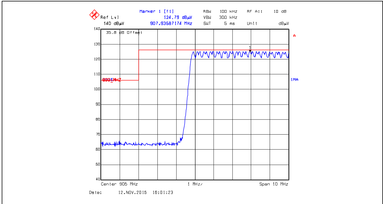
Plot 5.5.4.5.28. Band-Edge RF Radiated Emissions at 3 m, Vertical Polarization Pseudorandom Hopping Mode, Low End of Frequency Band, 905.0 MHz, XTC0, Data Rate at 10 kbps
