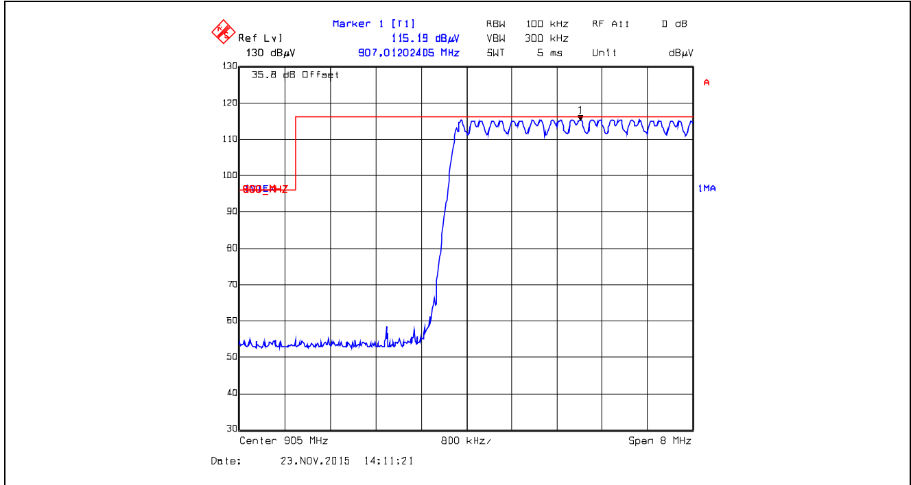
Plot 5.5.4.4.26. Band-Edge RF Radiated Emissions at 3 m, Horizontal Polarization Pseudorandom Hopping Mode, Low End of Frequency Band, 905.0 MHz, XTC0, Data Rate at 10 kbps
