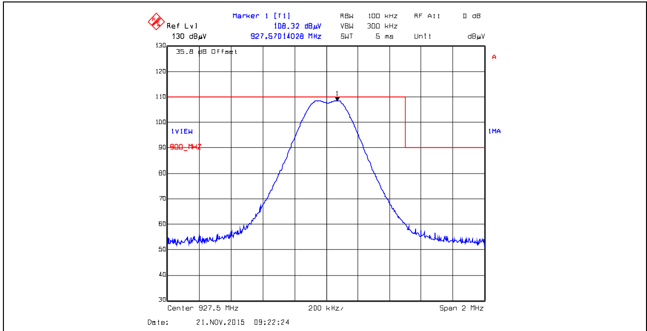
Plot 5.5.4.3.2.15. Band-Edge RF Radiated Emissions at 3 m, Vertical Polarization Single Frequency Mode, High End of Frequency Band, 927.5 MHz, XB1, Data Rate at 110 kbps
