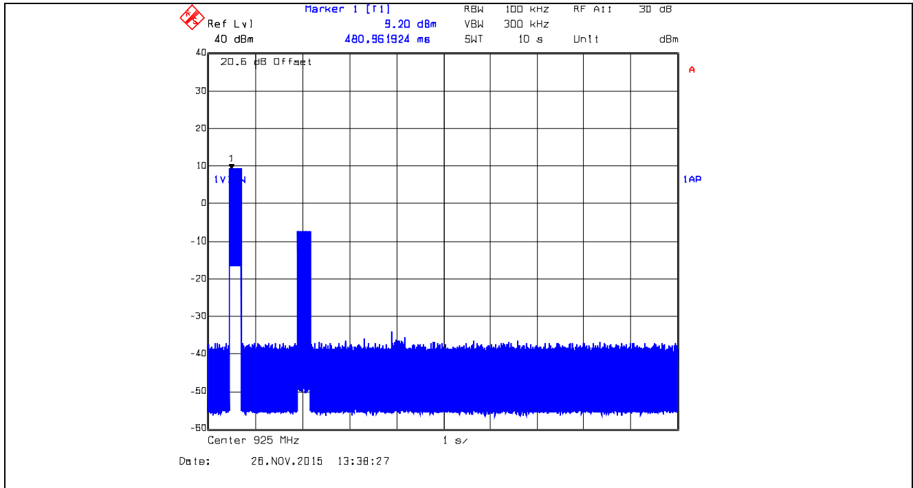
Plot 5.3.4.71. Time of Occupancy, 925.0 MHz, XTC0, Data Rate at 10 kbps Average time of occupancy = (Dwell Time) x (number of hops) = 272.55 ms x 1 = 272.55 ms < 0.4 sec within 10 sec
