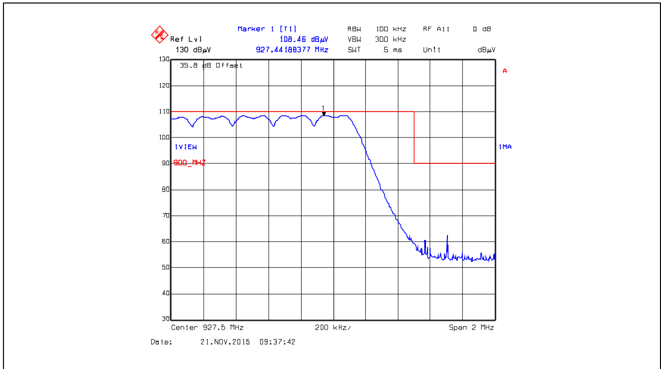
Plot 5.5.4.3.2.16. Band-Edge RF Radiated Emissions at 3 m, Vertical Polarization Pseudorandom Hopping Mode, High End of Frequency Band, 927.5 MHz, XB1, Data Rate at 110 kbps
