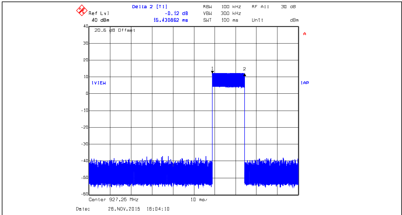
Plot 5.3.4.64. Time of Occupancy, 927.25 MHz, XB2, Data Rate at 250 kbps Dwell Time @ 927.25 MHz = 15.4309 ms
