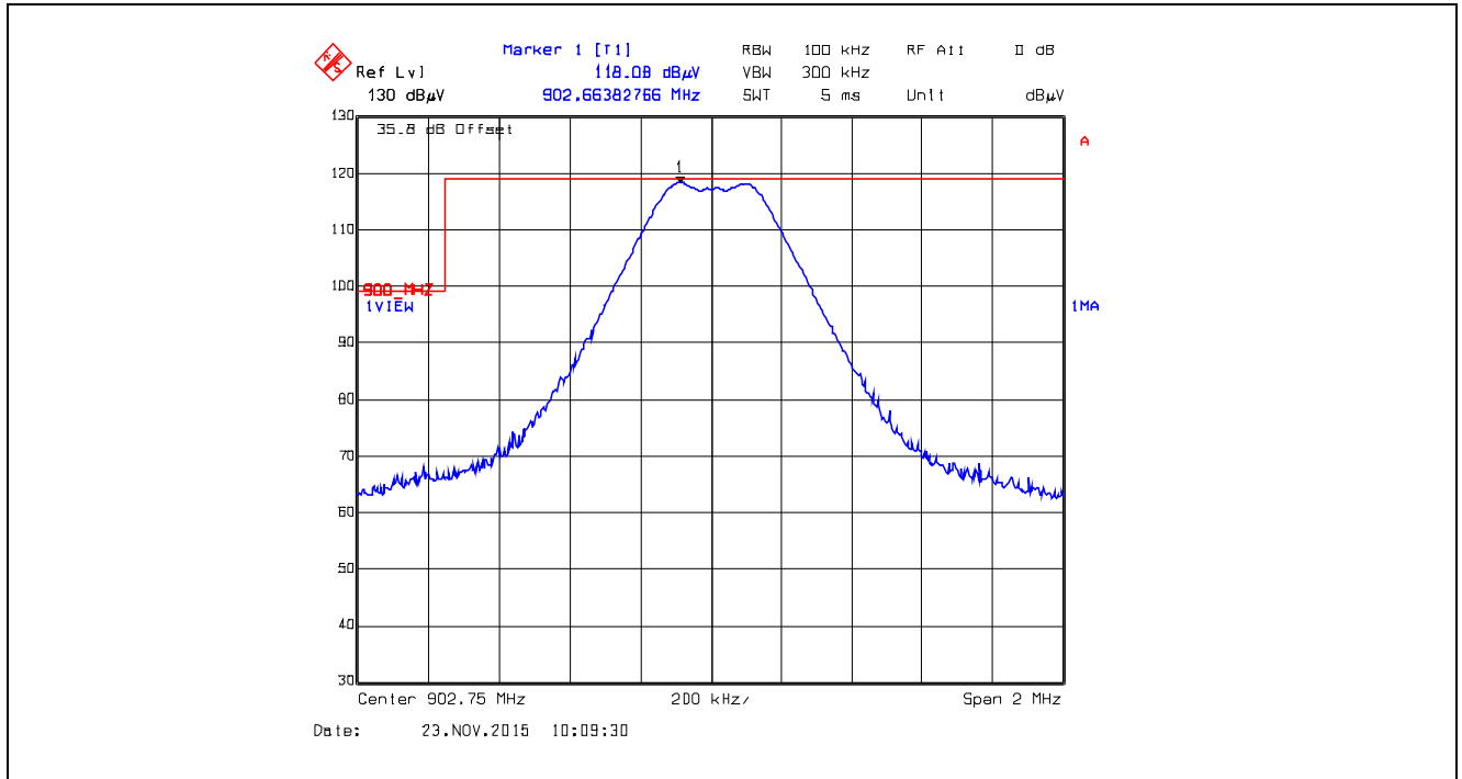
Plot 5.5.4.4.2.17. Band-Edge RF Radiated Emissions at 3 m, Horizontal Polarization Single Frequency Mode, Low End of Frequency Band, 902.75 MHz, XB2, Data Rate at 250 kbps
