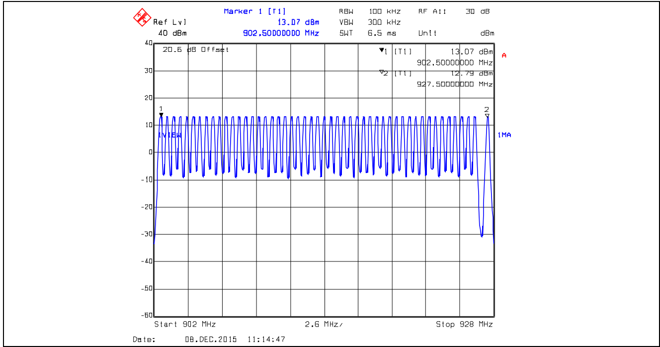
Plot 5.3.4.30. Number of Hopping Frequencies, XB1, Data Rate at 110 kbps 50 Hopping Channels from 902 – 928 MHz
