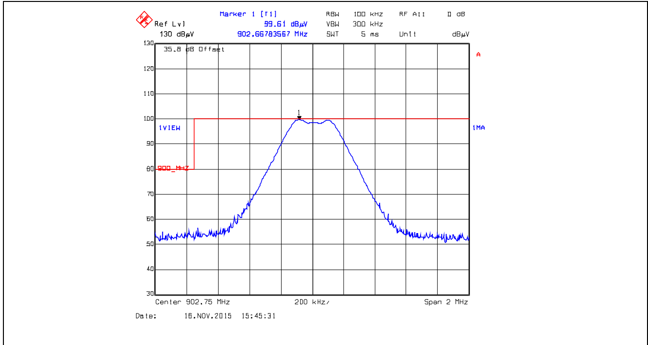
Plot 5.5.4.2.2.17. Band-Edge RF Radiated Emissions at 3 m, Horizontal Polarization Single Frequency Mode, Low End of Frequency Band, 902.75 MHz, XB2, Data Rate at 250 kbps
