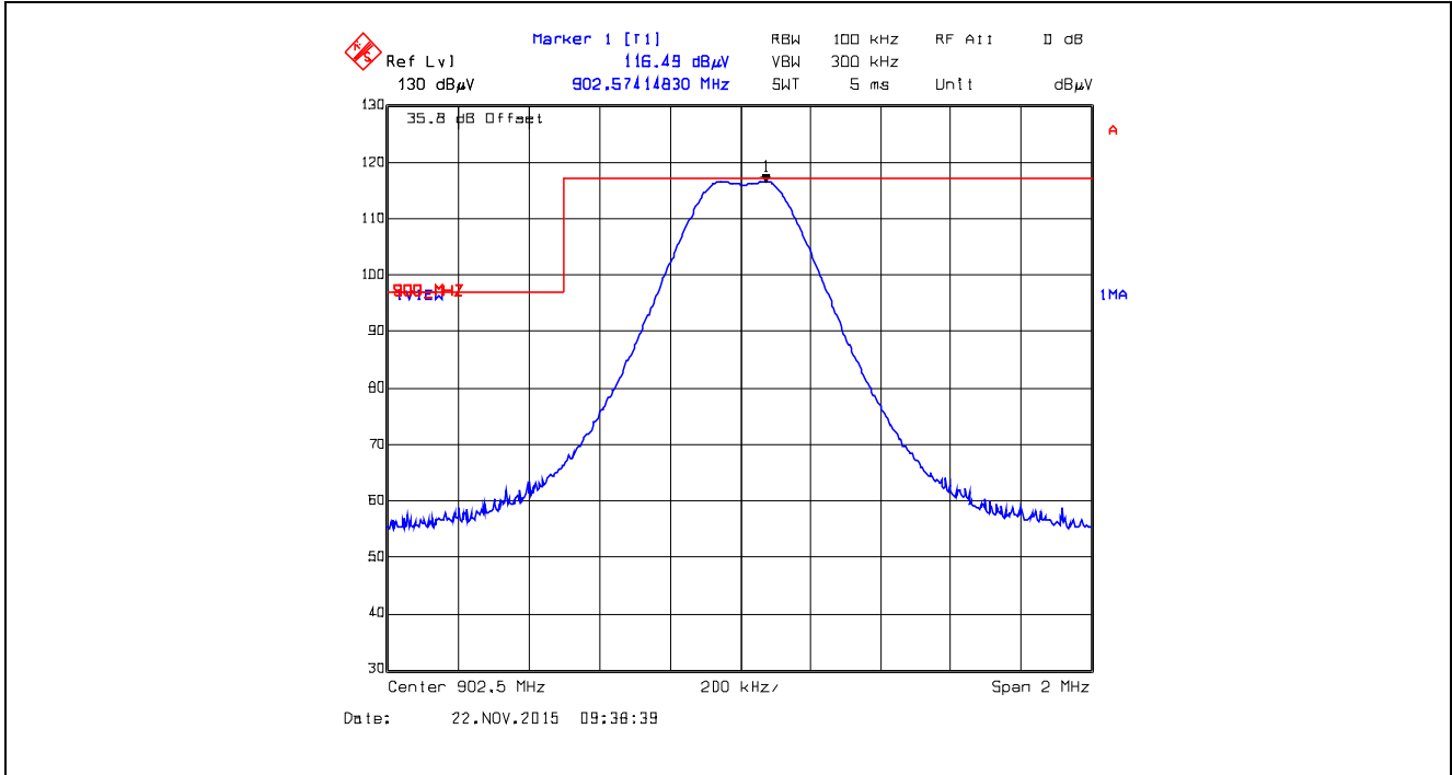
Plot 5.5.4.4.2.11. Band-Edge RF Radiated Emissions at 3 m, Vertical Polarization Single Frequency Mode, Low End of Frequency Band, 902.5 MHz, XB1, Data Rate at 110 kbps
