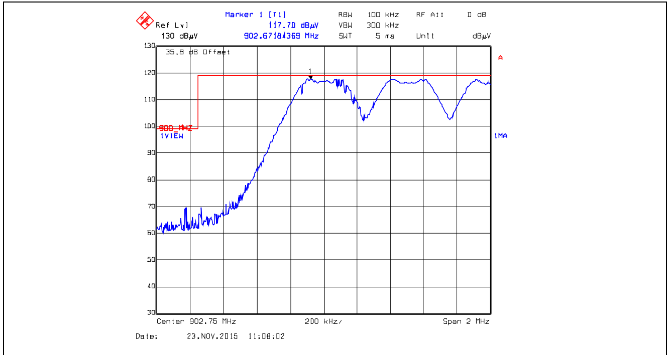
Plot 5.5.4.4.2.18. Band-Edge RF Radiated Emissions at 3 m, Horizontal Polarization Pseudorandom Hopping Mode, Low End of Frequency Band, 902.75 MHz, XB2, Data Rate at 250 kbps
