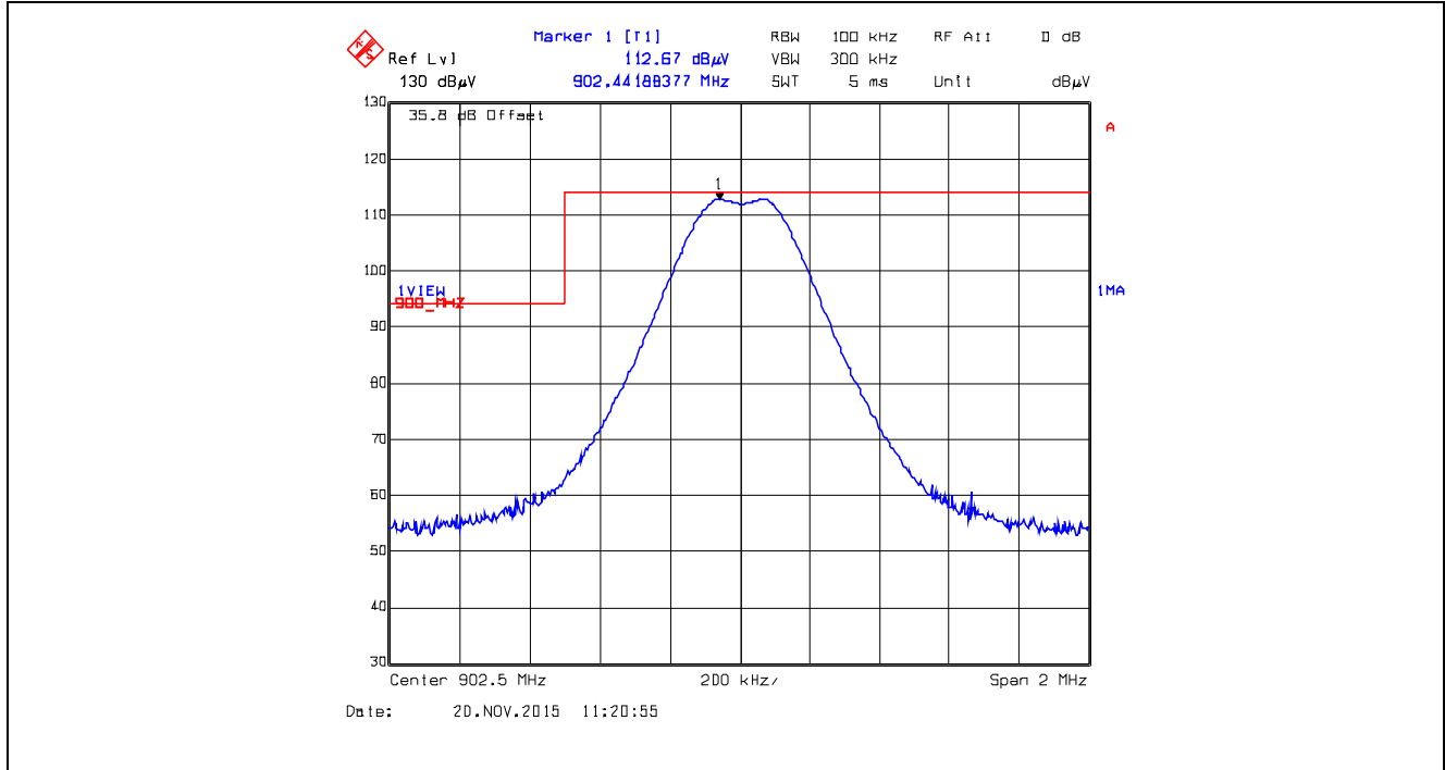
Plot 5.5.4.1.2.11. Band-Edge RF Radiated Emissions at 3 m, Vertical Polarization Single Frequency Mode, Low End of Frequency Band, 902.5 MHz, XB1, Data Rate at 110 kbps
