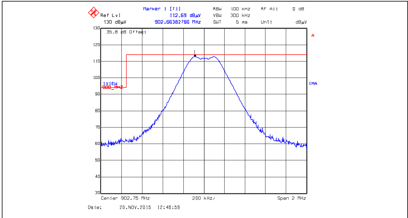
Plot 5.5.4.1.2.19. Band-Edge RF Radiated Emissions at 3 m, Vertical Polarization Single Frequency Mode, Low End of Frequency Band, 902.75 MHz, XBX2, Data Rate at 250 kbps
