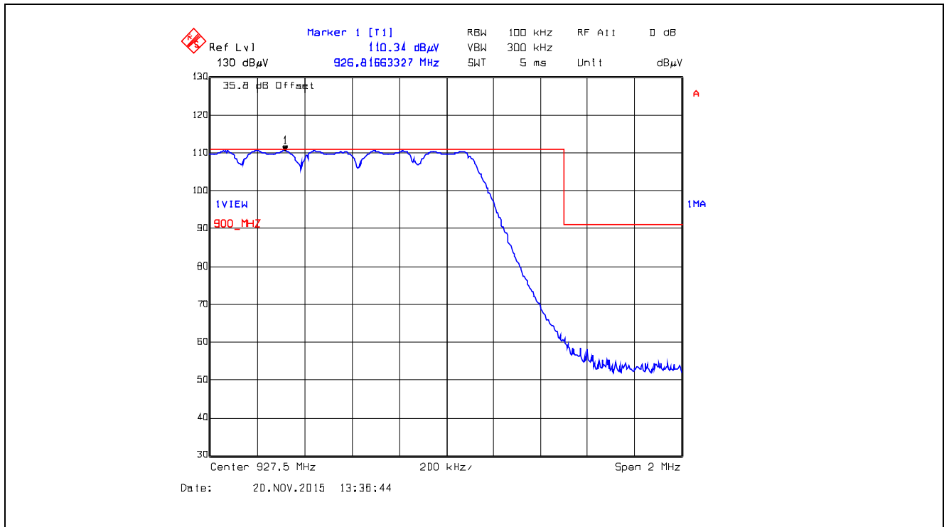
Plot 5.5.4.1.2.16. Band-Edge RF Radiated Emissions at 3 m, Vertical Polarization Pseudorandom Hopping Mode, High End of Frequency Band, 927.5 MHz, XB1, Data Rate at 110 kbps
