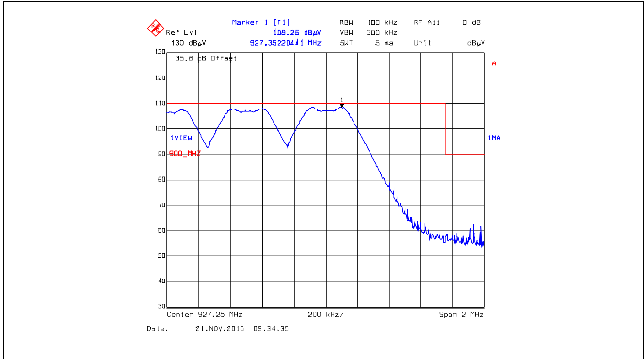
Plot 5.5.4.3.2.24. Band-Edge RF Radiated Emissions at 3 m, Vertical Polarization Pseudorandom Hopping Mode, High End of Frequency Band, 927.25 MHz, XB2, Data Rate at 250 kbps
