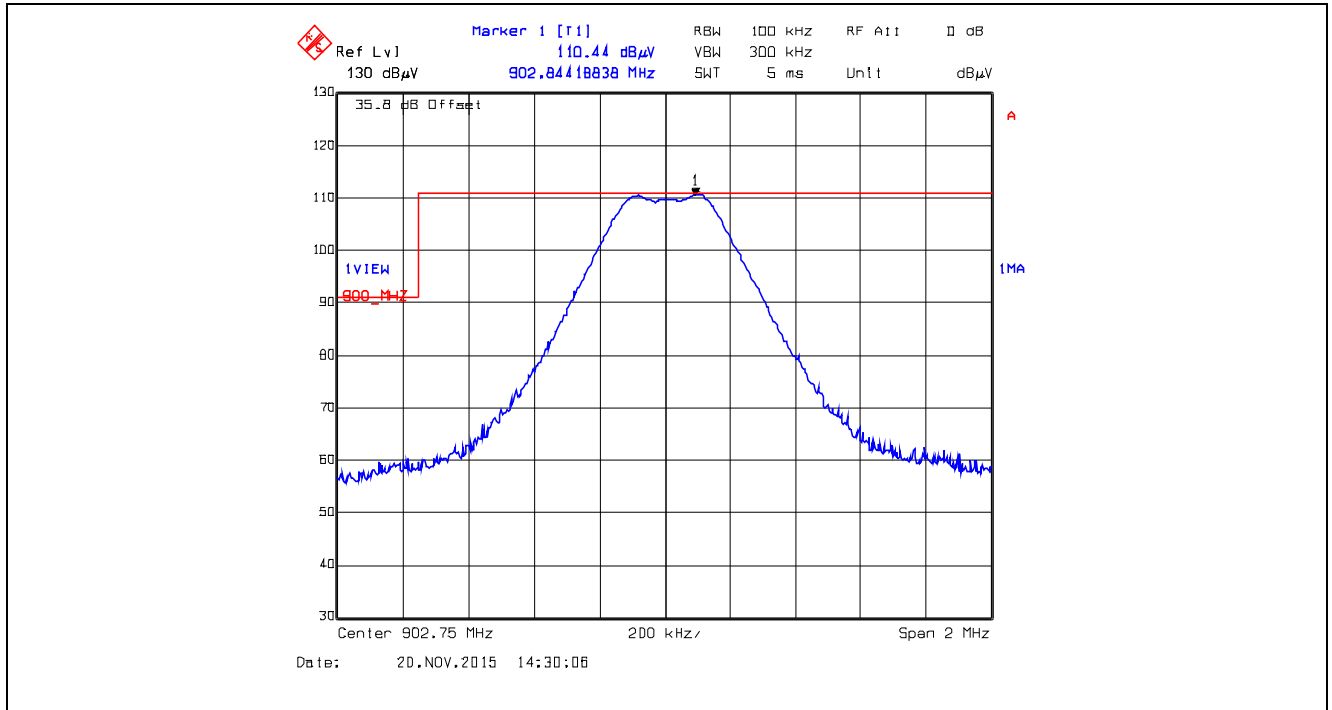
Plot 5.5.4.1.2.17. Band-Edge RF Radiated Emissions at 3 m, Horizontal Polarization Single Frequency Mode, Low End of Frequency Band, 902.75 MHz, XB2, Data Rate at 250 kbps
