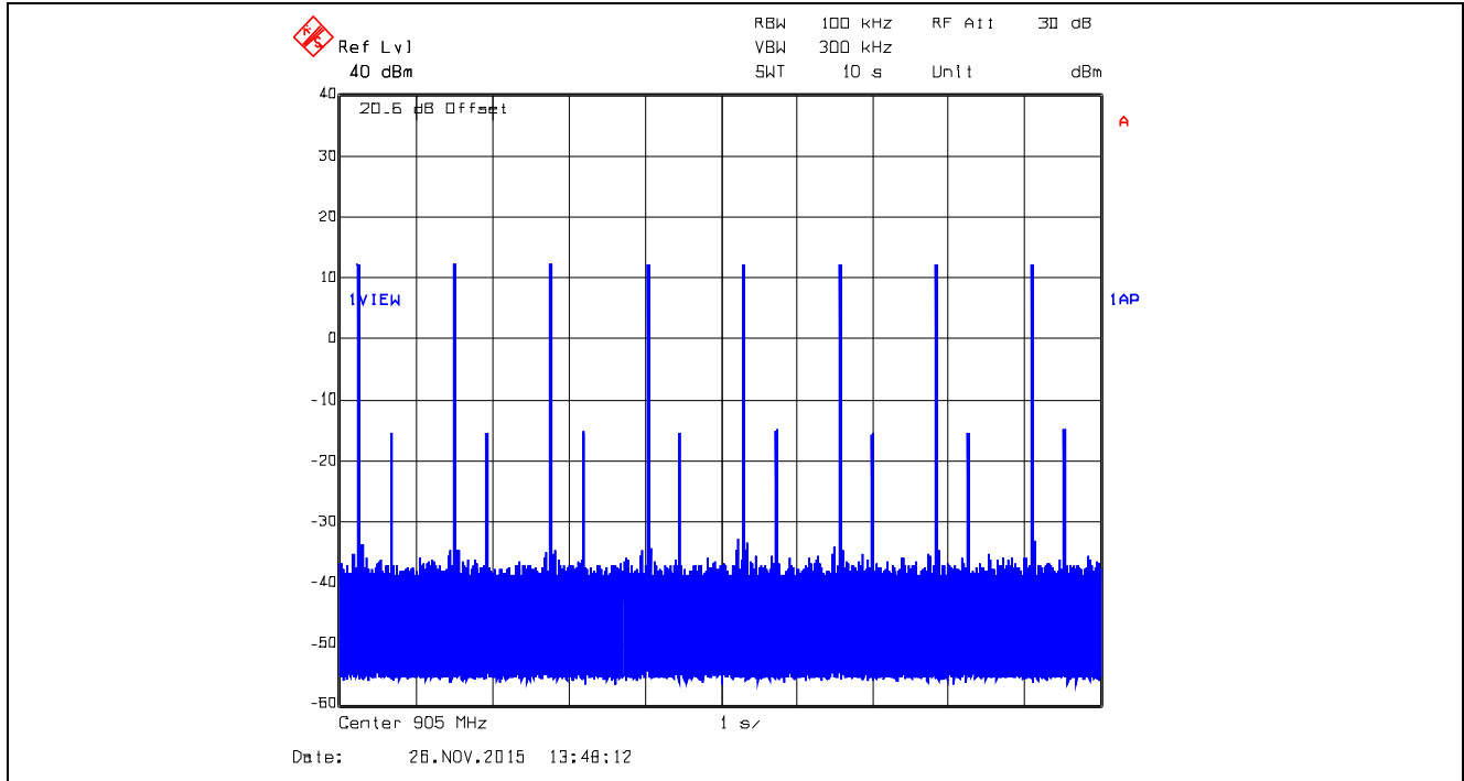
Plot 5.3.4.73. Time of Occupancy, 905 MHz, XTC1, Data Rate at 125 kbps Average time of occupancy = (Dwell Time) x (number of hops) = 22.8457ms x 8 = 182.77 ms < 0.4 sec within 10 sec
