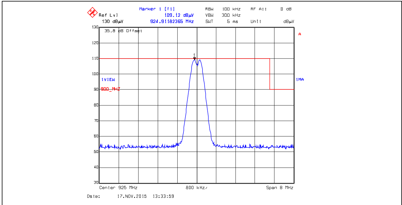
Plot 5.5.4.2.31. Band-Edge RF Radiated Emissions at 3 m, Vertical Polarization Single Frequency Mode, High End of Frequency Band, 925.0 MHz, XTC0, Data Rate at 10 kbps
