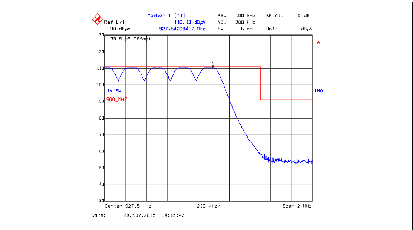
Plot 5.5.4.1.2.6. Band-Edge RF Radiated Emissions at 3 m, Horizontal Polarization Pseudorandom Hopping Mode, High End of Frequency Band, 927.5 MHz, XBX0, Data Rate at 10 kbps
