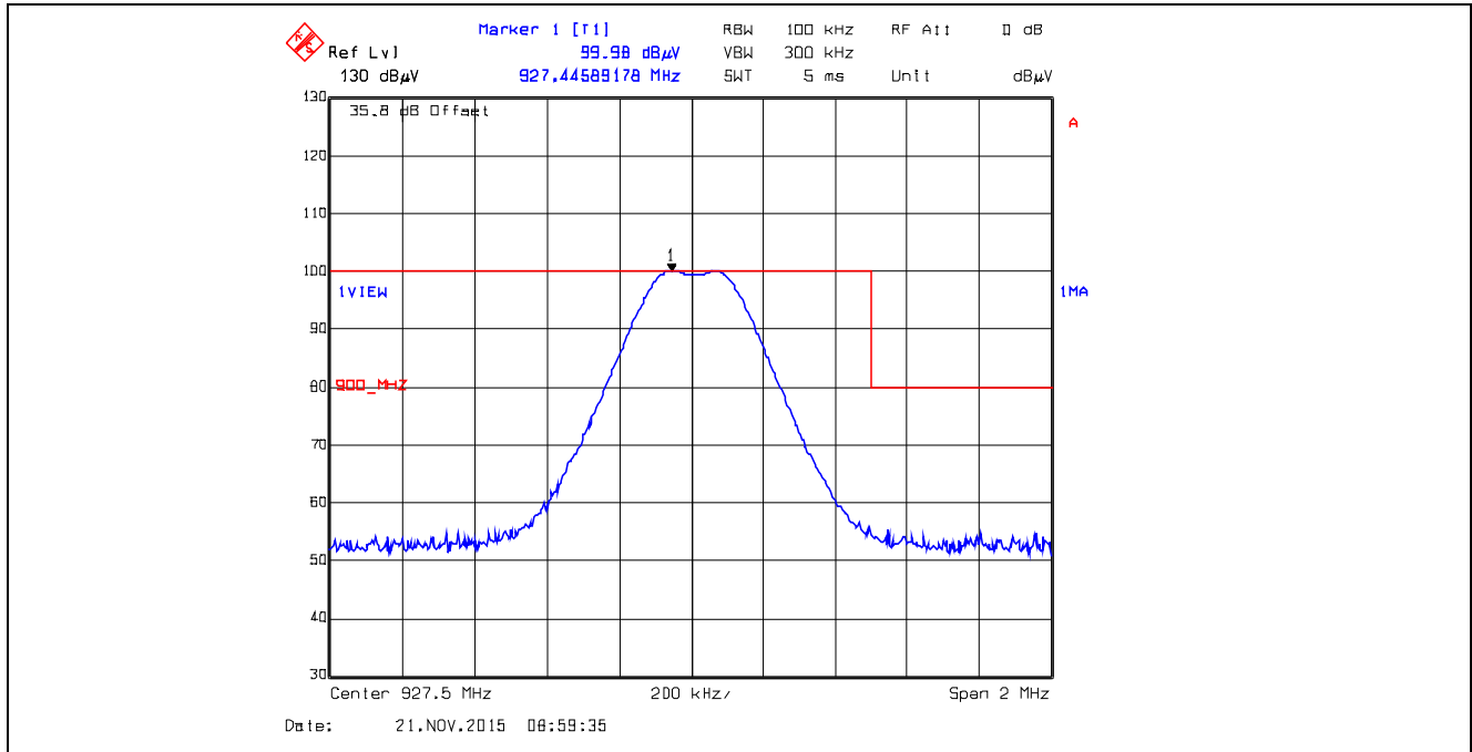
Plot 5.5.4.3.2.13. Band-Edge RF Radiated Emissions at 3 m, Horizontal Polarization Single Frequency Mode, High End of Frequency Band, 927.5 MHz, XB1, Data Rate at 110 kbps
