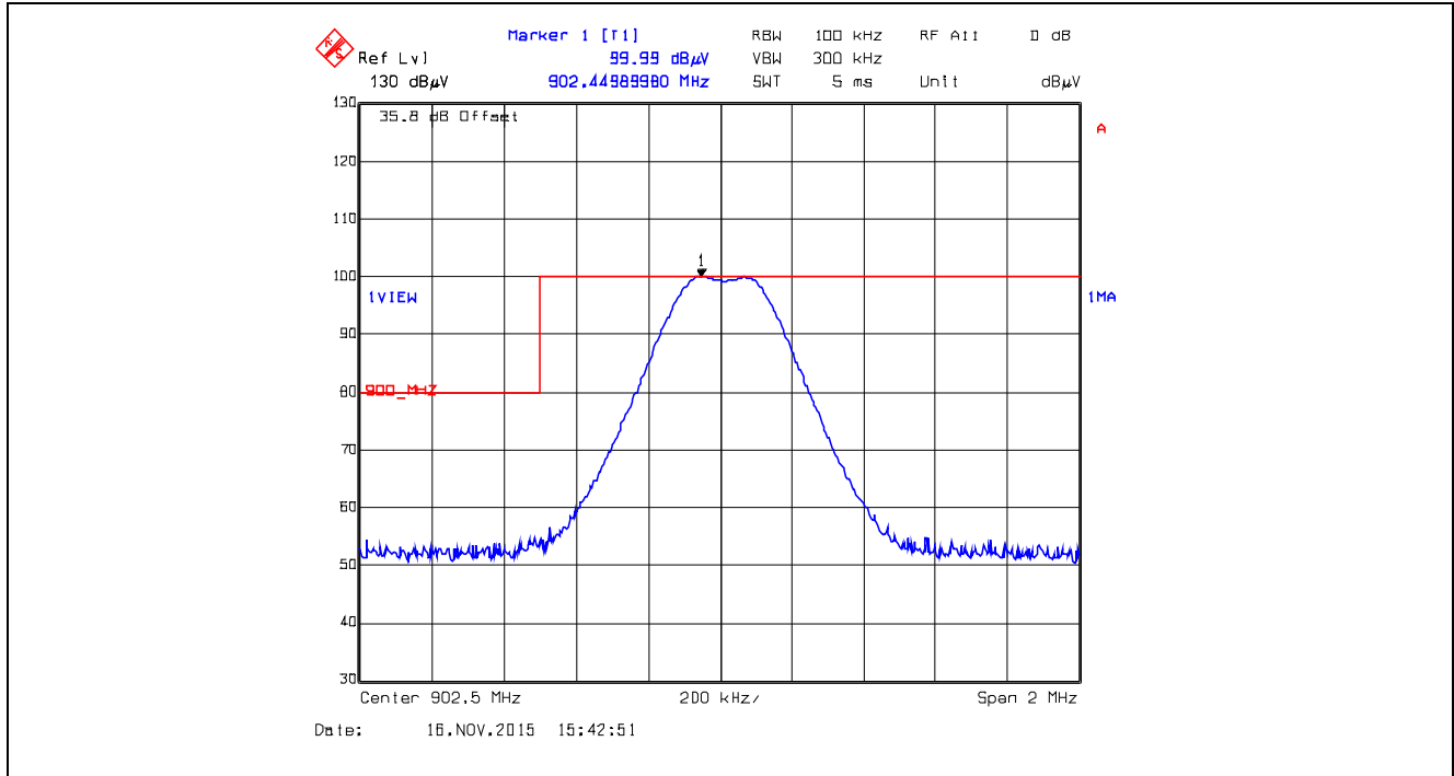
Plot 5.5.4.2.2.9. Band-Edge RF Radiated Emissions at 3 m, Horizontal Polarization Single Frequency Mode, Low End of Frequency Band, 902.5 MHz, XB1, Data Rate at 110 kbps
