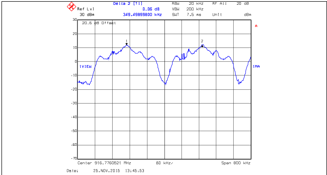
Plot 5.3.4.26. Carrier Frequency Separation, XTC1, Data Rate at 125 kbps
