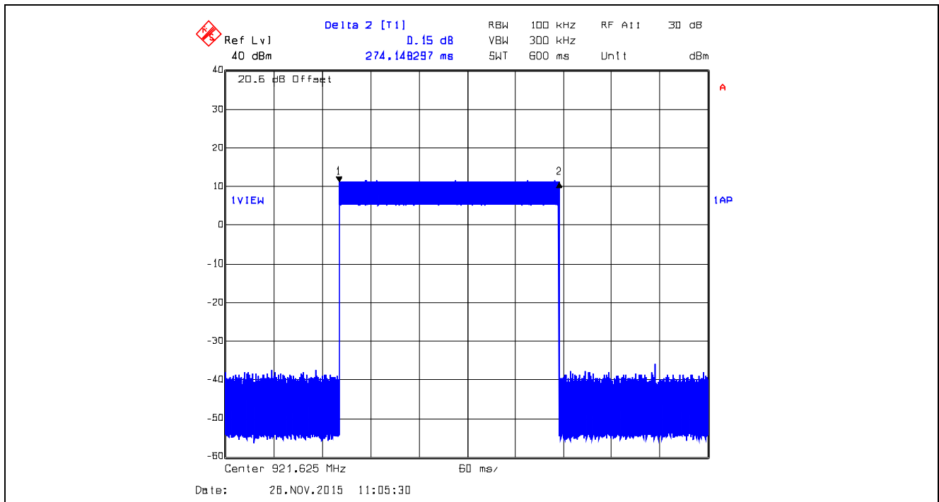
Plot 5.3.4.80. Time of Occupancy, 921.625 MHz, XTCA0, Data Rate at 10 kbps Dwell Time @ 921.625 MHz = 274.1483 ms
