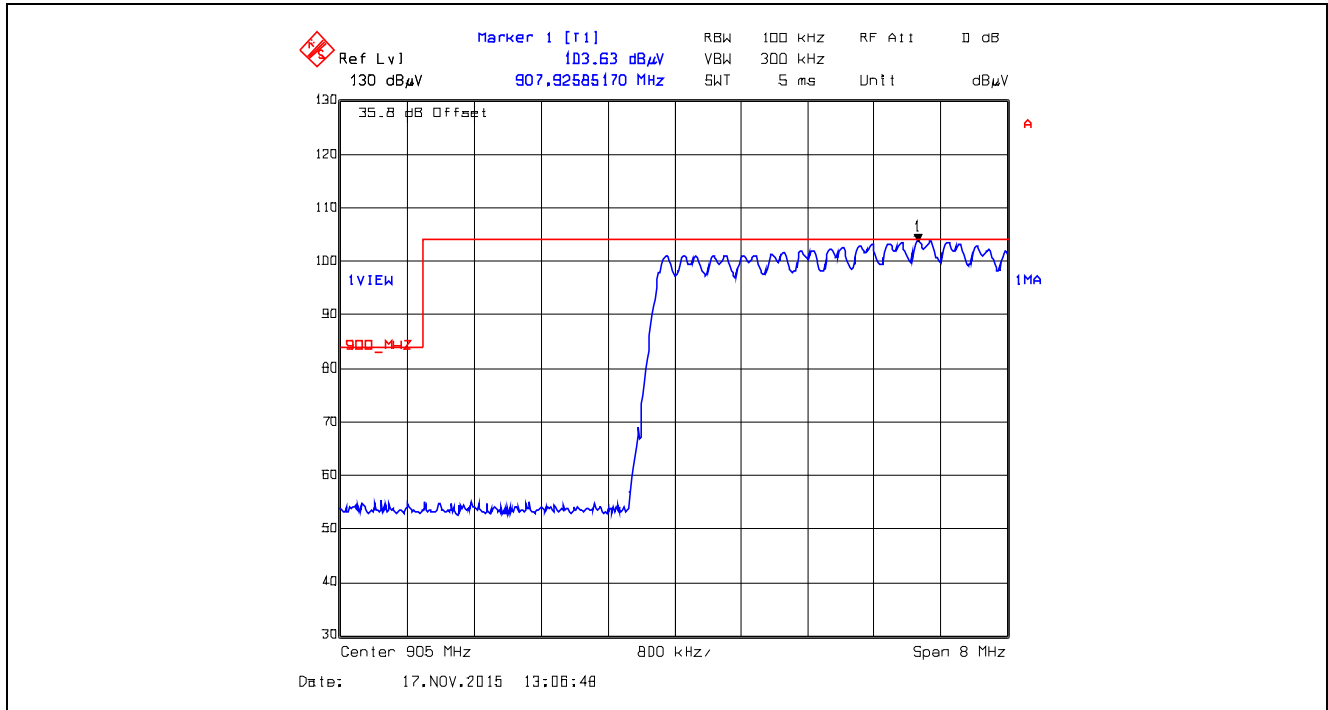
Plot 5.5.4.2.26. Band-Edge RF Radiated Emissions at 3 m, Horizontal Polarization Pseudorandom Hopping Mode, Low End of Frequency Band, 905.0 MHz, XTC0, Data Rate at 10 kbps
