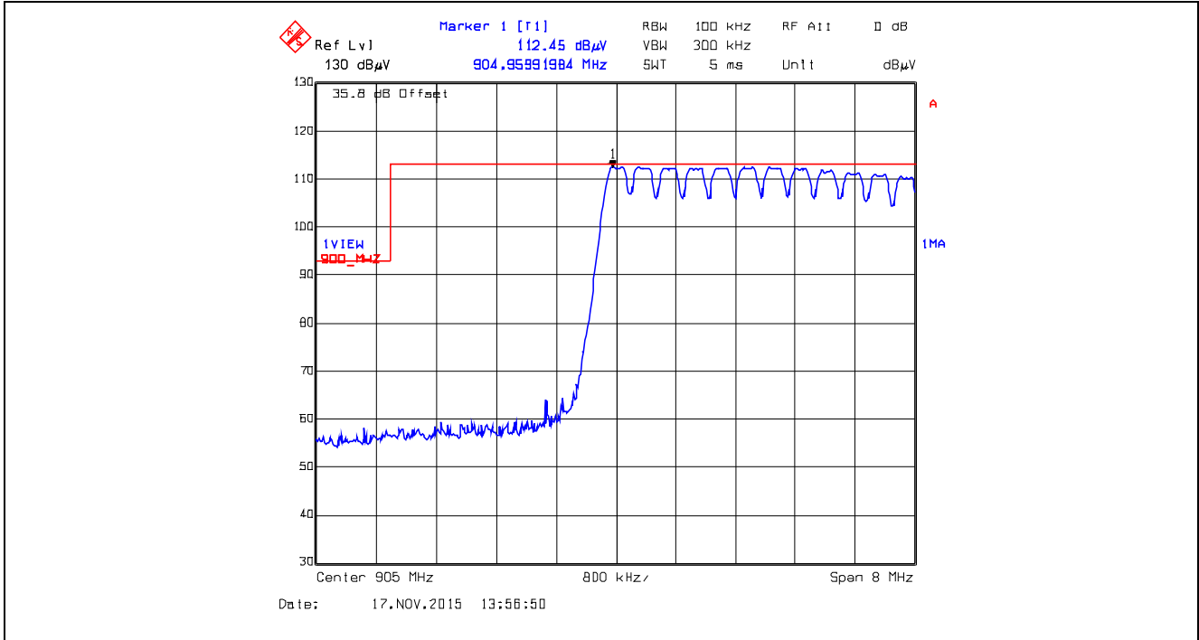
Plot 5.5.4.2.36. Band-Edge RF Radiated Emissions at 3 m, Vertical Polarization Pseudorandom Hopping Mode, Low End of Frequency Band, 905.0 MHz, XTC1, Data Rate at 125 kbps
