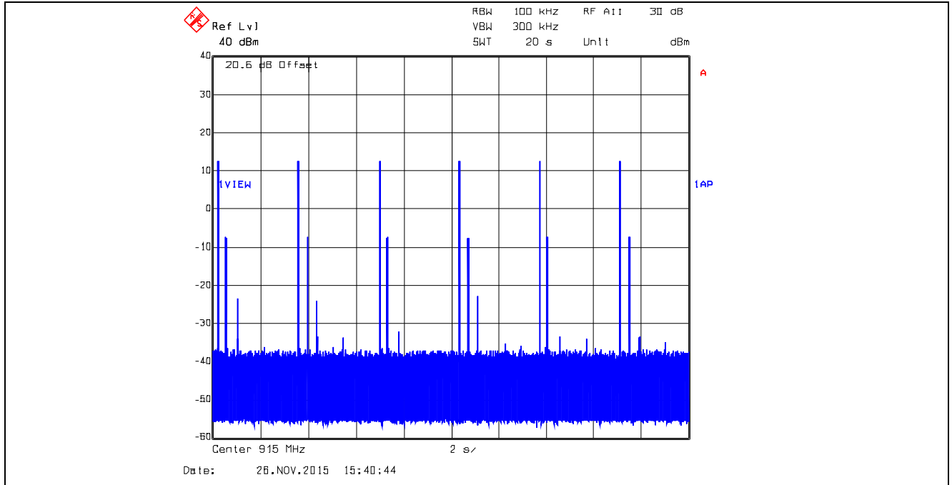
Plot 5.3.4.57. Time of Occupancy, 915.0 MHz, XB1, Data Rate at 110 kbps Average time of occupancy = (Dwell Time) x (number of hops) = 30.4609 ms x 6 = 182.77 ms < 0.4 sec within 20 sec
