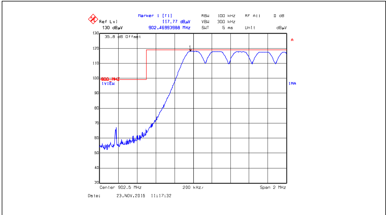
Plot 5.5.4.4.2.2. Band-Edge RF Radiated Emissions at 3 m, Horizontal Polarization Pseudorandom Hopping Mode, Low End of Frequency Band, 902.5 MHz, XB0, Data Rate at 10 kbps
