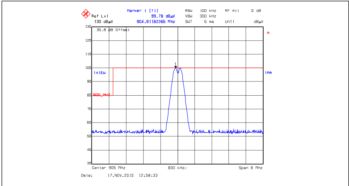
Plot 5.5.4.2.25. Band-Edge RF Radiated Emissions at 3 m, Horizontal Polarization Single Frequency Mode, Low End of Frequency Band, 905.0 MHz, XTC0, Data Rate at 10 kbps
