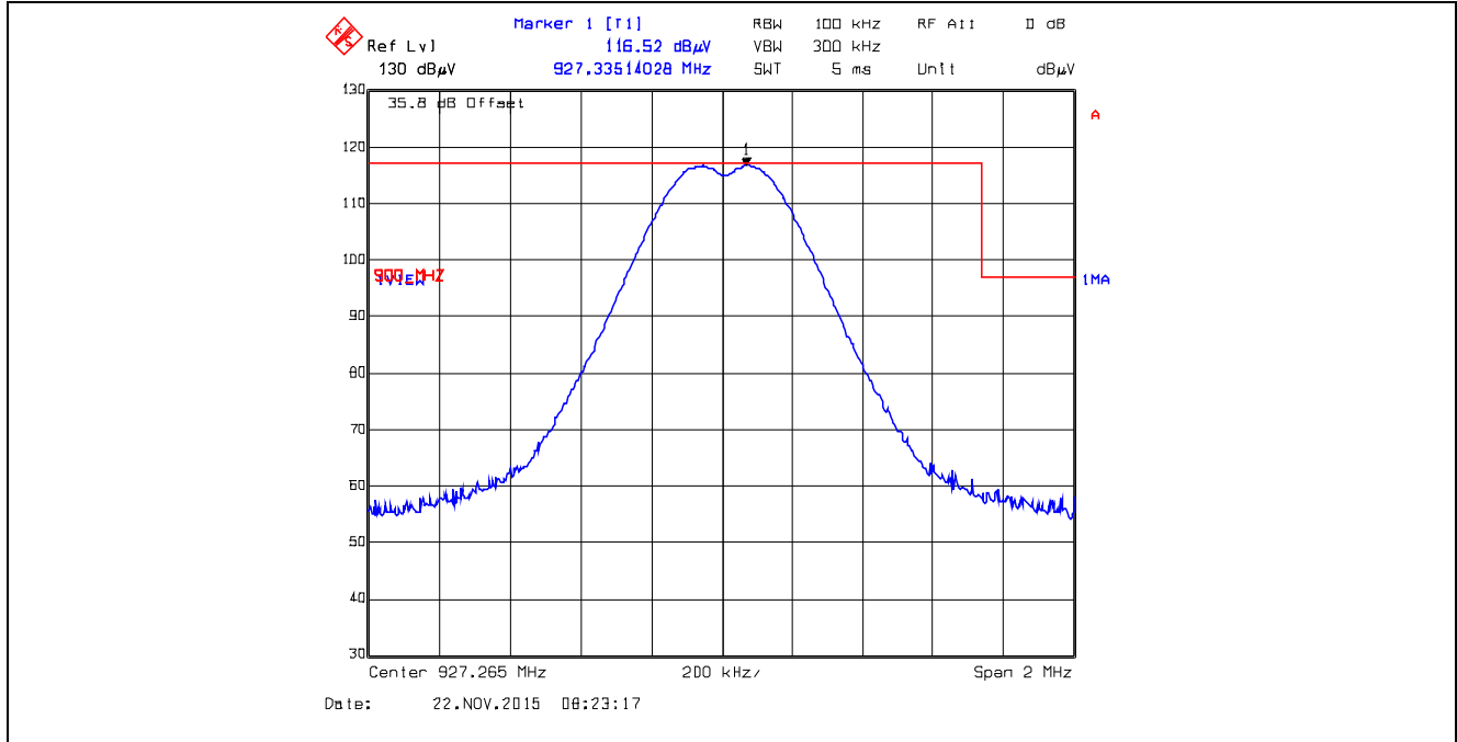
Plot 5.5.4.4.27. Band-Edge RF Radiated Emissions at 3 m, Vertical Polarization Single Frequency Mode, High End of Frequency Band, 927.265 MHz, XTCA0, Data Rate at 10 kbps
