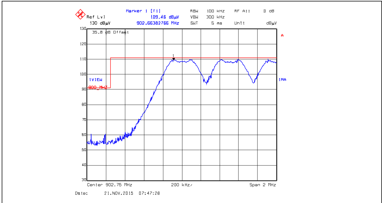
Plot 5.5.4.3.2.20. Band-Edge RF Radiated Emissions at 3 m, Vertical Polarization Pseudorandom Hopping Mode, Low End of Frequency Band, 902.75 MHz, XB2, Data Rate at 250 kbps
