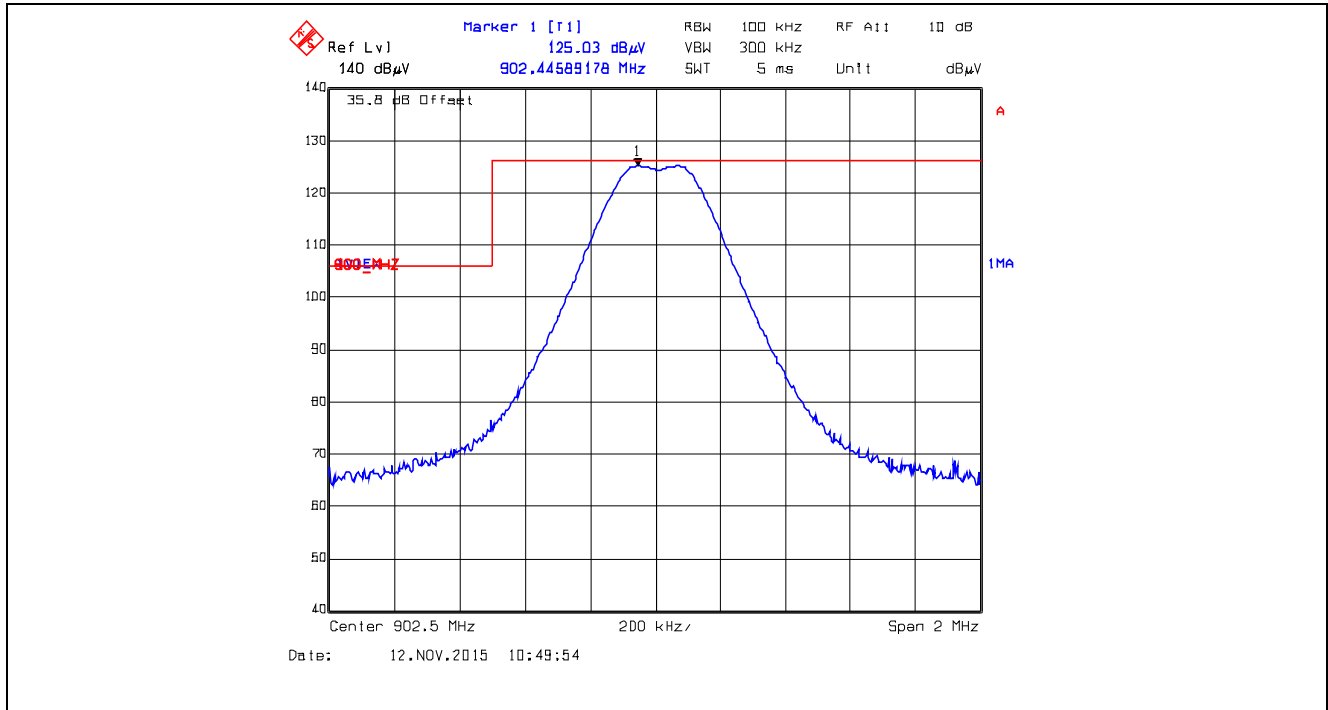
Plot 5.5.4.5.2.11. Band-Edge RF Radiated Emissions at 3 m, Vertical Polarization Single Frequency Mode, Low End of Frequency Band, 902.5 MHz, XB1, Data Rate at 110 kbps
