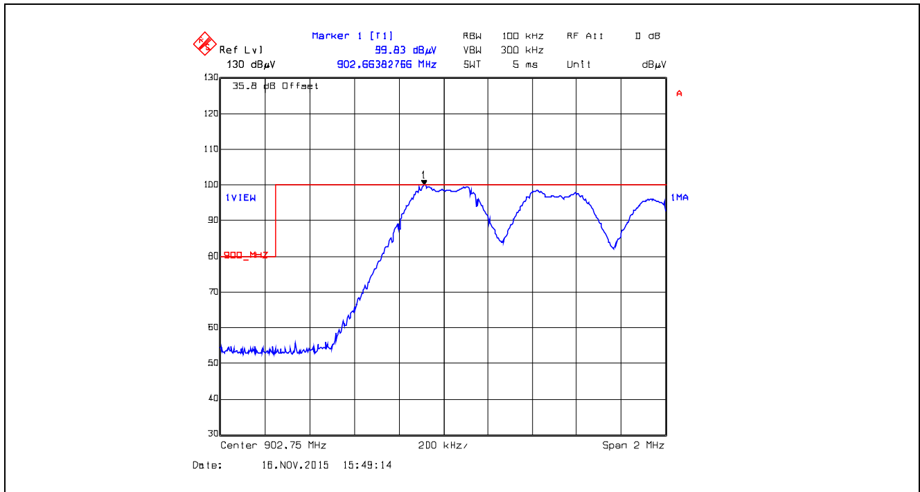
Plot 5.5.4.2.2.18. Band-Edge RF Radiated Emissions at 3 m, Horizontal Polarization Pseudorandom Hopping Mode, Low End of Frequency Band, 902.75 MHz, XB2, Data Rate at 250 kbps
