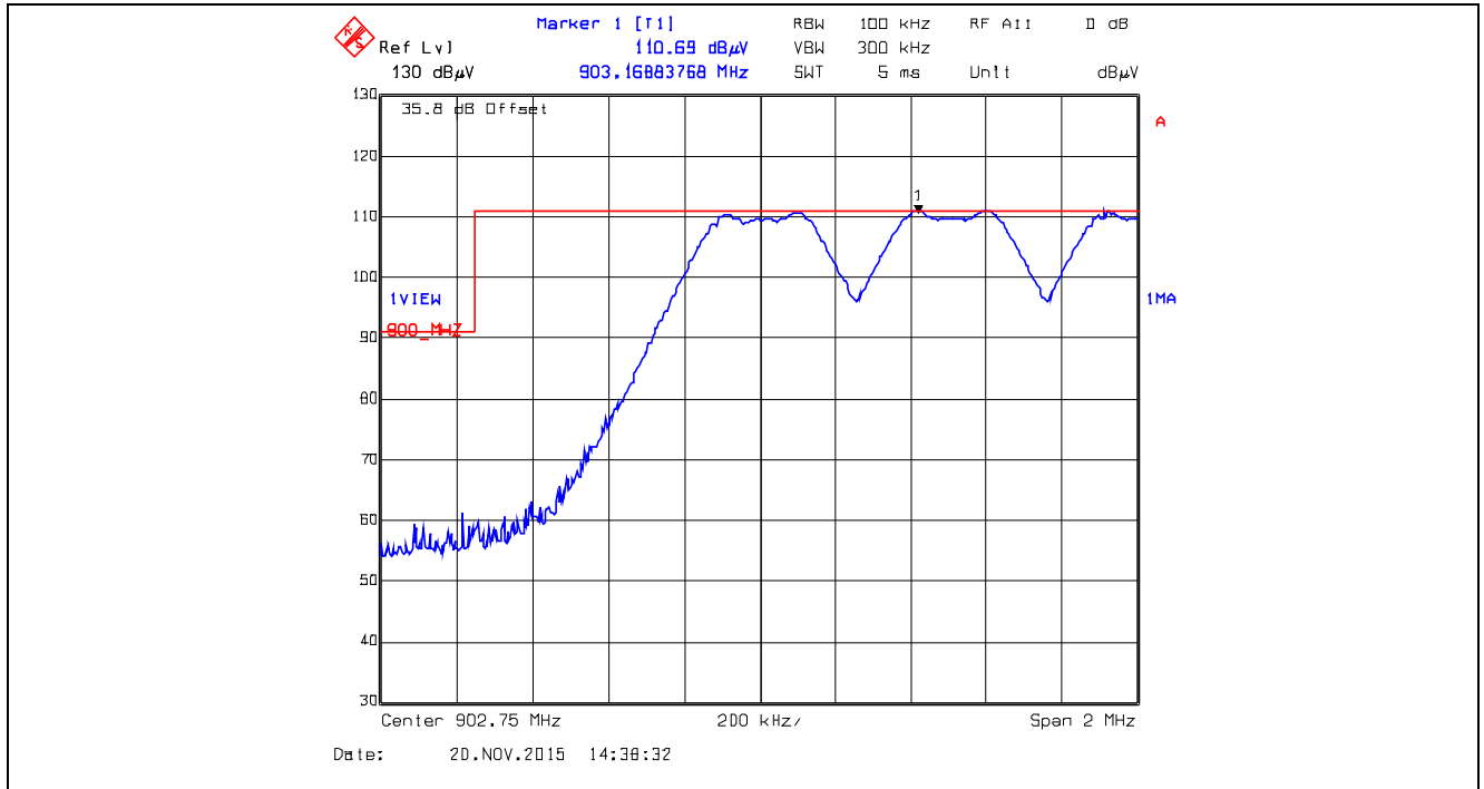
Plot 5.5.4.1.2.18. Band-Edge RF Radiated Emissions at 3 m, Horizontal Polarization Pseudorandom Hopping Mode, Low End of Frequency Band, 902.75 MHz, XB2, Data Rate at 250 kbps
