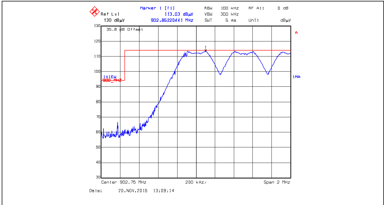
Plot 5.5.4.1.2.20. Band-Edge RF Radiated Emissions at 3 m, Vertical Polarization Pseudorandom Hopping Mode, Low End of Frequency Band, 902.75 MHz, XBX2, Data Rate at 250 kbps
