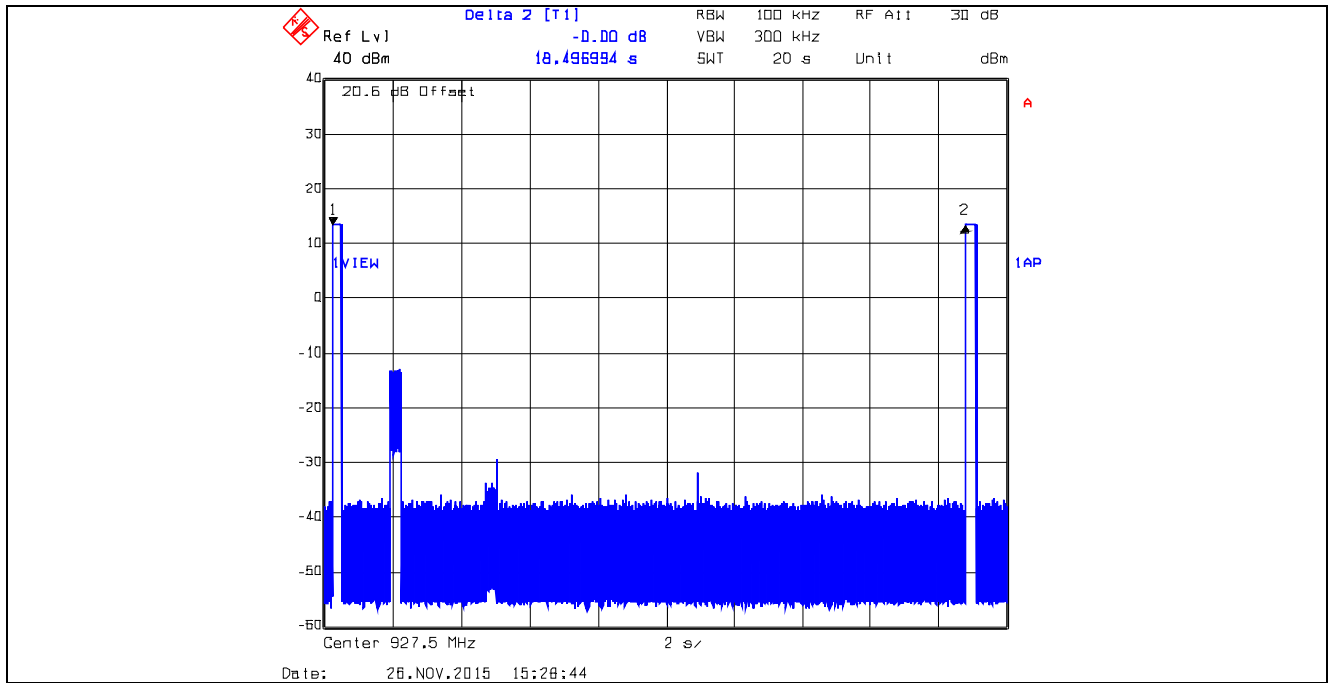
Plot 5.3.4.53. Time of Occupancy, 927.5 MHz XB0, Data Rate at 10 kbps Average time of occupancy = 20 \times (T_{on}) / (T_{total}) = 20 \times 0.3006012s / 18.4970s = 0.3250s < 0.4s
