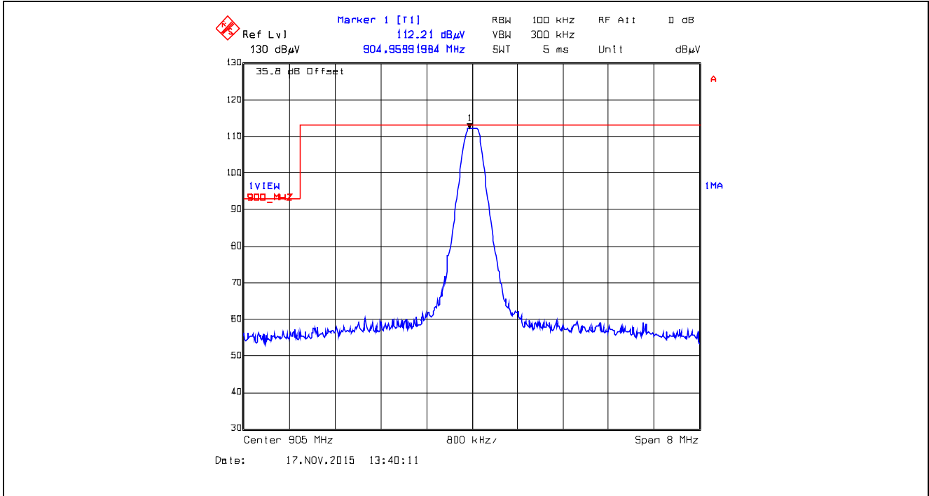
Plot 5.5.4.2.35. Band-Edge RF Radiated Emissions at 3 m, Vertical Polarization Single Frequency Mode, Low End of Frequency Band, 905.0 MHz, XTC1, Data Rate at 125 kbps
