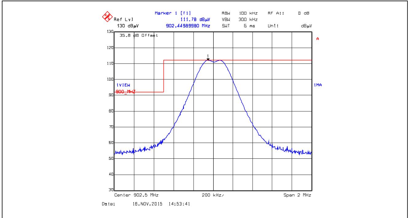
Plot 5.5.4.2.11. Band-Edge RF Radiated Emissions at 3 m, Vertical Polarization Single Frequency Mode, Low End of Frequency Band, 902.5 MHz, XB1, Data Rate at 110 kbps
