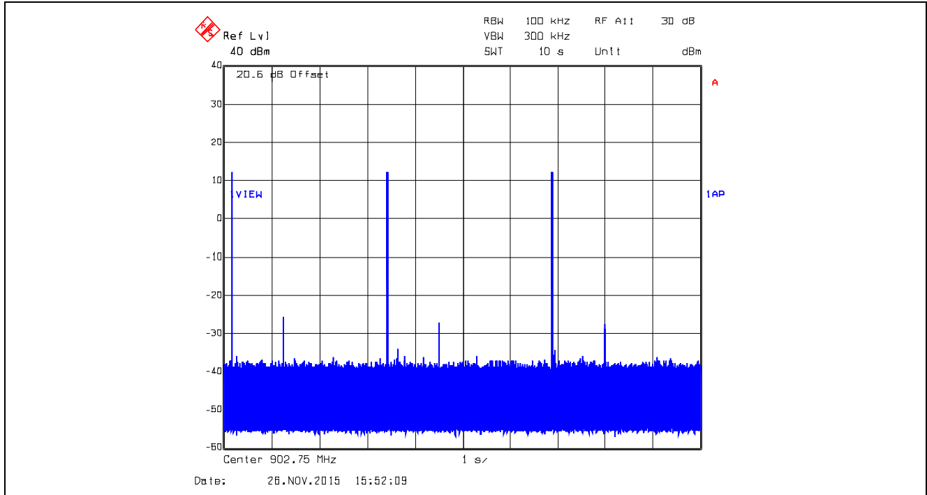
Plot 5.3.4.61. Time of Occupancy, 902.75 MHz, XB2, Data Rate at 250 kbps Average time of occupancy = (Dwell Time) x (number of hops) = 15.4309 ms x 3 = 46.2927 ms < 0.4 sec within 10 sec
