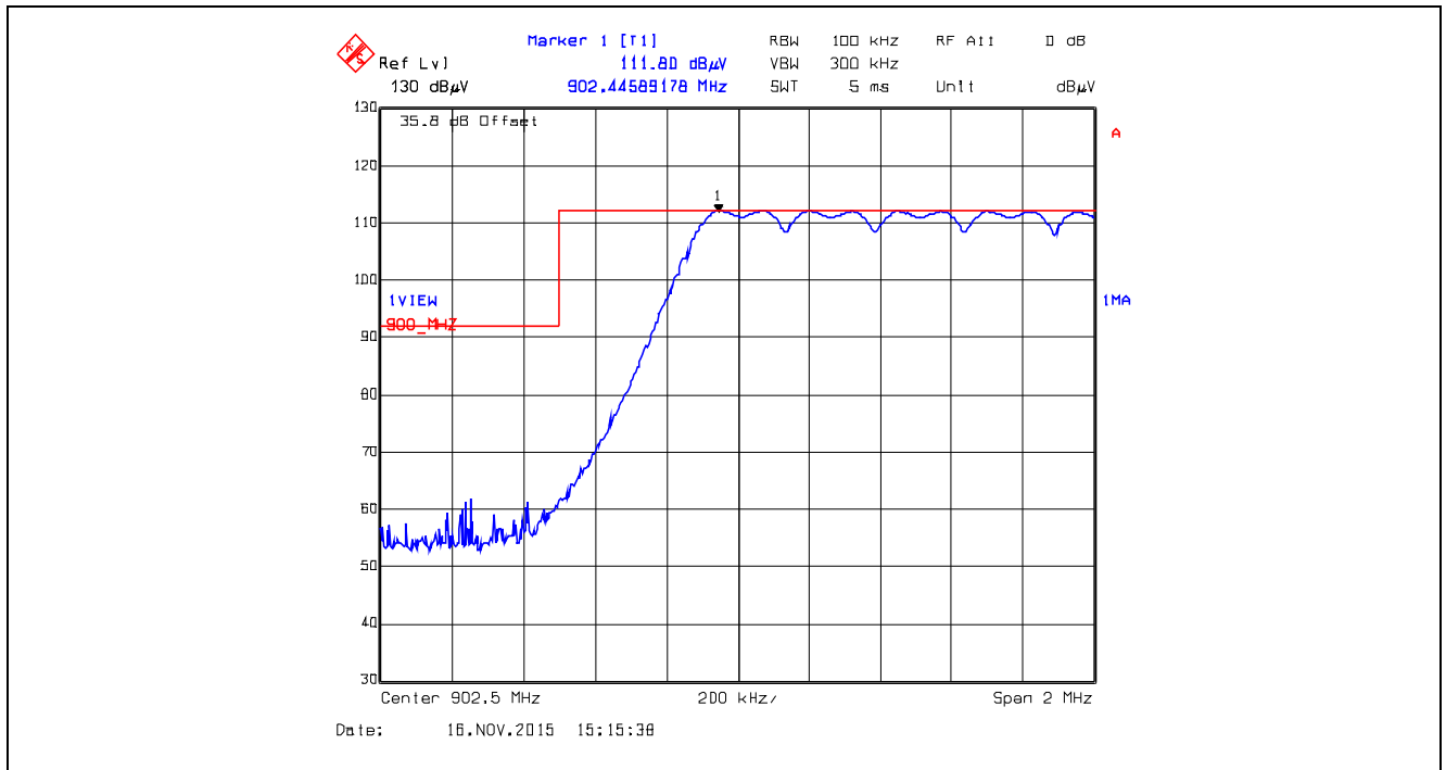
Plot 5.5.4.2.12. Band-Edge RF Radiated Emissions at 3 m, Vertical Polarization Pseudorandom Hopping Mode, Low End of Frequency Band, 902.5 MHz, XB1, Data Rate at 110 kbps
