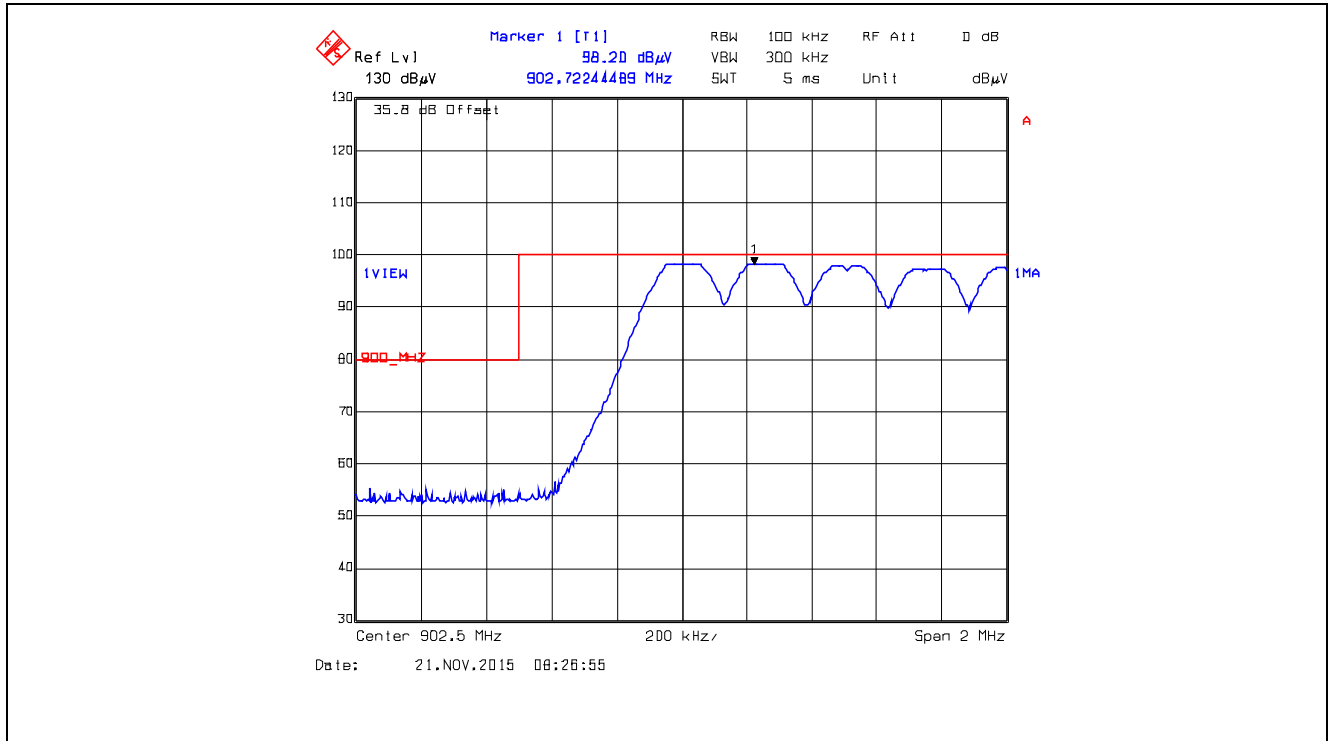
Plot 5.5.4.3.2.2. Band-Edge RF Radiated Emissions at 3 m, Horizontal Polarization Pseudorandom Hopping Mode, Low End of Frequency Band, 902.5 MHz, XB0, Data Rate at 10 kbps
