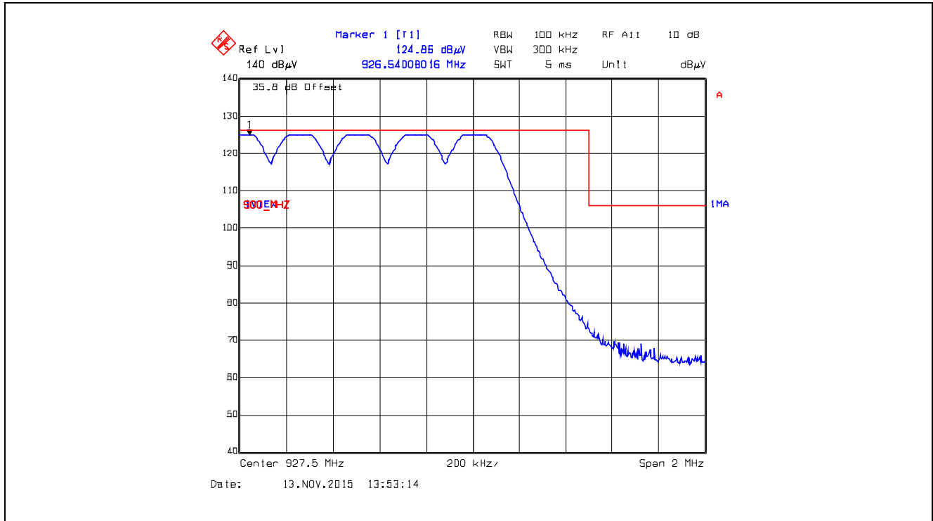
Plot 5.5.4.5.2.6. Band-Edge RF Radiated Emissions at 3 m, Horizontal Polarization Pseudorandom Hopping Mode, High End of Frequency Band, 927.5 MHz, XB0, Data Rate at 10 kbps
