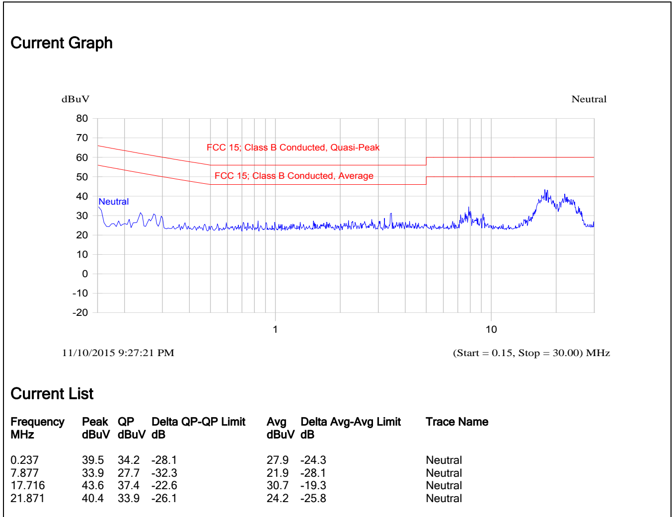
Plot 5.1.4.2. Power Line Conducted Emissions (Tx Mode) Line Voltage: 120 VAC; Line Tested: Neutral
