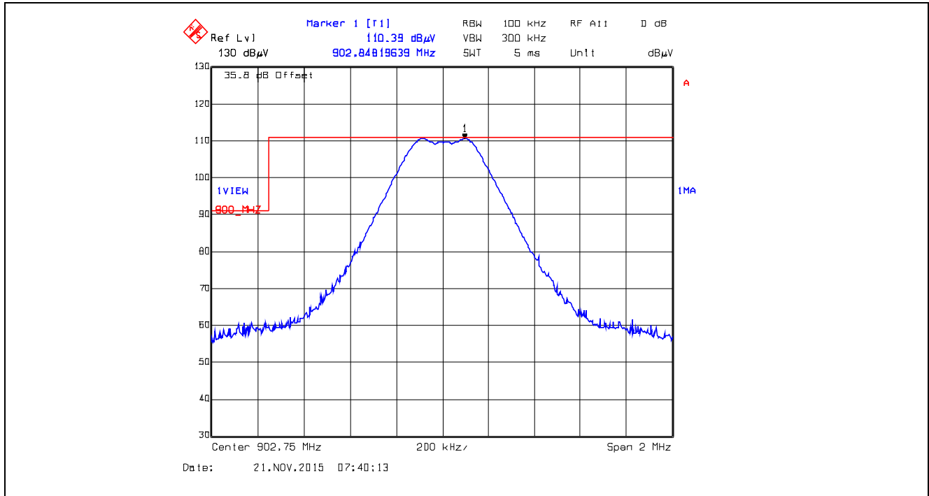
Plot 5.5.4.3.2.19. Band-Edge RF Radiated Emissions at 3 m, Vertical Polarization Single Frequency Mode, Low End of Frequency Band, 902.75 MHz, XB2, Data Rate at 250 kbps
