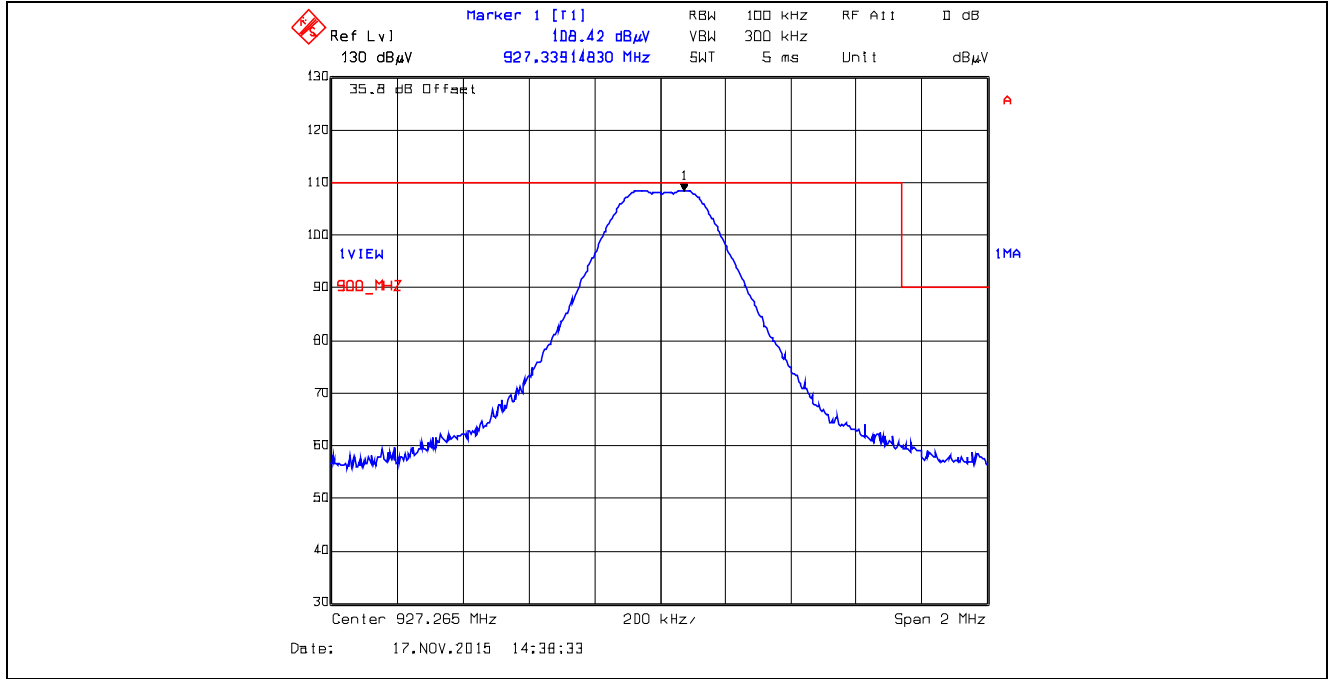
Plot 5.5.4.2.255. Band-Edge RF Radiated Emissions at 3 m, Vertical Polarization Single Frequency Mode, High End of Frequency Band, 927.265 MHz, XTCA1, Data Rate at 105kbps
