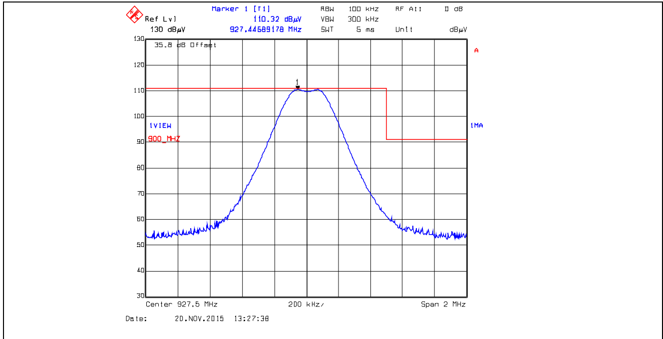
Plot 5.5.4.1.2.15. Band-Edge RF Radiated Emissions at 3 m, Vertical Polarization Single Frequency Mode, High End of Frequency Band, 927.5 MHz, XB1, Data Rate at 110 kbps
