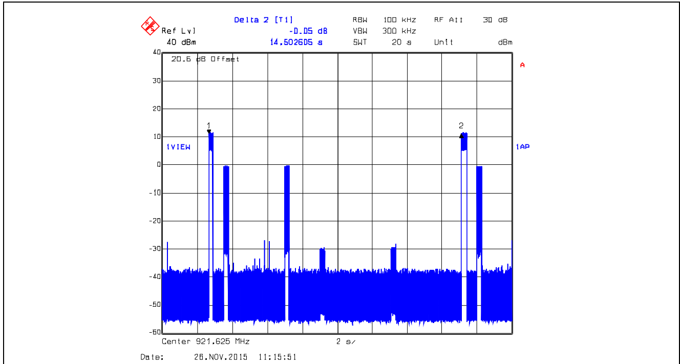
Plot 5.3.4.81. Time of Occupancy, 921.625 MHz XTCA0, Data Rate at 10 kbps Average time of occupancy = 20 \times (T_{on}) / (T_{total}) = 20 \times 0.2741483s / 14.5025s = 0.3781s < 0.4s
