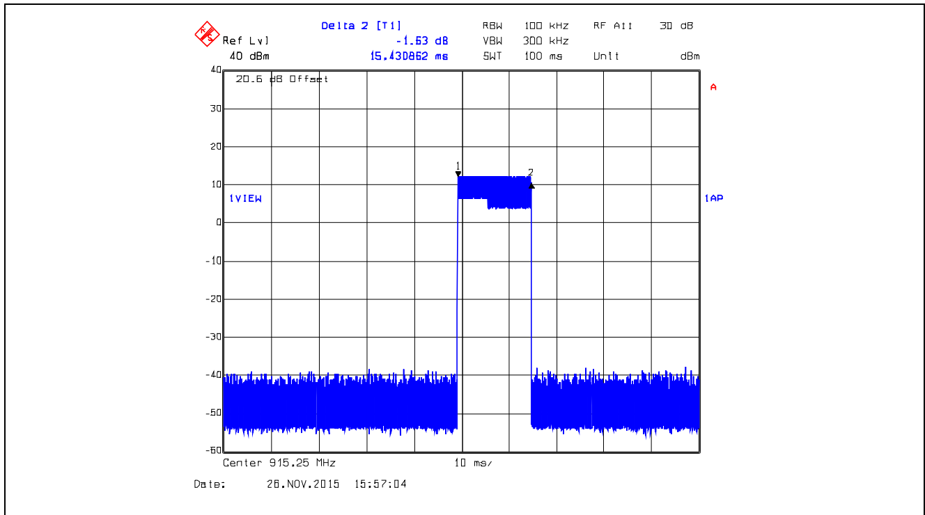
Plot 5.3.4.62. Time of Occupancy, 915.25 MHz, XB2, Data Rate at 250 kbps Dwell Time @ 915.25 MHz = 15.4309 ms
