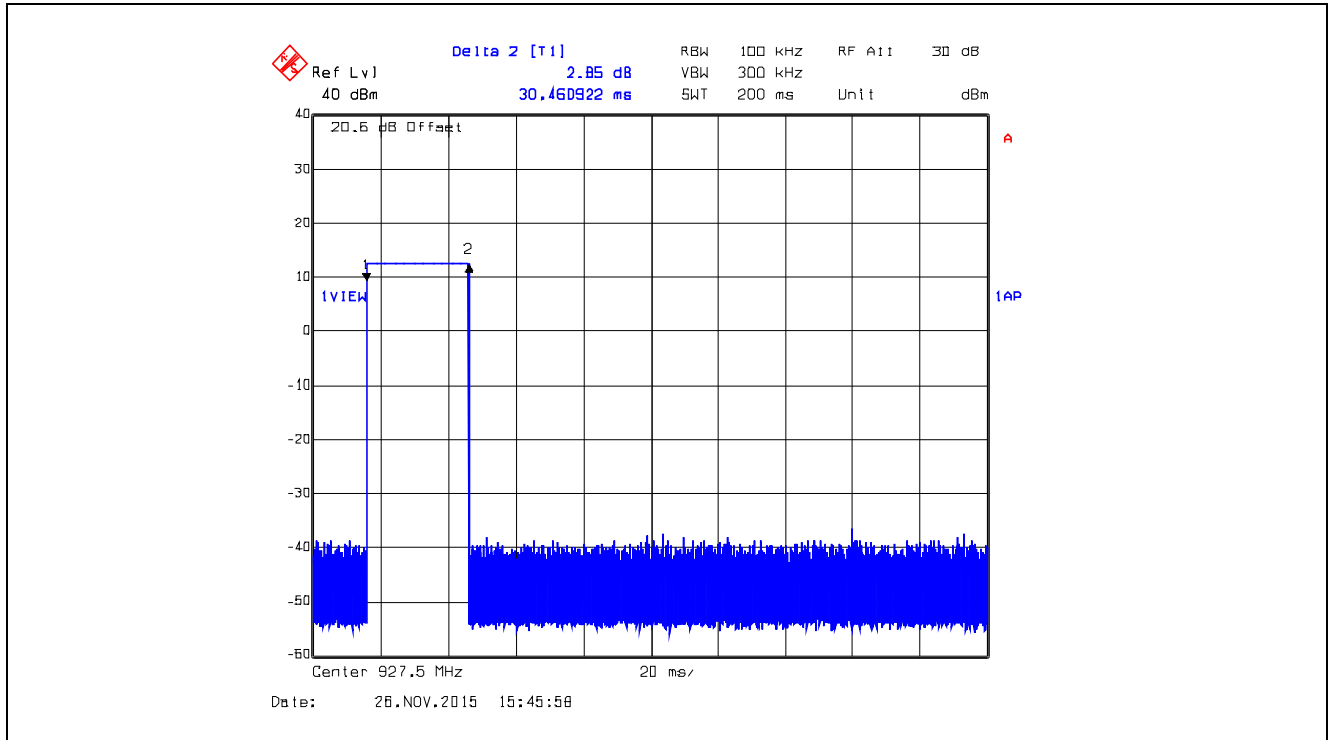
Plot 5.3.4.58. Time of Occupancy, 927.5 MHz, XB1, Data Rate at 110 kbps Dwell Time @ 927.5 MHz = 30.4609 ms
