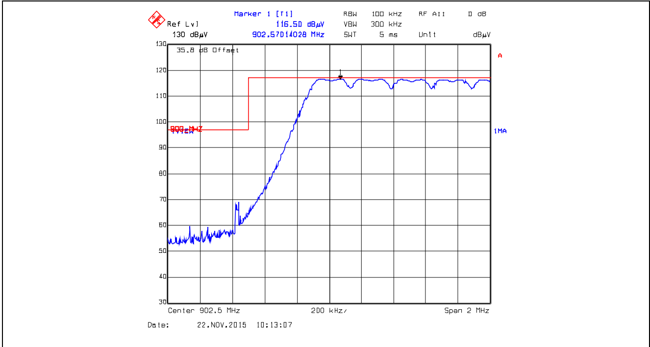
Plot 5.5.4.4.2.12. Band-Edge RF Radiated Emissions at 3 m, Vertical Polarization Pseudorandom Hopping Mode, Low End of Frequency Band, 902.5 MHz, XB1, Data Rate at 110 kbps
