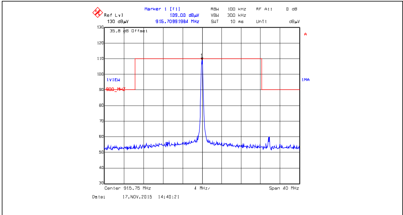
Plot 5.5.4.2.51. Band-Edge RF Radiated Emissions at 3 m, Vertical Polarization Single Frequency Mode, Low End of Frequency Band, 915.75 MHz, XTCA1, Data Rate at 105kbps
