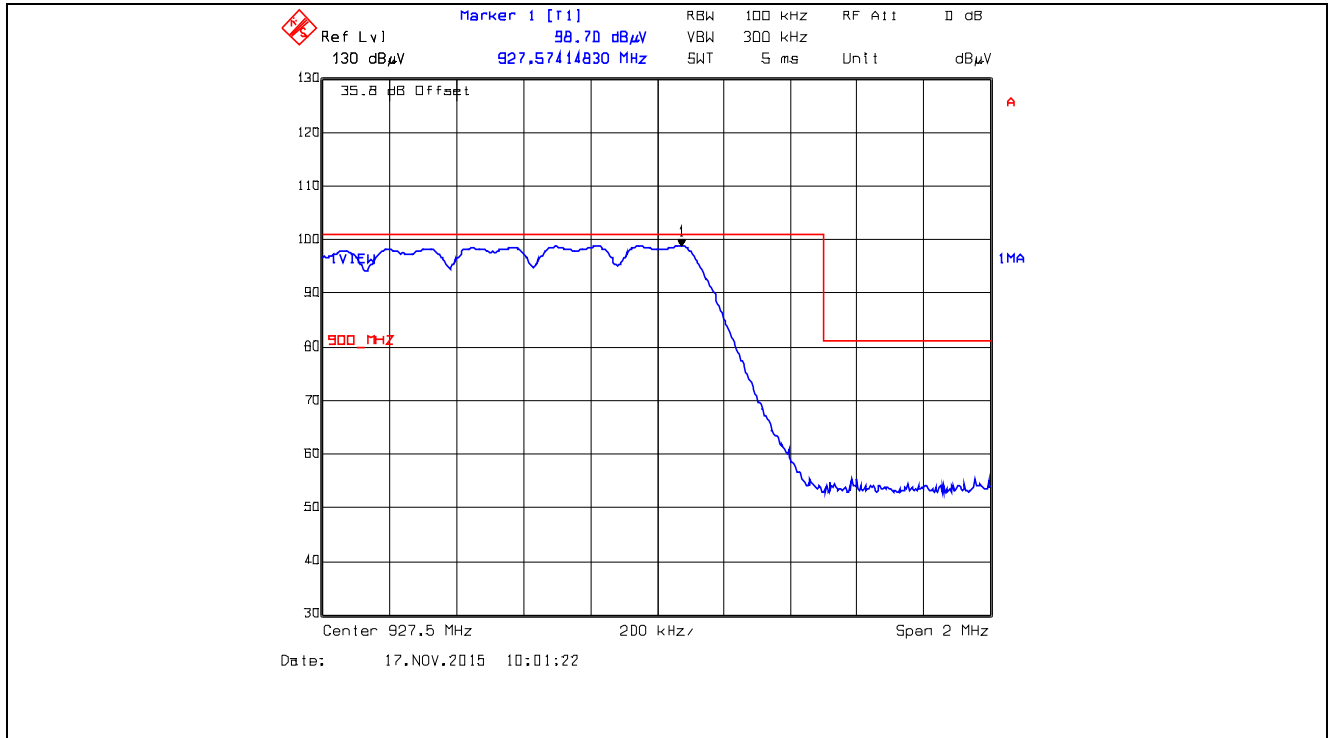
Plot 5.5.4.2.2.14. Band-Edge RF Radiated Emissions at 3 m, Horizontal Polarization Pseudorandom Hopping Mode, High End of Frequency Band, 927.5 MHz, XB1, Data Rate at 110 kbps
