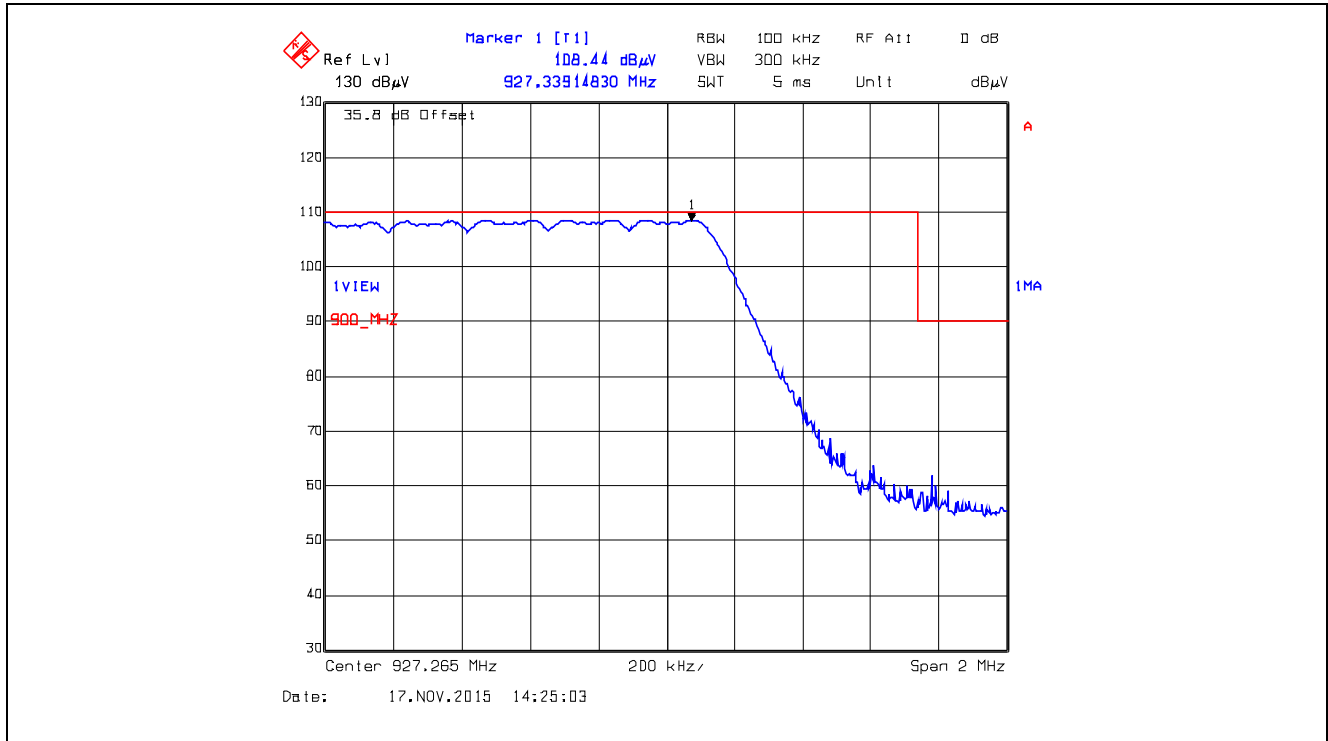
Plot 5.5.4.2.256. Band-Edge RF Radiated Emissions at 3 m, Vertical Polarization Pseudorandom Hopping Mode, High End of Frequency Band, 927.265 MHz, XTCA1, Data Rate at 105kbps
