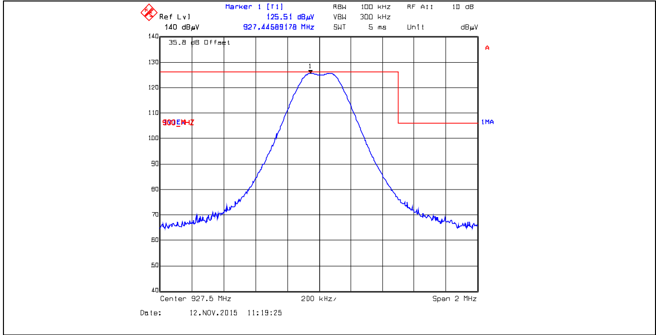
Plot 5.5.4.5.2.15. Band-Edge RF Radiated Emissions at 3 m, Vertical Polarization Single Frequency Mode, High End of Frequency Band, 927.5 MHz, XB1, Data Rate at 110 kbps
