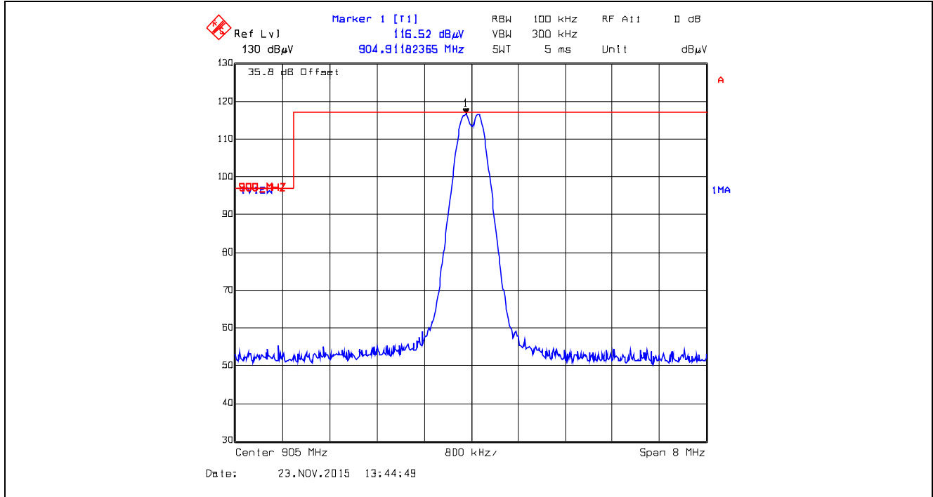
Plot 5.5.4.4.25. Band-Edge RF Radiated Emissions at 3 m, Horizontal Polarization Single Frequency Mode, Low End of Frequency Band, 905.0 MHz, XTC0, Data Rate at 10 kbps
