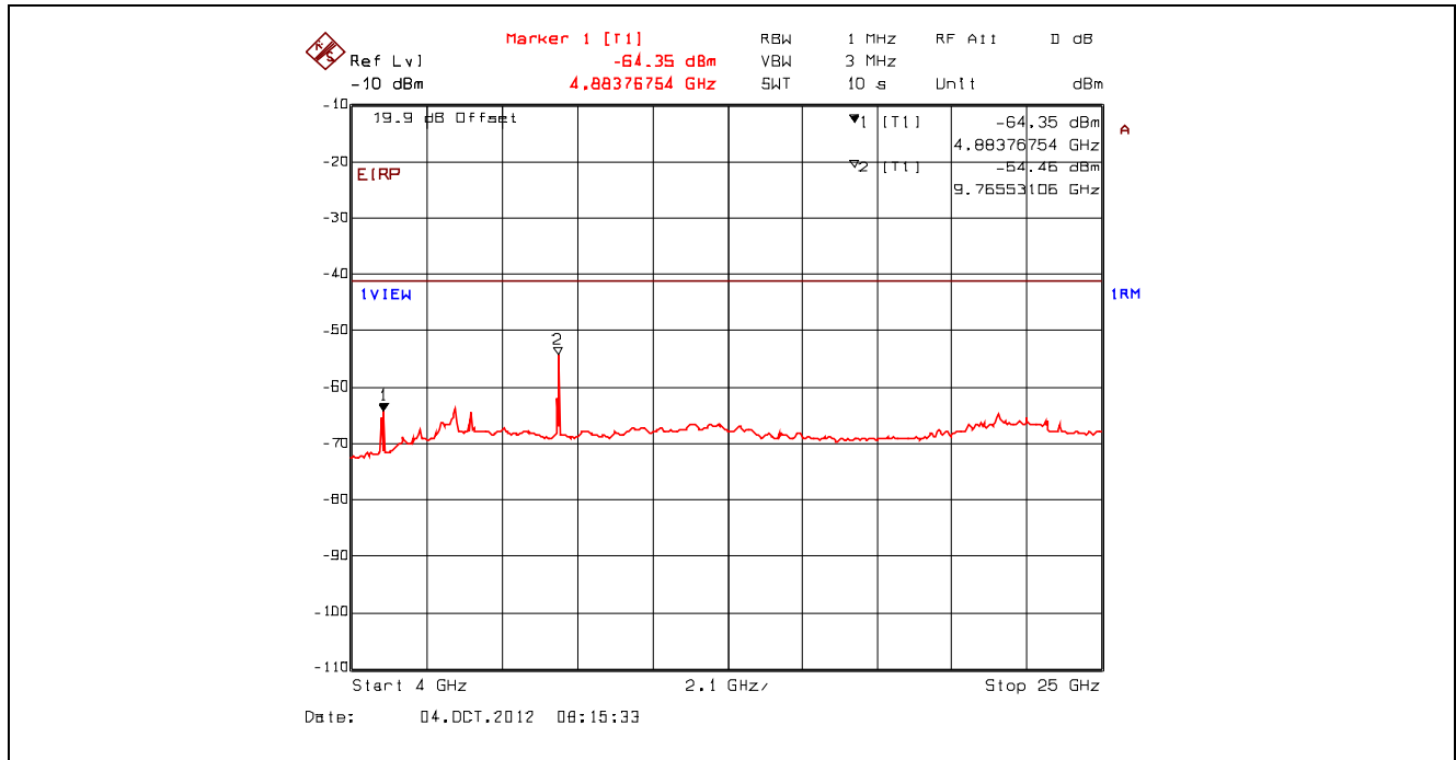
Plot 5.4.4.3.71. Conducted Spurious Emissions – Restricted Bands, 802.11n 800ns, 6.5 Mbps BPSK 1/2 2442 MHz, 4 GHz - 25 GHz, Power Averaging with High Pass Filter
