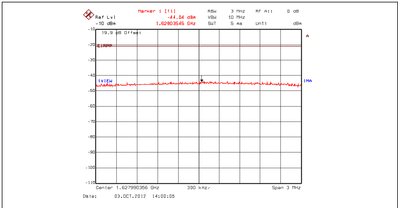
Plot 5.4.4.3.15. Conducted Spurious Emissions – Restricted Bands, 802.11b, 11 Mbps CCK 2442 MHz, Peak Power at 1.63 GHz with Band (Notch) Reject Filter
