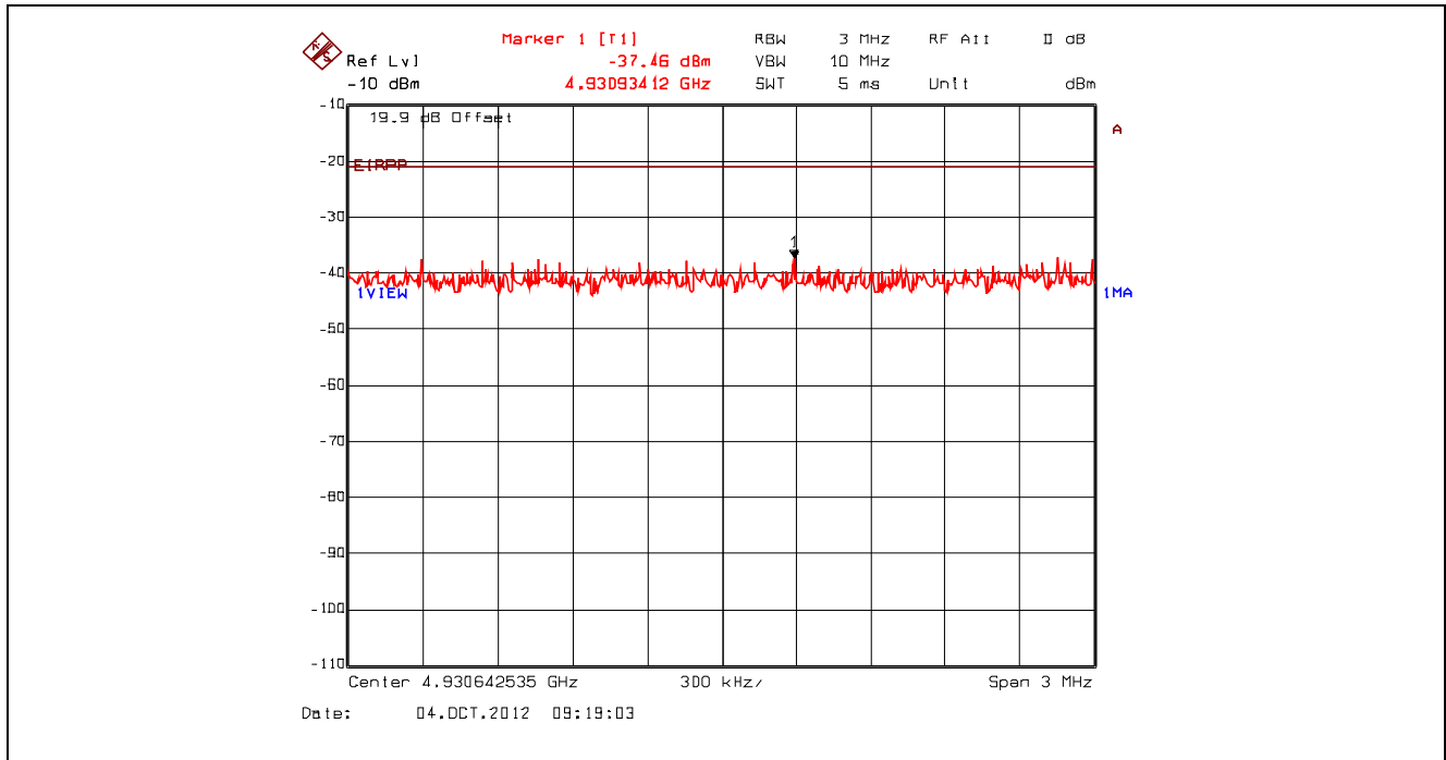
Plot 5.4.4.3.114. Conducted Spurious Emissions – Restricted Bands, 802.11n 400ns, 7.2 Mbps BPSK 1/2 2462 MHz, Peak Power at 4.93 GHz with High Pass Filter
