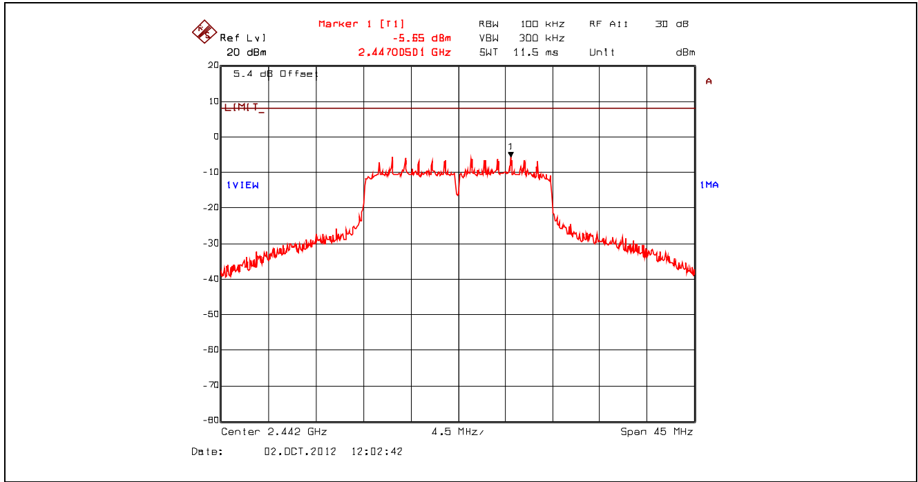
Plot 5.6.4.26. Power Spectral Density, 802.11n 800ns, 19.5 Mbps QPSK 3/4, 2442 MHz, Setting 23 Offset: Insertion Loss + BWCF = 20.63 dB + 10*log(3 kHz/ 100 kHz) = 5.43 dB
