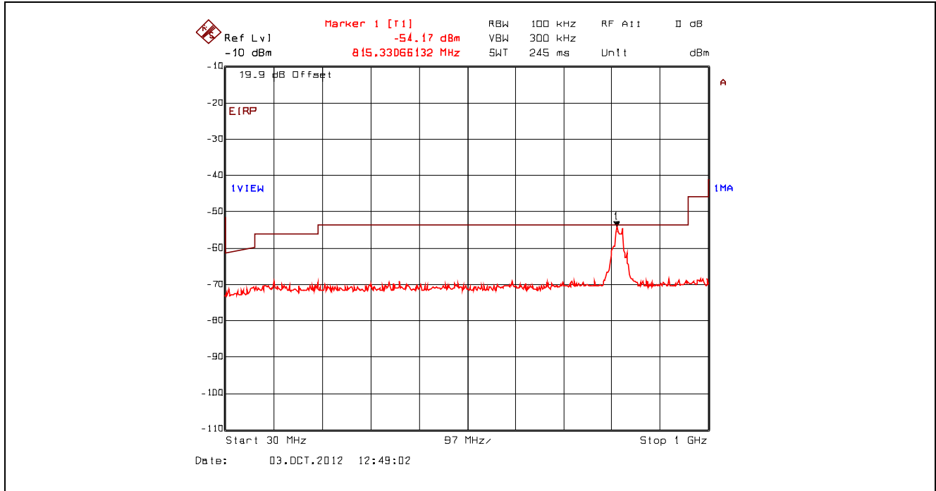
Plot 5.4.4.3.48. Conducted Spurious Emissions – Restricted Bands, 802.11g, 9 Mbps BPSK 2462 MHz, 30 MHz - 1 GHz, Peak Detector with Band (Notch) Reject Filter
