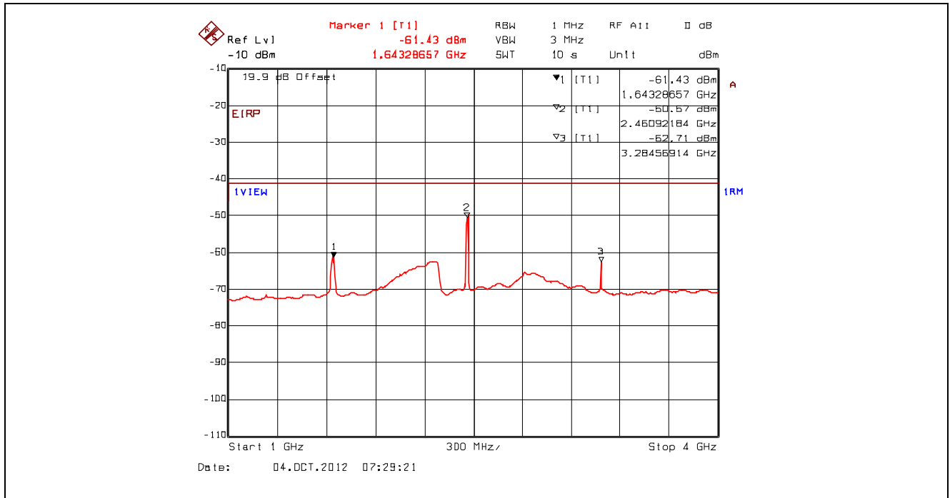
Plot 5.4.4.3.50. Conducted Spurious Emissions – Restricted Bands, 802.11g, 9 Mbps BPSK 2462 MHz, 1 GHz - 4 GHz, Power Averaging with Band (Notch) Reject Filter
