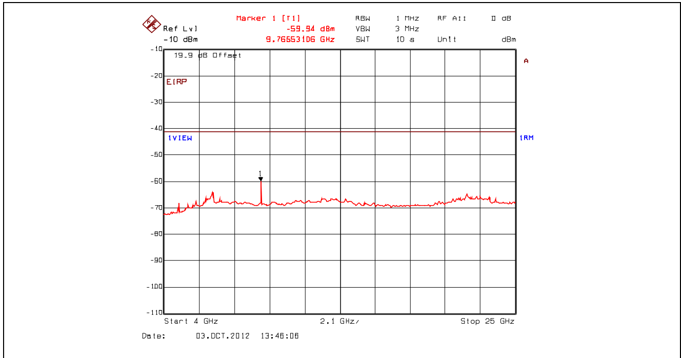
Plot 5.4.4.3.14. Conducted Spurious Emissions – Restricted Bands, 802.11b, 11 Mbps CCK 2442 MHz, 4 GHz - 25 GHz, Power Averaging with High Pass Filter
