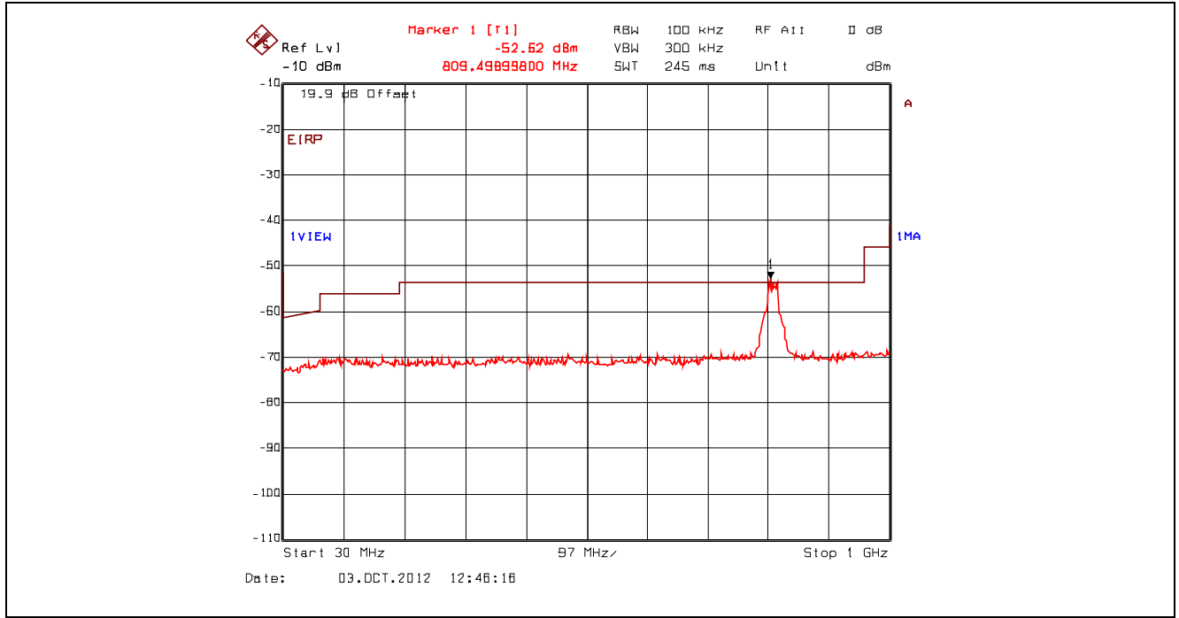
Plot 5.4.4.3.38. Conducted Spurious Emissions – Restricted Bands, 802.11g, 9 Mbps BPSK 2442 MHz, 30 MHz - 1 GHz, Peak Detector with Band (Notch) Reject Filter
