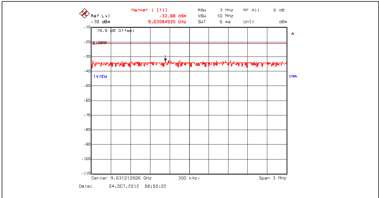
Plot 5.4.4.3.65. Conducted Spurious Emissions – Restricted Bands, 802.11n 800ns, 6.5 Mbps BPSK 1/2 2412 MHz, Peak Power at 9.63 GHz with High Pass Filter
