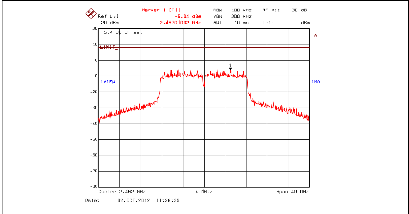
Plot 5.6.4.18. Power Spectral Density, 802.11g, 36 Mbps 16-QAM, 2462 MHz, Setting 23 Offset: Insertion Loss + BWCF = 20.63 dB + 10*log(3 kHz/ 100 kHz) = 5.43 dB
