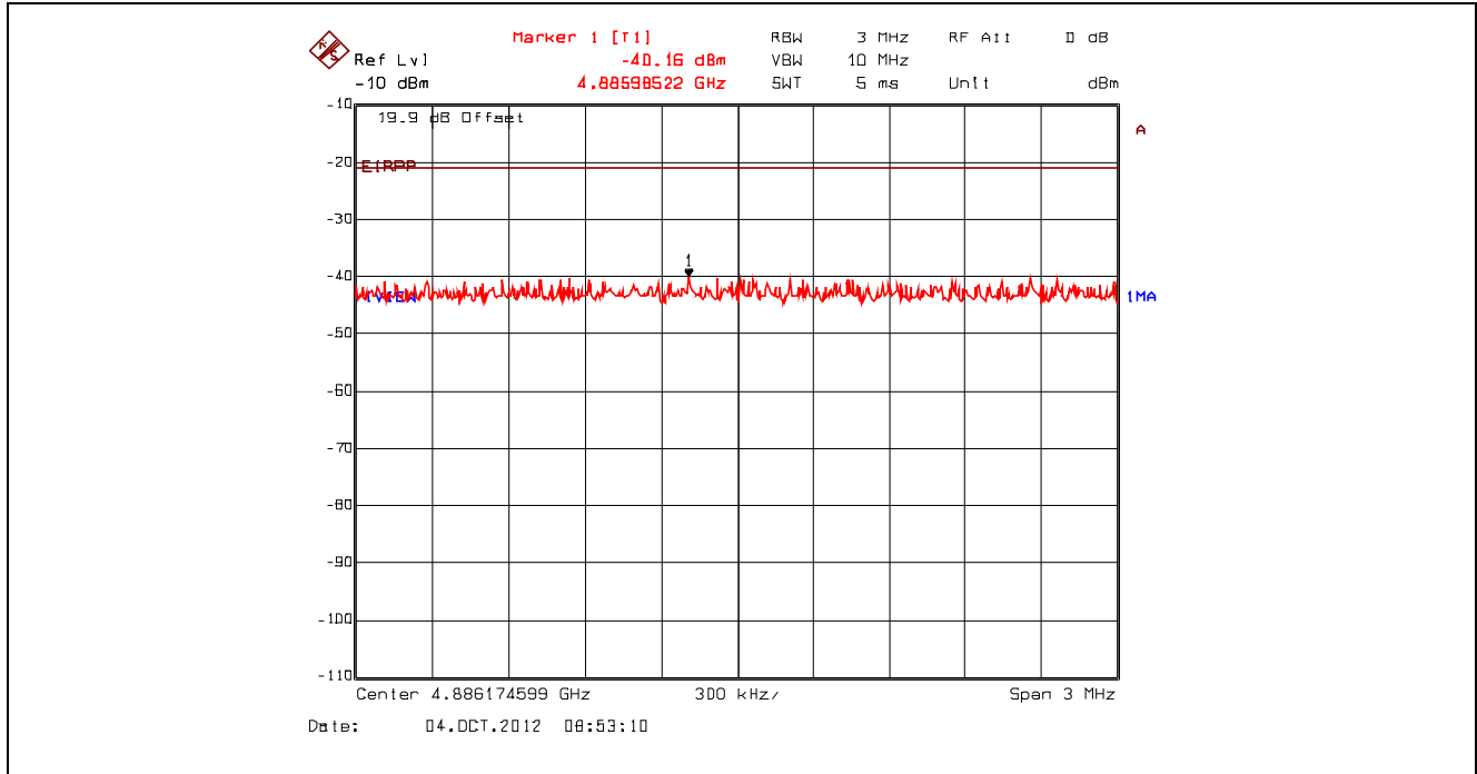
Plot 5.4.4.3.74. Conducted Spurious Emissions – Restricted Bands, 802.11n 800ns, 6.5 Mbps BPSK 1/2 2442 MHz, Peak Power at 4.89 GHz with High Pass Filter
