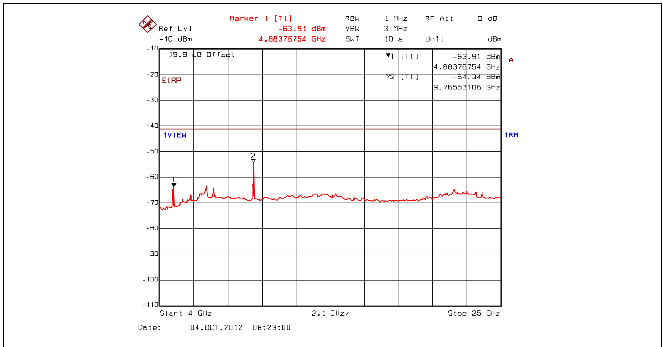
Plot 5.4.4.3.41. Conducted Spurious Emissions – Restricted Bands, 802.11g, 9 Mbps BPSK 2442 MHz, 4 GHz - 25 GHz, Power Averaging with High Pass Filter
