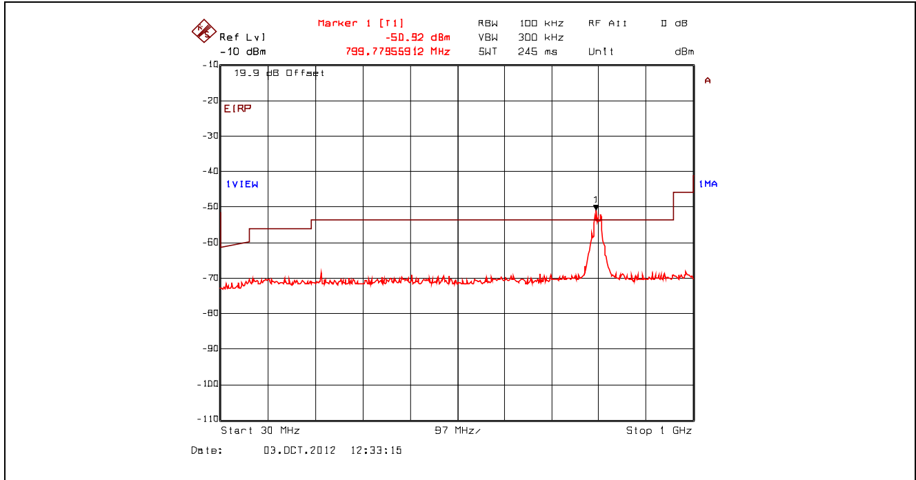
Plot 5.4.4.3.28. Conducted Spurious Emissions – Restricted Bands, 802.11g, 9 Mbps BPSK 2412 MHz, 30 MHz - 1 GHz, Peak Detector with Band (Notch) Reject Filter
