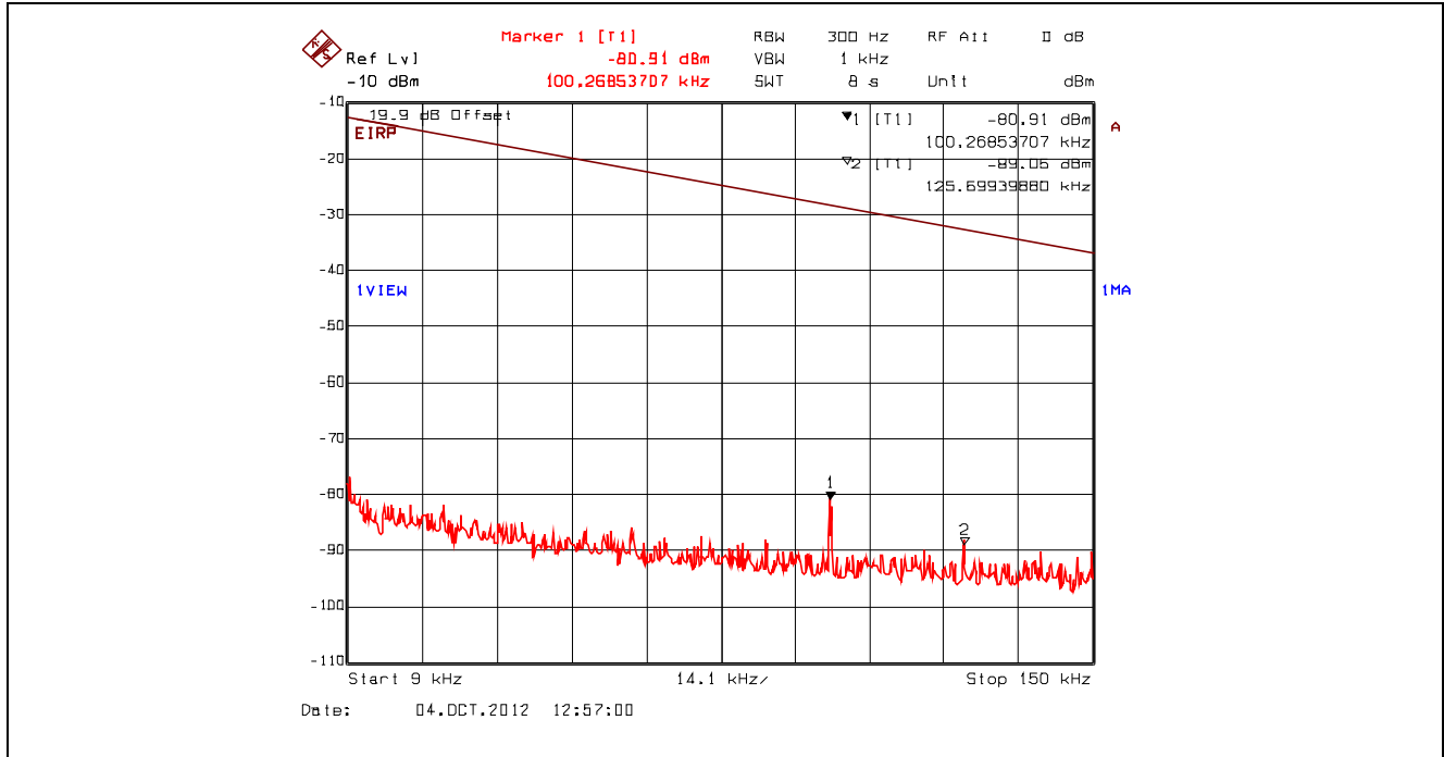
Plot 5.4.4.3.86. Conducted Spurious Emissions – Restricted Bands, 802.11n 400ns, 7.2 Mbps BPSK 1/2 2412 MHz, 9 kHz - 150 kHz, Peak Detector with Band (Notch) Reject Filter
