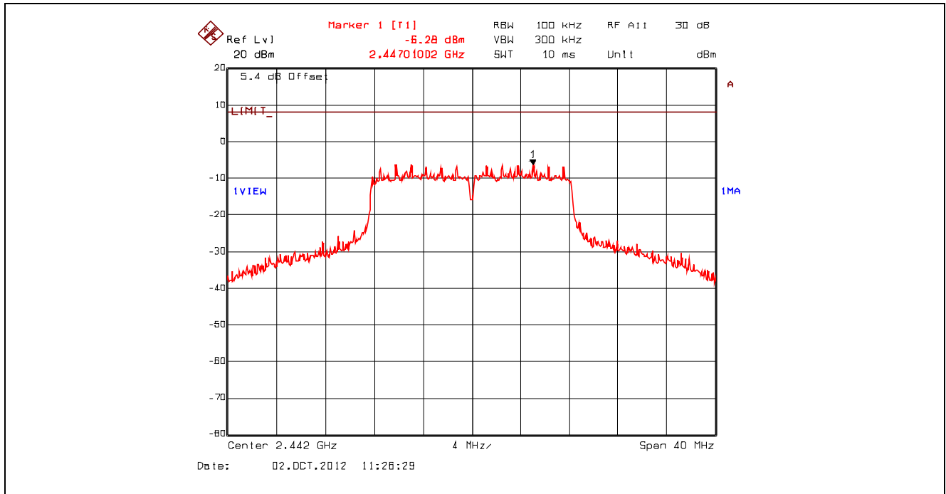
Plot 5.6.4.17. Power Spectral Density, 802.11g, 36 Mbps 16-QAM, 2442 MHz, Setting 23 Offset: Insertion Loss + BWCF = 20.63 dB + 10*log(3 kHz/ 100 kHz) = 5.43 dB
