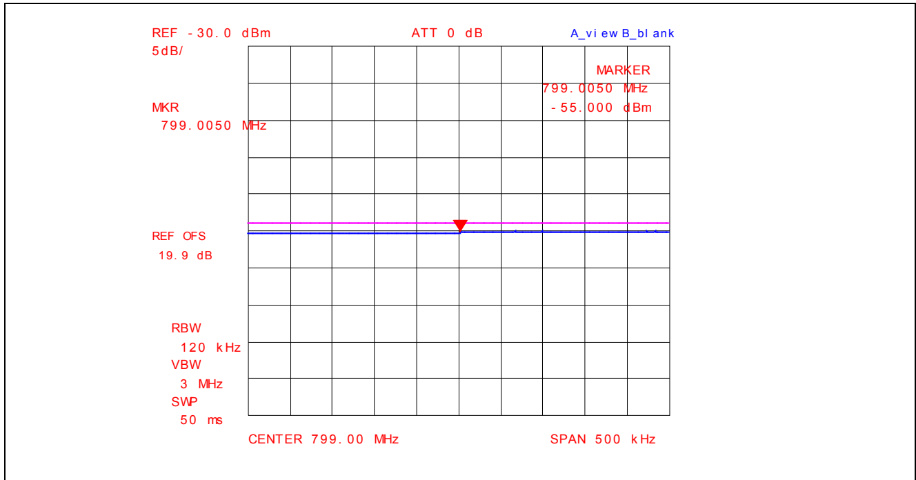
Plot 5.4.4.3.89. Conducted Spurious Emissions – Restricted Bands, 802.11n 400ns, 7.2 Mbps BPSK 1/2 2412 MHz, QP Power at 799.01MHz with Band (Notch) Reject Filter
