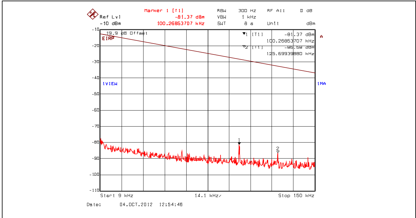
Plot 5.4.4.3.96. Conducted Spurious Emissions – Restricted Bands, 802.11n 400ns, 7.2 Mbps BPSK 1/2 2442 MHz, 9 kHz - 150 kHz, Peak Detector with Band (Notch) Reject Filter
