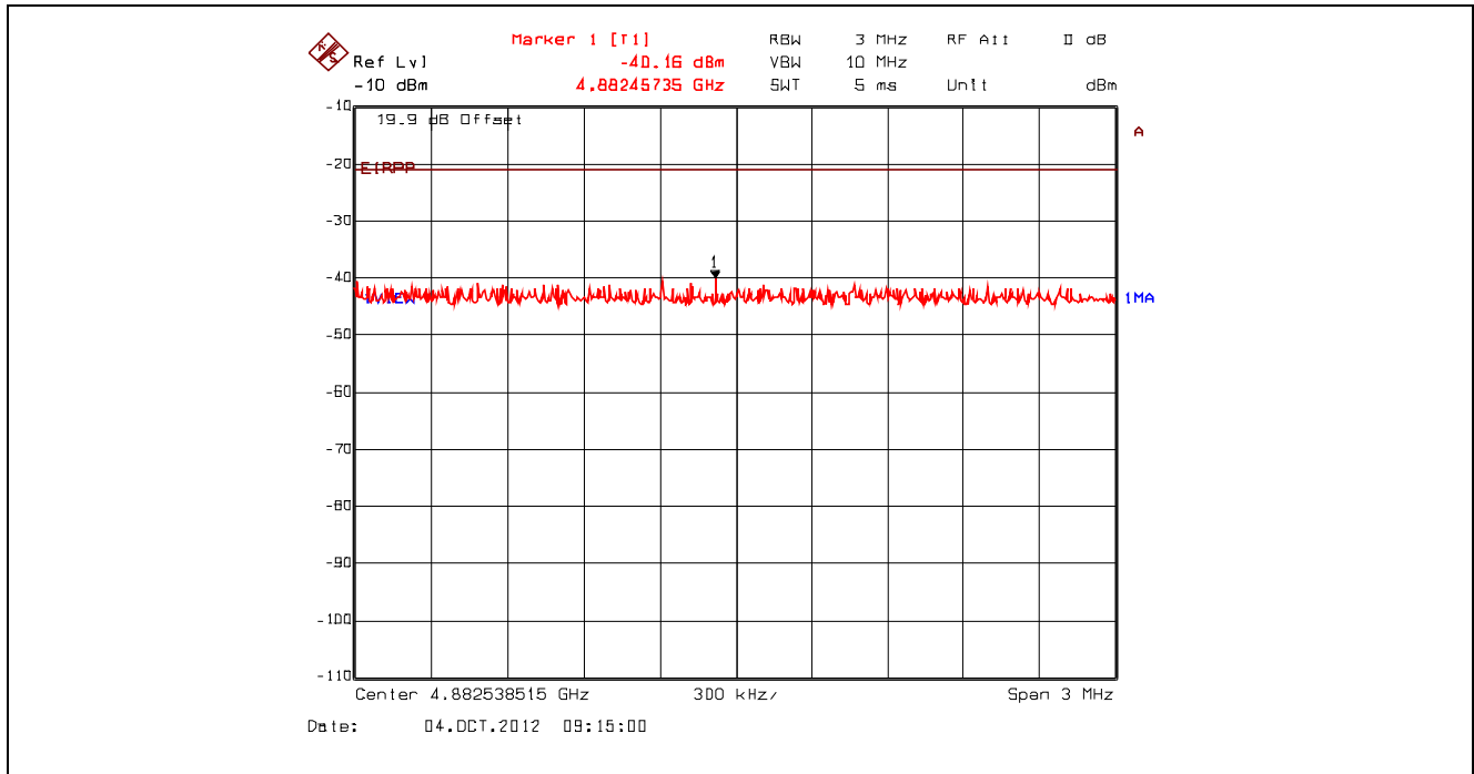
Plot 5.4.4.3.104. Conducted Spurious Emissions – Restricted Bands, 802.11n 400ns, 7.2 Mbps BPSK 1/2 2442 MHz, Peak Power at 4.88 GHz with High Pass Filter
