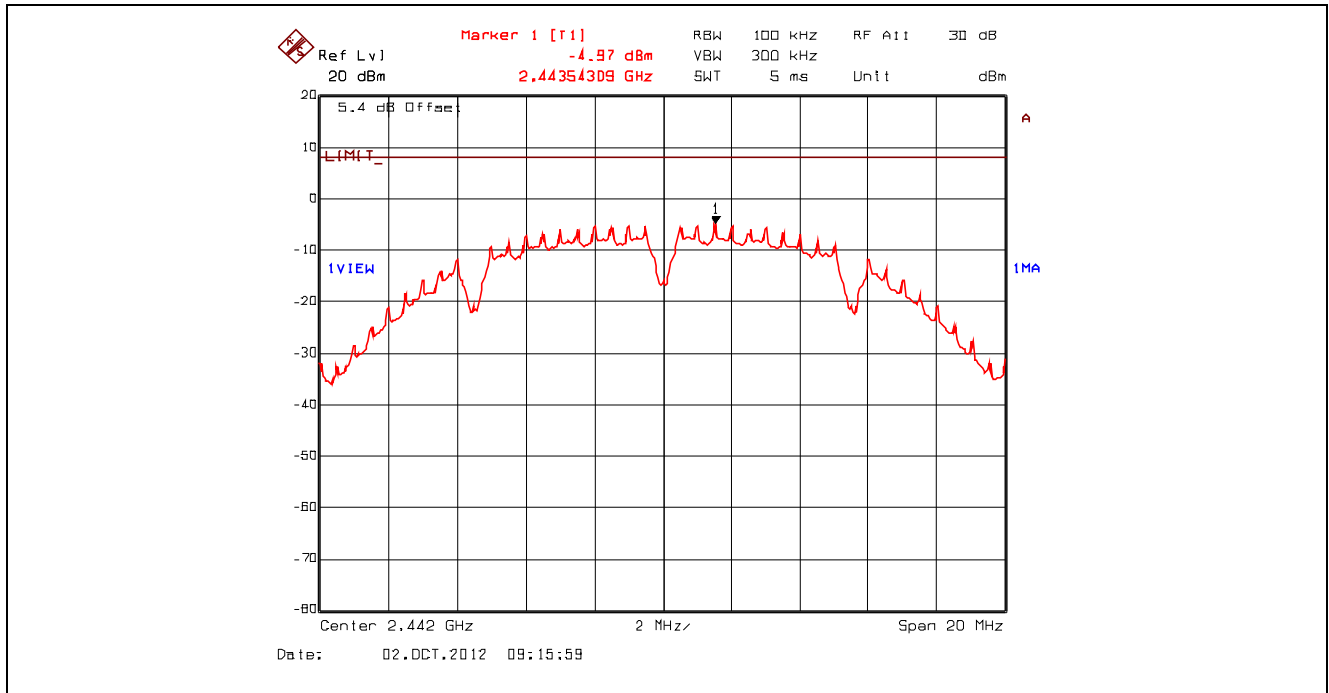
Plot 5.6.4.2. Power Spectral Density, 802.11b, 1 Mbps DBPSK, 2442 MHz, Setting 23 Offset: Insertion Loss + BWCF = 20.63 dB + 10*log(3 kHz/ 100 kHz) = 5.43 dB
