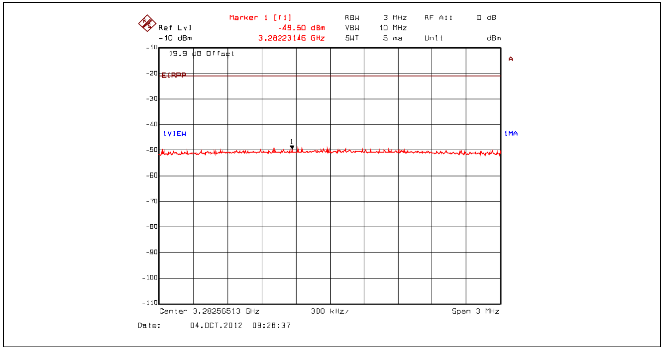
Plot 5.4.4.3.113. Conducted Spurious Emissions – Restricted Bands, 802.11n 400ns, 7.2 Mbps BPSK 1/2 2462 MHz, Peak Power at 3.28 GHz with Band (Notch) Reject Filter
