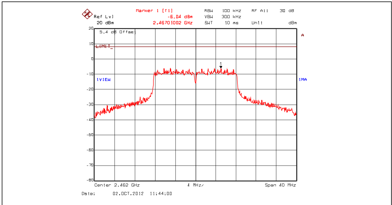
Plot 5.6.4.21. Power Spectral Density, 802.11g, 54 Mbps 64-QAM, 2462 MHz, Setting 23 Offset: Insertion Loss + BWCF = 20.63 dB + 10*log(3 kHz/ 100 kHz) = 5.43 dB
