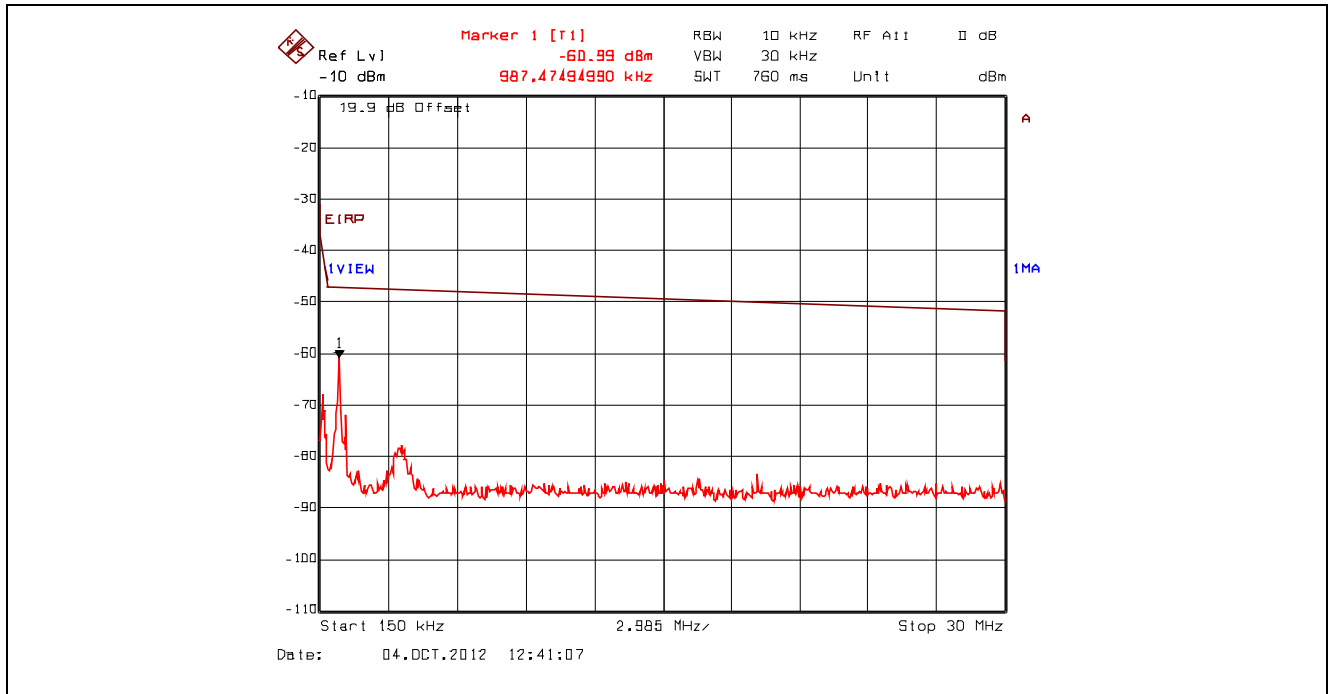
Plot 5.4.4.3.77. Conducted Spurious Emissions – Restricted Bands, 802.11n 800ns, 6.5 Mbps BPSK 1/2 2462 MHz, 150 kHz - 30 MHz, Peak Detector with Band (Notch) Reject Filter
