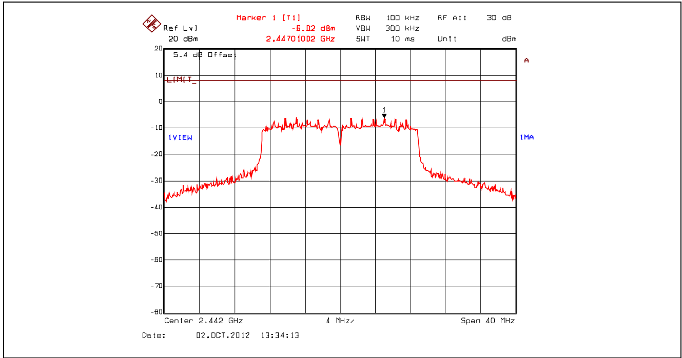
Plot 5.6.4.44. Power Spectral Density, 802.11n 400ns, 72.2 Mbps 64-QAM 5/6, 2442 MHz, Setting 23 Offset: Insertion Loss + BWCF = 20.63 dB + 10*log(3 kHz/ 100 kHz) = 5.43 dB
