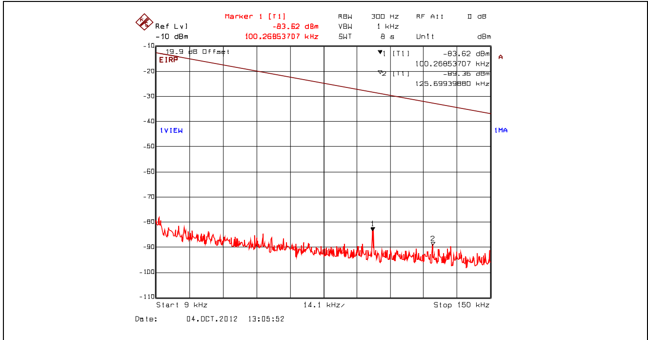
Plot 5.4.4.3.66. Conducted Spurious Emissions – Restricted Bands, 802.11n 800ns, 6.5 Mbps BPSK 1/2 2442 MHz, 9 kHz - 150 kHz, Peak Detector with Band (Notch) Reject Filter
