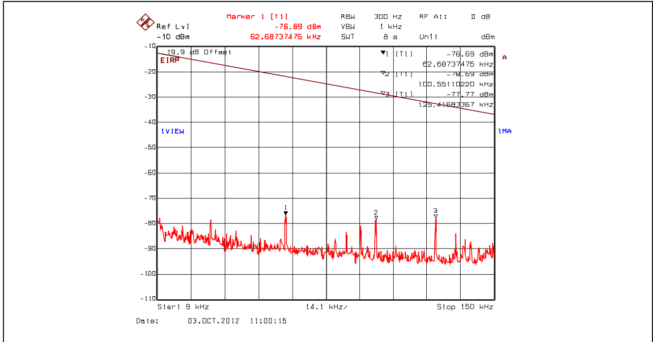
Plot 5.4.4.3.26. Conducted Spurious Emissions – Restricted Bands, 802.11g, 9 Mbps BPSK 2412 MHz, 9 kHz - 150 kHz, Peak Detector with Band (Notch) Reject Filter
