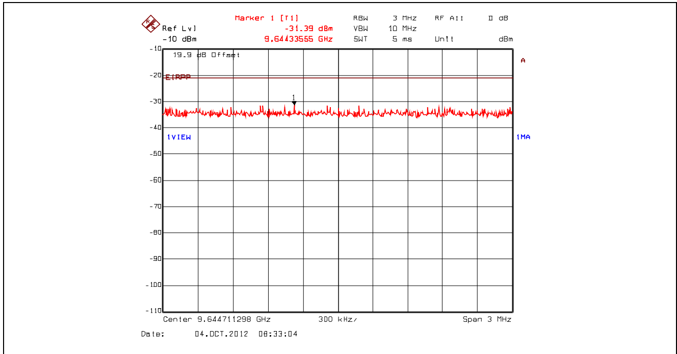
Plot 5.4.4.3.35. Conducted Spurious Emissions – Restricted Bands, 802.11g, 9 Mbps BPSK 2412 MHz, Peak Power at 9.64 GHz with High Pass Filter
