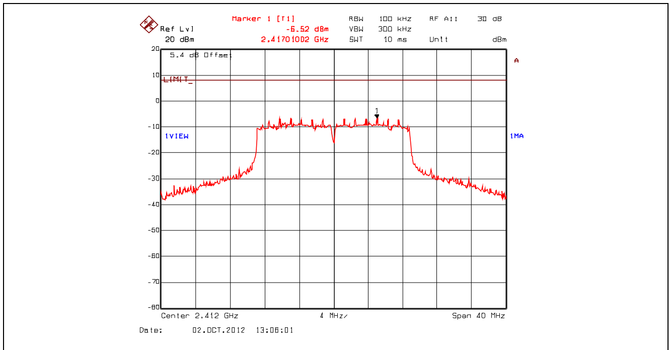
Plot 5.6.4.43. Power Spectral Density, 802.11n 400ns, 72.2 Mbps 64-QAM 5/6, 2412 MHz, Setting 23 Offset: Insertion Loss + BWCF = 20.63 dB + 10*log(3 kHz/ 100 kHz) = 5.43 dB
