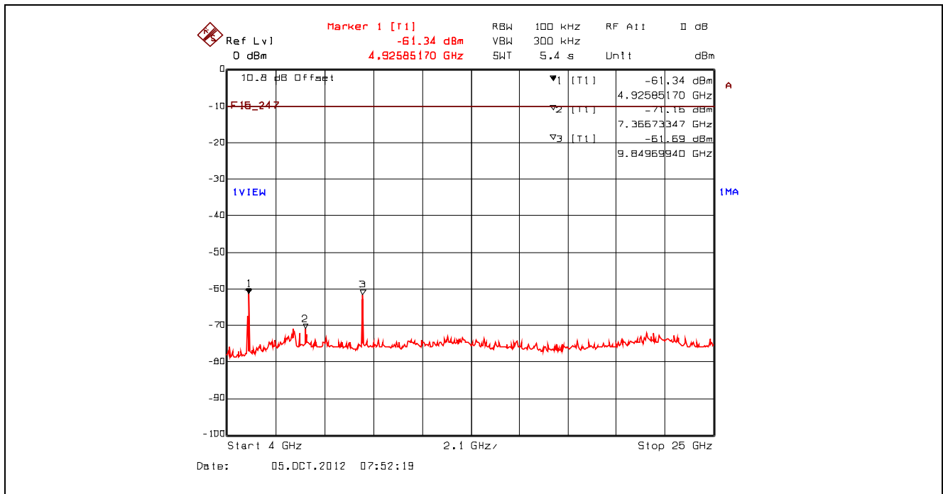
Plot 5.4.4.2.18. Conducted Spurious Emissions - Non Restricted Frequency Bands, 802.11n 800ns, 4 GHz – 25 GHz 2462 MHz, High Power, 6.5 Mbps BPSK 1/2, Power Setting 23 dBm
