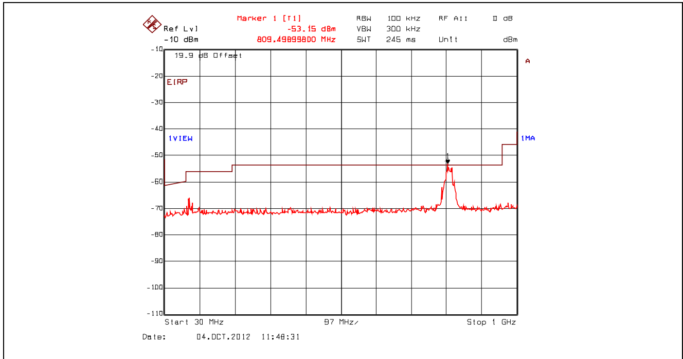
Plot 5.4.4.3.98. Conducted Spurious Emissions – Restricted Bands, 802.11n 400ns, 7.2 Mbps BPSK 1/2 2442 MHz, 30 MHz - 1 GHz, Peak Detector with Band (Notch) Reject Filter
