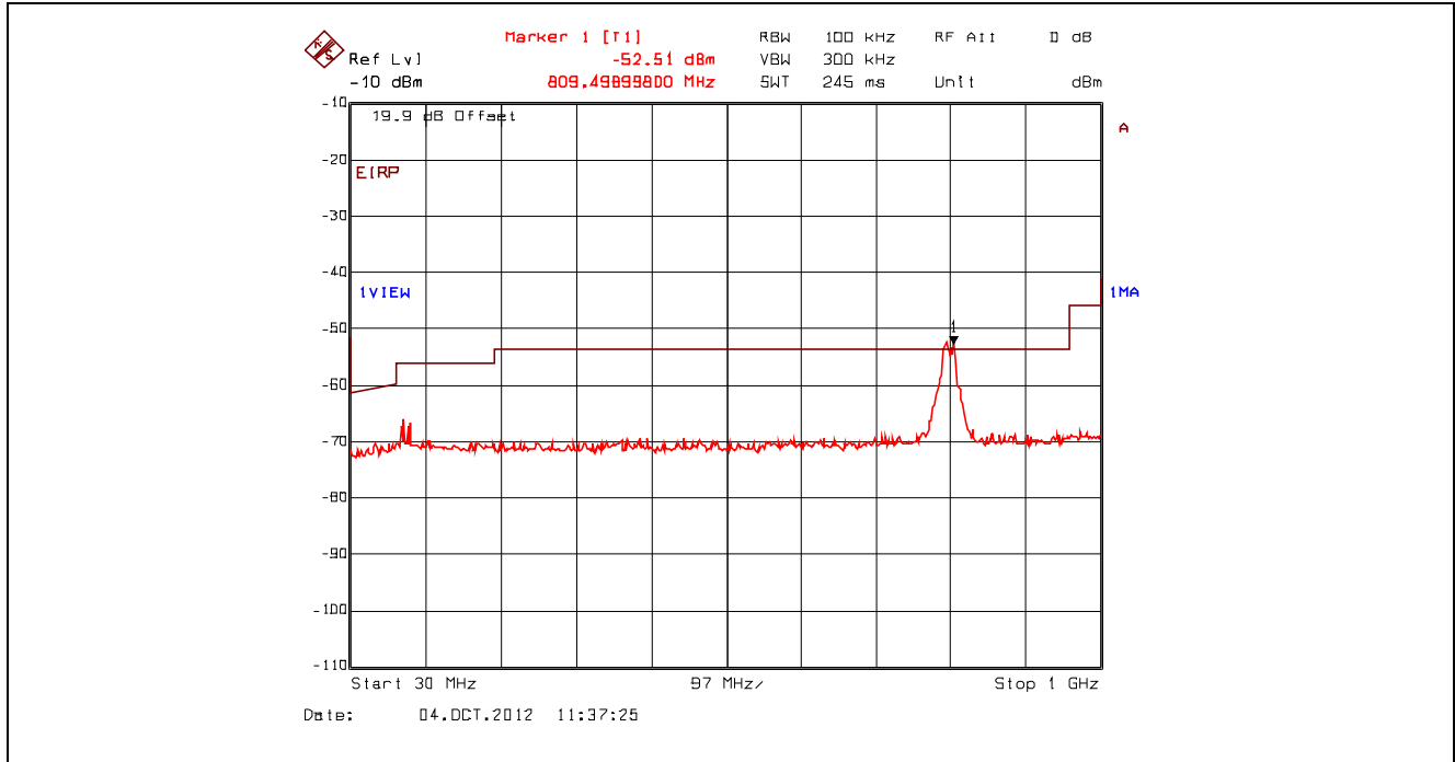
Plot 5.4.4.3.58. Conducted Spurious Emissions – Restricted Bands, 802.11n 800ns, 6.5 Mbps BPSK 1/2 2412 MHz, 30 MHz - 1 GHz, Peak Detector with Band (Notch) Reject Filter
