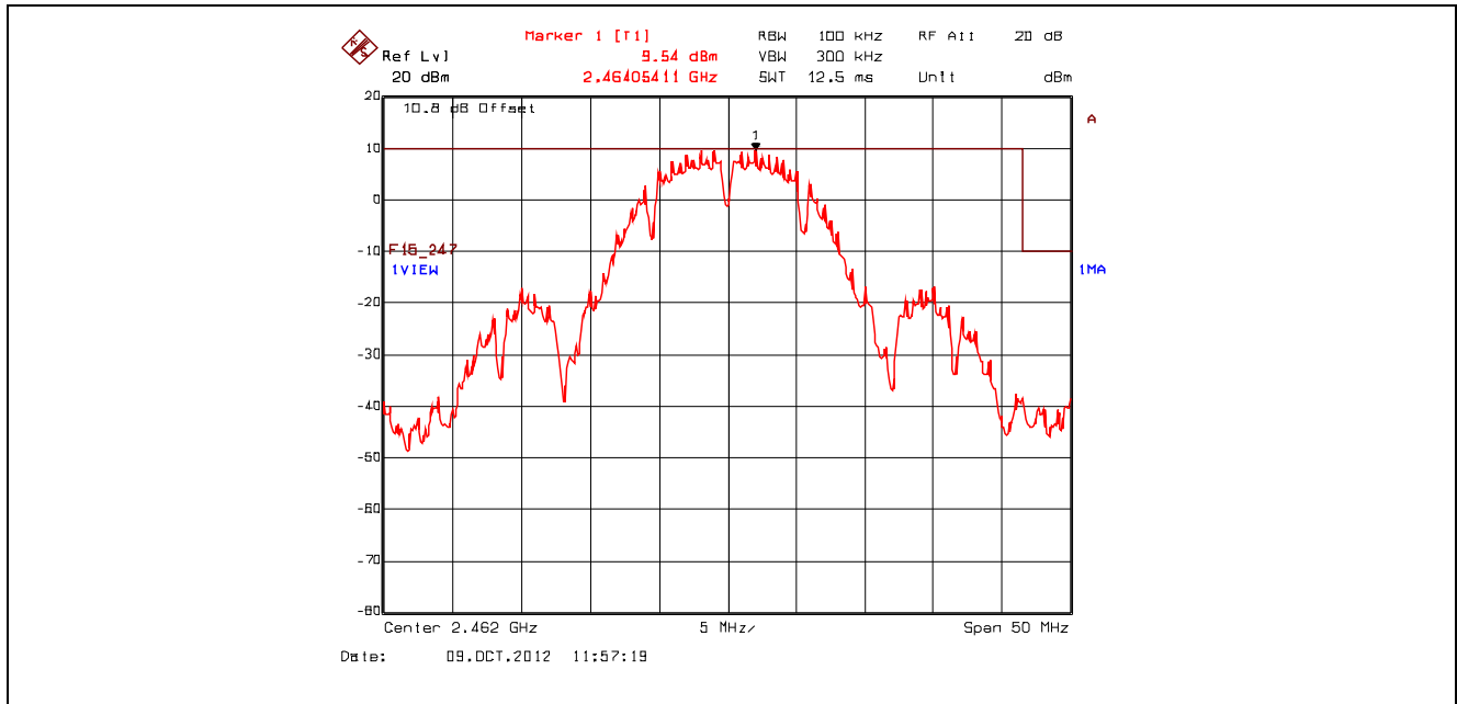
Plot 5.4.4.1.2. Band-Edge RF Conducted Emissions, Upper Band-edge, 2462 MHz, 802.11b, 1 Mbps DBPSK
