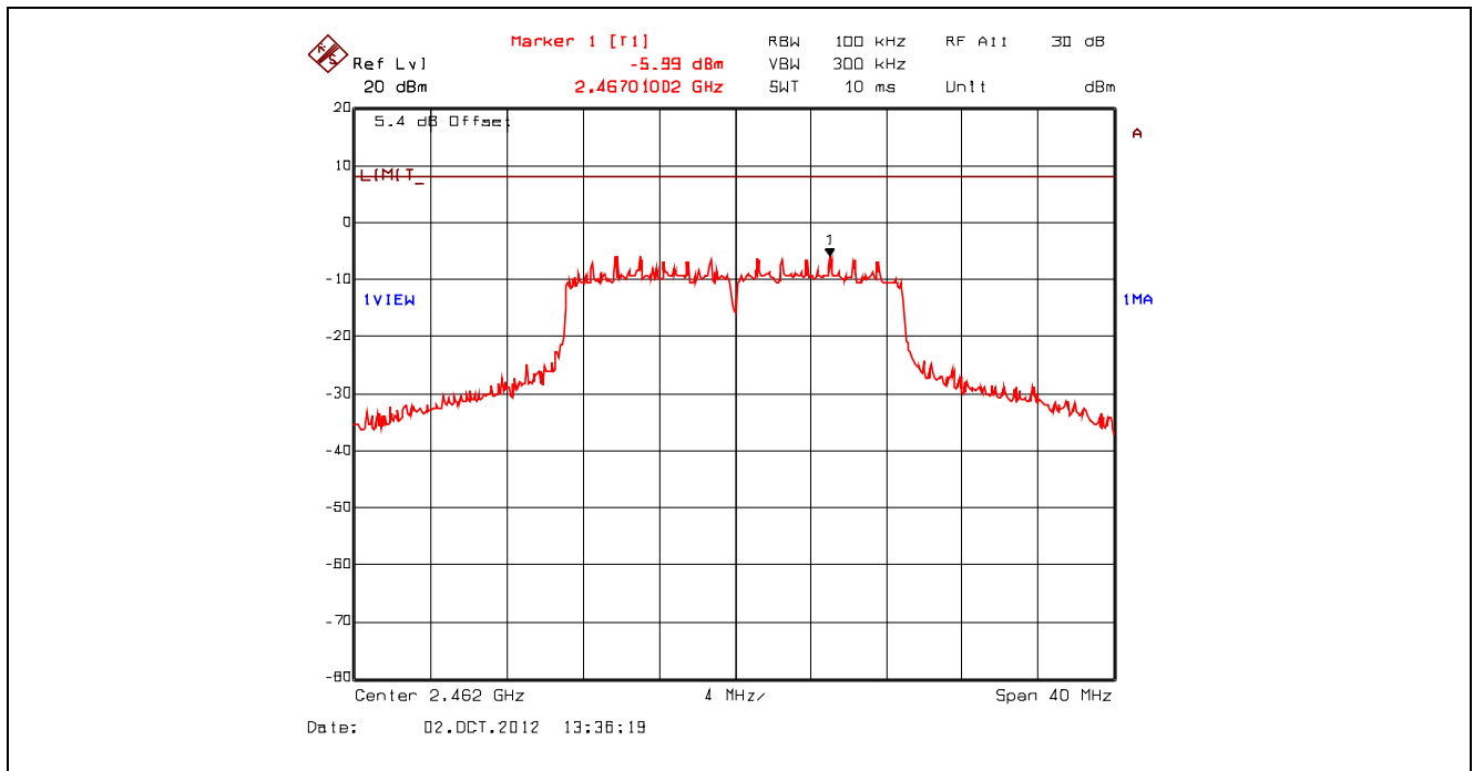
Plot 5.6.4.45. Power Spectral Density, 802.11n 400ns, 72.2 Mbps 64-QAM 5/6, 2462 MHz, Setting 23 Offset: Insertion Loss + BWCF = 20.63 dB + 10*log(3 kHz/ 100 kHz) = 5.43 dB
