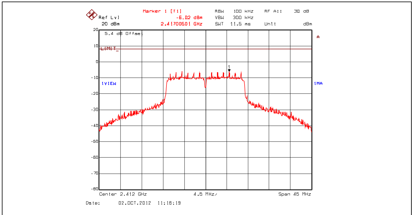
Plot 5.6.4.13. Power Spectral Density, 802.11g, 18 Mbps QPSK, 2412 MHz, Setting 23 Offset: Insertion Loss + BWCF = 20.63 dB + 10*log(3 kHz/ 100 kHz) = 5.43 dB
