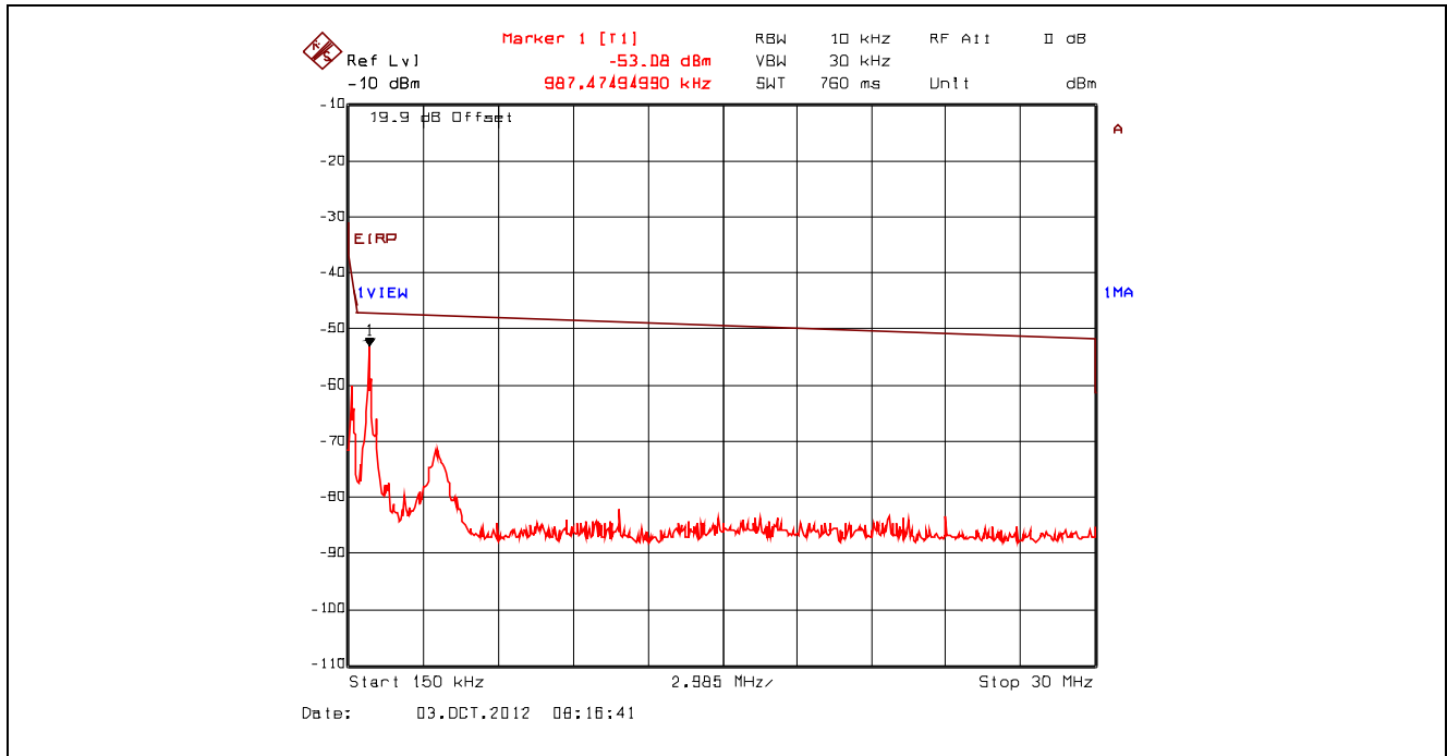
Plot 5.4.4.3.11. Conducted Spurious Emissions – Restricted Bands, 802.11b, 11 Mbps CCK 2442 MHz, 150 kHz - 30 MHz, Peak Detector with Band (Notch) Reject Filter
