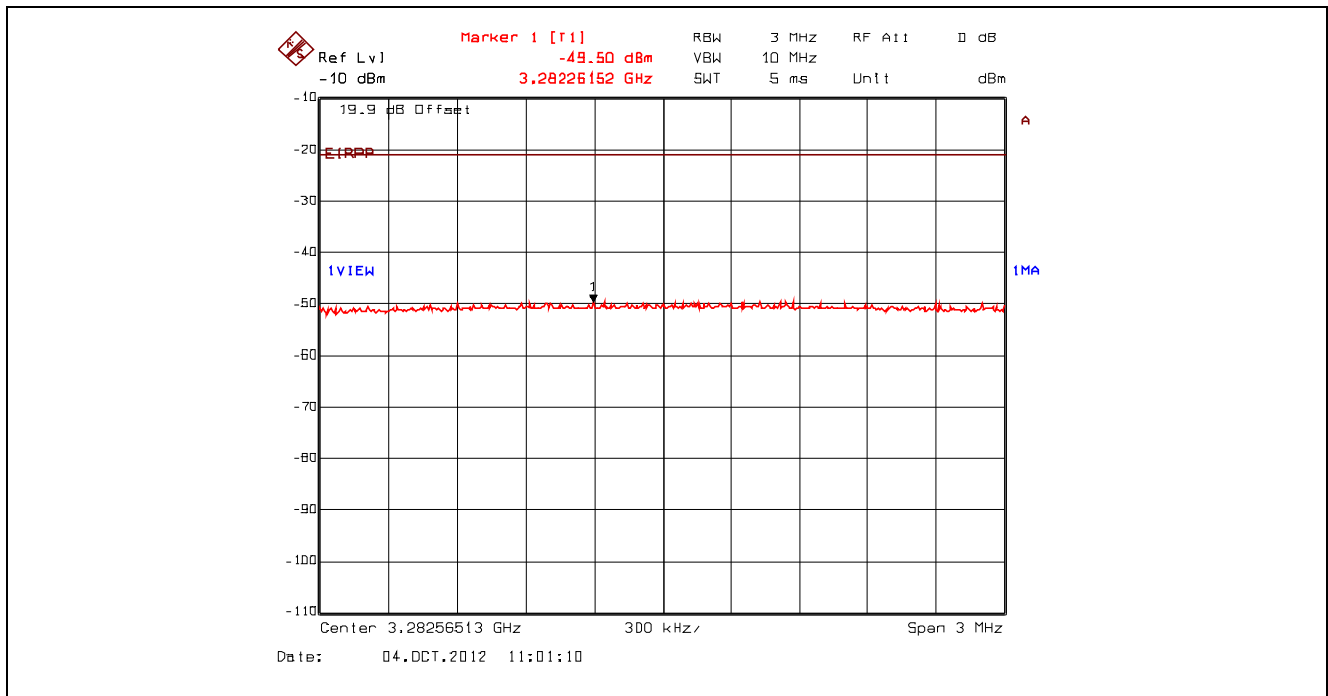
Plot 5.4.4.3.83. Conducted Spurious Emissions – Restricted Bands, 802.11n 800ns, 6.5 Mbps BPSK 1/2 2462 MHz, Peak Power at 3.28 GHz with Band (Notch) Reject Filter
