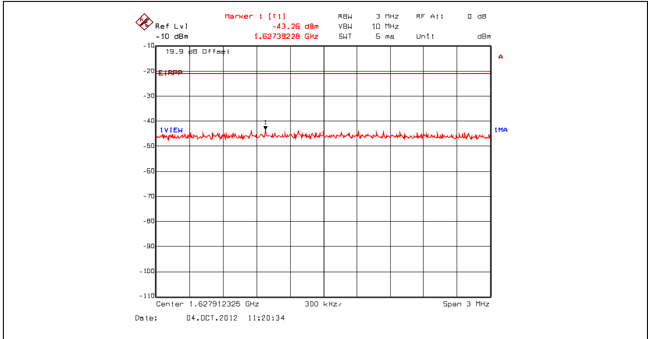
Plot 5.4.4.3.42. Conducted Spurious Emissions – Restricted Bands, 802.11g, 9 Mbps BPSK 2442 MHz, Peak Power at 1.63 GHz with Band (Notch) Reject Filter
