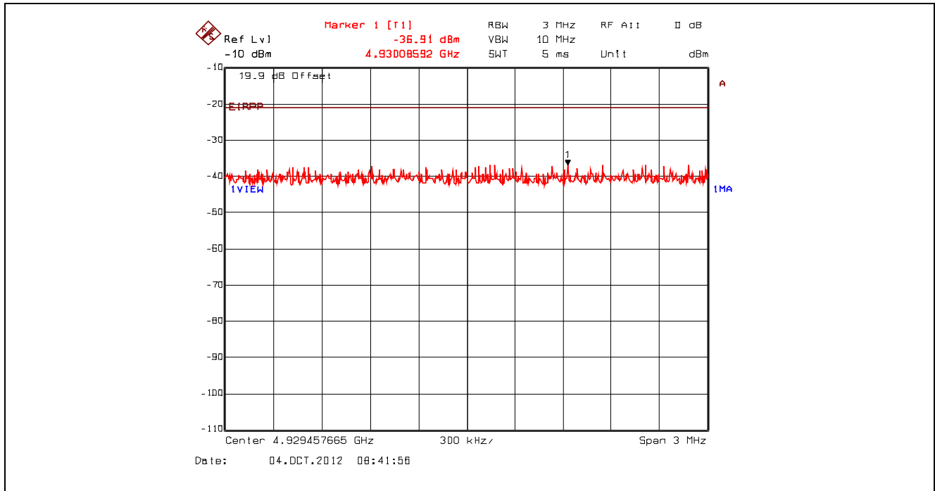
Plot 5.4.4.3.54. Conducted Spurious Emissions – Restricted Bands, 802.11g, 9 Mbps BPSK 2462 MHz, Peak Power at 4.93 GHz with High Pass Filter
