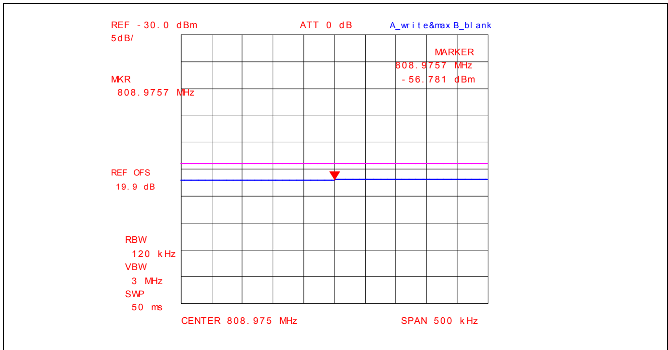
Plot 5.4.4.3.99. Conducted Spurious Emissions – Restricted Bands, 802.11n 400ns, 7.2 Mbps BPSK 1/2 2442 MHz, QP Power at 808.98 MHz with Band (Notch) Reject Filter
