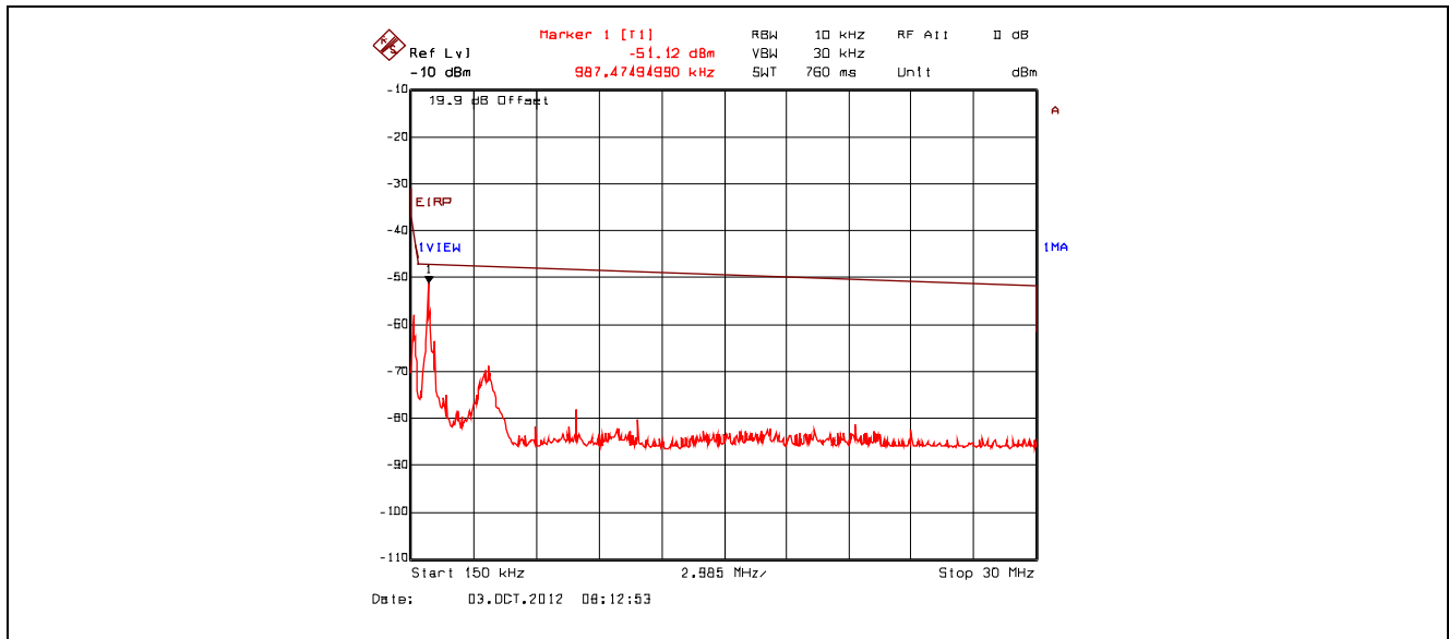
Plot 5.4.4.3.2. Conducted Spurious Emissions – Restricted Bands, 802.11b, 11 Mbps CCK 2412 MHz, 150 kHz - 30 MHz, Peak Detector with Band (Notch) Reject Filter
