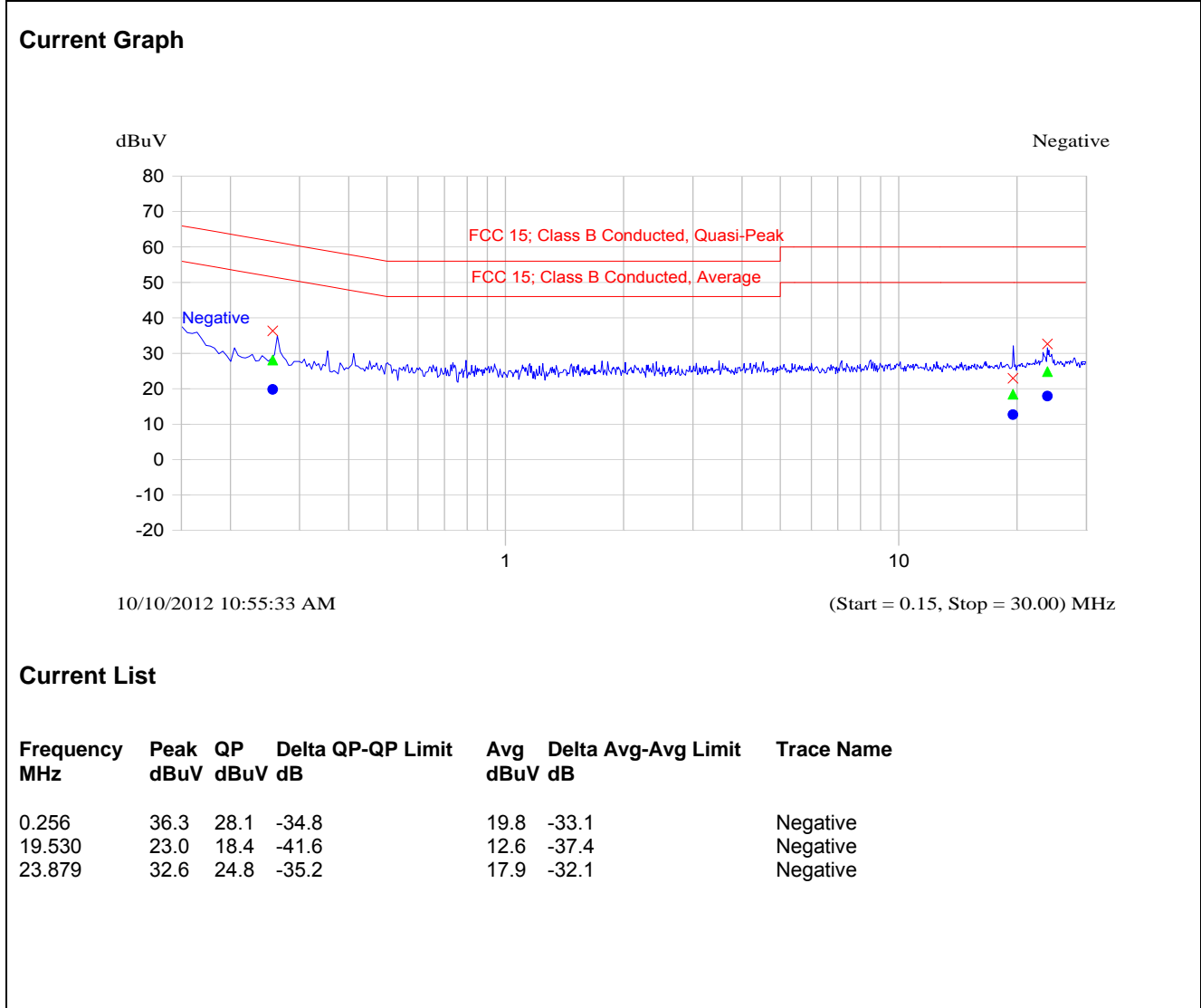
Plot 5.1.4.2. Power Line Conducted Emissions; Line Voltage: 3.5 V DC; Line Tested: Negative
