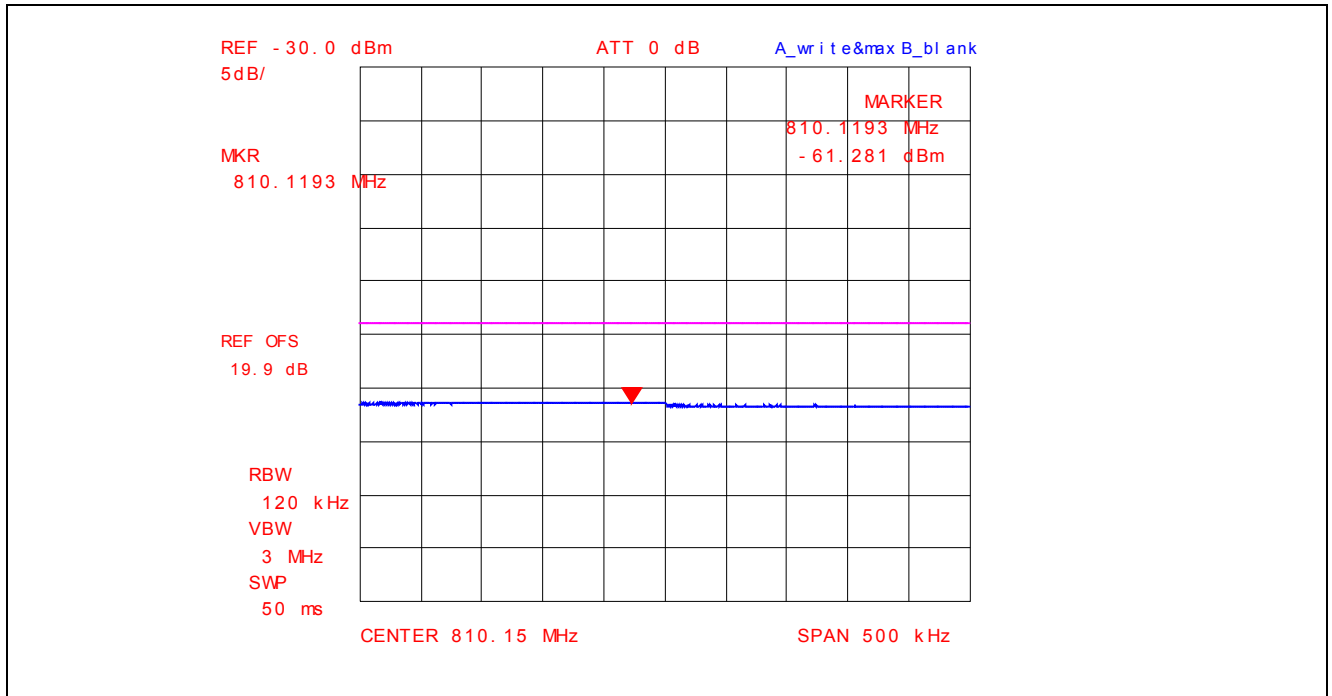
Plot 5.4.4.3.69. Conducted Spurious Emissions – Restricted Bands, 802.11n 800ns, 6.5 Mbps BPSK 1/2 2442 MHz, QP Power at 810.12 MHz with Band (Notch) Reject Filter
