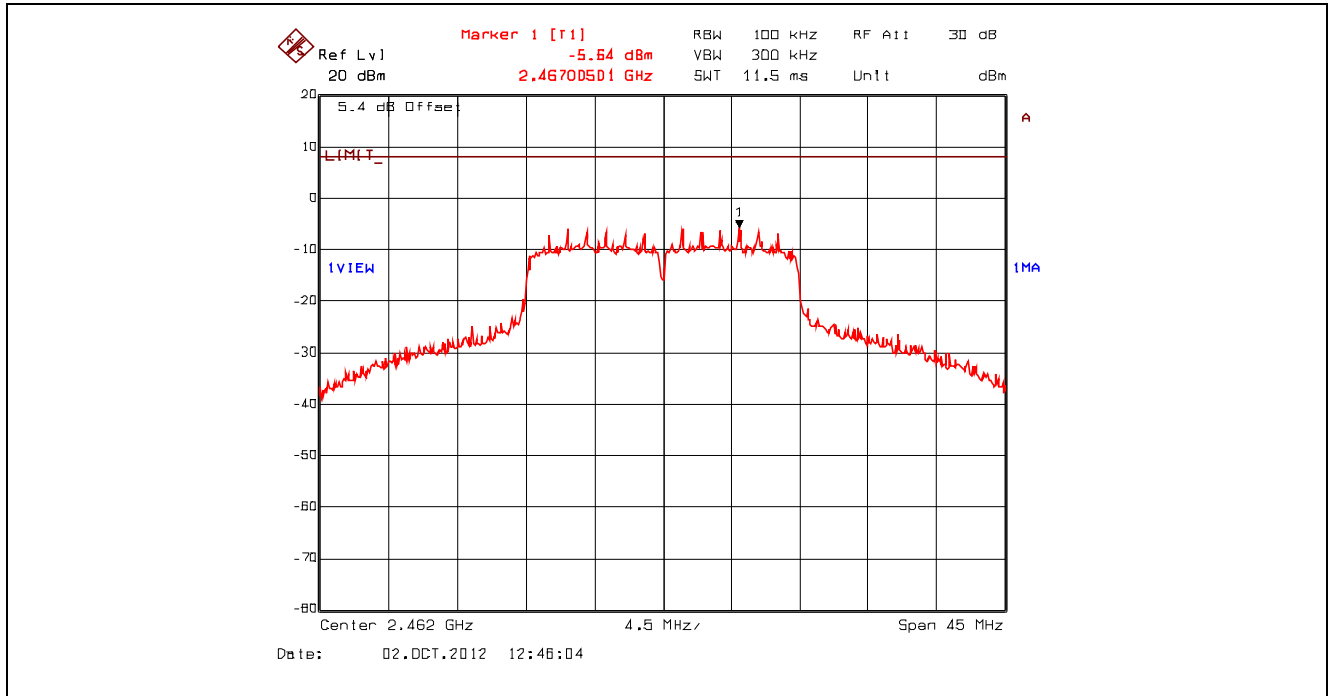
Plot 5.6.4.36. Power Spectral Density, 802.11n 400ns, 7.2 Mbps BPSK1/2, 2462 MHz, Setting 23 Offset: Insertion Loss + BWCF = 20.63 dB + 10*log(3 kHz/ 100 kHz) = 5.43 dB
