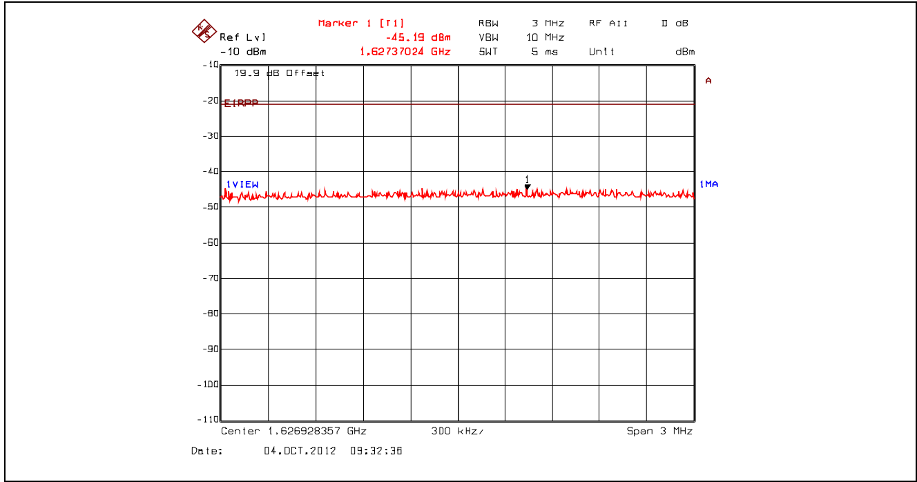
Plot 5.4.4.3.102. Conducted Spurious Emissions – Restricted Bands, 802.11n 400ns, 7.2 Mbps BPSK 1/2 2442 MHz, Peak Power at 1.63 GHz with Band (Notch) Reject Filter
