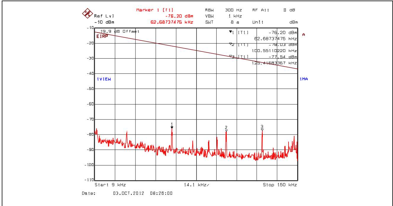
Plot 5.4.4.3.18. Conducted Spurious Emissions – Restricted Bands, 802.11b, 11 Mbps CCK 2462 MHz, 9 kHz - 150 kHz, Peak Detector with Band (Notch) Reject Filter
