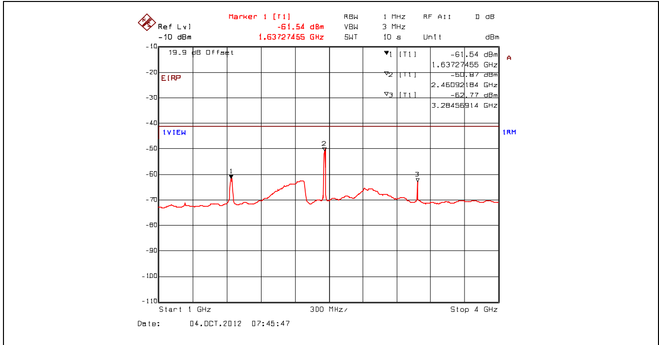
Plot 5.4.4.3.80. Conducted Spurious Emissions – Restricted Bands, 802.11n 800ns, 6.5 Mbps BPSK 1/2 2462 MHz, 1 GHz - 4 GHz, Power Averaging with Band (Notch) Reject Filter
