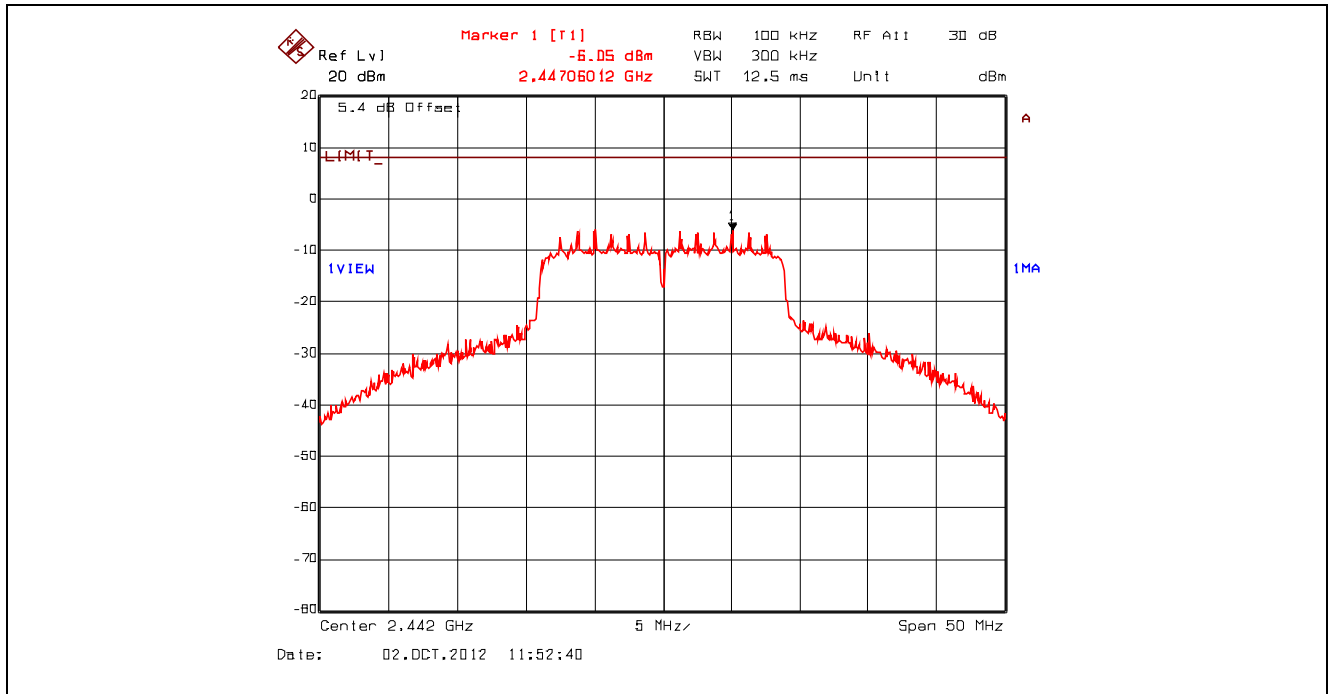
Plot 5.6.4.23. Power Spectral Density, 802.11n 800ns, 6.5 Mbps BPSK1/2, 2442 MHz, Setting 23 Offset: Insertion Loss + BWCF = 20.63 dB + 10*log(3 kHz/ 100 kHz) = 5.43 dB
