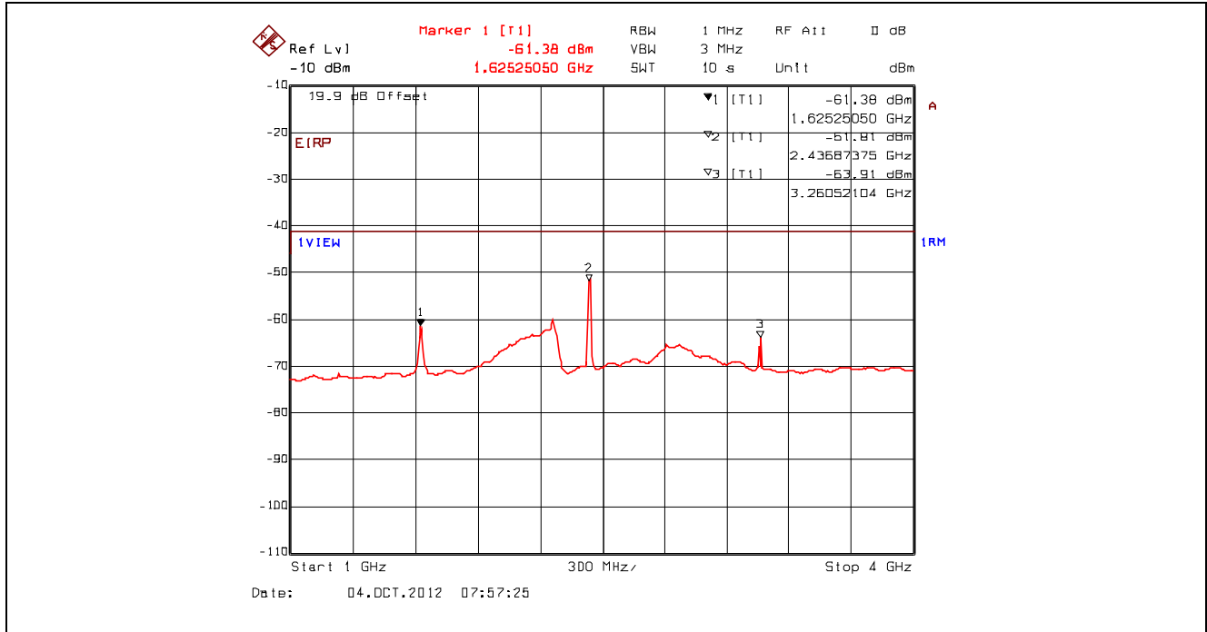
Plot 5.4.4.3.100. Conducted Spurious Emissions – Restricted Bands, 802.11n 400ns, 7.2 Mbps BPSK 1/2 2442 MHz, 1 GHz - 4 GHz, Power Averaging with Band (Notch) Reject Filter
