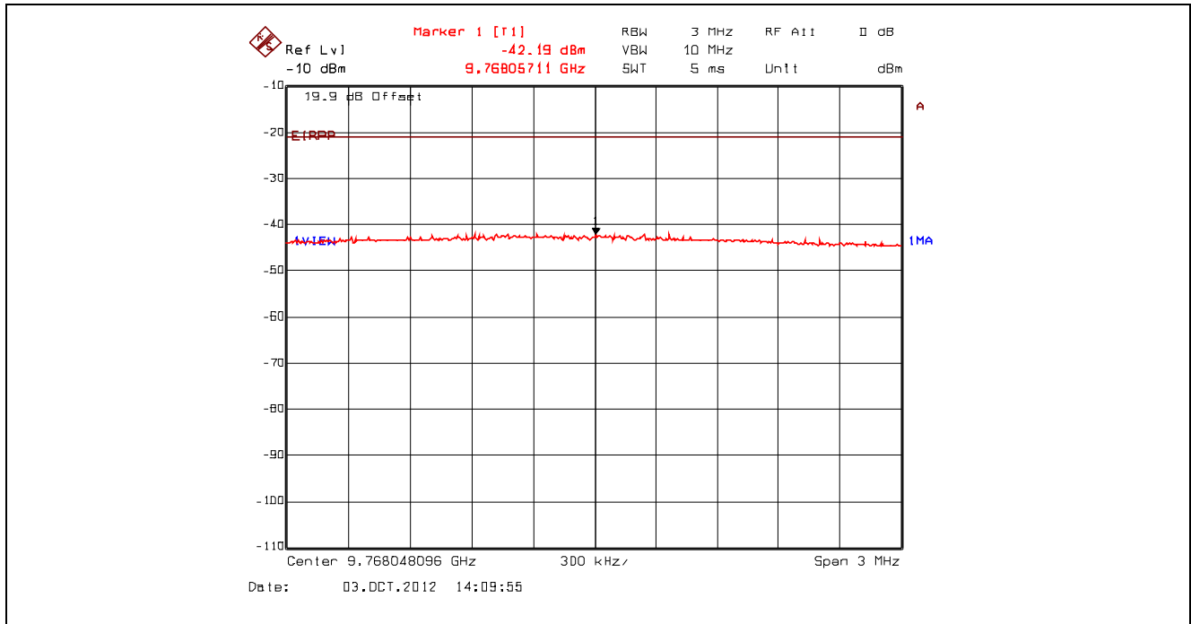
Plot 5.4.4.3.17. Conducted Spurious Emissions – Restricted Bands, 802.11b, 11 Mbps CCK 2442 MHz, Peak Power at 9.77 GHz with High Pass Filter
