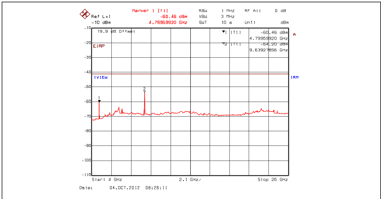
Plot 5.4.4.3.31. Conducted Spurious Emissions – Restricted Bands, 802.11g, 9 Mbps BPSK 2412 MHz, 4 GHz - 25 GHz, Power Averaging with High Pass Filter
