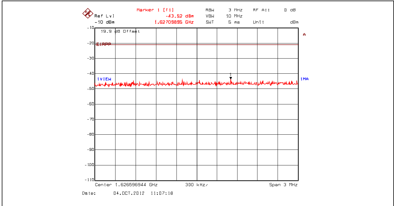
Plot 5.4.4.3.72. Conducted Spurious Emissions – Restricted Bands, 802.11n 800ns, 6.5 Mbps BPSK 1/2 2442 MHz, Peak Power at 1.63 GHz with Band (Notch) Reject Filter
