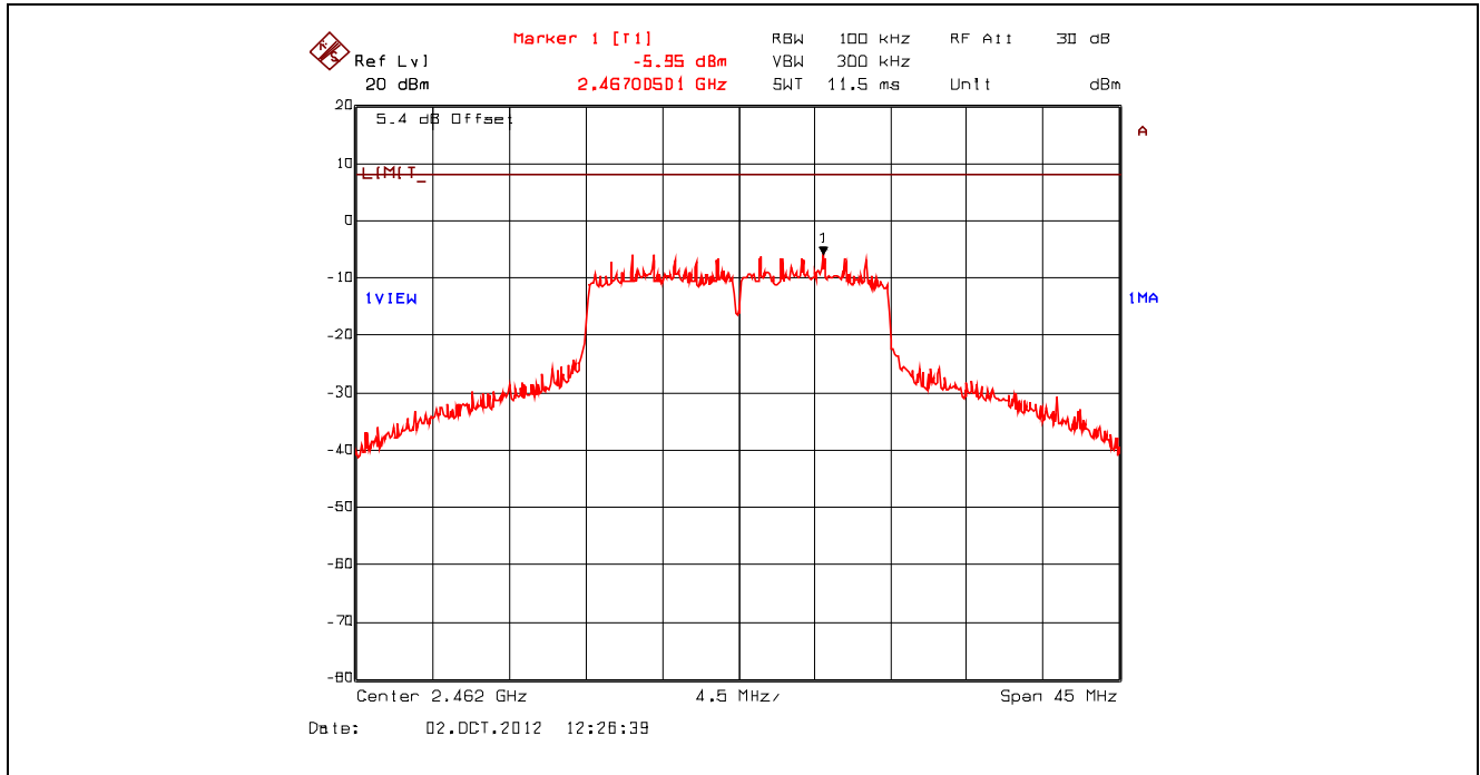
Plot 5.6.4.30. Power Spectral Density, 802.11n 800ns, 39 Mbps 16-QAM 3/4, 2462 MHz, Setting 23 Offset: Insertion Loss + BWCF = 20.63 dB + 10 \cdot \log(3 \text{ kHz} / 100 \text{ kHz}) = 5.43 \text{ dB}
