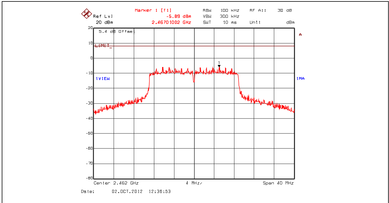
Plot 5.6.4.33. Power Spectral Density, 802.11n 800ns, 65 Mbps 64-QAM 5/6, 2462 MHz, Setting 23 Offset: Insertion Loss + BWCF = 20.63 dB + 10*log(3 kHz/ 100 kHz) = 5.43 dB
