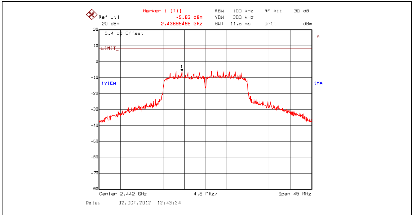
Plot 5.6.4.35. Power Spectral Density, 802.11n 400ns, 7.2 Mbps BPSK1/2, 2442 MHz, Setting 23 Offset: Insertion Loss + BWCF = 20.63 dB + 10*log(3 kHz/ 100 kHz) = 5.43 dB
