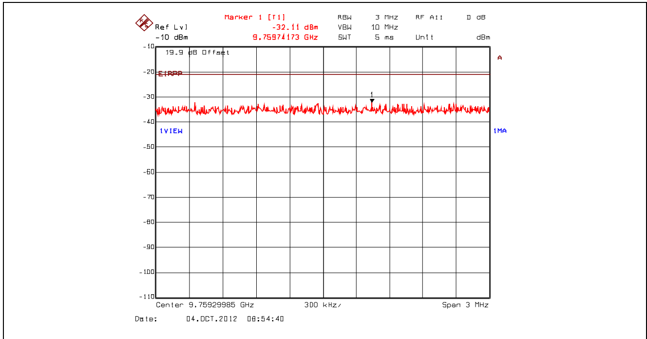
Plot 5.4.4.3.75. Conducted Spurious Emissions – Restricted Bands, 802.11n 800ns, 6.5 Mbps BPSK 1/2 2442 MHz, Peak Power at 9.76 GHz with High Pass Filter
