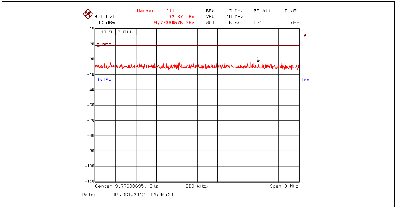
Plot 5.4.4.3.45. Conducted Spurious Emissions – Restricted Bands, 802.11g, 9 Mbps BPSK 2442 MHz, Peak Power at 9.77 GHz with High Pass Filter
