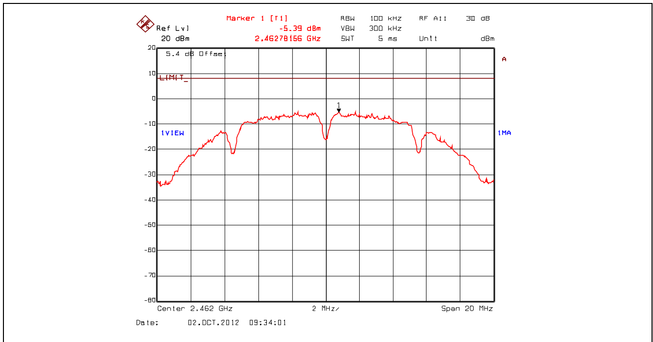
Plot 5.6.4.6. Power Spectral Density, 802.11b, 2 Mbps DQPSK, 2462 MHz, Setting 23 Offset: Insertion Loss + BWCF = 20.63 dB + 10*log(3 kHz/ 100 kHz) = 5.43 dB
