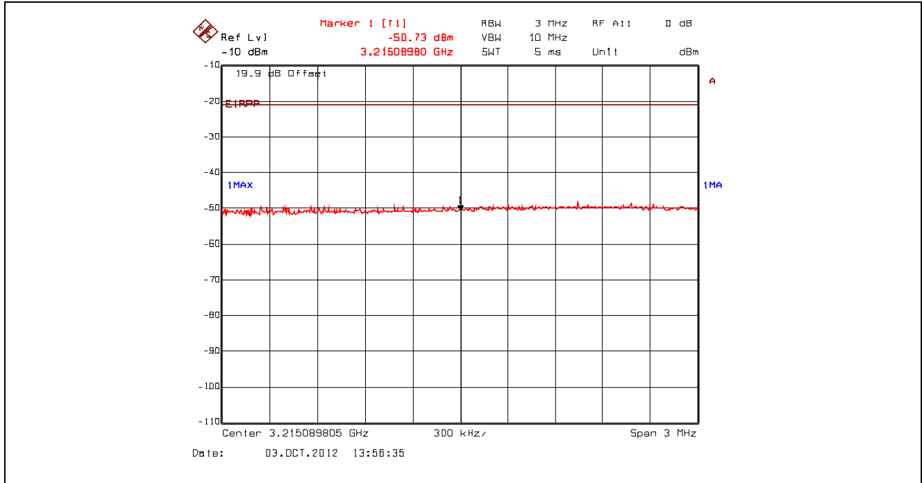
Plot 5.4.4.3.7. Conducted Spurious Emissions – Restricted Bands, 802.11b, 11 Mbps CCK 2412 MHz, Peak Power at 3.22 GHz with Band (Notch) Reject Filter
