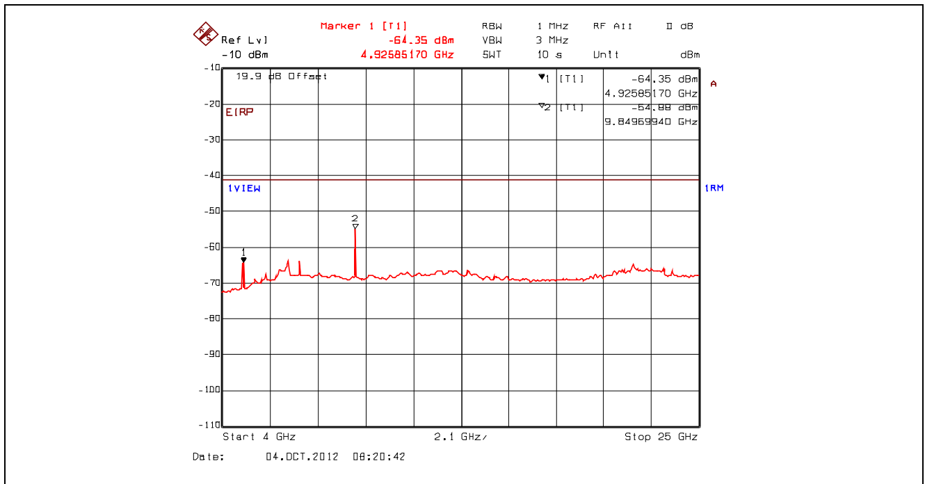
Plot 5.4.4.3.51. Conducted Spurious Emissions – Restricted Bands, 802.11g, 9 Mbps BPSK 2462 MHz, 4 GHz - 25 GHz, Power Averaging with High Pass Filter
