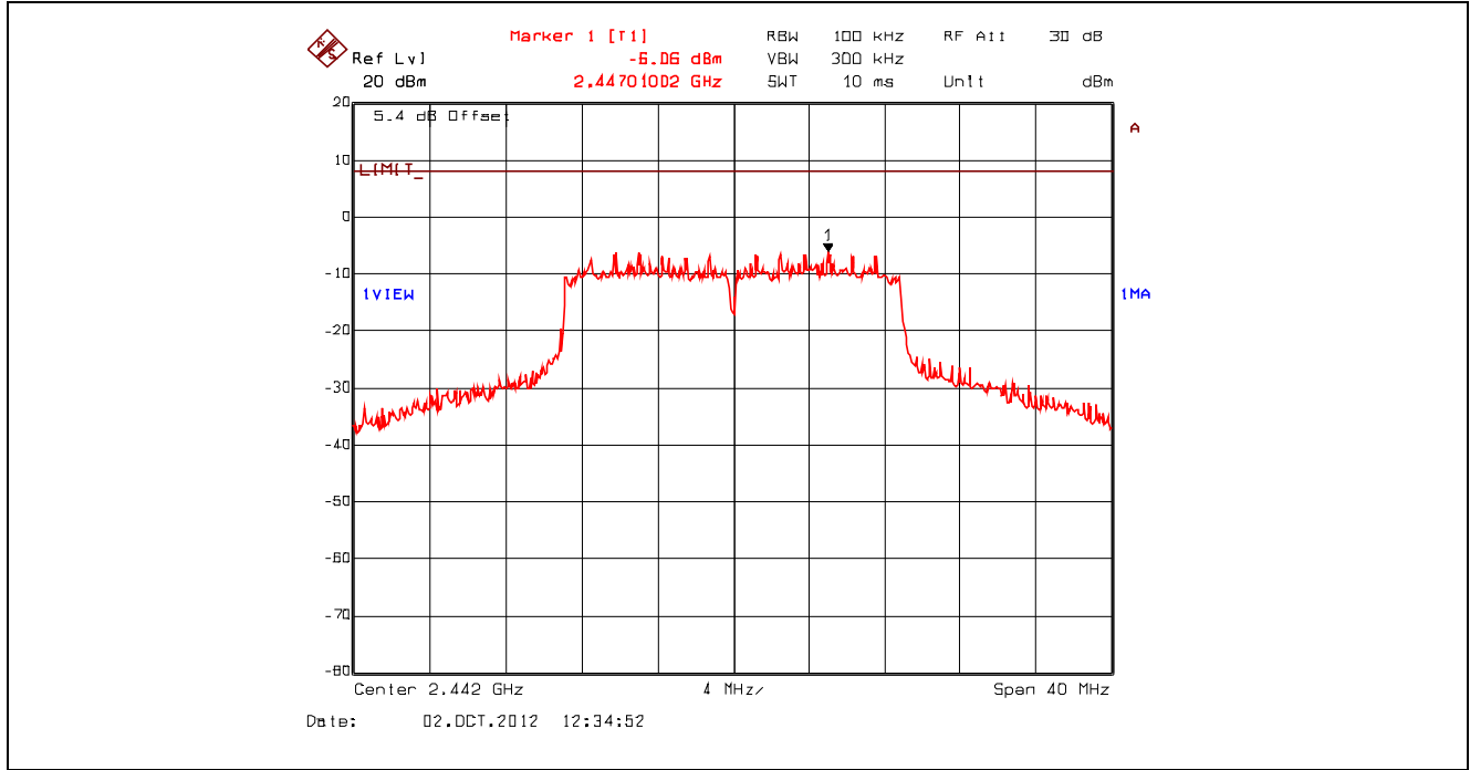
Plot 5.6.4.32. Power Spectral Density, 802.11n 800ns, 65 Mbps 64-QAM 5/6, 2442 MHz, Setting 23 Offset: Insertion Loss + BWCF = 20.63 dB + 10*log(3 kHz/ 100 kHz) = 5.43 dB
