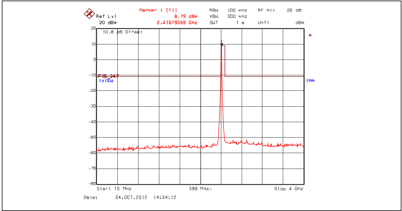
Plot 5.4.4.2.13. Conducted Spurious Emissions - Non Restricted Frequency Bands, 802.11n 800ns, 10 MHz – 4 GHz 2412 MHz, High Power, 6.5 Mbps BPSK 1/2, Power Setting 23 dBm
