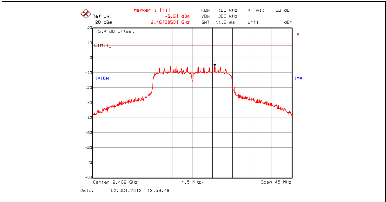
Plot 5.6.4.39. Power Spectral Density, 802.11n 400ns, 21.7 Mbps QPSK 3/4, 2462 MHz, Setting 23 Offset: Insertion Loss + BWCF = 20.63 dB + 10 \cdot \log(3 \text{ kHz} / 100 \text{ kHz}) = 5.43 \text{ dB}
