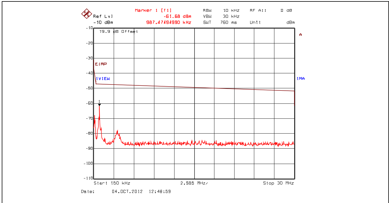
Plot 5.4.4.3.107. Conducted Spurious Emissions – Restricted Bands, 802.11n 400ns, 7.2 Mbps BPSK 1/2 2462 MHz, 150 kHz - 30 MHz, Peak Detector with Band (Notch) Reject Filter
