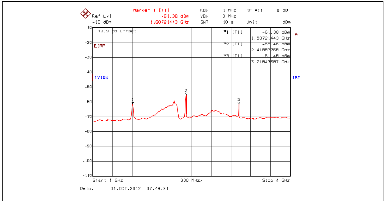
Plot 5.4.4.3.90. Conducted Spurious Emissions – Restricted Bands, 802.11n 400ns, 7.2 Mbps BPSK 1/2 2412 MHz, 1 GHz - 4 GHz, Power Averaging with Band (Notch) Reject Filter
