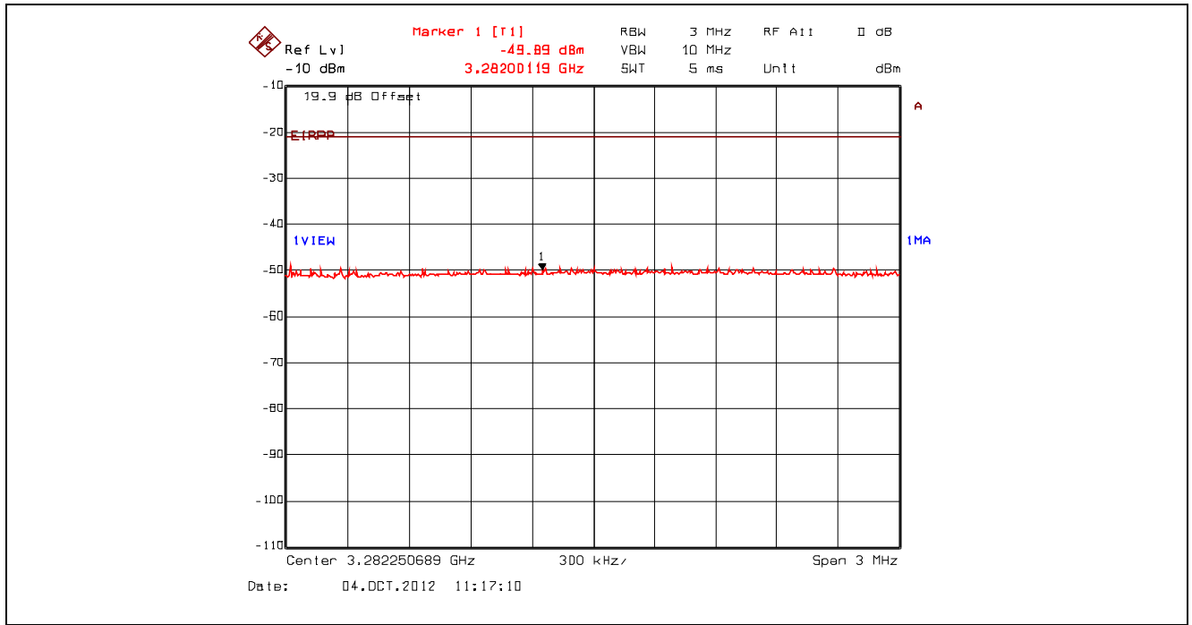
Plot 5.4.4.3.53. Conducted Spurious Emissions – Restricted Bands, 802.11g, 9 Mbps BPSK 2462 MHz, Peak Power at 3.28 GHz with Band (Notch) Reject Filter
