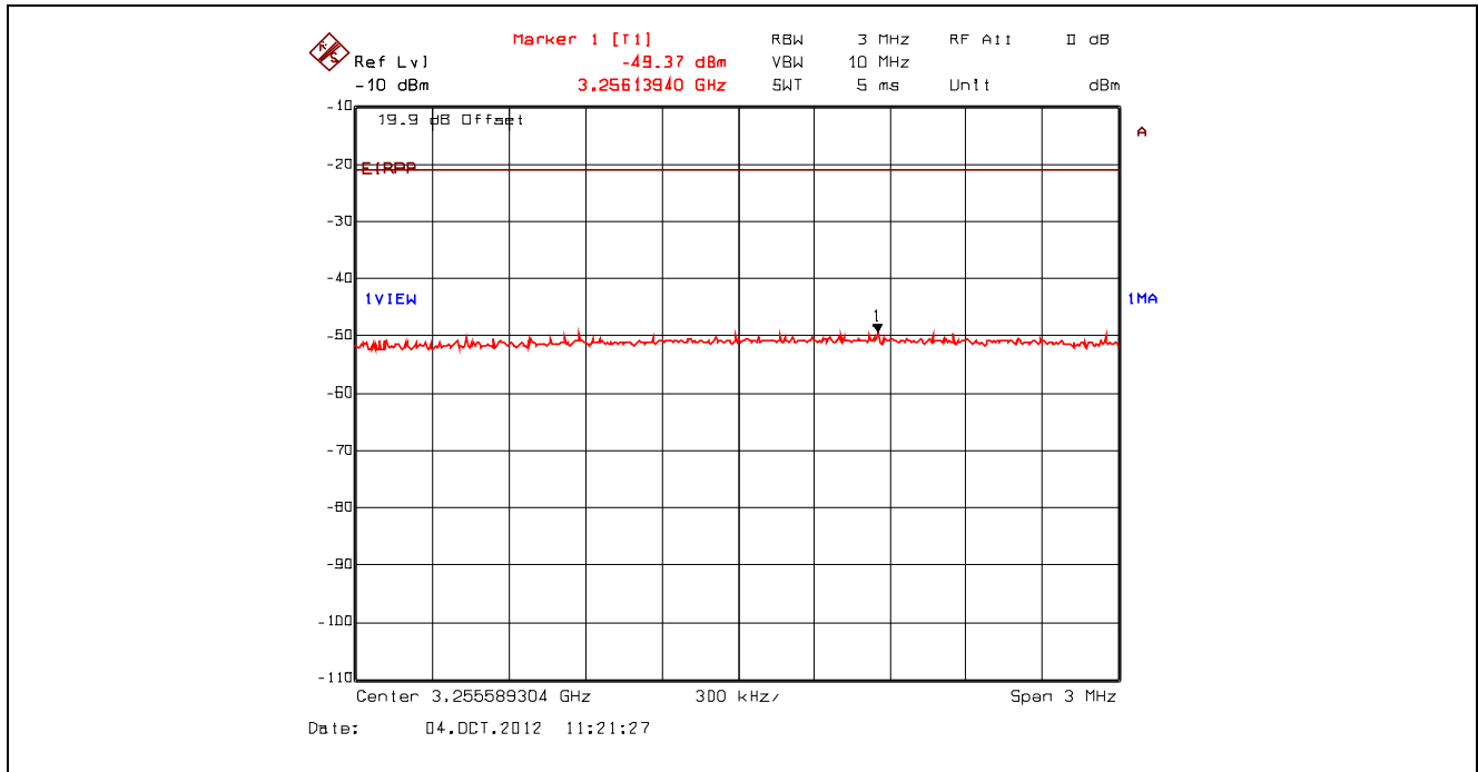
Plot 5.4.4.3.43. Conducted Spurious Emissions – Restricted Bands, 802.11g, 9 Mbps BPSK 2442 MHz, Peak Power at 3.26 GHz with Band (Notch) Reject Filter
