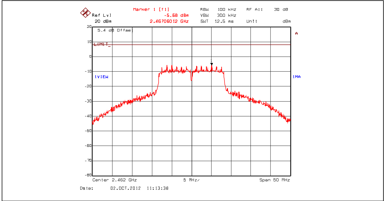
Plot 5.6.4.12. Power Spectral Density, 802.11g, 9 Mbps BPSK, 2462 MHz, Setting 23 Offset: Insertion Loss + BWCF = 20.63 dB + 10*log(3 kHz/ 100 kHz) = 5.43 dB
