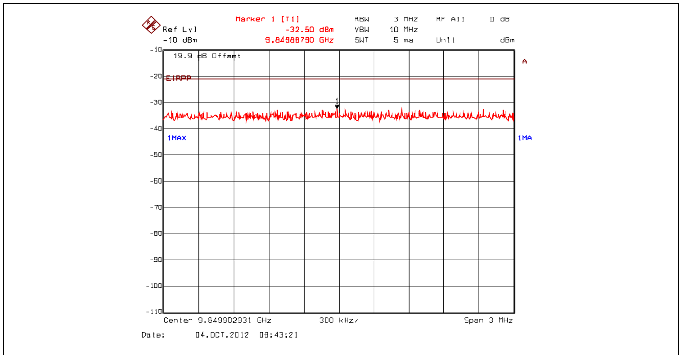
Plot 5.4.4.3.55. Conducted Spurious Emissions – Restricted Bands, 802.11g, 9 Mbps BPSK 2462 MHz, Peak Power at 9.85 GHz with High Pass Filter
