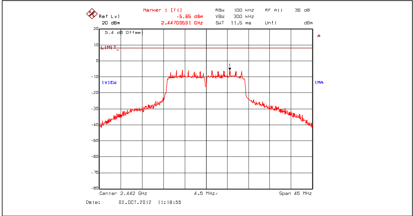
Plot 5.6.4.14. Power Spectral Density, 802.11g, 18 Mbps QPSK, 2442 MHz, Setting 23 Offset: Insertion Loss + BWCF = 20.63 dB + 10*log(3 kHz/ 100 kHz) = 5.43 dB
