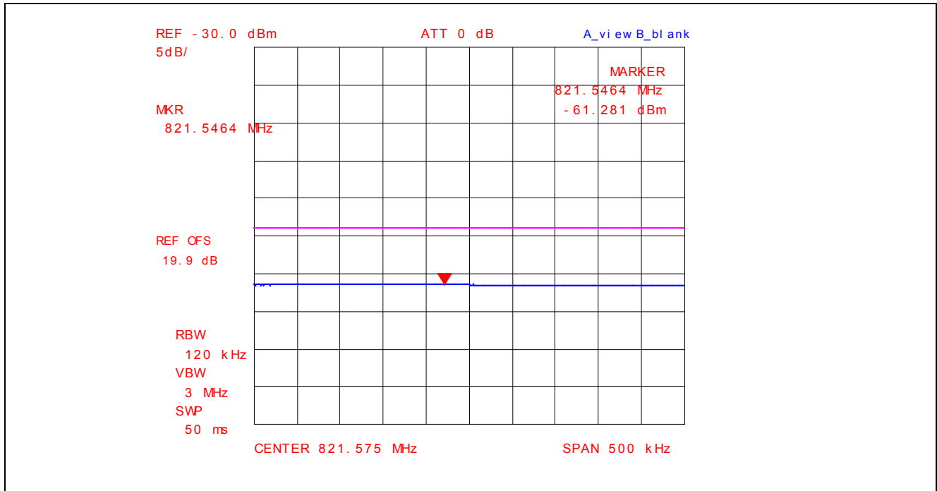
Plot 5.4.4.3.79. Conducted Spurious Emissions – Restricted Bands, 802.11n 800ns, 6.5 Mbps BPSK 1/2 2462 MHz, QP Power at 821.55 MHz with Band (Notch) Reject Filter
