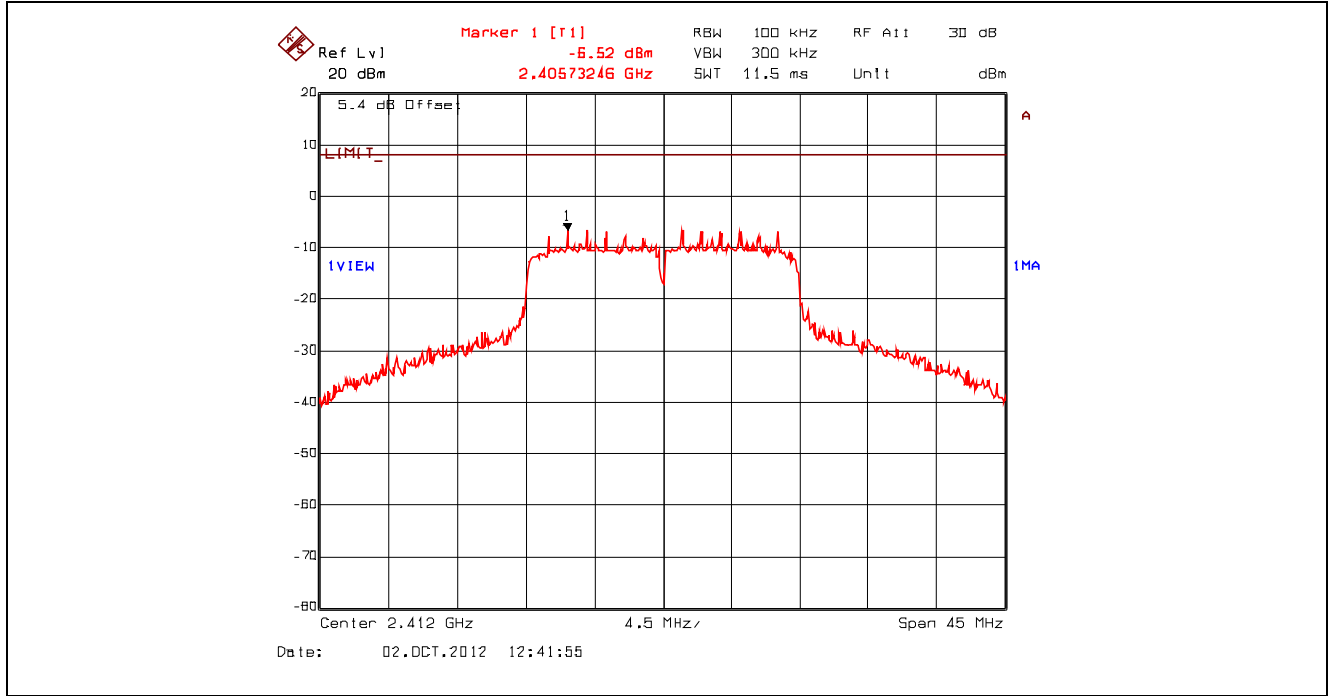
Plot 5.6.4.34. Power Spectral Density, 802.11n 400ns, 7.2 Mbps BPSK1/2, 2412 MHz, Setting 23 Offset: Insertion Loss + BWCF = 20.63 dB + 10*log(3 kHz/ 100 kHz) = 5.43 dB
