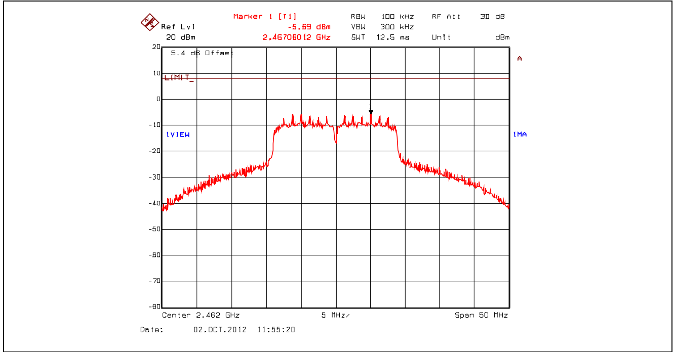
Plot 5.6.4.24. Power Spectral Density, 802.11n 800ns, 6.5 Mbps BPSK1/2, 2462 MHz, Setting 23 Offset: Insertion Loss + BWCF = 20.63 dB + 10*log(3 kHz/ 100 kHz) = 5.43 dB
