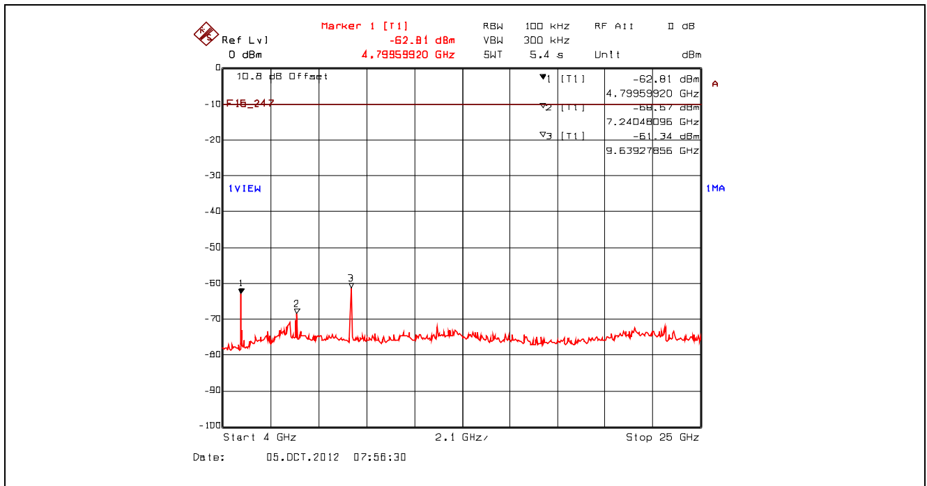
Plot 5.4.4.2.14. Conducted Spurious Emissions - Non Restricted Frequency Bands, 802.11n 800ns, 4 GHz – 25 GHz 2412 MHz, High Power, 6.5 Mbps BPSK 1/2, Power Setting 23 dBm
