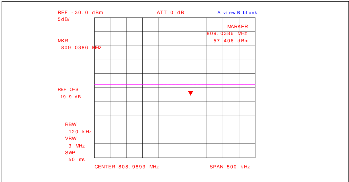
Plot 5.4.4.3.29. Conducted Spurious Emissions – Restricted Bands, 802.11g, 9 Mbps BPSK 2412 MHz, QP Power at 809.04 MHz with Band (Notch) Reject Filter
