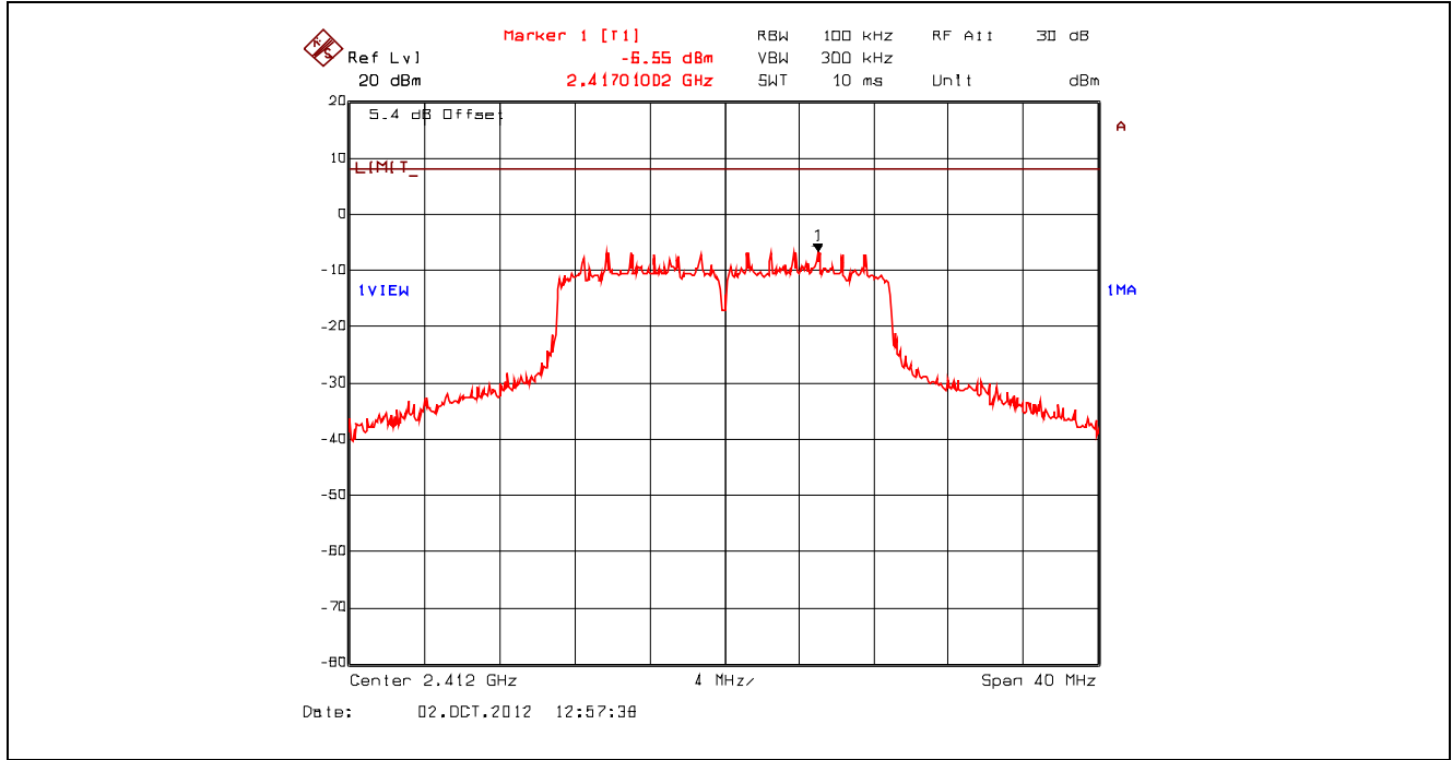
Plot 5.6.4.40. Power Spectral Density, 802.11n 400ns, 43.3 Mbps 16-QAM 3/4, 2412 MHz, Setting 23 Offset: Insertion Loss + BWCF = 20.63 dB + 10*log(3 kHz/ 100 kHz) = 5.43 dB
