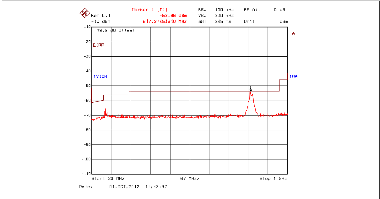
Plot 5.4.4.3.78. Conducted Spurious Emissions – Restricted Bands, 802.11n 800ns, 6.5 Mbps BPSK 1/2 2462 MHz, 30 MHz - 1 GHz, Peak Detector with Band (Notch) Reject Filter
