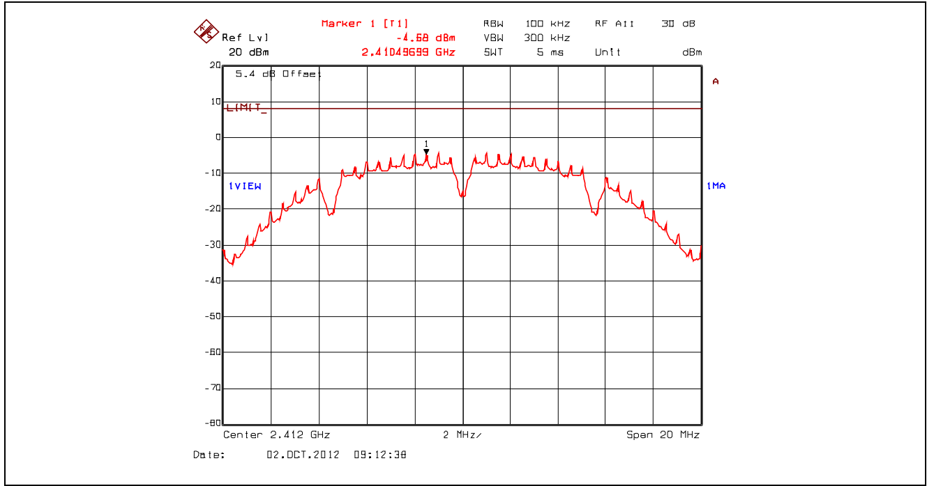
Plot 5.6.4.1. Power Spectral Density, 802.11b, 1 Mbps DBPSK, 2412 MHz, Setting 23 Offset: Insertion Loss + BWCF = 20.63 dB + 10*log(3 kHz/ 100 kHz) = 5.43 dB
