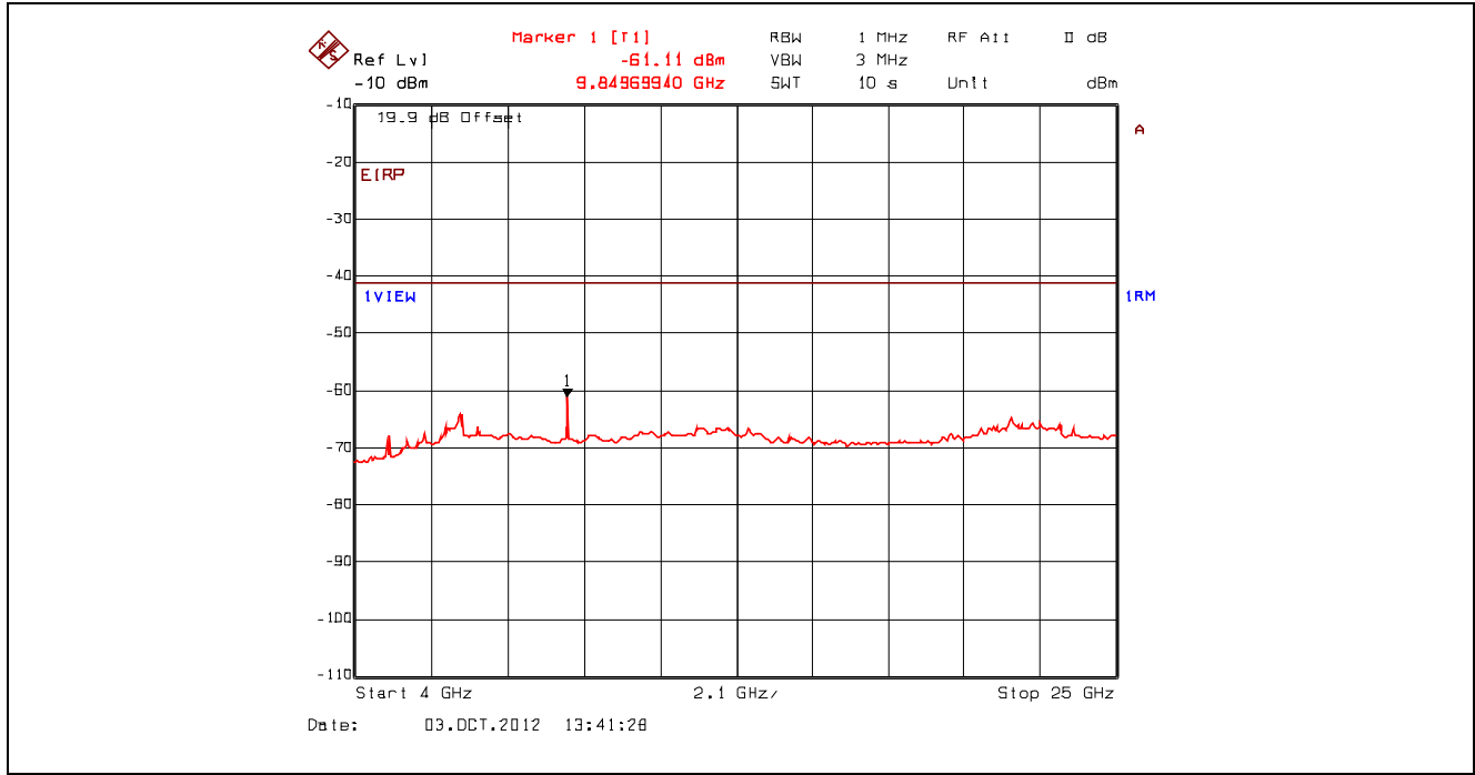
Plot 5.4.4.3.22. Conducted Spurious Emissions – Restricted Bands, 802.11b, 11 Mbps CCK 2462 MHz, 4 GHz - 25 GHz, Power Averaging with High Pass Filter
