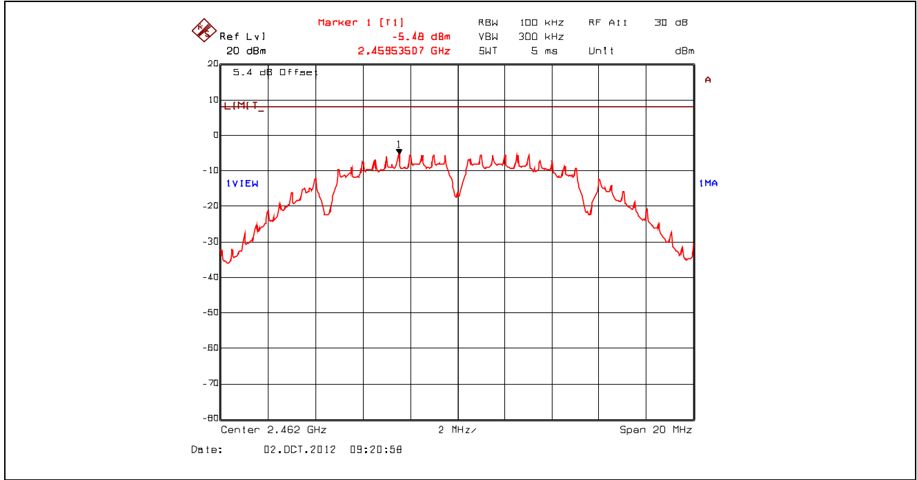
Plot 5.6.4.3. Power Spectral Density, 802.11b, 1 Mbps DBPSK, 2462 MHz, Setting 23 Offset: Insertion Loss + BWCF = 20.63 dB + 10 \cdot \log(3 \text{ kHz} / 100 \text{ kHz}) = 5.43 \text{ dB}
