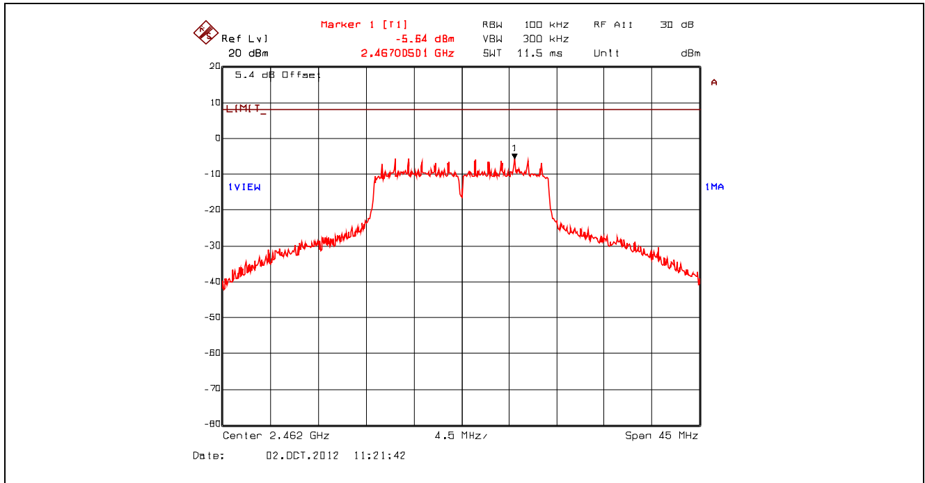
Plot 5.6.4.15. Power Spectral Density, 802.11g, 18 Mbps QPSK, 2462 MHz, Setting 23 Offset: Insertion Loss + BWCF = 20.63 dB + 10*log(3 kHz/ 100 kHz) = 5.43 dB
