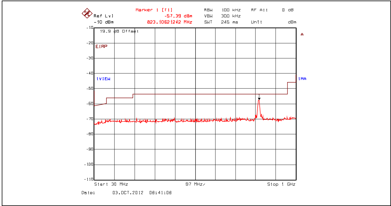
Plot 5.4.4.3.20. Conducted Spurious Emissions – Restricted Bands, 802.11b, 11 Mbps CCK 2462 MHz, 30 MHz - 1 GHz, Peak Detector with Band (Notch) Reject Filter
