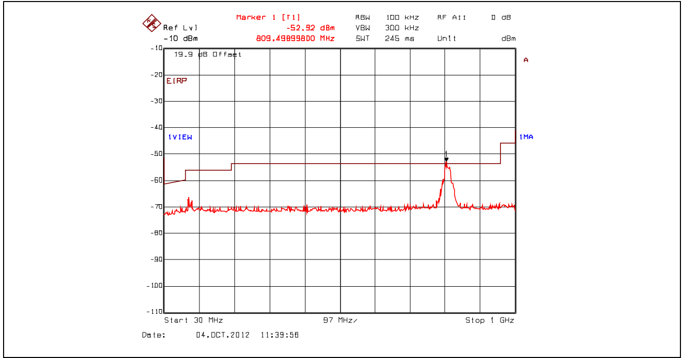
Plot 5.4.4.3.68. Conducted Spurious Emissions – Restricted Bands, 802.11n 800ns, 6.5 Mbps BPSK 1/2 2442 MHz, 30 MHz - 1 GHz, Peak Detector with Band (Notch) Reject Filter
