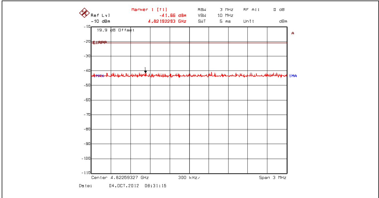
Plot 5.4.4.3.34. Conducted Spurious Emissions – Restricted Bands, 802.11g, 9 Mbps BPSK 2412 MHz, Peak Power at 4.82 GHz with High Pass Filter
