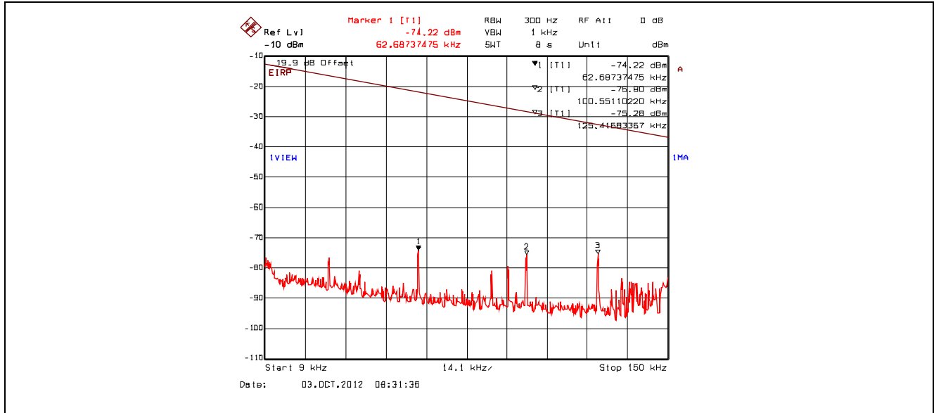
Plot 5.4.4.3.1. Conducted Spurious Emissions – Restricted Bands, 802.11b, 11 Mbps CCK 2412 MHz, 9 kHz - 150 kHz, Peak Detector with Band (Notch) Reject Filter
