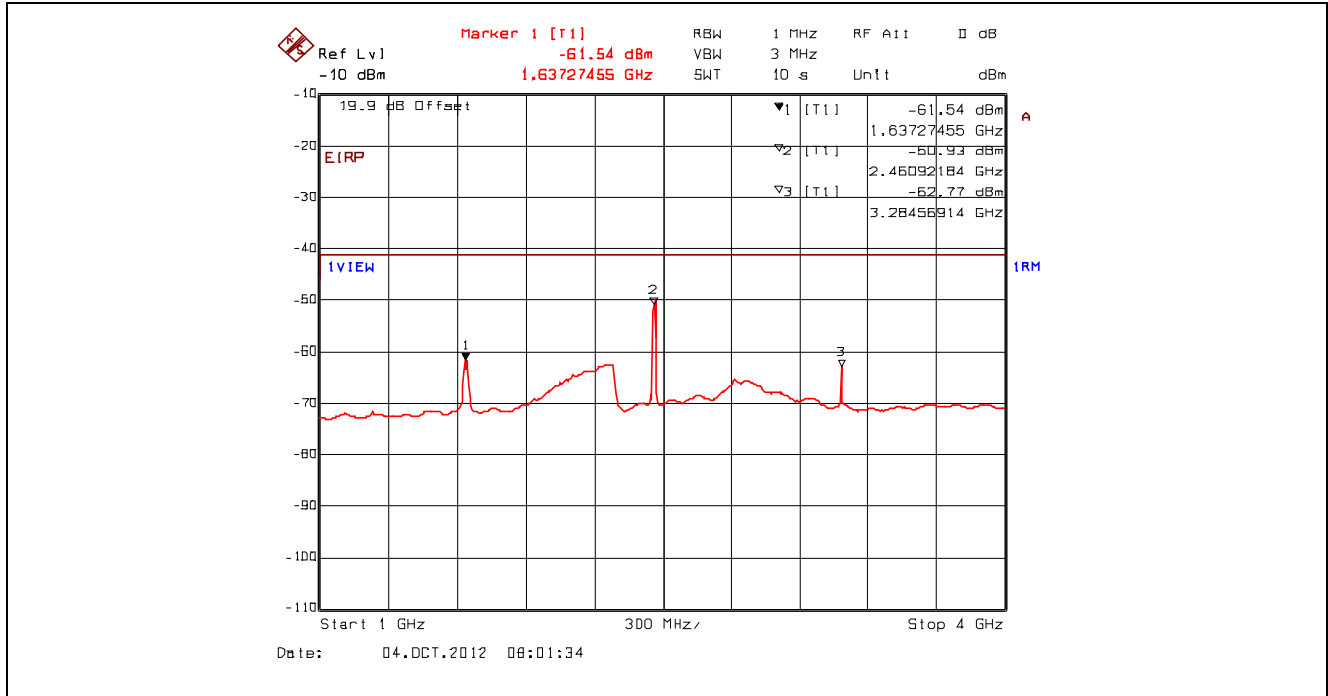
Plot 5.4.4.3.110. Conducted Spurious Emissions – Restricted Bands, 802.11n 400ns, 7.2 Mbps BPSK 1/2 2462 MHz, 1 GHz - 4 GHz, Power Averaging with Band (Notch) Reject Filter
