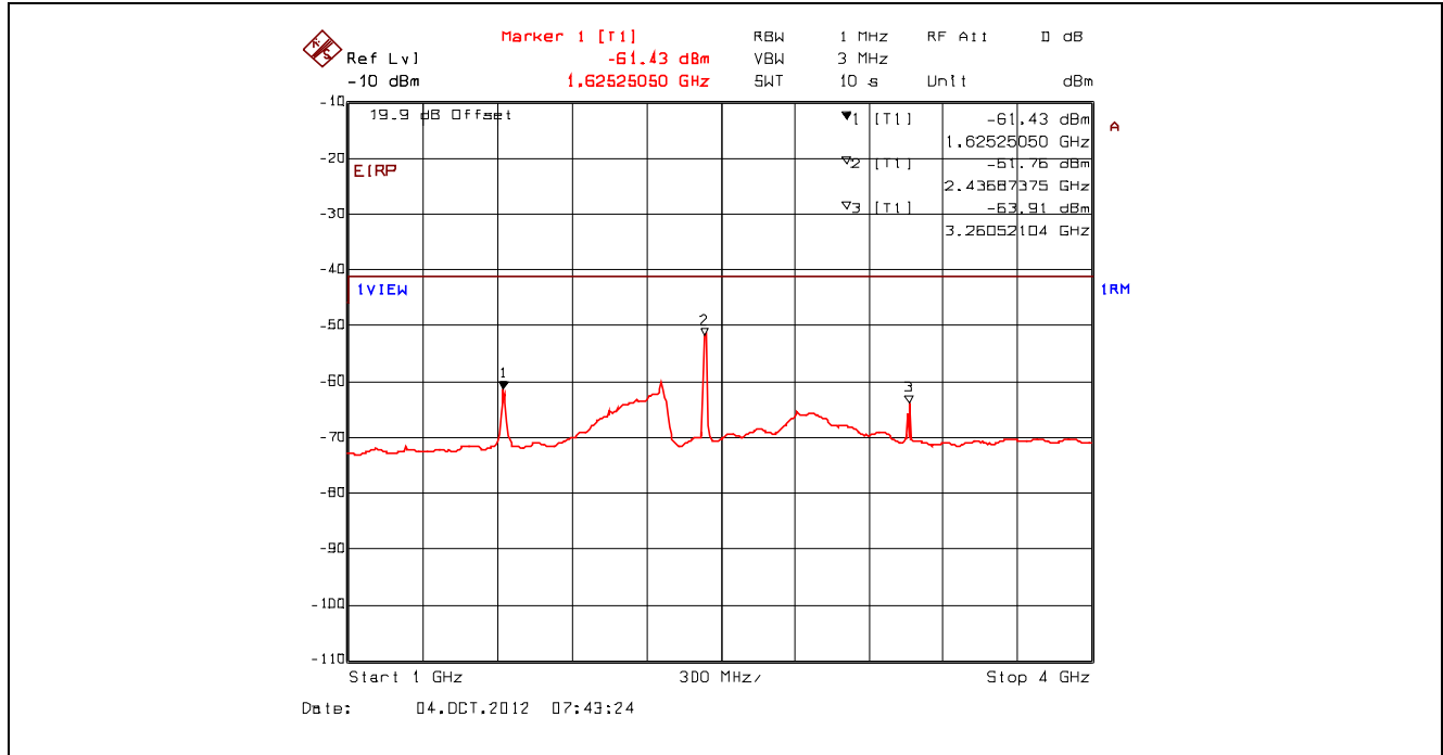
Plot 5.4.4.3.70. Conducted Spurious Emissions – Restricted Bands, 802.11n 800ns, 6.5 Mbps BPSK 1/2 2442 MHz, 1 GHz - 4 GHz, Power Averaging with Band (Notch) Reject Filter
