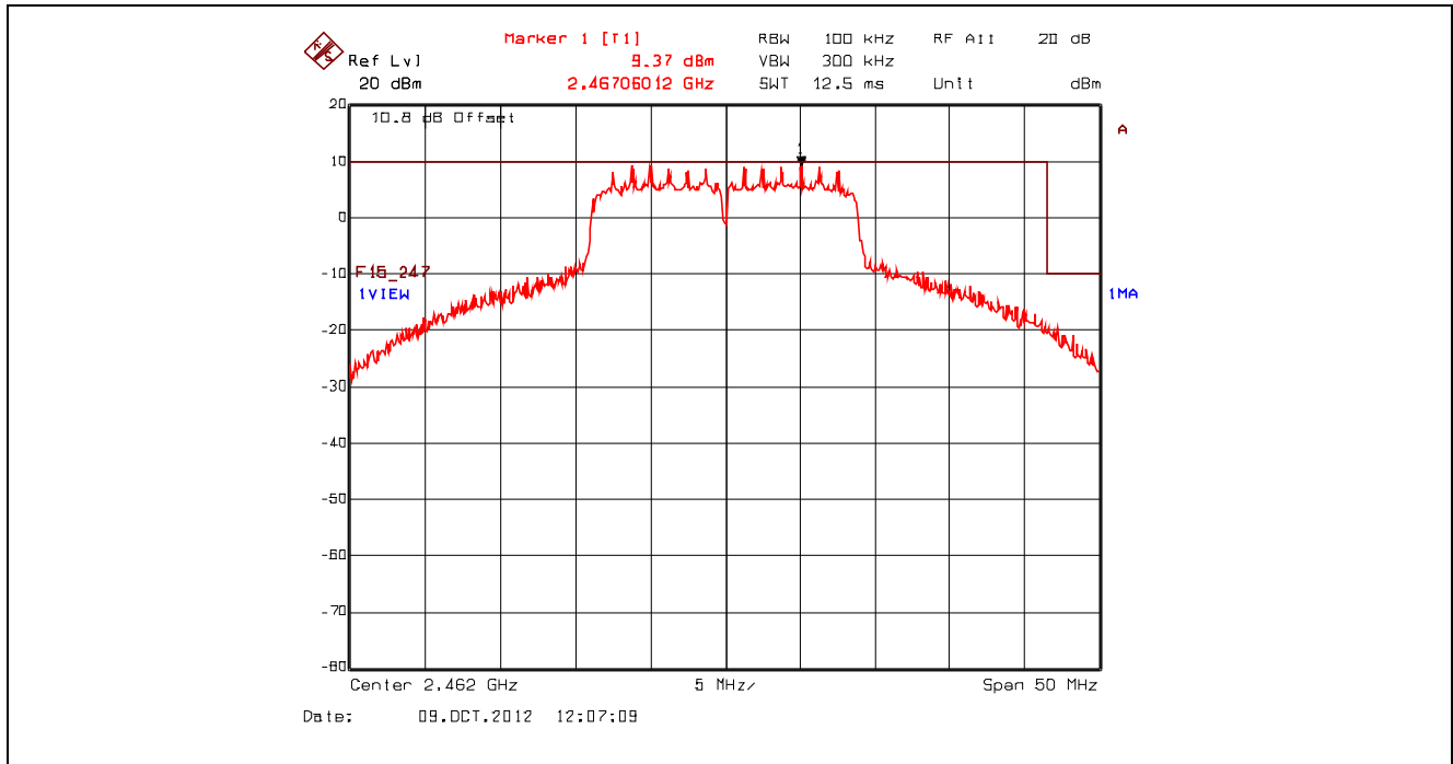
Plot 5.4.4.1.6. Band-Edge RF Conducted Emissions, Upper Band-edge, 2462 MHz, 802.11n 800ns, 6.5 Mbps BPSK 1/2
