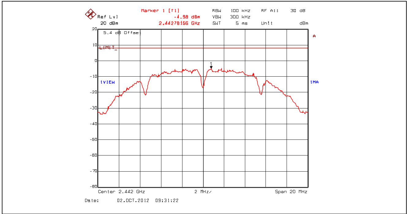
Plot 5.6.4.5. Power Spectral Density, 802.11b, 2 Mbps DQPSK, 2442 MHz, Setting 23 Offset: Insertion Loss + BWCF = 20.63 dB + 10*log(3 kHz/ 100 kHz) = 5.43 dB
