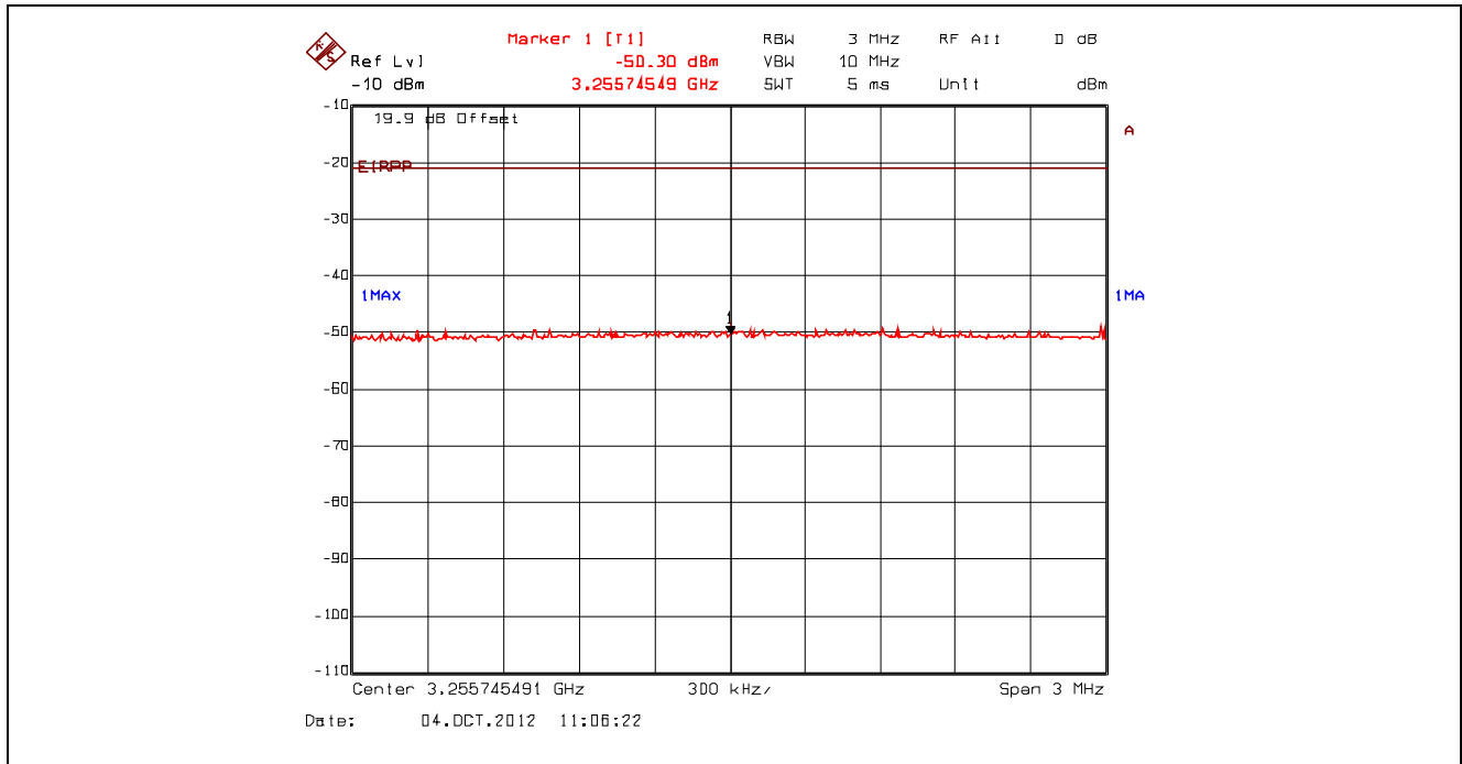
Plot 5.4.4.3.73. Conducted Spurious Emissions – Restricted Bands, 802.11n 800ns, 6.5 Mbps BPSK 1/2 2442 MHz, Peak Power at 3.26 GHz with Band (Notch) Reject Filter
