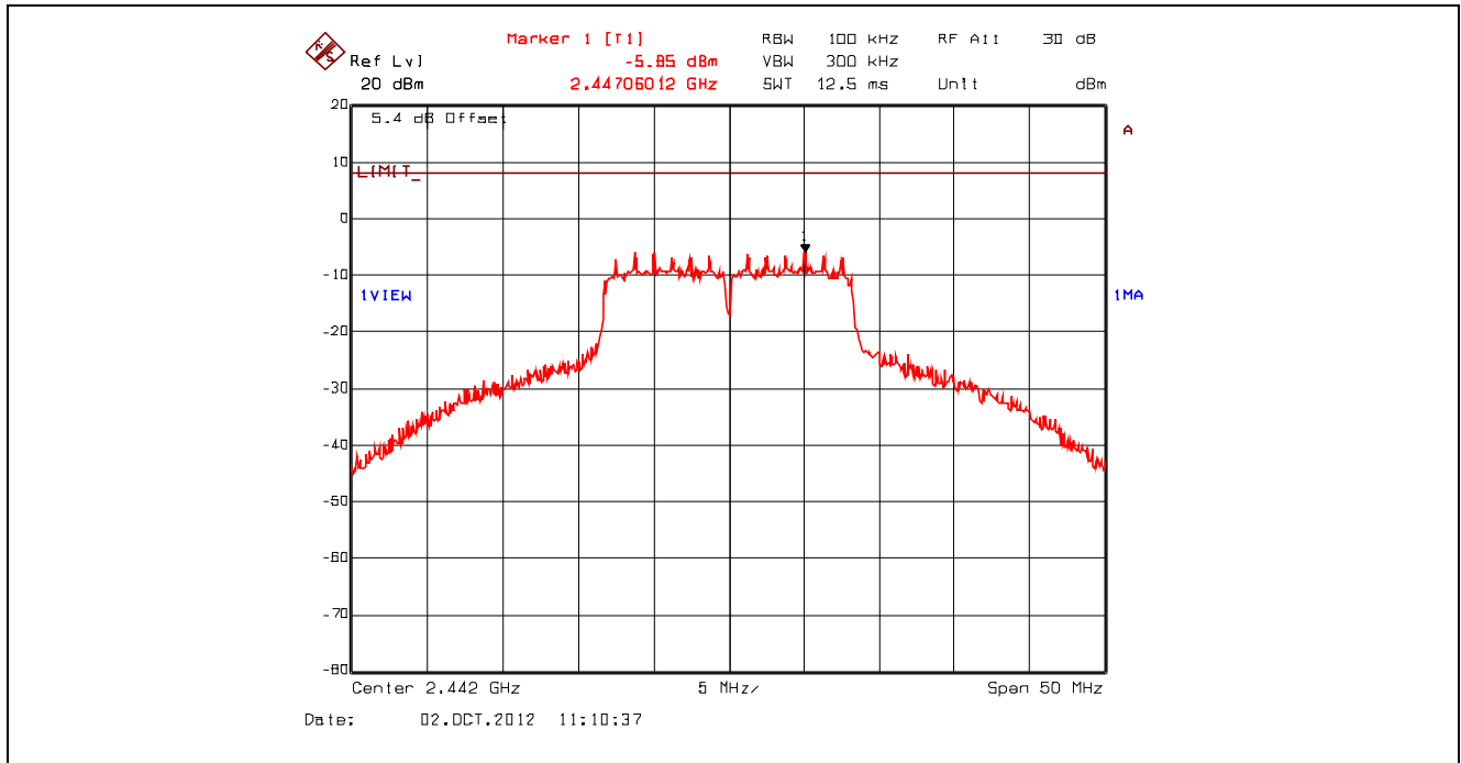
Plot 5.6.4.11. Power Spectral Density, 802.11g, 9 Mbps BPSK, 2442 MHz, Setting 23 Offset: Insertion Loss + BWCF = 20.63 dB + 10*log(3 kHz/ 100 kHz) = 5.43 dB
