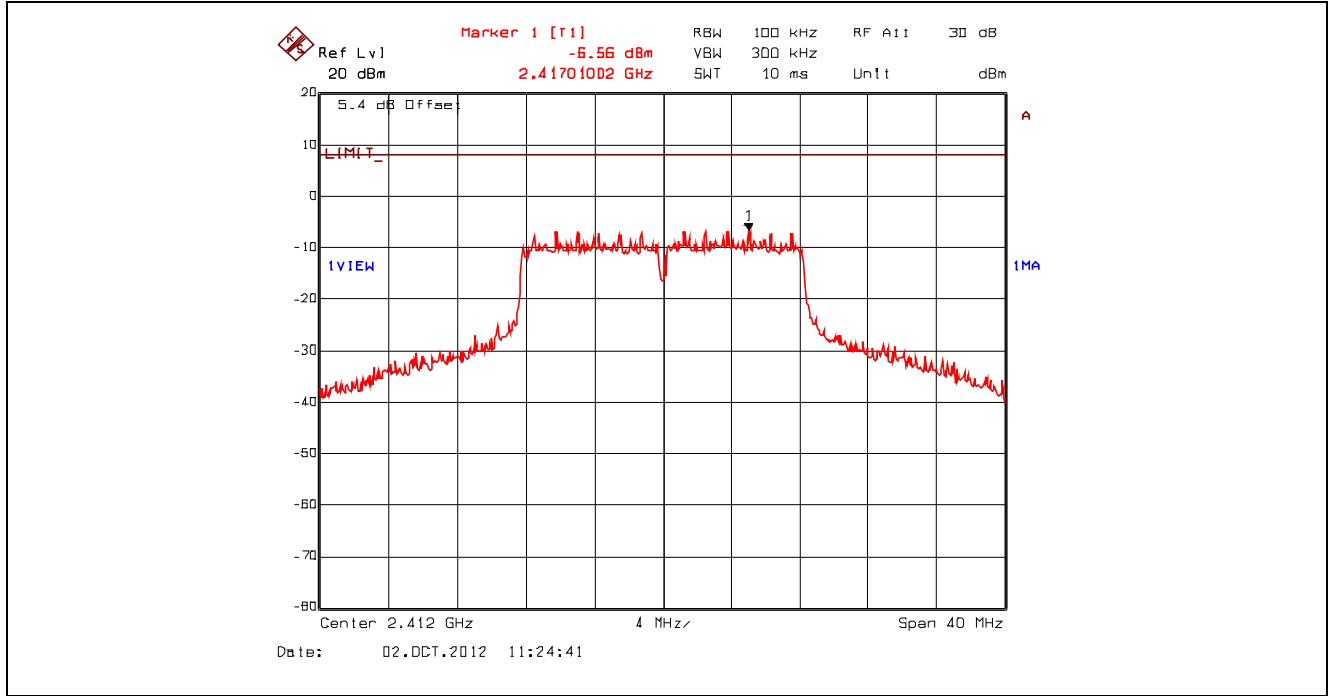
Plot 5.6.4.16. Power Spectral Density, 802.11g, 36 Mbps 16-QAM, 2412 MHz, Setting 23 Offset: Insertion Loss + BWCF = 20.63 dB + 10*log(3 kHz/ 100 kHz) = 5.43 dB
