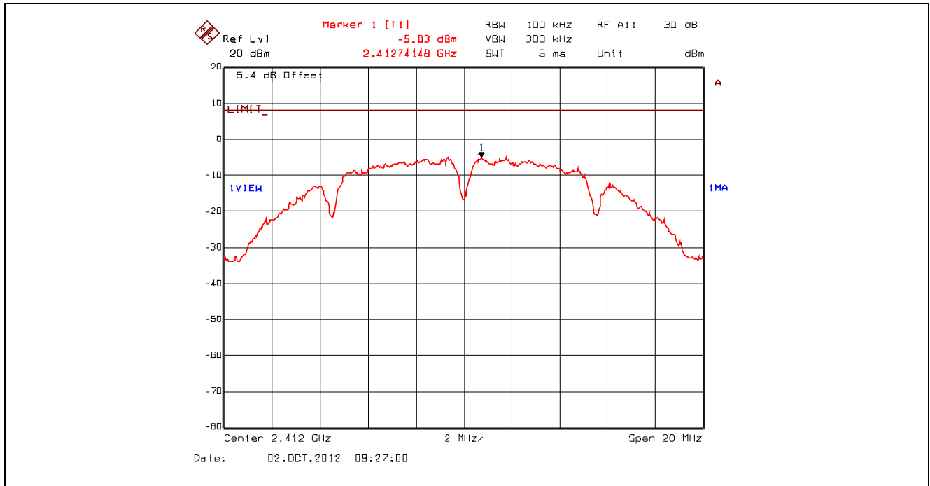
Plot 5.6.4.4. Power Spectral Density, 802.11b, 2 Mbps DQPSK, 2412 MHz, Setting 23 Offset: Insertion Loss + BWCF = 20.63 dB + 10 \cdot \log(3 \text{ kHz} / 100 \text{ kHz}) = 5.43 \text{ dB}
