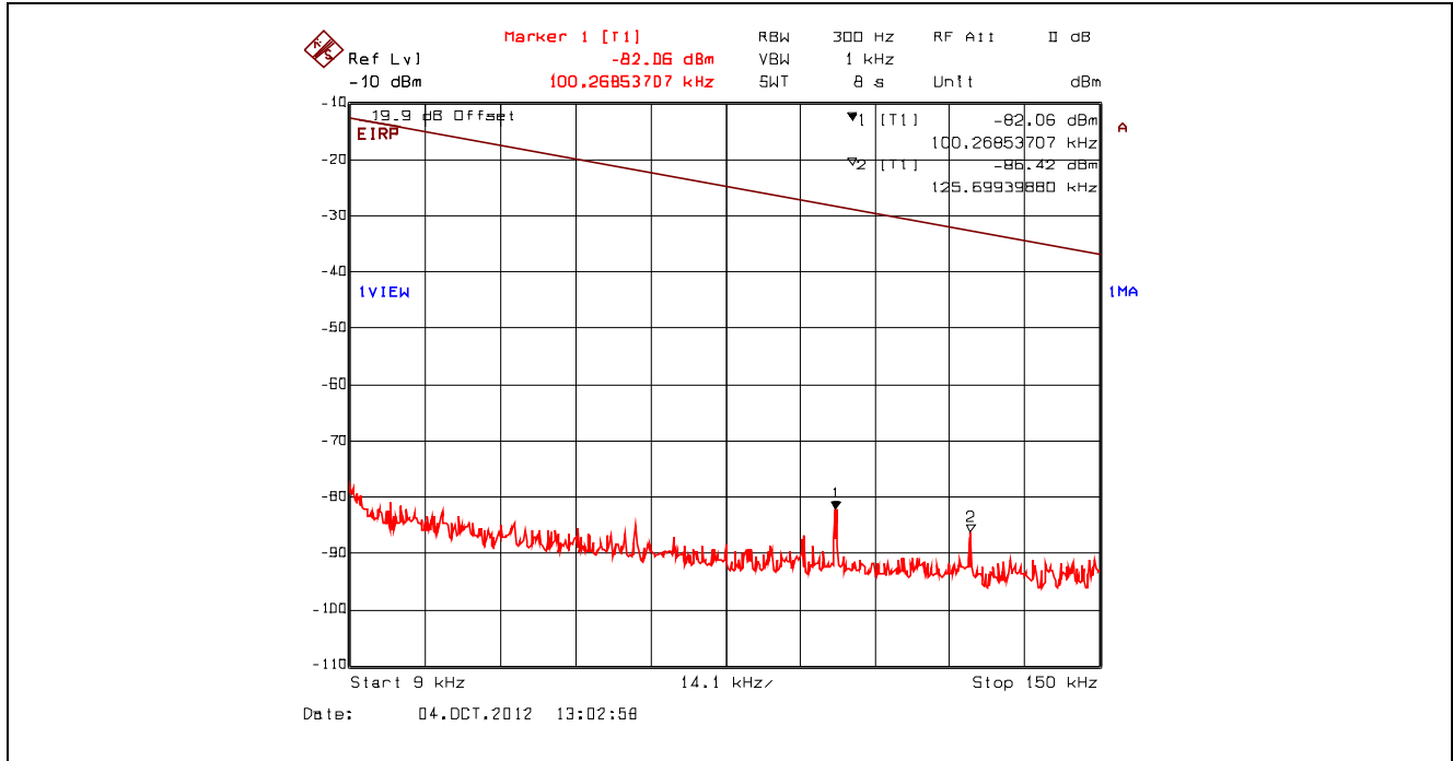
Plot 5.4.4.3.76. Conducted Spurious Emissions – Restricted Bands, 802.11n 800ns, 6.5 Mbps BPSK 1/2 2462 MHz, 9 kHz - 150 kHz, Peak Detector with Band (Notch) Reject Filter
