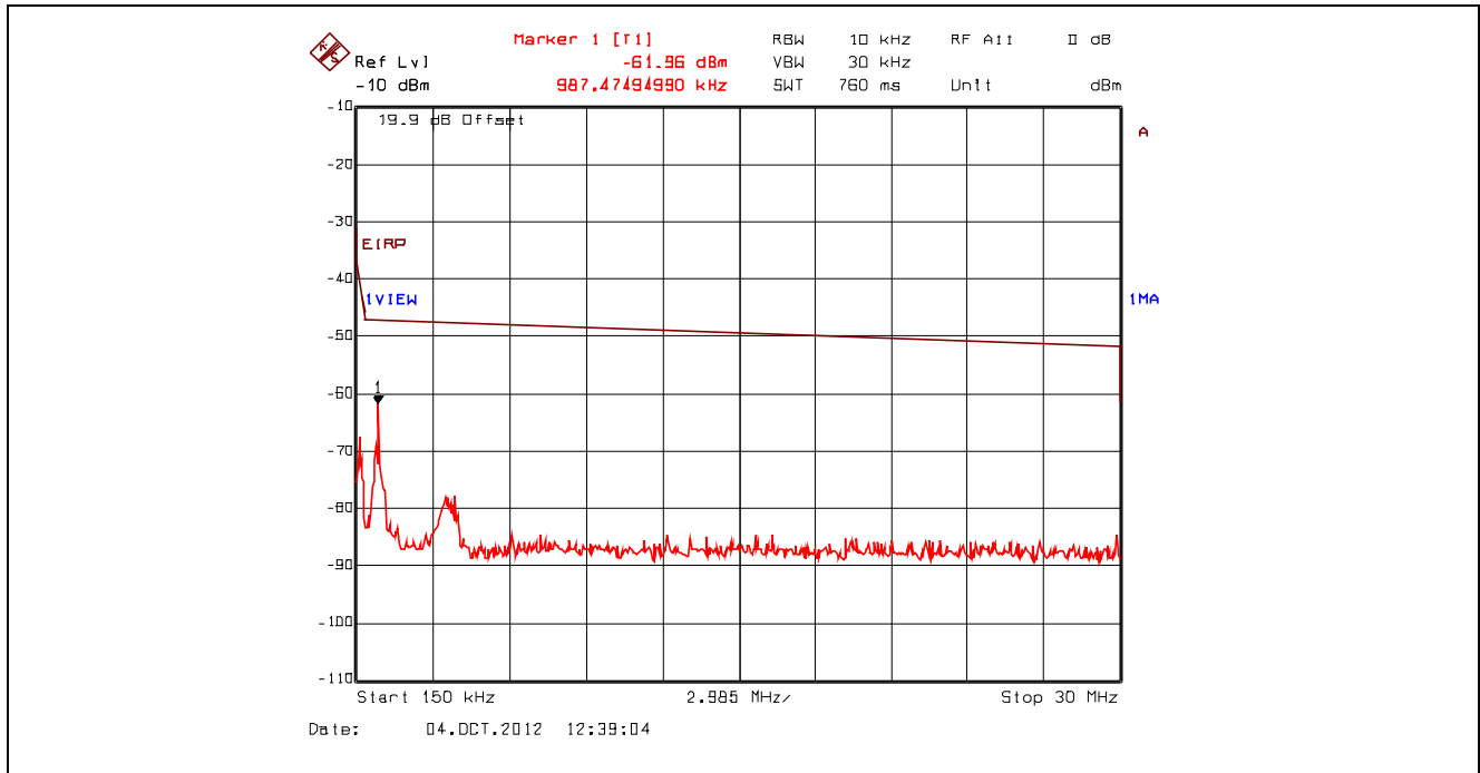
Plot 5.4.4.3.67. Conducted Spurious Emissions – Restricted Bands, 802.11n 800ns, 6.5 Mbps BPSK 1/2 2442 MHz, 150 kHz - 30 MHz, Peak Detector with Band (Notch) Reject Filter
