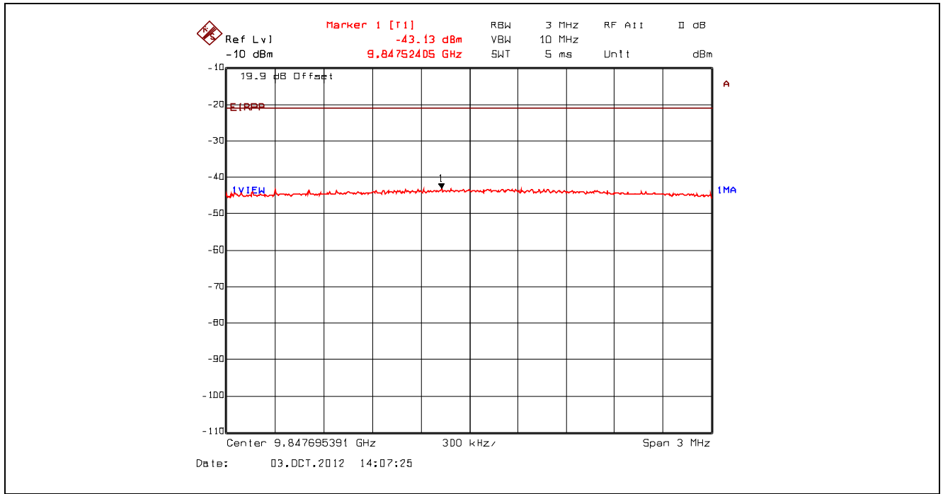
Plot 5.4.4.3.25. Conducted Spurious Emissions – Restricted Bands, 802.11b, 11 Mbps CCK 2462 MHz, Peak Power at 9.85 GHz with High Pass Filter
