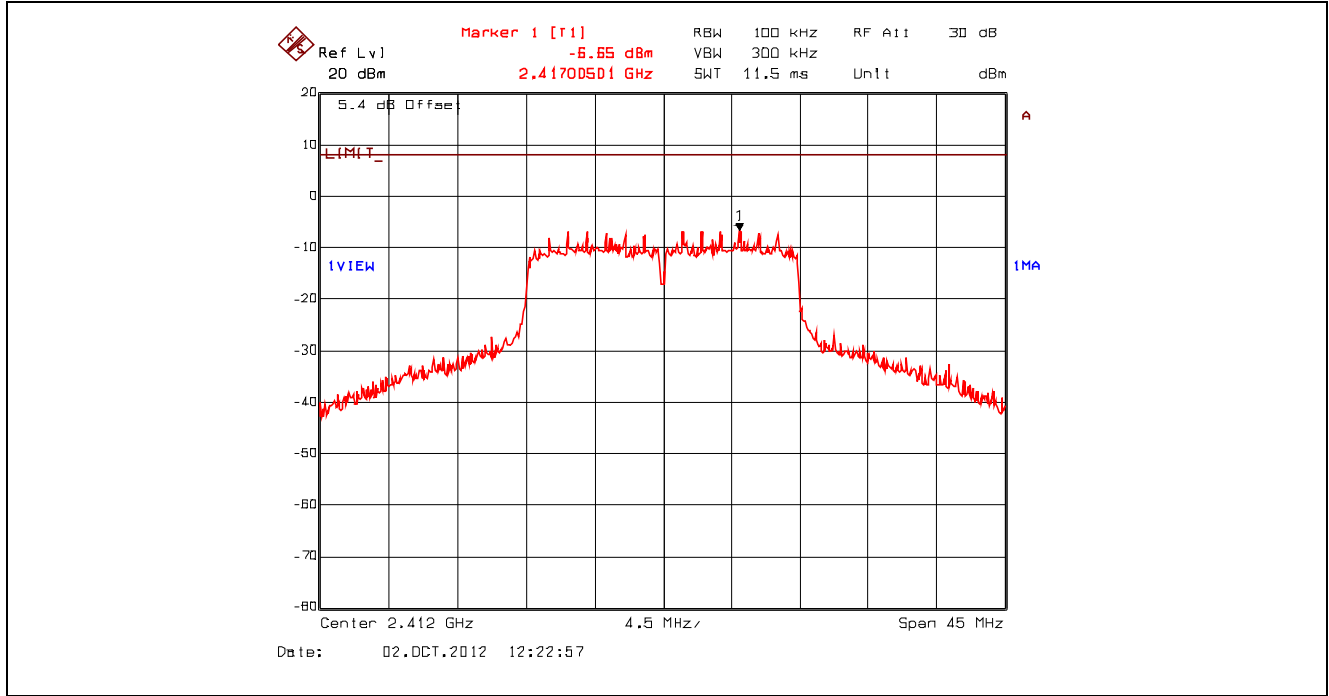
Plot 5.6.4.28. Power Spectral Density, 802.11n 800ns, 39 Mbps 16-QAM 3/4, 2412 MHz, Setting 23 Offset: Insertion Loss + BWCF = 20.63 dB + 10 \cdot \log(3 \text{ kHz} / 100 \text{ kHz}) = 5.43 \text{ dB}
