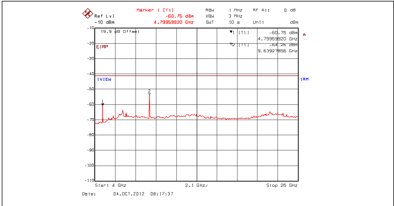
Plot 5.4.4.3.61. Conducted Spurious Emissions – Restricted Bands, 802.11n 800ns, 6.5 Mbps BPSK 1/2 2412 MHz, 4 GHz - 25 GHz, Power Averaging with High Pass Filter
