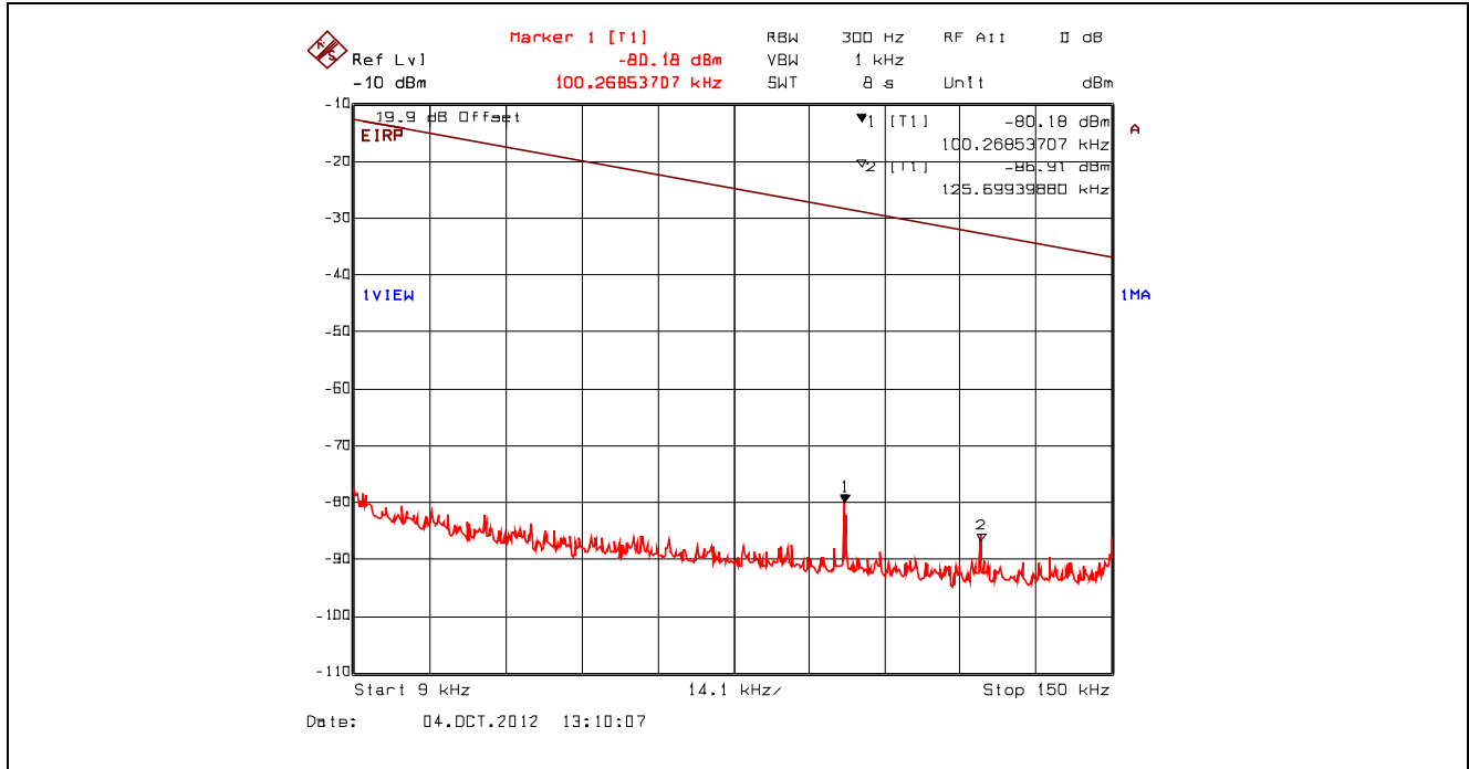
Plot 5.4.4.3.56. Conducted Spurious Emissions – Restricted Bands, 802.11n 800ns, 6.5 Mbps BPSK 1/2 2412 MHz, 9 kHz - 150 kHz, Peak Detector with Band (Notch) Reject Filter
