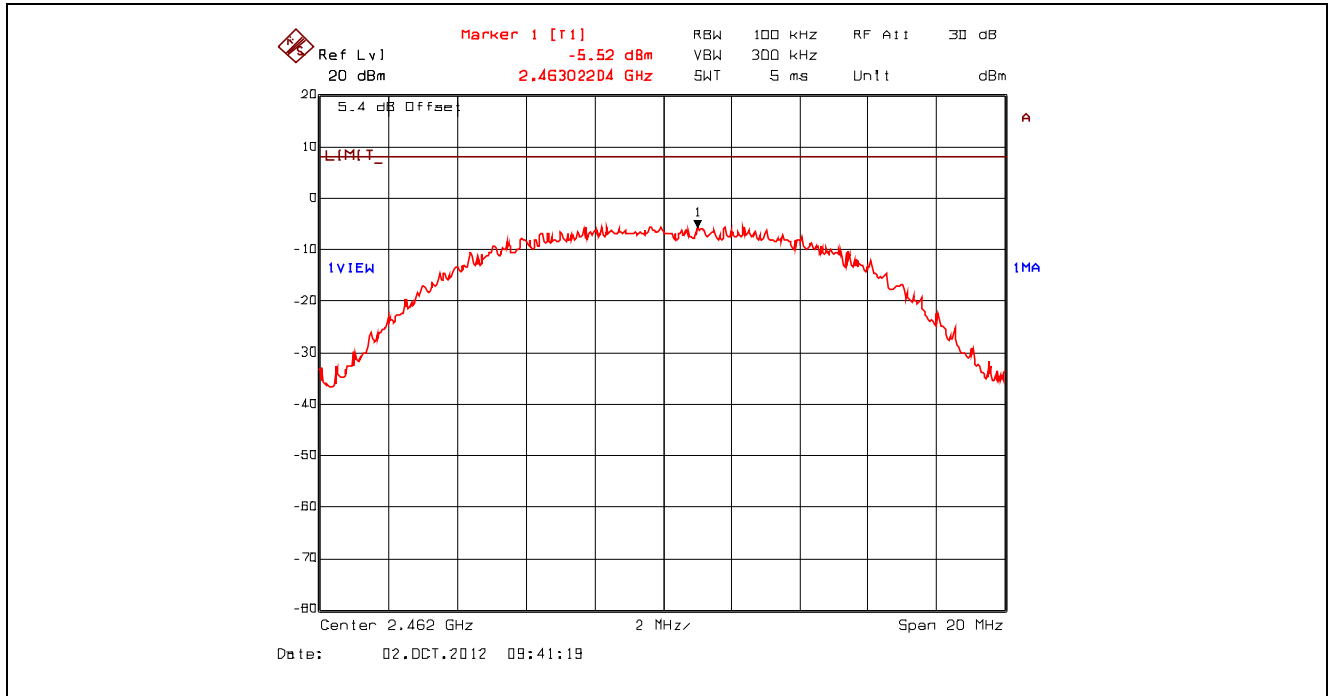
Plot 5.6.4.9. Power Spectral Density, 802.11b, 11 Mbps CCK, 2462 MHz, Setting 23 Offset: Insertion Loss + BWCF = 20.63 dB + 10*log(3 kHz/ 100 kHz) = 5.43 dB
