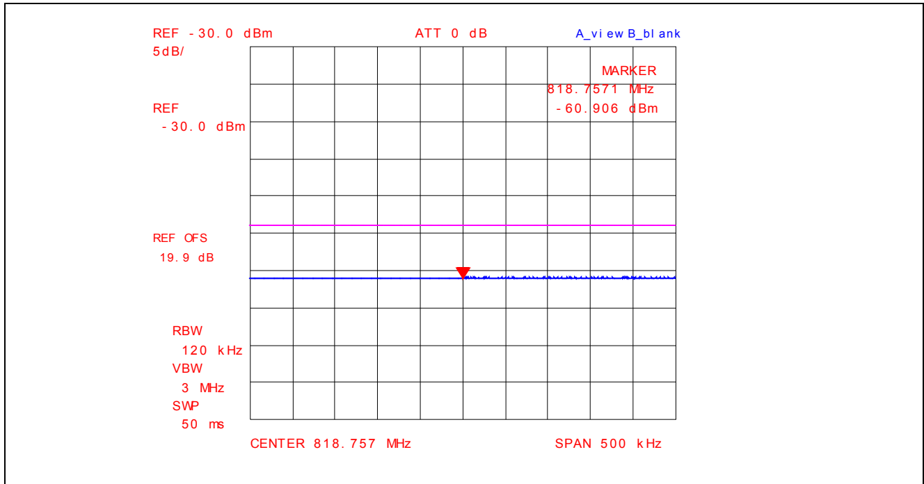
Plot 5.4.4.3.49. Conducted Spurious Emissions – Restricted Bands, 802.11g, 9 Mbps BPSK 2462 MHz, QP Power at 818.76 MHz with Band (Notch) Reject Filter
