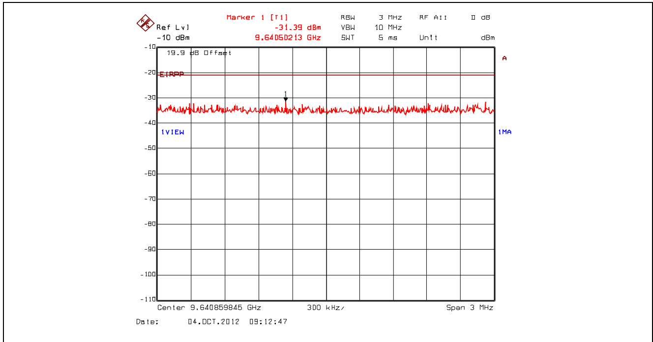
Plot 5.4.4.3.95. Conducted Spurious Emissions – Restricted Bands, 802.11n 400ns, 7.2 Mbps BPSK 1/2 2412 MHz, Peak Power at 9.64 GHz with High Pass Filter
