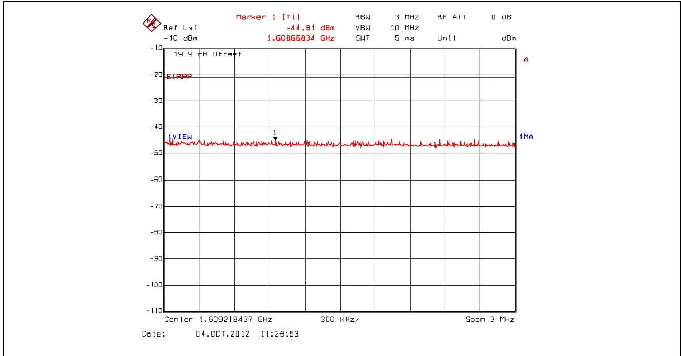
Plot 5.4.4.3.32. Conducted Spurious Emissions – Restricted Bands, 802.11g, 9 Mbps BPSK 2412 MHz, Peak Power at 1.61 GHz with Band (Notch) Reject Filter
