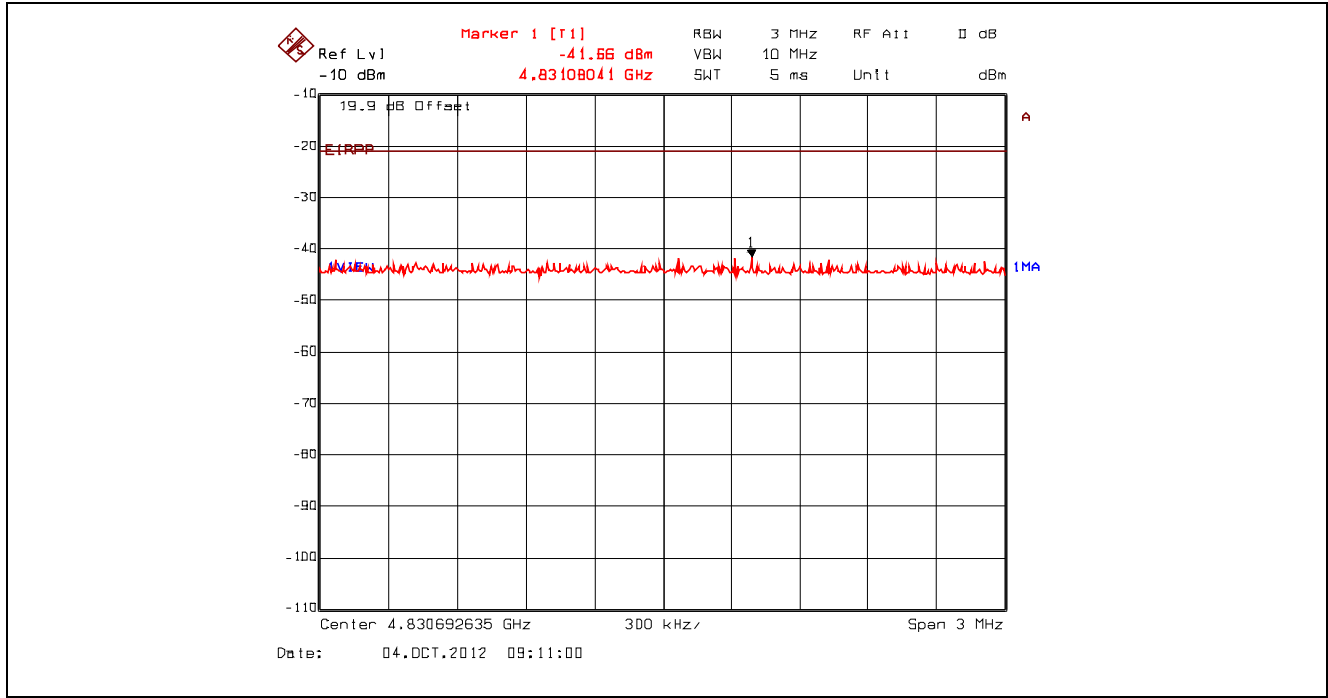
Plot 5.4.4.3.94. Conducted Spurious Emissions – Restricted Bands, 802.11n 400ns, 7.2 Mbps BPSK 1/2 2412 MHz, Peak Power at 4.83 GHz with High Pass Filter
