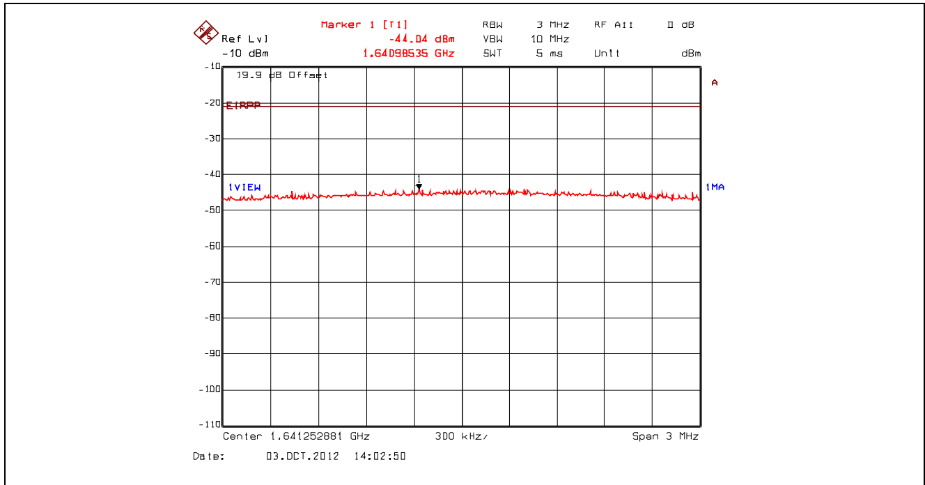
Plot 5.4.4.3.23. Conducted Spurious Emissions – Restricted Bands, 802.11b, 11 Mbps CCK 2462 MHz, Peak Power at 1.64 GHz with Band (Notch) Reject Filter
