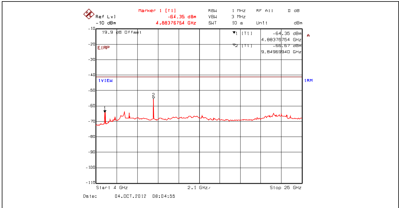
Plot 5.4.4.3.111. Conducted Spurious Emissions – Restricted Bands, 802.11n 400ns, 7.2 Mbps BPSK 1/2 2462 MHz, 4 GHz - 25 GHz, Power Averaging with High Pass Filter
