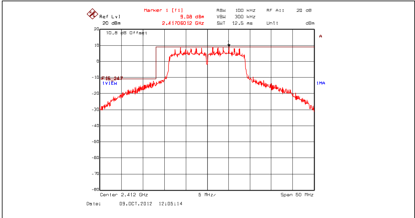
Plot 5.4.4.1.5. Band-Edge RF Conducted Emissions, Lower Band-edge, 2412 MHz, 802.11n 800ns, 6.5 Mbps BPSK 1/2
