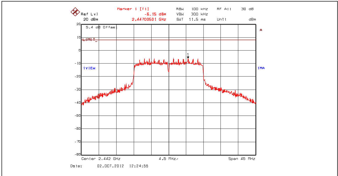
Plot 5.6.4.29. Power Spectral Density, 802.11n 800ns, 39 Mbps 16-QAM 3/4, 2442 MHz, Setting 23 Offset: Insertion Loss + BWCF = 20.63 dB + 10 \cdot \log(3 \text{ kHz} / 100 \text{ kHz}) = 5.43 \text{ dB}
