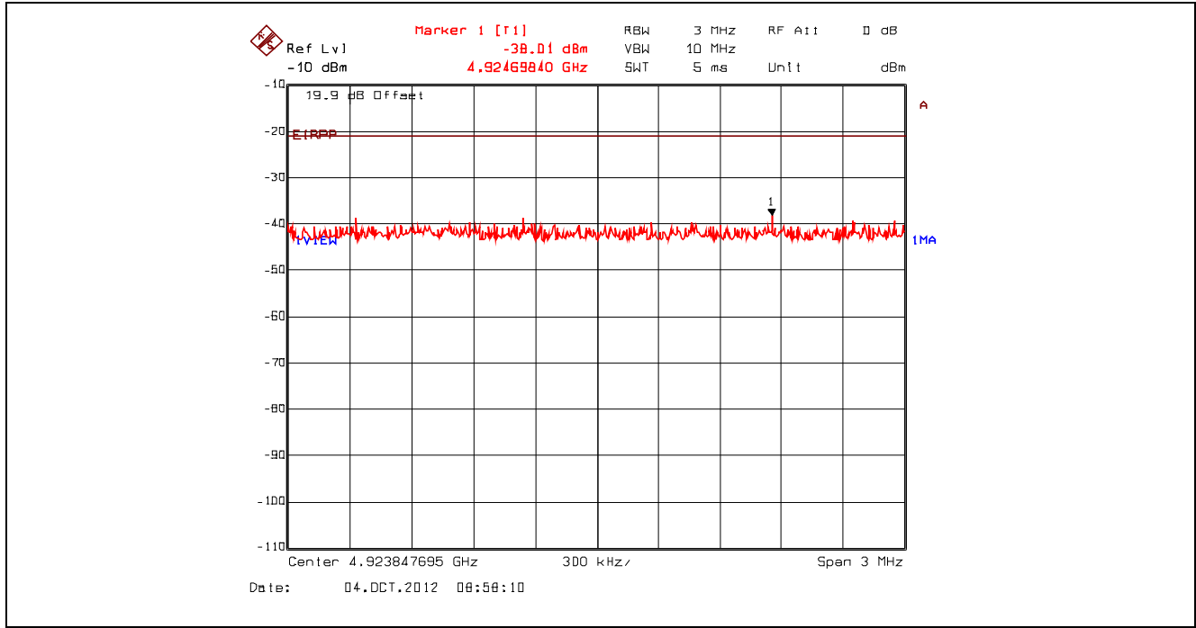
Plot 5.4.4.3.84. Conducted Spurious Emissions – Restricted Bands, 802.11n 800ns, 6.5 Mbps BPSK 1/2 2462 MHz, Peak Power at 4.92 GHz with High Pass Filter
