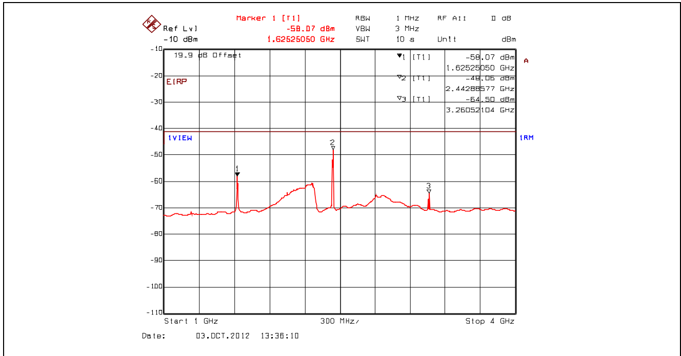
Plot 5.4.4.3.13. Conducted Spurious Emissions – Restricted Bands, 802.11b, 11 Mbps CCK 2442 MHz, 1 GHz - 4 GHz, Power Averaging with Band (Notch) Reject Filter
