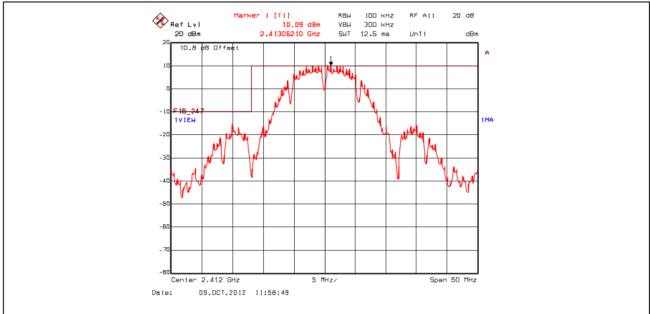
Plot 5.4.4.1.1. Band-Edge RF Conducted Emissions, Lower Band-edge, 2412 MHz, 802.11b, 1 Mbps DBPSK
