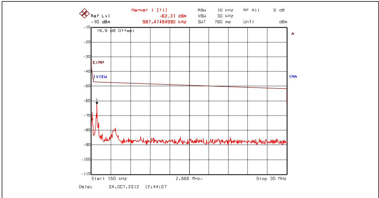
Plot 5.4.4.3.87. Conducted Spurious Emissions – Restricted Bands, 802.11n 400ns, 7.2 Mbps BPSK 1/2 2412 MHz, 150 kHz - 30 MHz, Peak Detector with Band (Notch) Reject Filter
