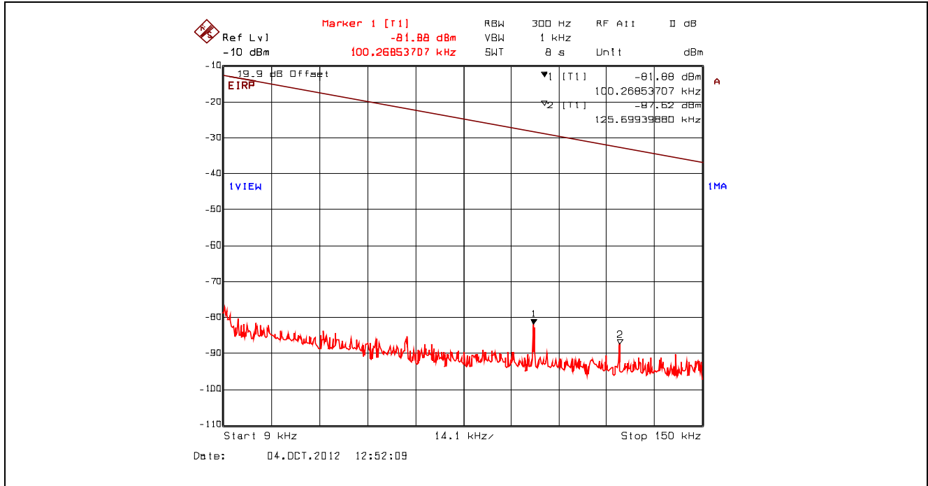
Plot 5.4.4.3.106. Conducted Spurious Emissions – Restricted Bands, 802.11n 400ns, 7.2 Mbps BPSK 1/2 2462 MHz, 9 kHz - 150 kHz, Peak Detector with Band (Notch) Reject Filter
