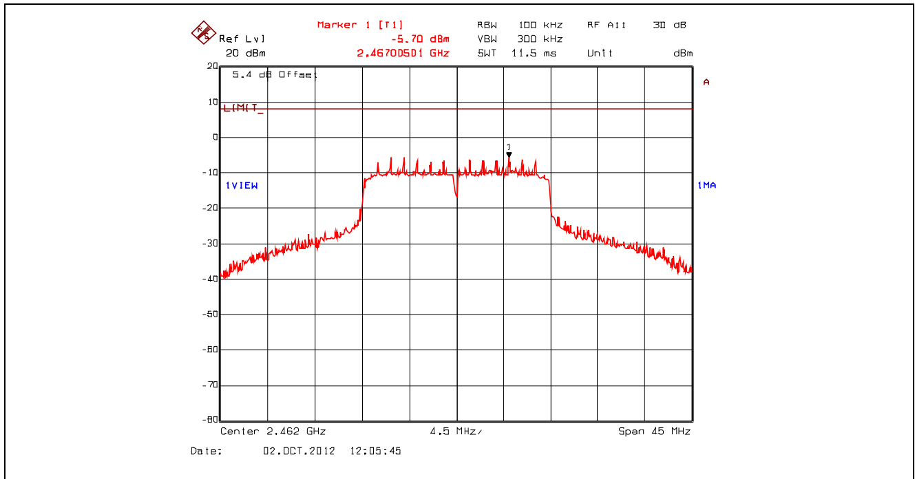
Plot 5.6.4.27. Power Spectral Density, 802.11n 800ns, 19.5 Mbps QPSK 3/4, 2462 MHz, Setting 23 Offset: Insertion Loss + BWCF = 20.63 dB + 10*log(3 kHz/ 100 kHz) = 5.43 dB
