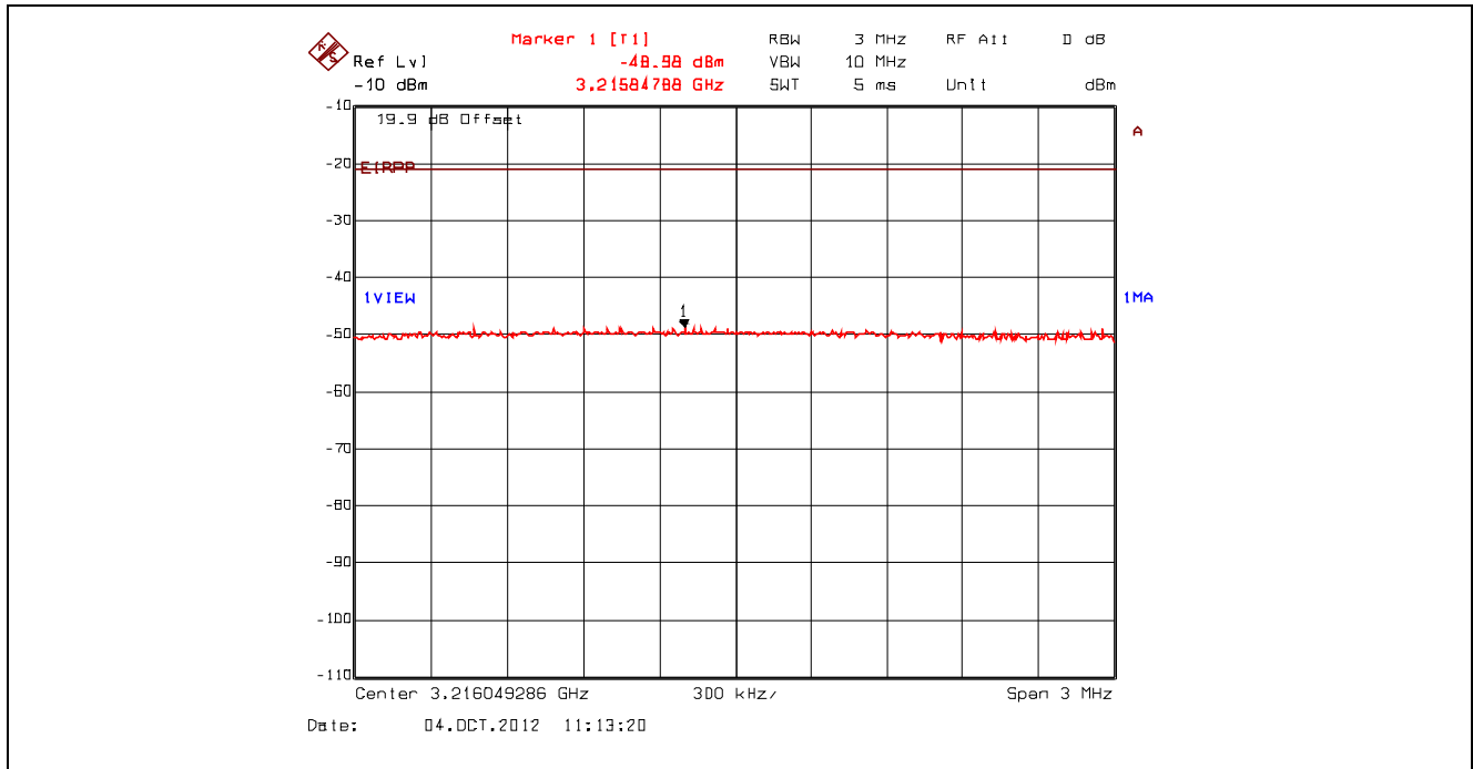
Plot 5.4.4.3.63. Conducted Spurious Emissions – Restricted Bands, 802.11n 800ns, 6.5 Mbps BPSK 1/2 2412 MHz, Peak Power at 3.22 GHz with Band (Notch) Reject Filter
