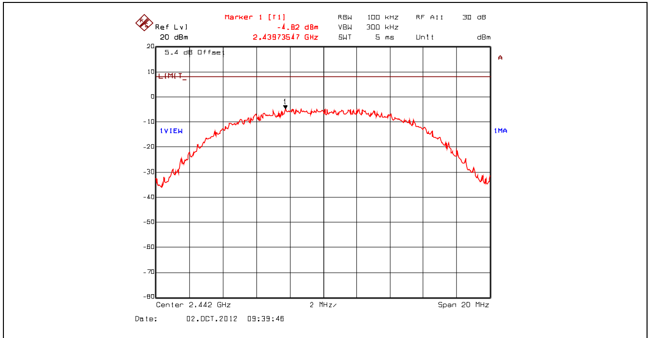
Plot 5.6.4.8. Power Spectral Density, 802.11b, 11 Mbps CCK, 2442 MHz, Setting 23 Offset: Insertion Loss + BWCF = 20.63 dB + 10 \cdot \log(3 \text{ kHz} / 100 \text{ kHz}) = 5.43 \text{ dB}
