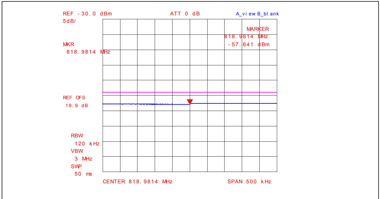
Plot 5.4.4.3.39. Conducted Spurious Emissions – Restricted Bands, 802.11g, 9 Mbps BPSK 2442 MHz, QP Power at 818.98 MHz with Band (Notch) Reject Filter
