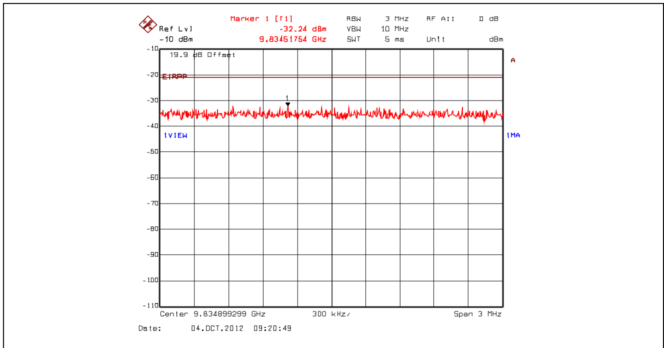
Plot 5.4.4.3.115. Conducted Spurious Emissions – Restricted Bands, 802.11n 400ns, 7.2 Mbps BPSK 1/2 2462 MHz, Peak Power at 9.83 GHz with High Pass Filter
