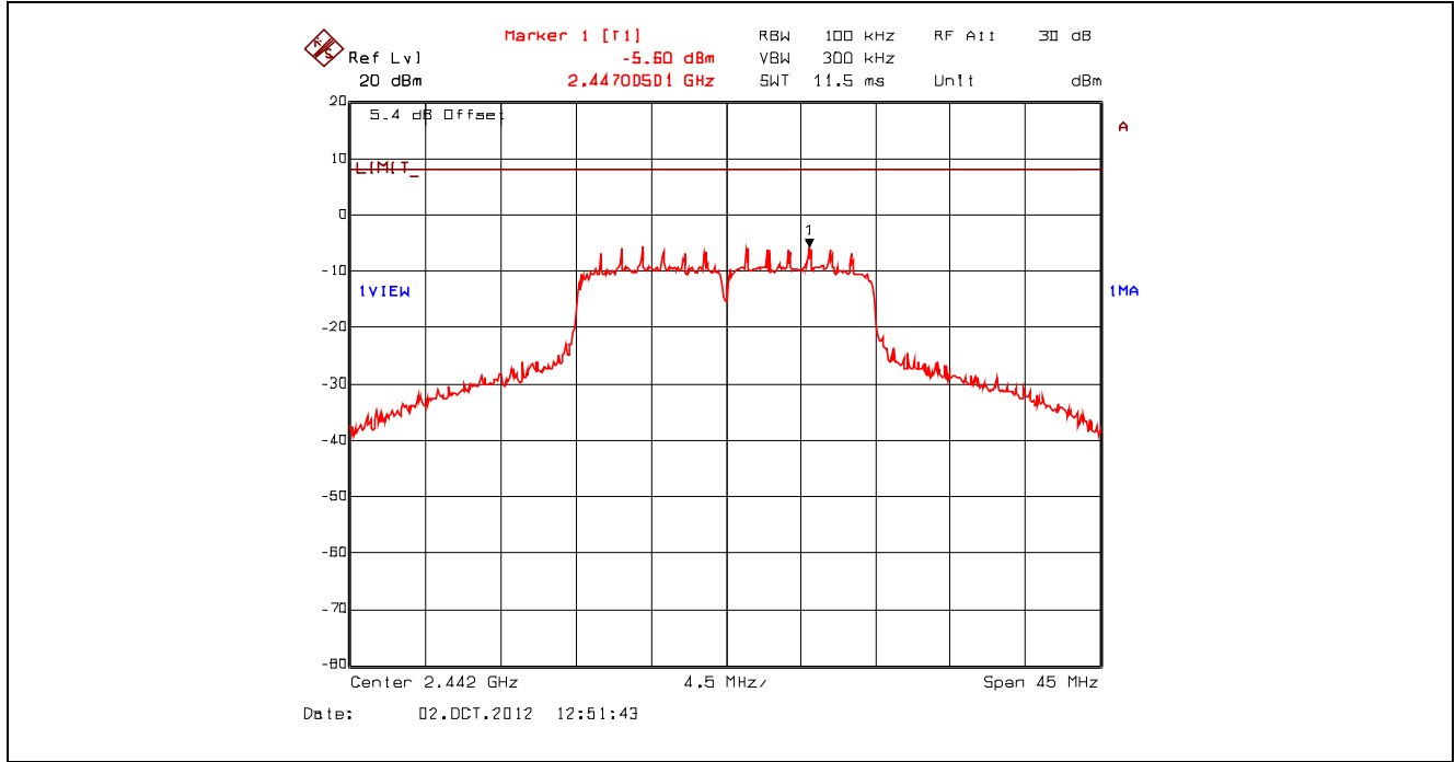
Plot 5.6.4.38. Power Spectral Density, 802.11n 400ns, 21.7 Mbps QPSK 3/4, 2442 MHz, Setting 23 Offset: Insertion Loss + BWCF = 20.63 dB + 10 \cdot \log(3 \text{ kHz} / 100 \text{ kHz}) = 5.43 \text{ dB}
