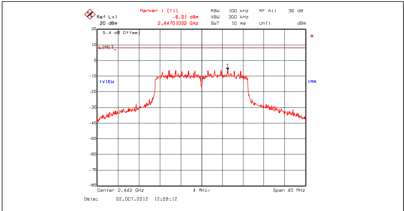
Plot 5.6.4.41. Power Spectral Density, 802.11n 400ns, 43.3 Mbps 16-QAM 3/4, 2442 MHz, Setting 23 Offset: Insertion Loss + BWCF = 20.63 dB + 10*log(3 kHz/ 100 kHz) = 5.43 dB
