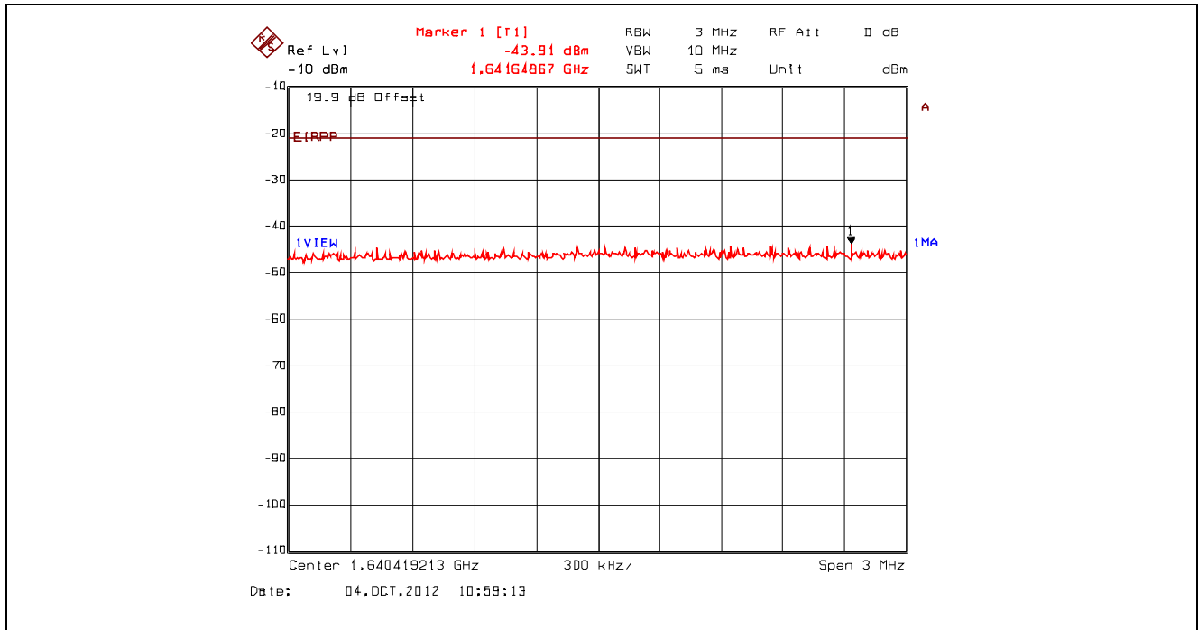
Plot 5.4.4.3.82. Conducted Spurious Emissions – Restricted Bands, 802.11n 800ns, 6.5 Mbps BPSK 1/2 2462 MHz, Peak Power at 1.64 GHz with Band (Notch) Reject Filter
