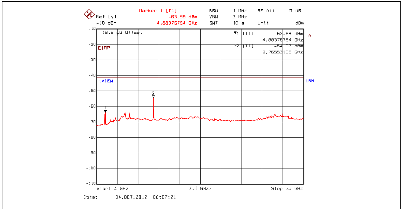
Plot 5.4.4.3.101. Conducted Spurious Emissions – Restricted Bands, 802.11n 400ns, 7.2 Mbps BPSK 1/2 2442 MHz, 4 GHz - 25 GHz, Power Averaging with High Pass Filter
