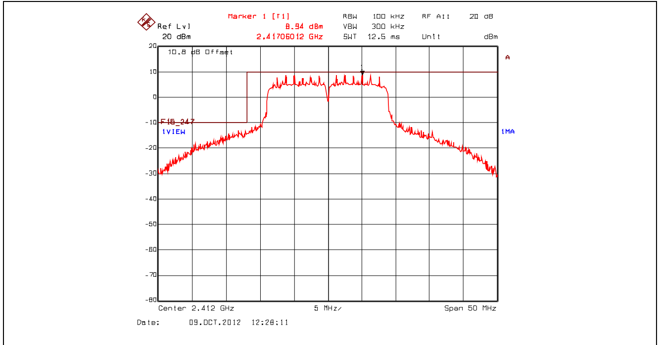
Plot 5.4.4.1.7. Band-Edge RF Conducted Emissions, Lower Band-edge, 2412 MHz, 802.11n 400ns, 7.2 Mbps BPSK 1/2
