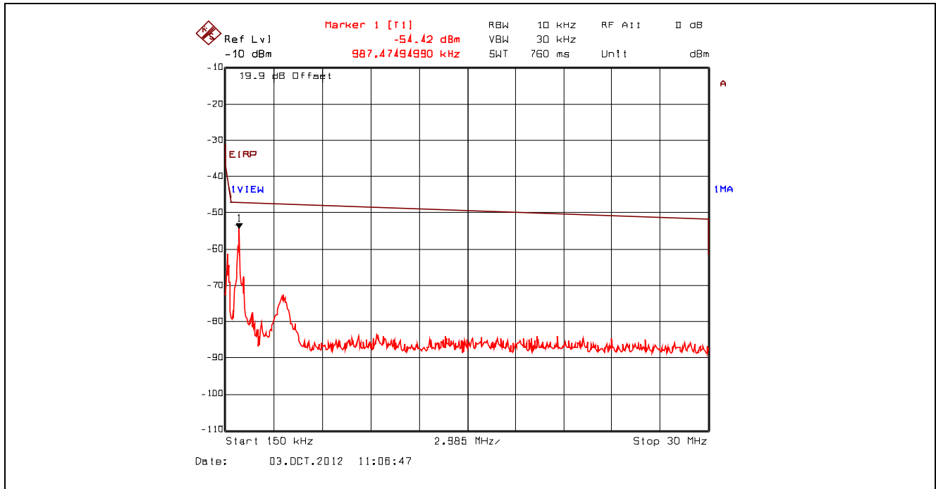
Plot 5.4.4.3.47. Conducted Spurious Emissions – Restricted Bands, 802.11g, 9 Mbps BPSK 2462 MHz, 150 kHz - 30 MHz, Peak Detector with Band (Notch) Reject Filter
