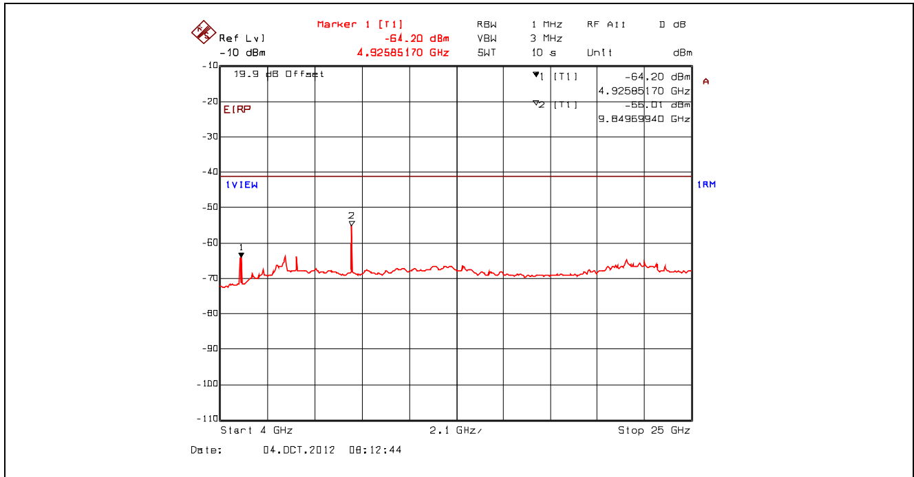
Plot 5.4.4.3.81. Conducted Spurious Emissions – Restricted Bands, 802.11n 800ns, 6.5 Mbps BPSK 1/2 2462 MHz, 4 GHz - 25 GHz, Power Averaging with High Pass Filter
