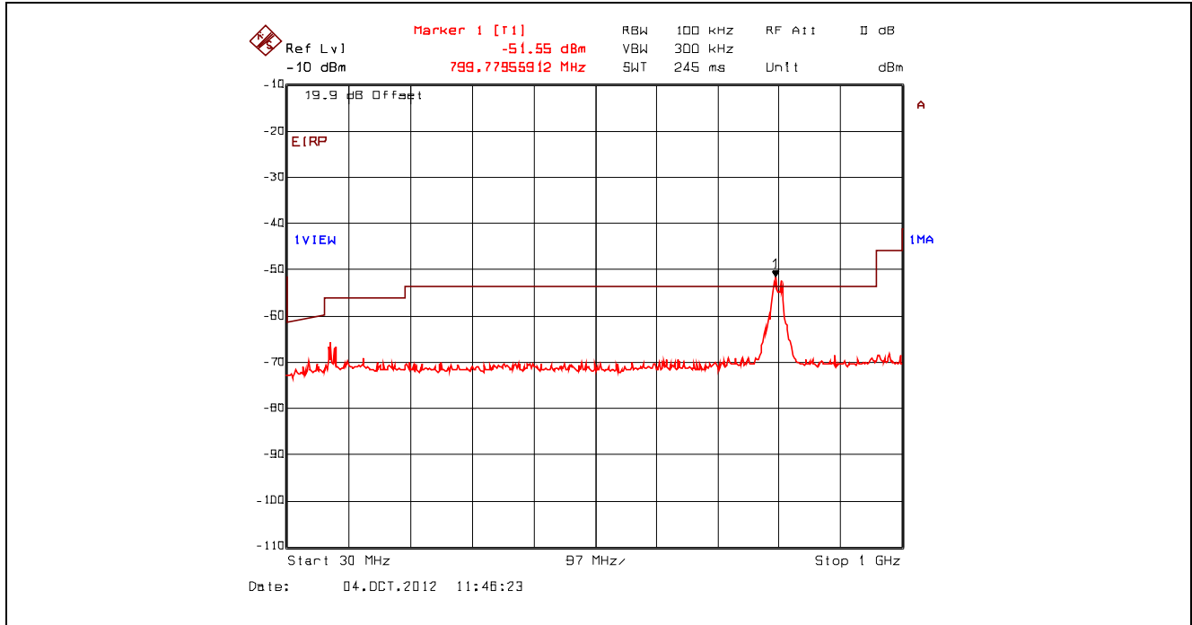
Plot 5.4.4.3.88. Conducted Spurious Emissions – Restricted Bands, 802.11n 400ns, 7.2 Mbps BPSK 1/2 2412 MHz, 30 MHz - 1 GHz, Peak Detector with Band (Notch) Reject Filter
