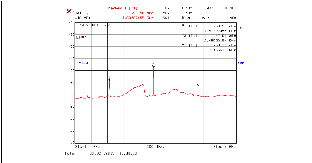
Plot 5.4.4.3.21. Conducted Spurious Emissions – Restricted Bands, 802.11b, 11 Mbps CCK 2462 MHz, 1 GHz - 4 GHz, Power Averaging with Band (Notch) Reject Filter
