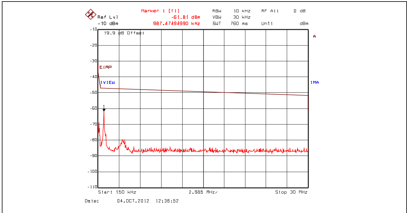
Plot 5.4.4.3.57. Conducted Spurious Emissions – Restricted Bands, 802.11n 800ns, 6.5 Mbps BPSK 1/2 2412 MHz, 150 kHz - 30 MHz, Peak Detector with Band (Notch) Reject Filter
