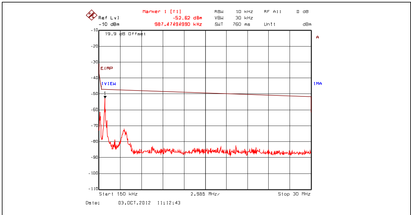
Plot 5.4.4.3.27. Conducted Spurious Emissions – Restricted Bands, 802.11g, 9 Mbps BPSK 2412 MHz, 150 kHz - 30 MHz, Peak Detector with Band (Notch) Reject Filter
