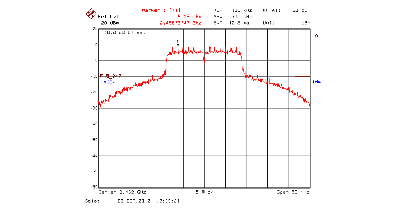
Plot 5.4.4.1.8. Band-Edge RF Conducted Emissions, Upper Band-edge, 2462 MHz, 802.11n 400ns, 7.2 Mbps BPSK 1/2
