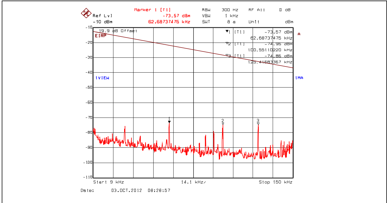
Plot 5.4.4.3.10. Conducted Spurious Emissions – Restricted Bands, 802.11b, 11 Mbps CCK 2442 MHz, 9 kHz - 150 kHz, Peak Detector with Band (Notch) Reject Filter
