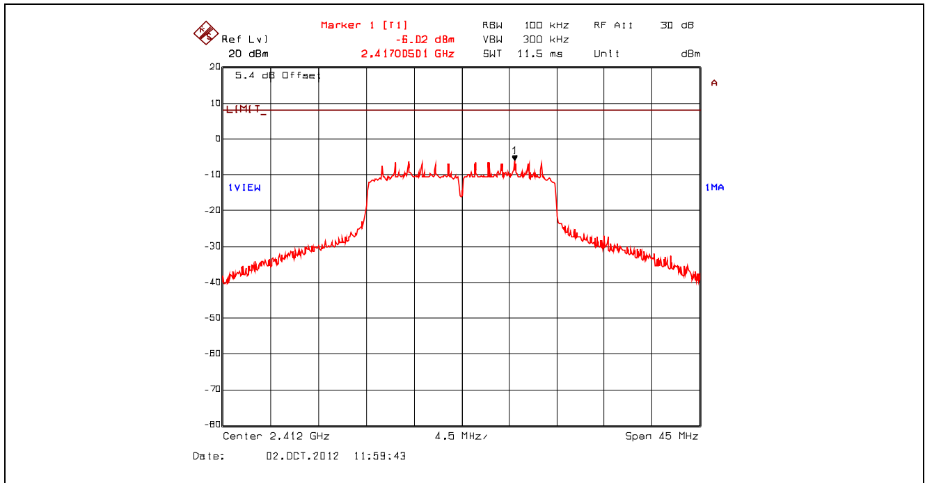
Plot 5.6.4.25. Power Spectral Density, 802.11n 800ns, 19.5 Mbps QPSK 3/4, 2412 MHz, Setting 23 Offset: Insertion Loss + BWCF = 20.63 dB + 10*log(3 kHz/ 100 kHz) = 5.43 dB
