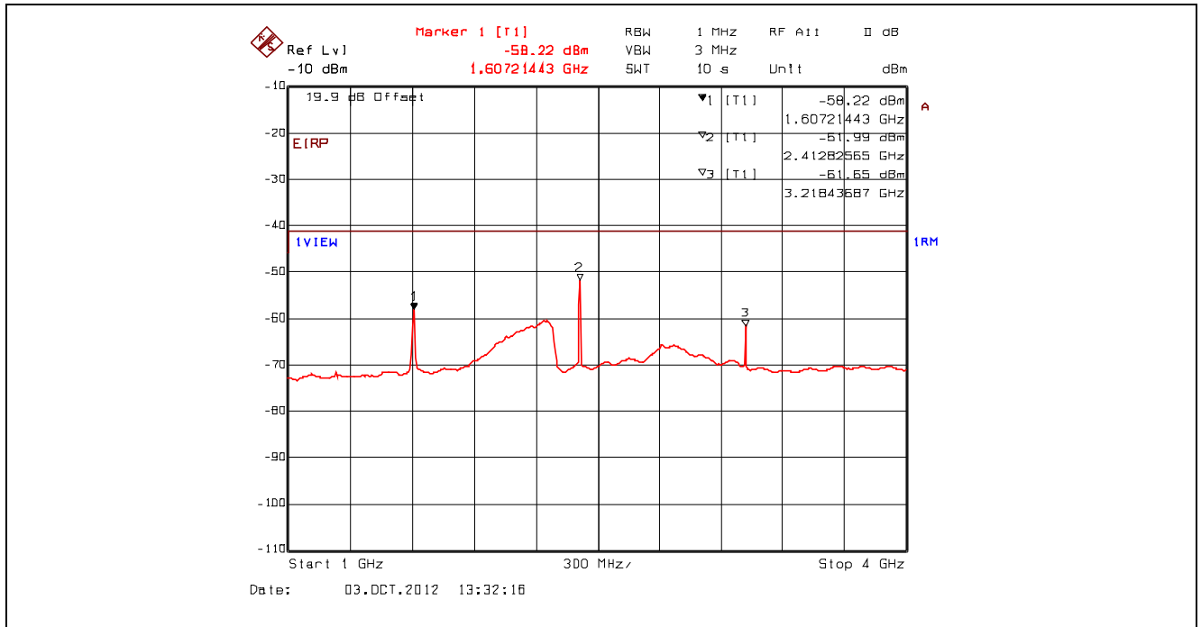
Plot 5.4.4.3.4. Conducted Spurious Emissions – Restricted Bands, 802.11b, 11 Mbps CCK 2412 MHz, 1 GHz - 4 GHz, Power Averaging with Band (Notch) Reject Filter
