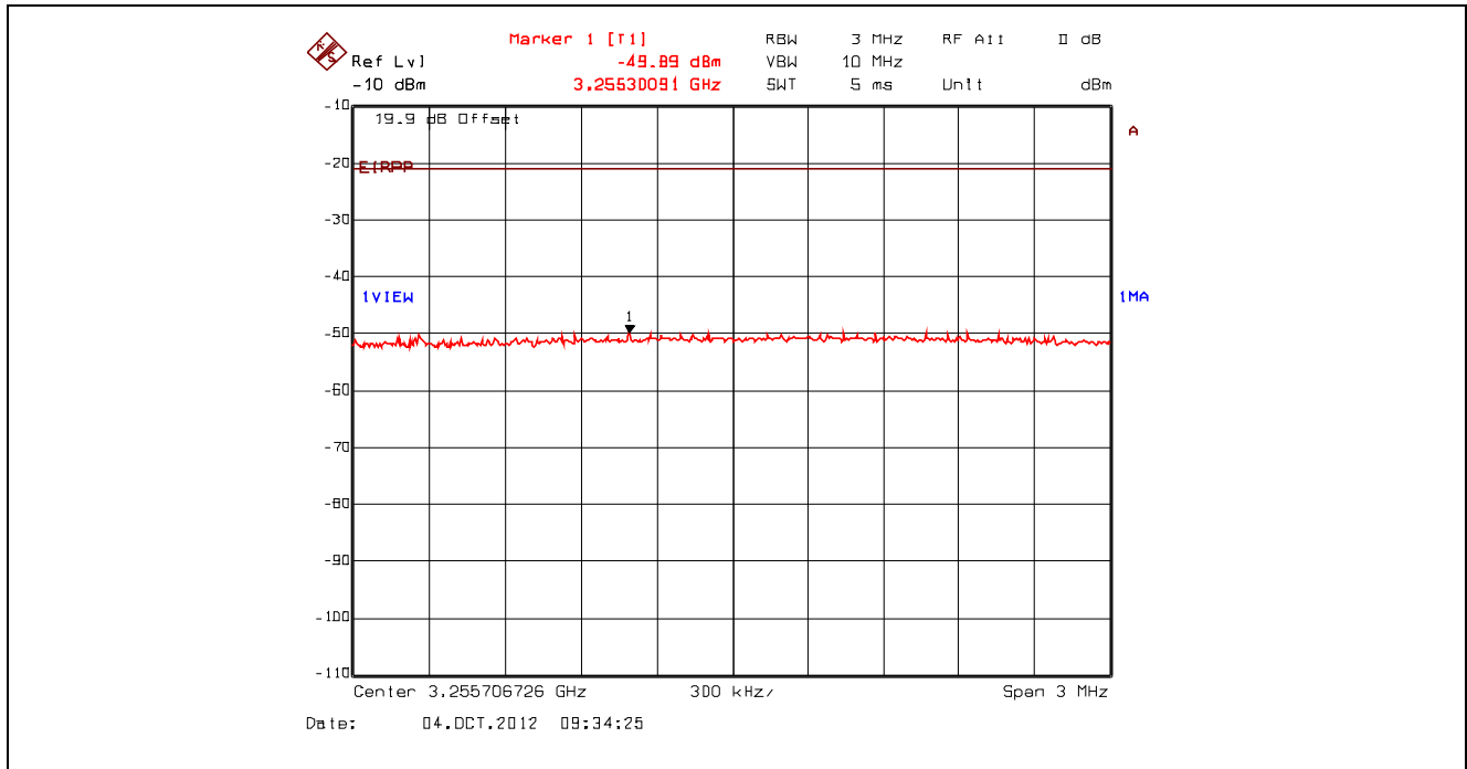
Plot 5.4.4.3.103. Conducted Spurious Emissions – Restricted Bands, 802.11n 400ns, 7.2 Mbps BPSK 1/2 2442 MHz, Peak Power at 3.26 GHz with Band (Notch) Reject Filter
