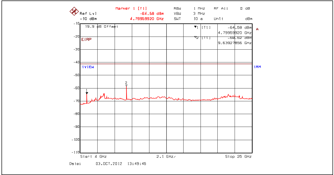
Plot 5.4.4.3.5. Conducted Spurious Emissions – Restricted Bands, 802.11b, 11 Mbps CCK 2412 MHz, 4 GHz - 25 GHz, Power Averaging with High Pass Filter
