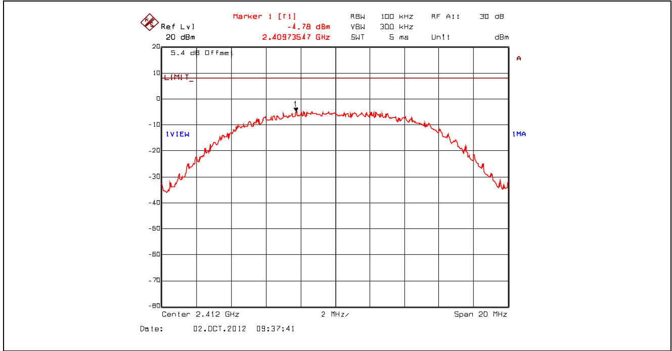
Plot 5.6.4.7. Power Spectral Density, 802.11b, 11 Mbps CCK, 2412 MHz, Setting 23 Offset: Insertion Loss + BWCF = 20.63 dB + 10 \cdot \log(3 \text{ kHz} / 100 \text{ kHz}) = 5.43 \text{ dB}
