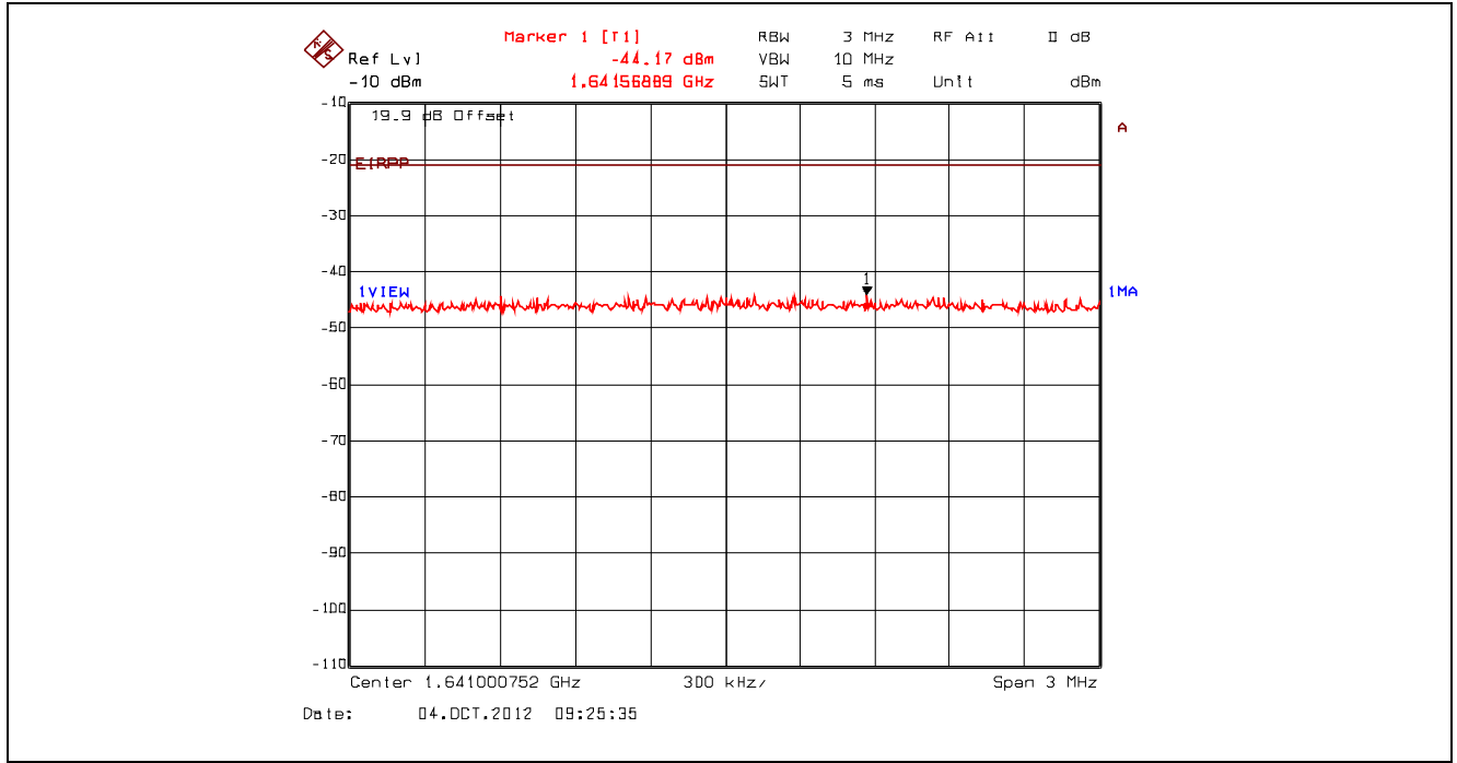
Plot 5.4.4.3.112. Conducted Spurious Emissions – Restricted Bands, 802.11n 400ns, 7.2 Mbps BPSK 1/2 2462 MHz, Peak Power at 1.64 GHz with Band (Notch) Reject Filter
