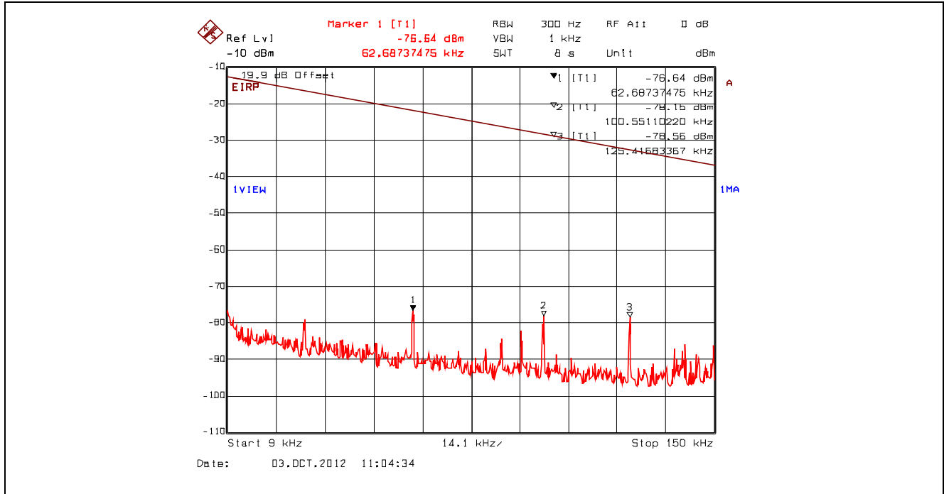
Plot 5.4.4.3.46. Conducted Spurious Emissions – Restricted Bands, 802.11g, 9 Mbps BPSK 2462 MHz, 9 kHz - 150 kHz, Peak Detector with Band (Notch) Reject Filter
