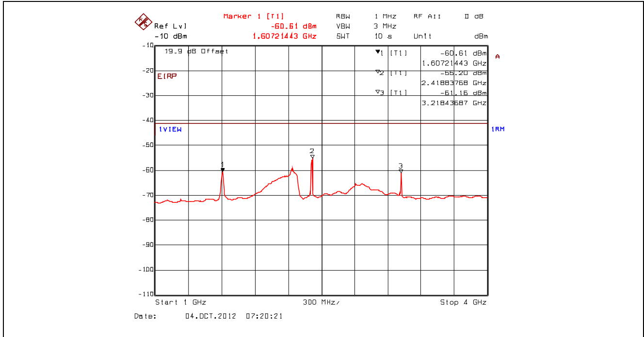
Plot 5.4.4.3.30. Conducted Spurious Emissions – Restricted Bands, 802.11g, 9 Mbps BPSK 2412 MHz, 1 GHz - 4 GHz, Power Averaging with Band (Notch) Reject Filter
