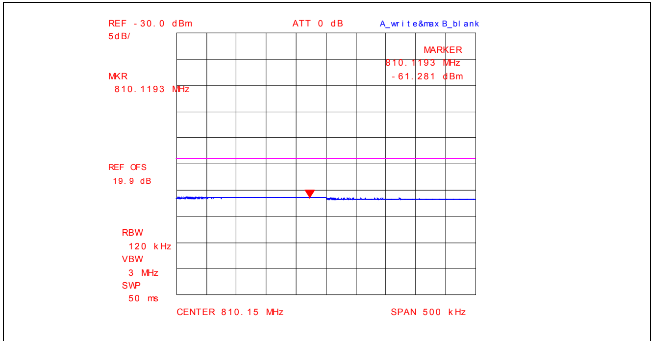
Plot 5.4.4.3.59. Conducted Spurious Emissions – Restricted Bands, 802.11n 800ns, 6.5 Mbps BPSK 1/2 2412 MHz, QP Power at 810.12 MHz with Band (Notch) Reject Filter
