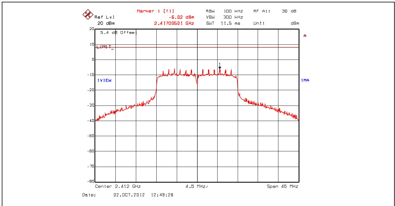
Plot 5.6.4.37. Power Spectral Density, 802.11n 400ns, 21.7 Mbps QPSK 3/4, 2412 MHz, Setting 23 Offset: Insertion Loss + BWCF = 20.63 dB + 10*log(3 kHz/ 100 kHz) = 5.43 dB
