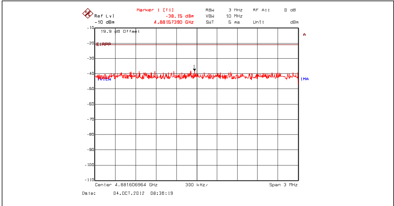
Plot 5.4.4.3.44. Conducted Spurious Emissions – Restricted Bands, 802.11g, 9 Mbps BPSK 2442 MHz, Peak Power at 4.88 GHz with High Pass Filter
