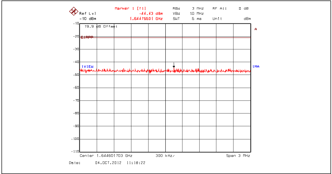
Plot 5.4.4.3.52. Conducted Spurious Emissions – Restricted Bands, 802.11g, 9 Mbps BPSK 2462 MHz, Peak Power at 1.64 GHz with Band (Notch) Reject Filter
