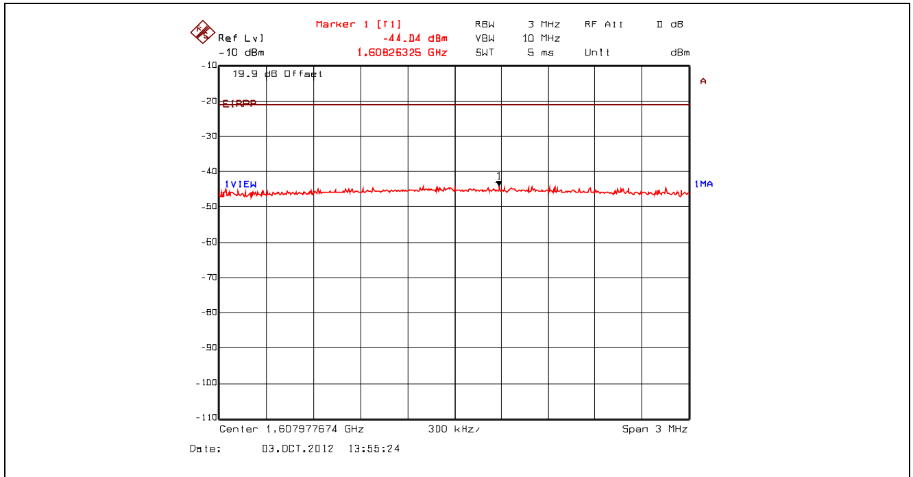
Plot 5.4.4.3.6. Conducted Spurious Emissions – Restricted Bands, 802.11b, 11 Mbps CCK 2412 MHz, Peak Power at 1.61 GHz with Band (Notch) Reject Filter
