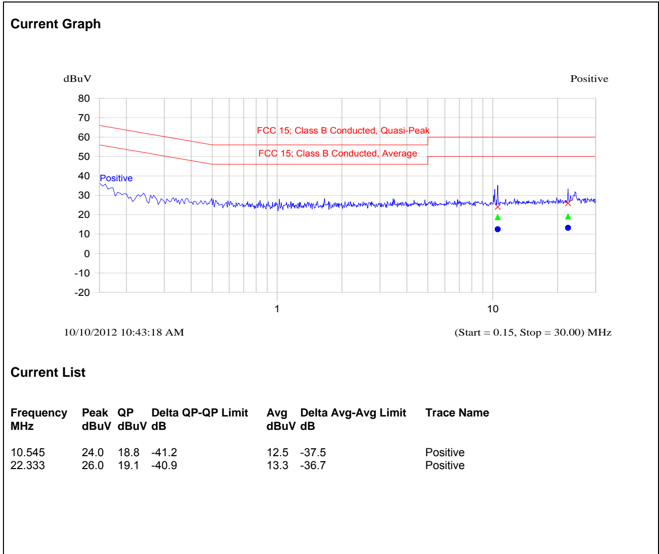
Plot 5.1.4.1. Power Line Conducted Emissions; Line Voltage: 3.5 V DC; Line Tested: Positive
