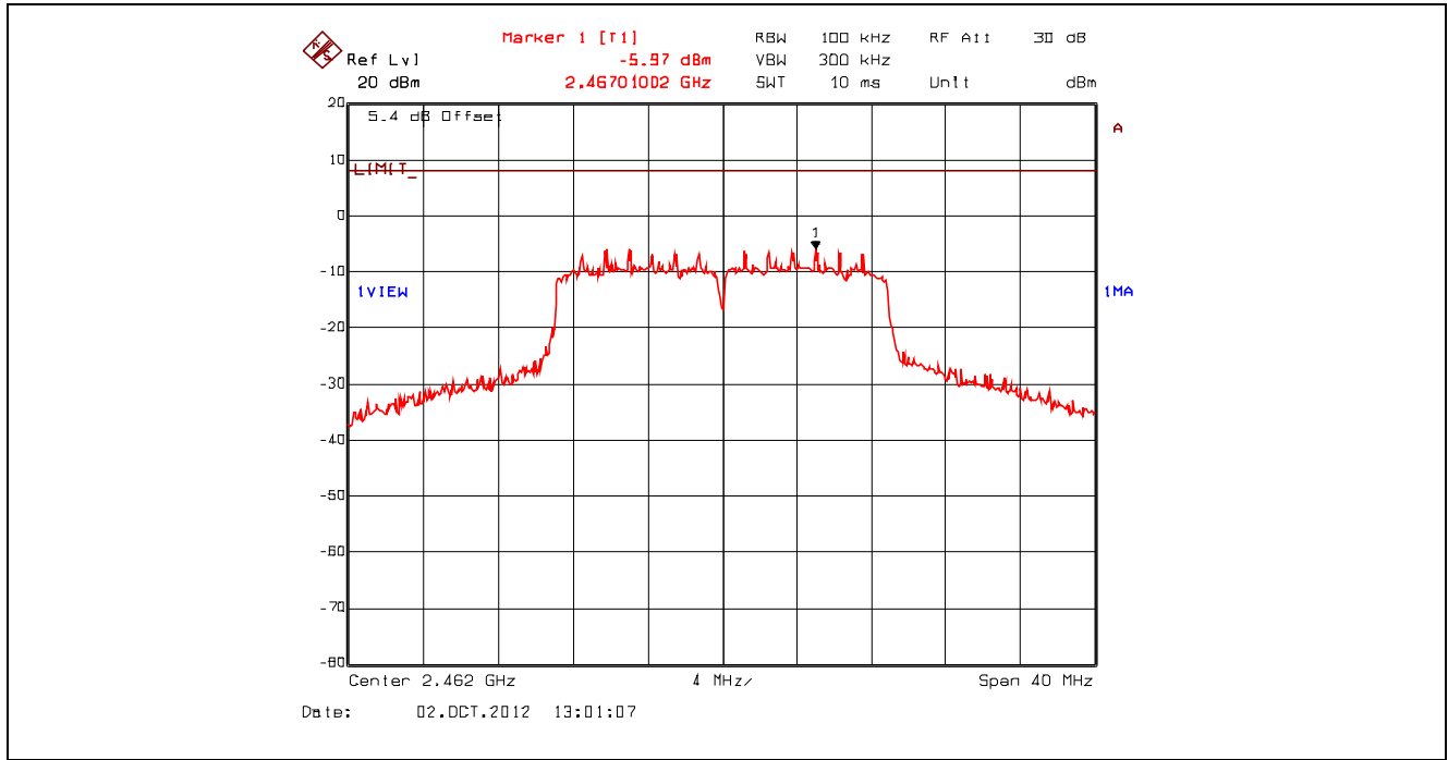
Plot 5.6.4.42. Power Spectral Density, 802.11n 400ns, 43.3 Mbps 16-QAM 3/4, 2462 MHz, Setting 23 Offset: Insertion Loss + BWCF = 20.63 dB + 10*log(3 kHz/ 100 kHz) = 5.43 dB
