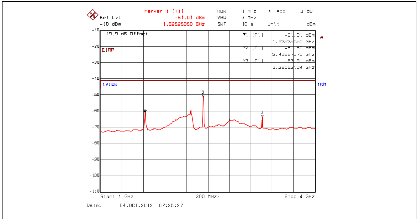
Plot 5.4.4.3.40. Conducted Spurious Emissions – Restricted Bands, 802.11g, 9 Mbps BPSK 2442 MHz, 1 GHz - 4 GHz, Power Averaging with Band (Notch) Reject Filter
