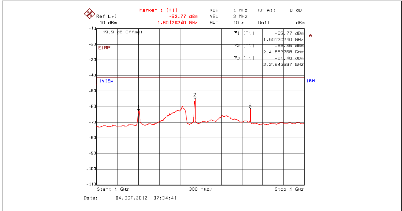
Plot 5.4.4.3.60. Conducted Spurious Emissions – Restricted Bands, 802.11n 800ns, 6.5 Mbps BPSK 1/2 2412 MHz, 1 GHz - 4 GHz, Power Averaging with Band (Notch) Reject Filter
