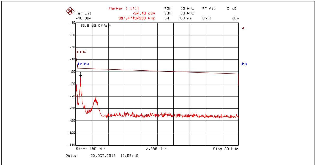
Plot 5.4.4.3.37. Conducted Spurious Emissions – Restricted Bands, 802.11g, 9 Mbps BPSK 2442 MHz, 150 kHz - 30 MHz, Peak Detector with Band (Notch) Reject Filter
