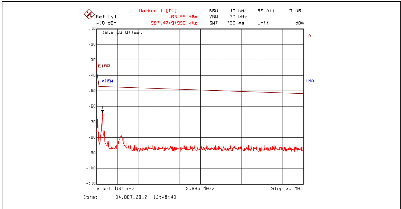
Plot 5.4.4.3.97. Conducted Spurious Emissions – Restricted Bands, 802.11n 400ns, 7.2 Mbps BPSK 1/2 2442 MHz, 150 kHz - 30 MHz, Peak Detector with Band (Notch) Reject Filter
