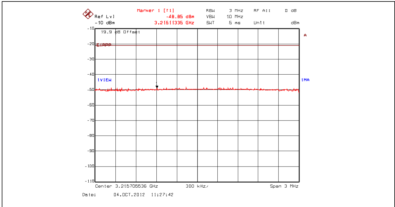
Plot 5.4.4.3.33. Conducted Spurious Emissions – Restricted Bands, 802.11g, 9 Mbps BPSK 2412 MHz, Peak Power at 3.22 GHz with High Pass Filter
