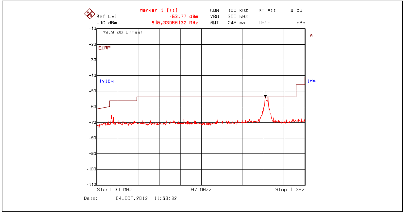
Plot 5.4.4.3.108. Conducted Spurious Emissions – Restricted Bands, 802.11n 400ns, 7.2 Mbps BPSK 1/2 2462 MHz, 30 MHz - 1 GHz, Peak Detector with Band (Notch) Reject Filter
