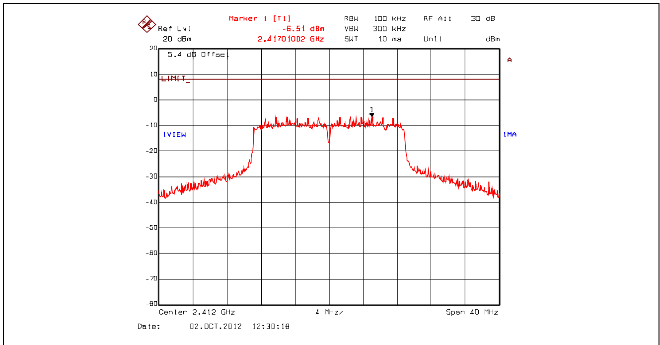
Plot 5.6.4.31. Power Spectral Density, 802.11n 800ns, 65 Mbps 64-QAM 5/6, 2412 MHz, Setting 23 Offset: Insertion Loss + BWCF = 20.63 dB + 10 \cdot \log(3 \text{ kHz} / 100 \text{ kHz}) = 5.43 \text{ dB}
