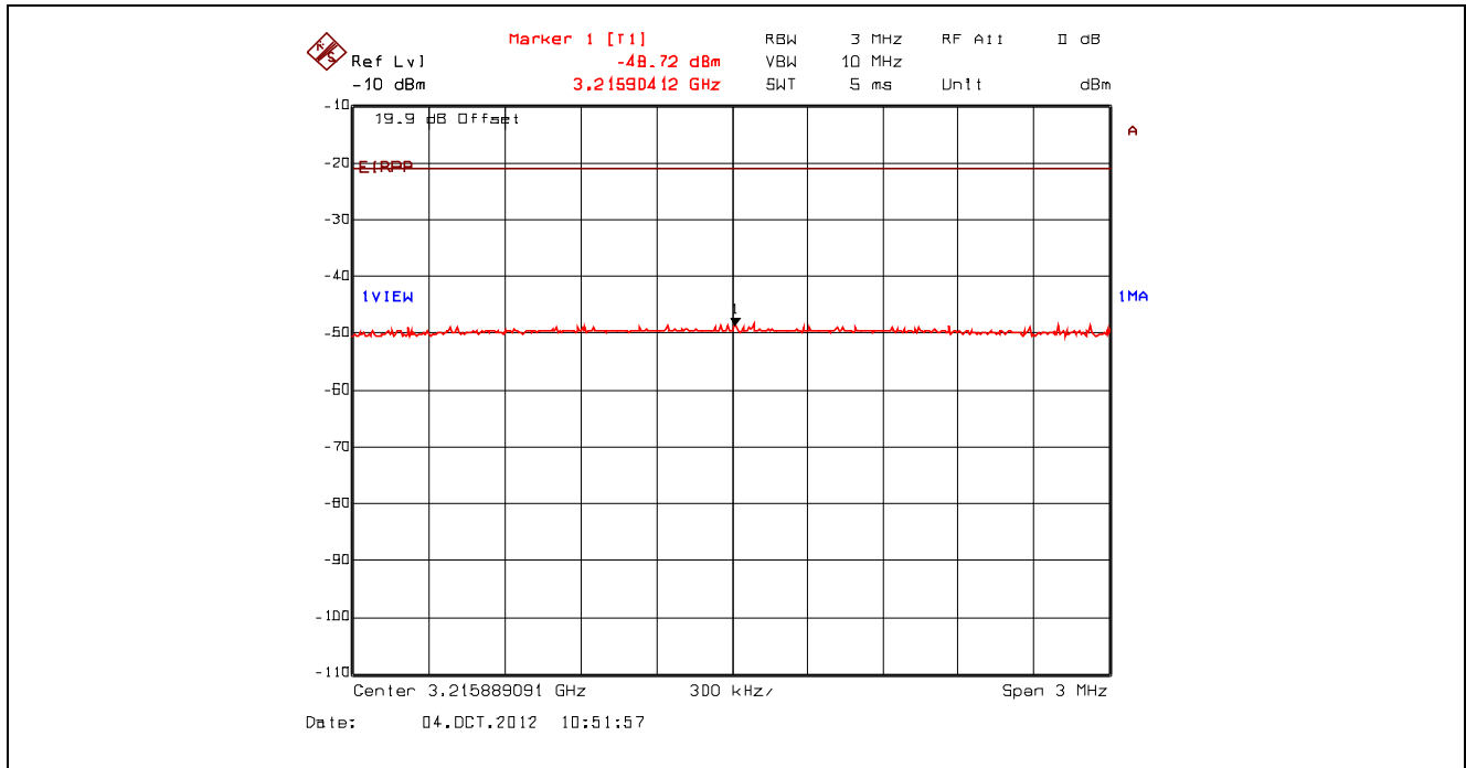
Plot 5.4.4.3.93. Conducted Spurious Emissions – Restricted Bands, 802.11n 400ns, 7.2 Mbps BPSK 1/2 2412 MHz, Peak Power at 3.22 GHz with Band (Notch) Reject Filter
