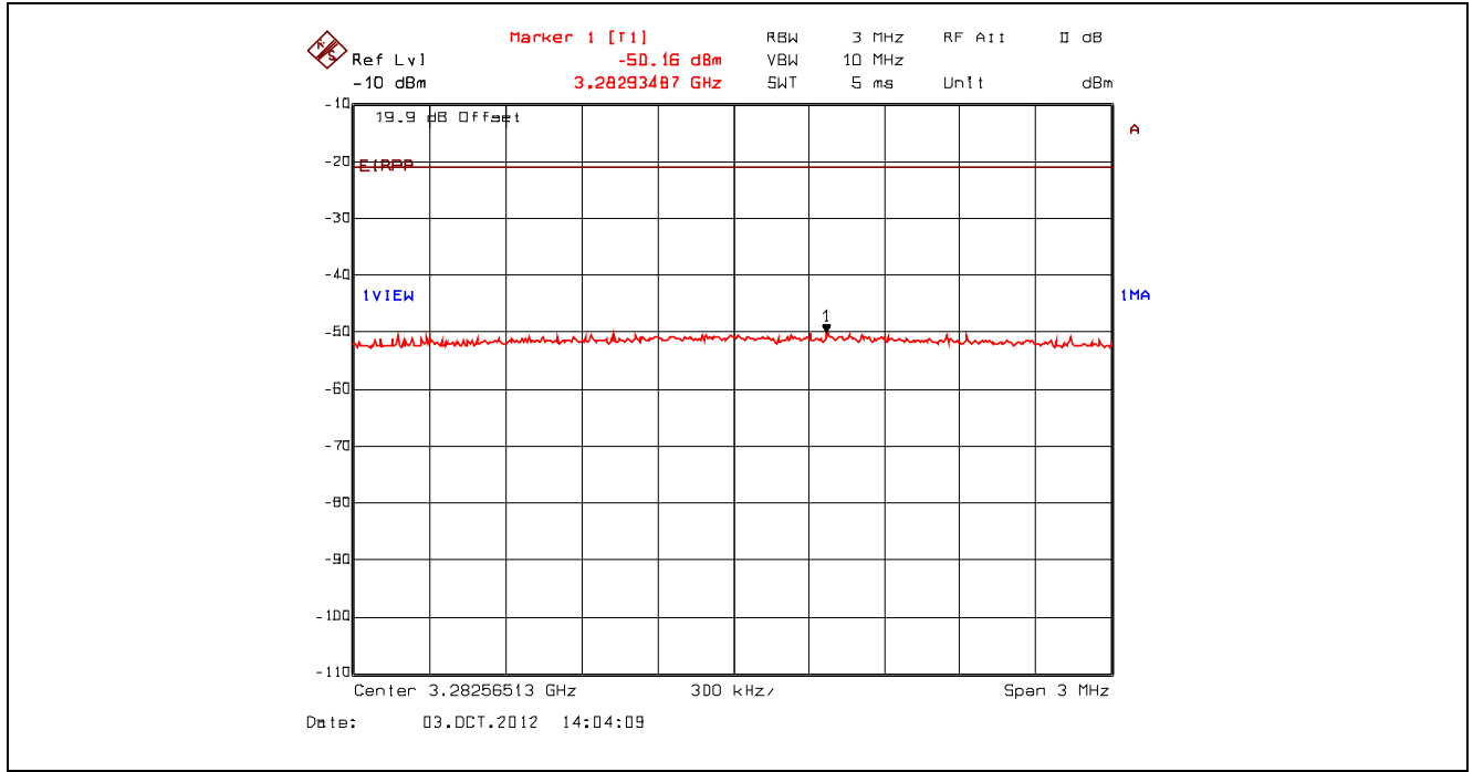
Plot 5.4.4.3.24. Conducted Spurious Emissions – Restricted Bands, 802.11b, 11 Mbps CCK 2462 MHz, Peak Power at 3.28 GHz with Band (Notch) Reject Filter
