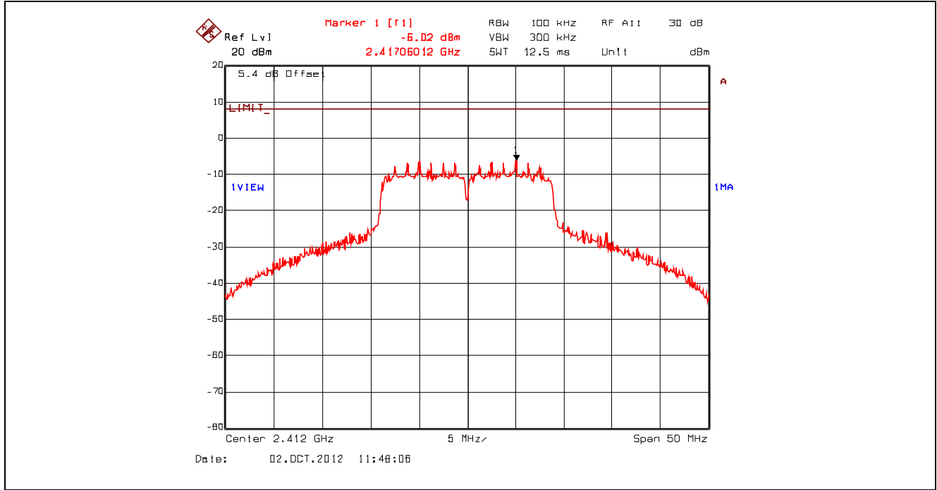
Plot 5.6.4.22. Power Spectral Density, 802.11n 800ns, 6.5 Mbps BPSK1/2, 2412 MHz, Setting 23 Offset: Insertion Loss + BWCF = 20.63 dB + 10*log(3 kHz/ 100 kHz) = 5.43 dB
