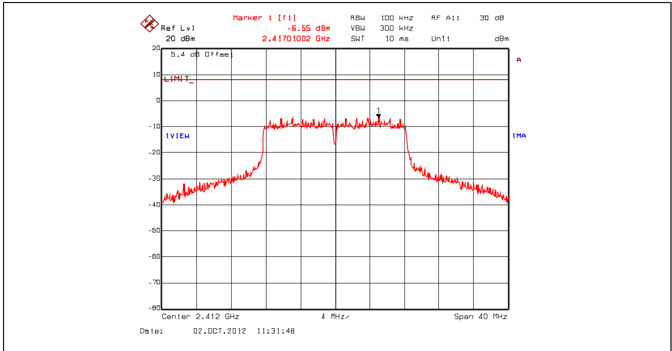
Plot 5.6.4.19. Power Spectral Density, 802.11g, 54 Mbps 64-QAM, 2412 MHz, Setting 23 Offset: Insertion Loss + BWCF = 20.63 dB + 10*log(3 kHz/ 100 kHz) = 5.43 dB
