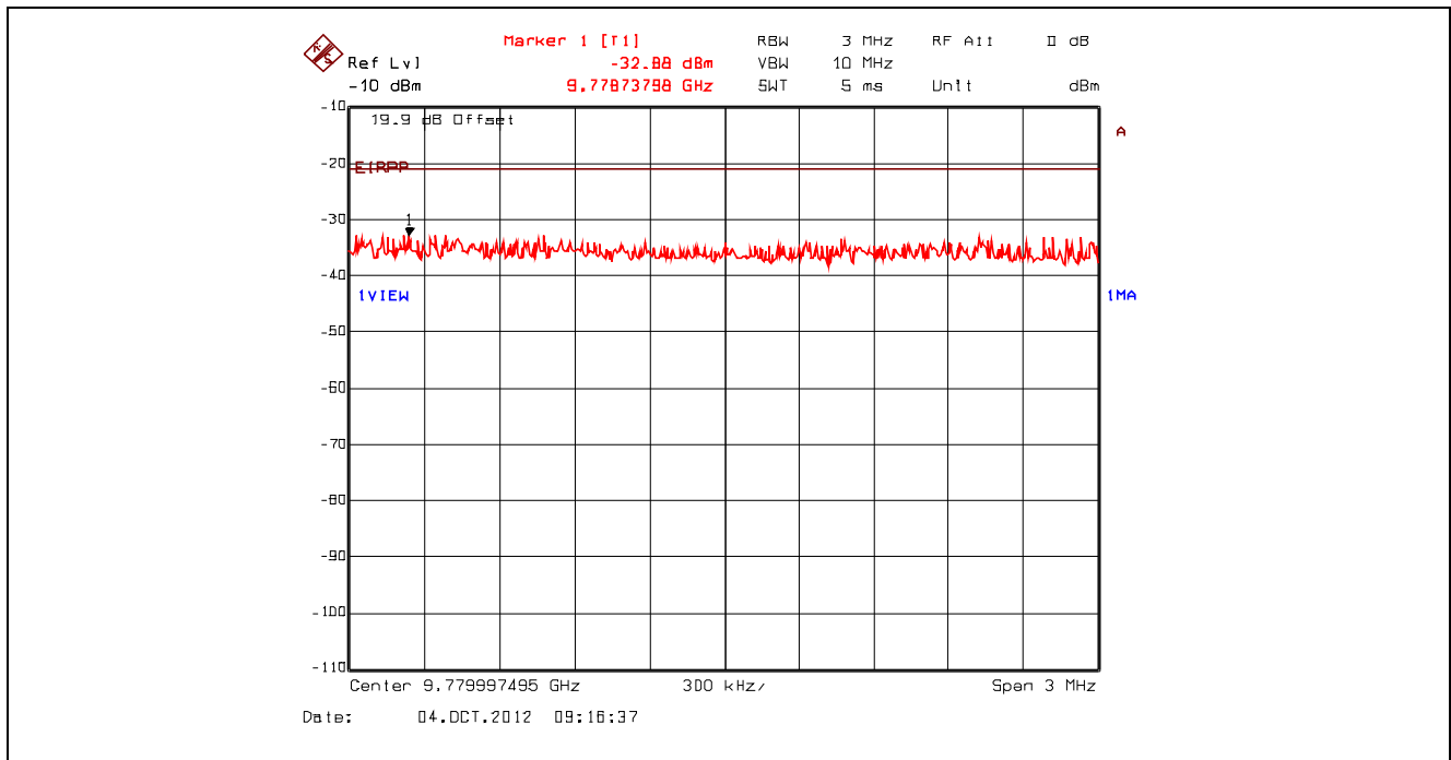
Plot 5.4.4.3.105. Conducted Spurious Emissions – Restricted Bands, 802.11n 400ns, 7.2 Mbps BPSK 1/2 2442 MHz, Peak Power at 9.78 GHz with High Pass Filter
