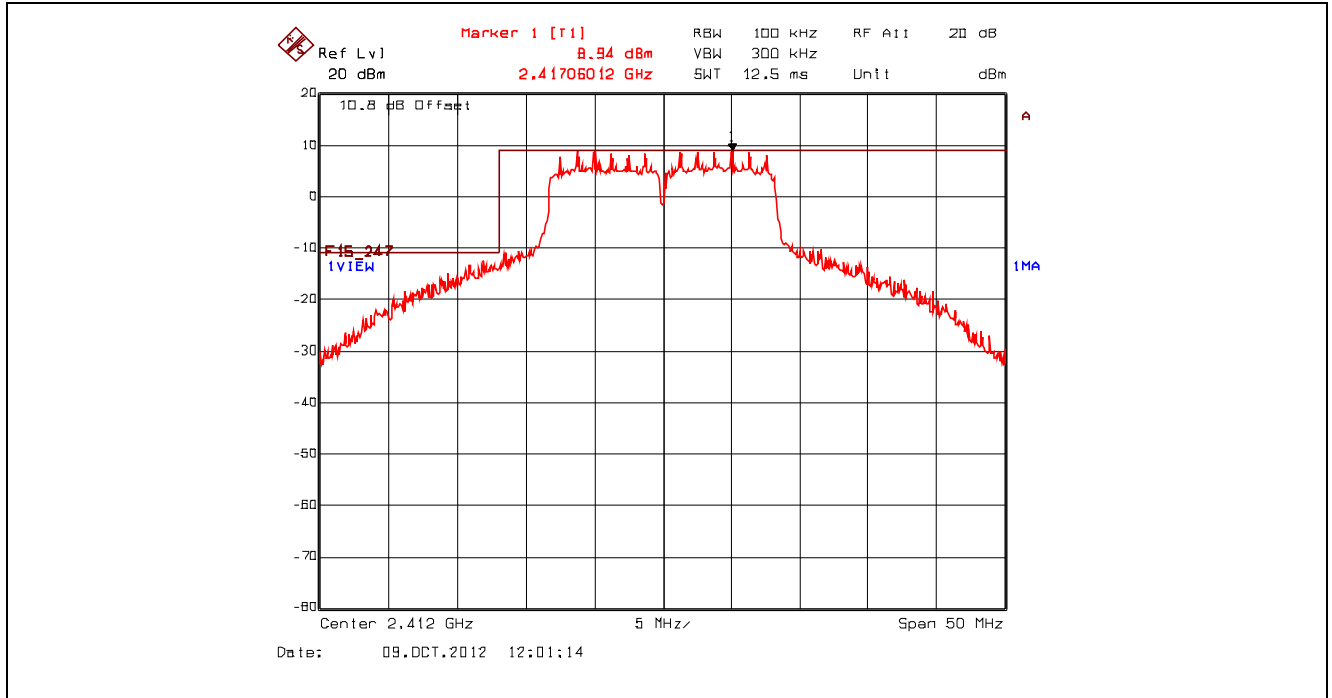
Plot 5.4.4.1.3. Band-Edge RF Conducted Emissions, Lower Band-edge, 2412 MHz, 802.11g, 9 Mbps BPSK
