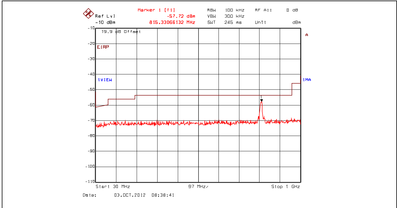
Plot 5.4.4.3.12. Conducted Spurious Emissions – Restricted Bands, 802.11b, 11 Mbps CCK 2442 MHz, 30 MHz - 1 GHz, Peak Detector with Band (Notch) Reject Filter
