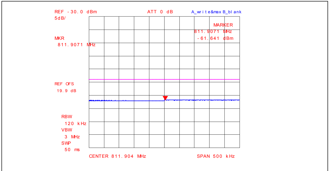
Plot 5.4.4.3.109. Conducted Spurious Emissions – Restricted Bands, 802.11n 400ns, 7.2 Mbps BPSK 1/2 2462 MHz, QP Power at 811.91 MHz with Band (Notch) Reject Filter
