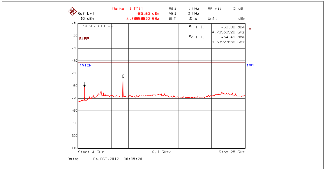
Plot 5.4.4.3.91. Conducted Spurious Emissions – Restricted Bands, 802.11n 400ns, 7.2 Mbps BPSK 1/2 2412 MHz, 4 GHz - 25 GHz, Power Averaging with High Pass Filter
