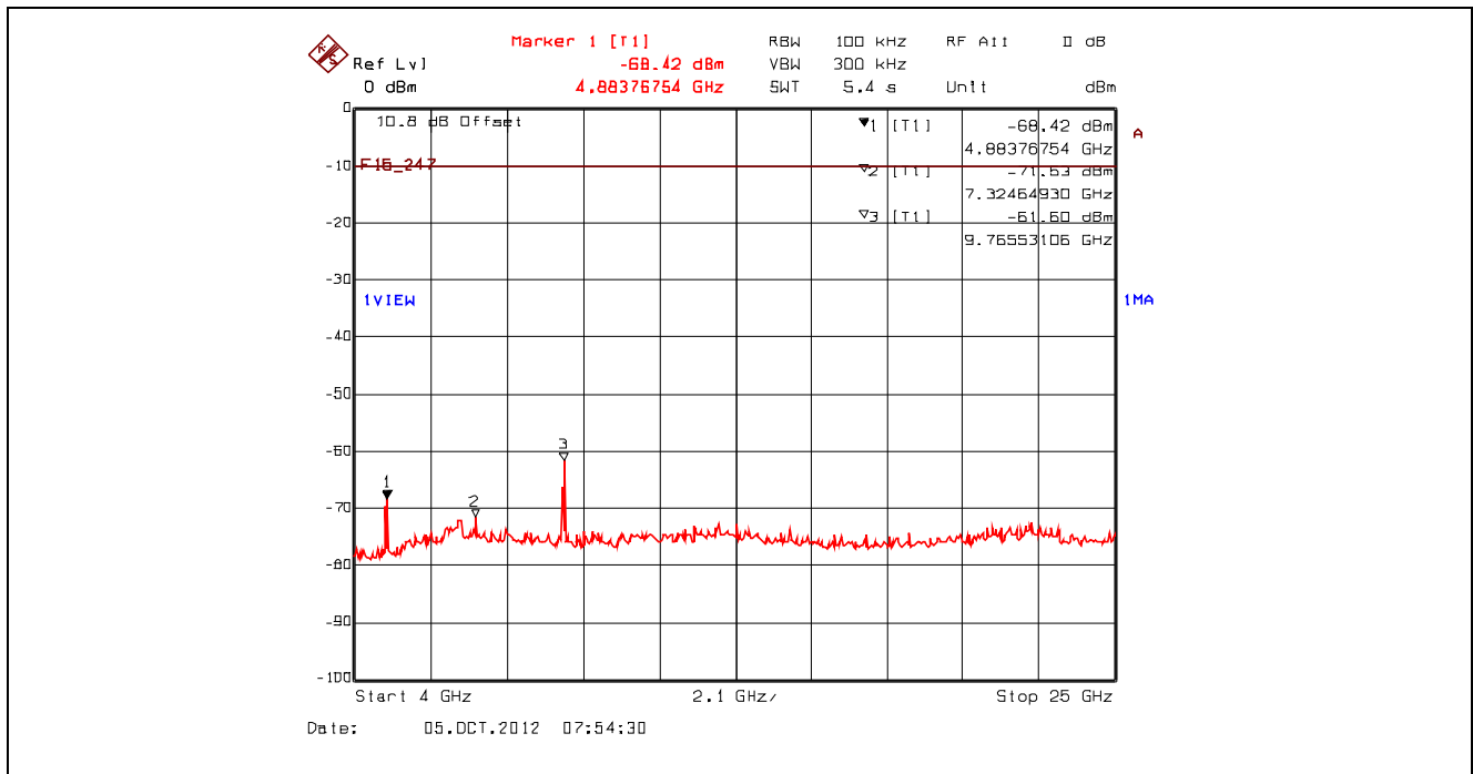
Plot 5.4.4.2.16. Conducted Spurious Emissions - Non Restricted Frequency Bands, 802.11n 800ns, 4 GHz – 25 GHz 2442 MHz, High Power, 6.5 Mbps BPSK 1/2, Power Setting 23 dBm
