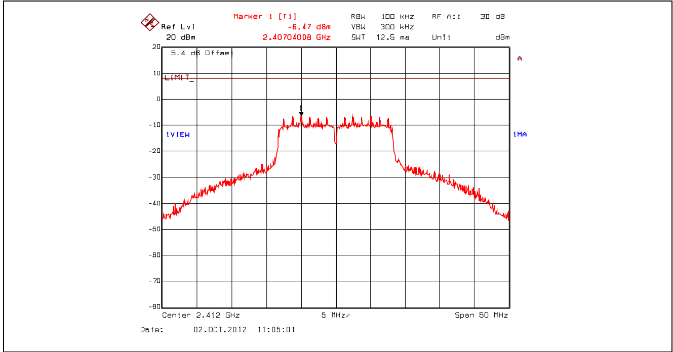
Plot 5.6.4.10. Power Spectral Density, 802.11g, 9 Mbps BPSK, 2412 MHz, Setting 23 Offset: Insertion Loss + BWCF = 20.63 dB + 10*log(3 kHz/ 100 kHz) = 5.43 dB
