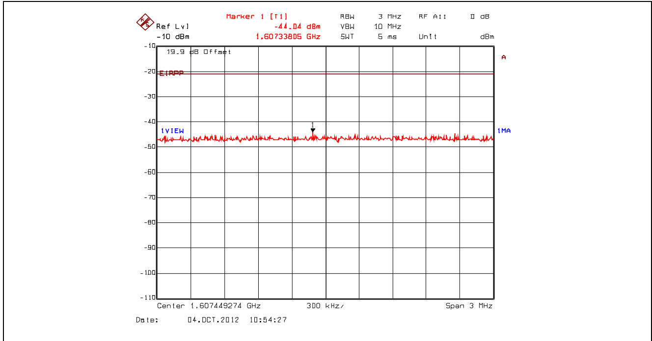
Plot 5.4.4.3.92. Conducted Spurious Emissions – Restricted Bands, 802.11n 400ns, 7.2 Mbps BPSK 1/2 2412 MHz, Peak Power at 1.61 GHz with Band (Notch) Reject Filter
