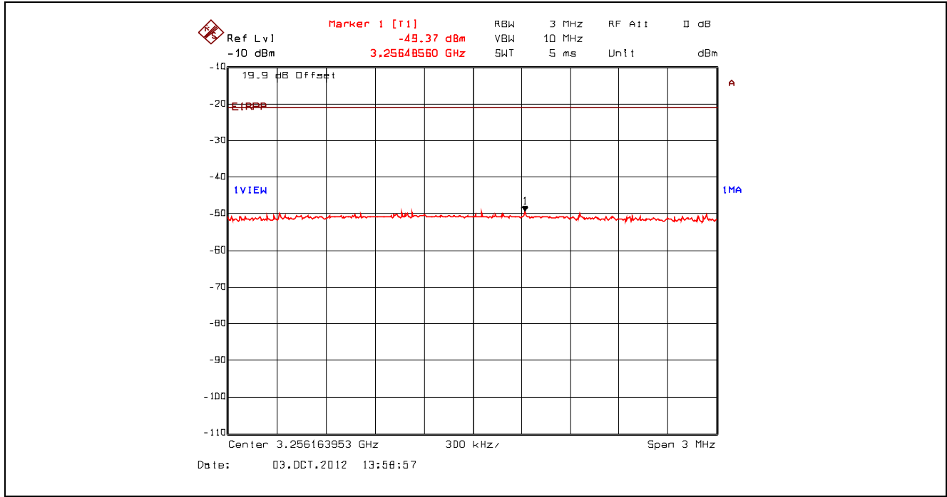
Plot 5.4.4.3.16. Conducted Spurious Emissions – Restricted Bands, 802.11b, 11 Mbps CCK 2442 MHz, Peak Power at 3.26 GHz with Band (Notch) Reject Filter
