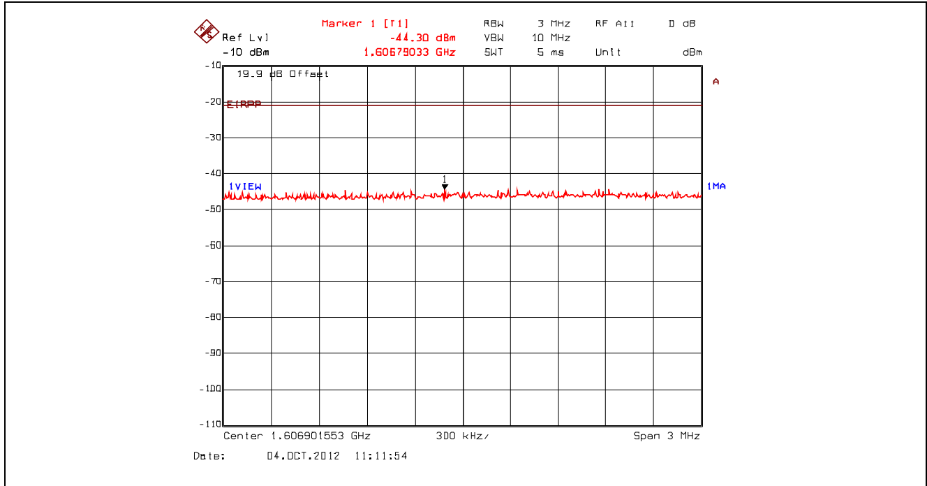
Plot 5.4.4.3.62. Conducted Spurious Emissions – Restricted Bands, 802.11n 800ns, 6.5 Mbps BPSK 1/2 2412 MHz, Peak Power at 1.61 GHz with Band (Notch) Reject Filter
