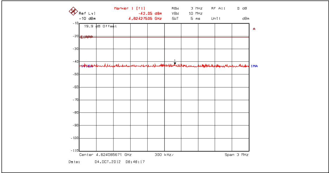
Plot 5.4.4.3.64. Conducted Spurious Emissions – Restricted Bands, 802.11n 800ns, 6.5 Mbps BPSK 1/2 2412 MHz, Peak Power at 4.82 GHz with High Pass Filter
