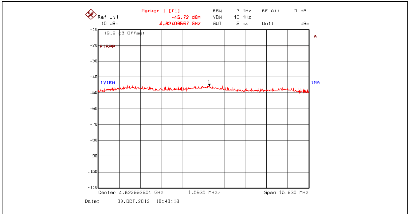
Plot 5.4.4.3.8. Conducted Spurious Emissions – Restricted Bands, 802.11b, 11 Mbps CCK 2412 MHz, Peak Power at 4.82 GHz with High Pass Filter
