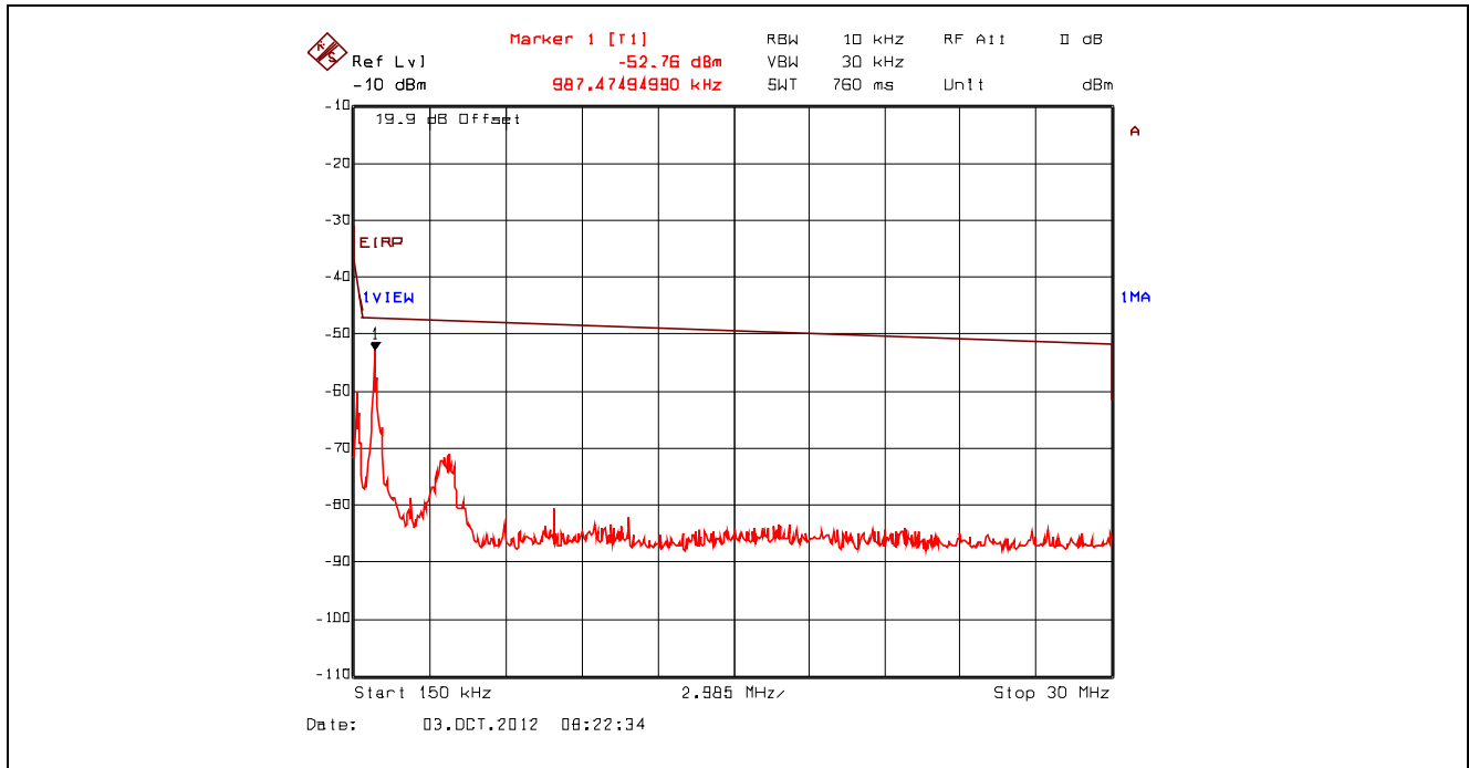
Plot 5.4.4.3.19. Conducted Spurious Emissions – Restricted Bands, 802.11b, 11 Mbps CCK 2462 MHz, 150 kHz - 30 MHz, Peak Detector with Band (Notch) Reject Filter
