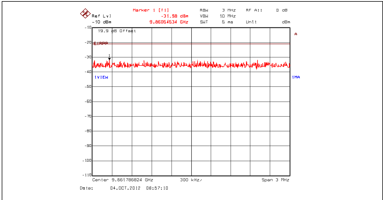
Plot 5.4.4.3.85. Conducted Spurious Emissions – Restricted Bands, 802.11n 800ns, 6.5 Mbps BPSK 1/2 2462 MHz, Peak Power at 9.86 GHz with High Pass Filter
