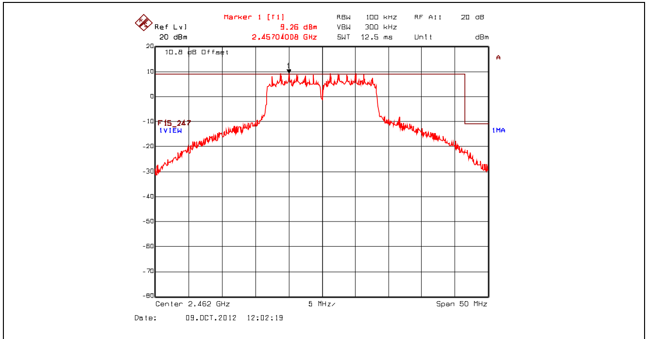
Plot 5.4.4.1.4. Band-Edge RF Conducted Emissions, Upper Band-edge, 2462 MHz, 802.11g, 9 Mbps BPSK
