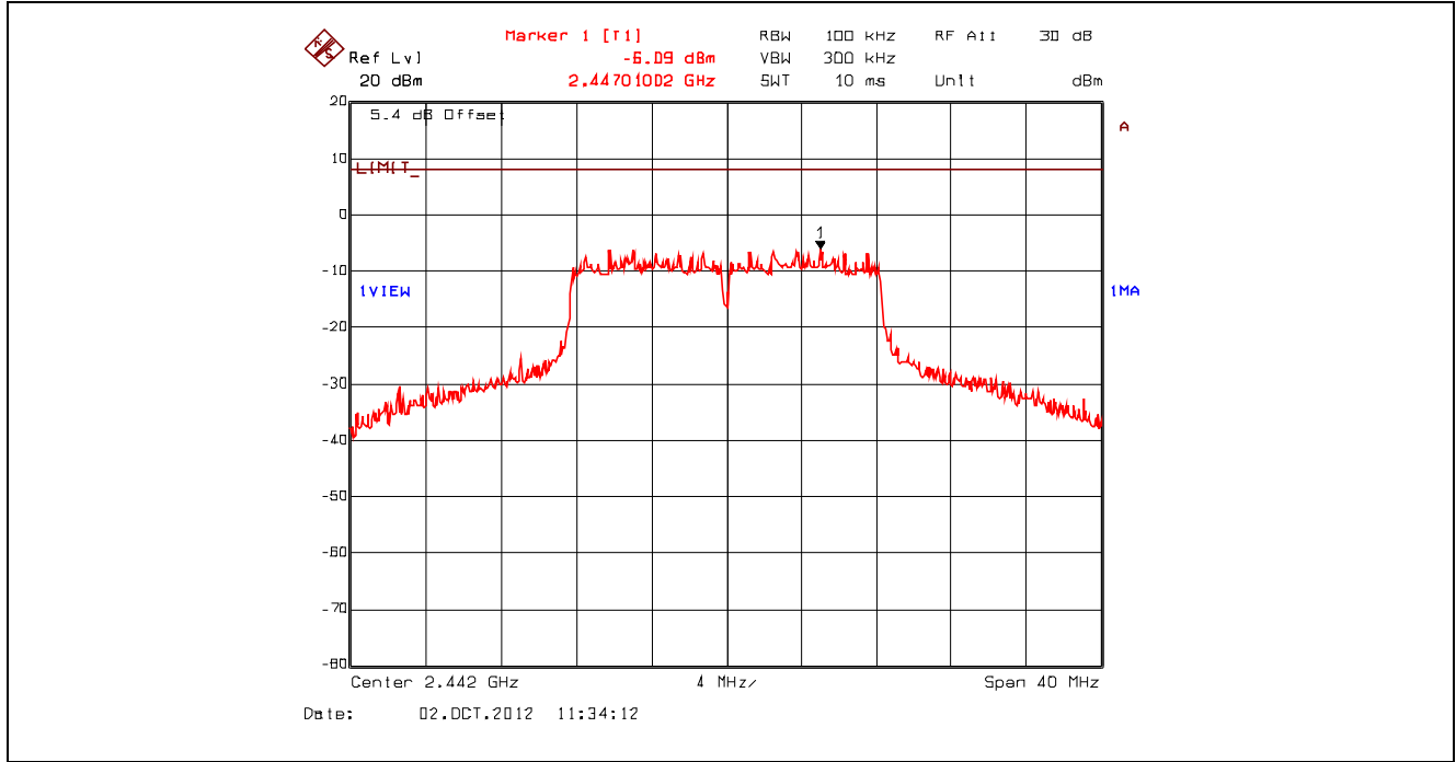
Plot 5.6.4.20. Power Spectral Density, 802.11g, 54 Mbps 64-QAM, 2442 MHz, Setting 23 Offset: Insertion Loss + BWCF = 20.63 dB + 10*log(3 kHz/ 100 kHz) = 5.43 dB
