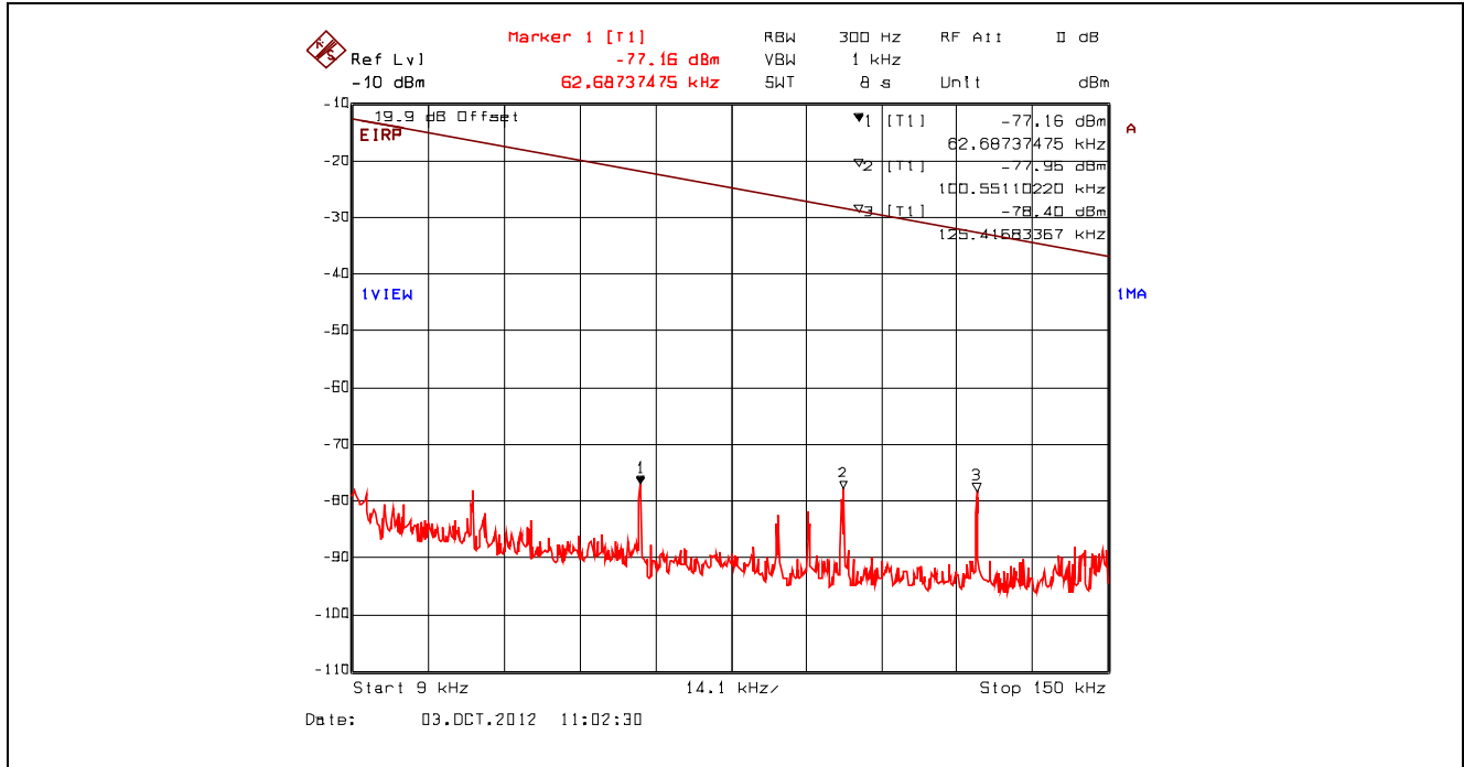
Plot 5.4.4.3.36. Conducted Spurious Emissions – Restricted Bands, 802.11g, 9 Mbps BPSK 2442 MHz, 9 kHz - 150 kHz, Peak Detector with Band (Notch) Reject Filter
