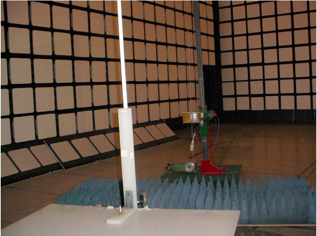
Radiated Emissions at 3 m EUT with 15 dBi Omni-directional Antenna
