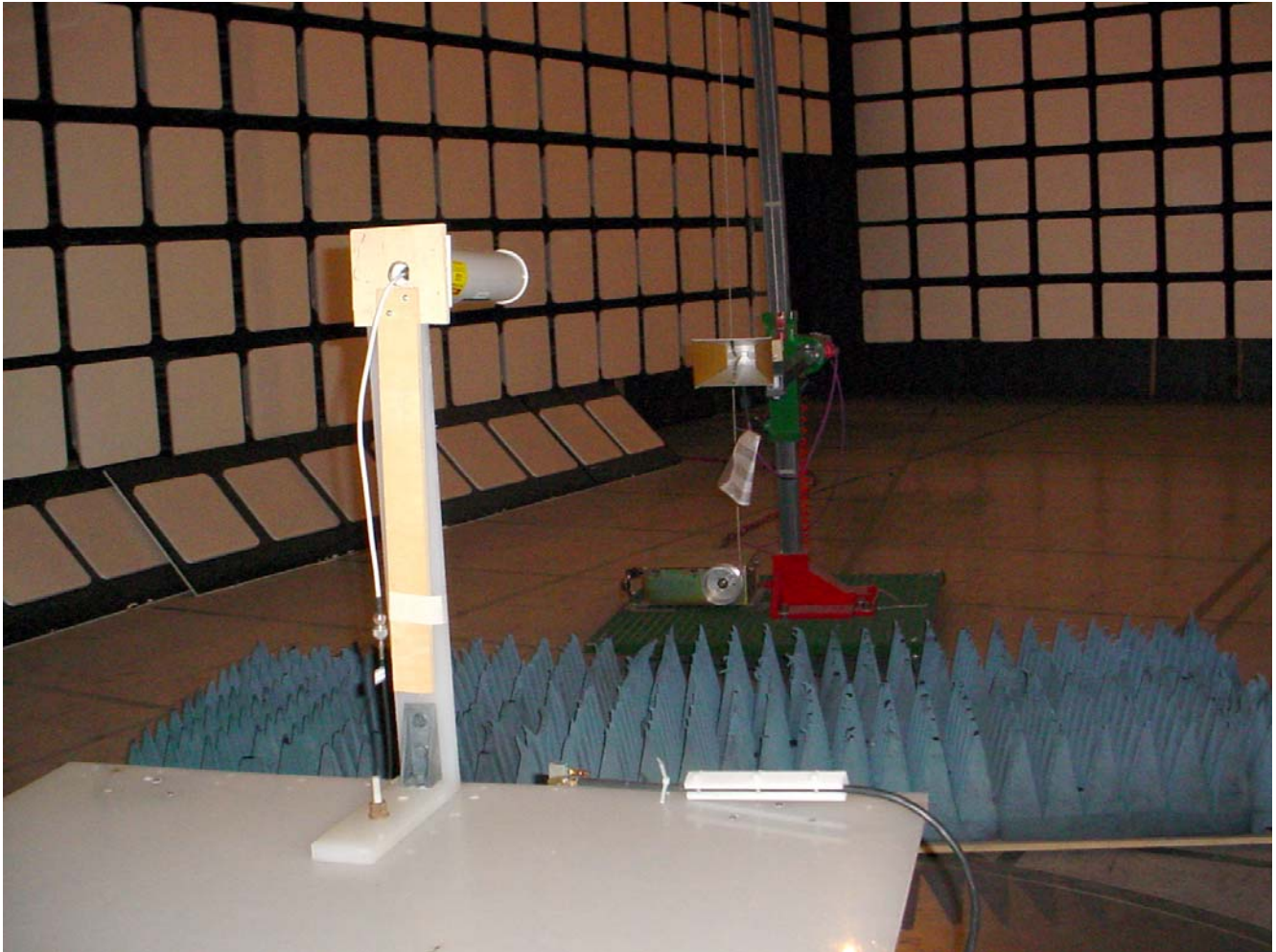
Radiated Emissions at 3 m EUT with 15 dBi Yagi Antenna
