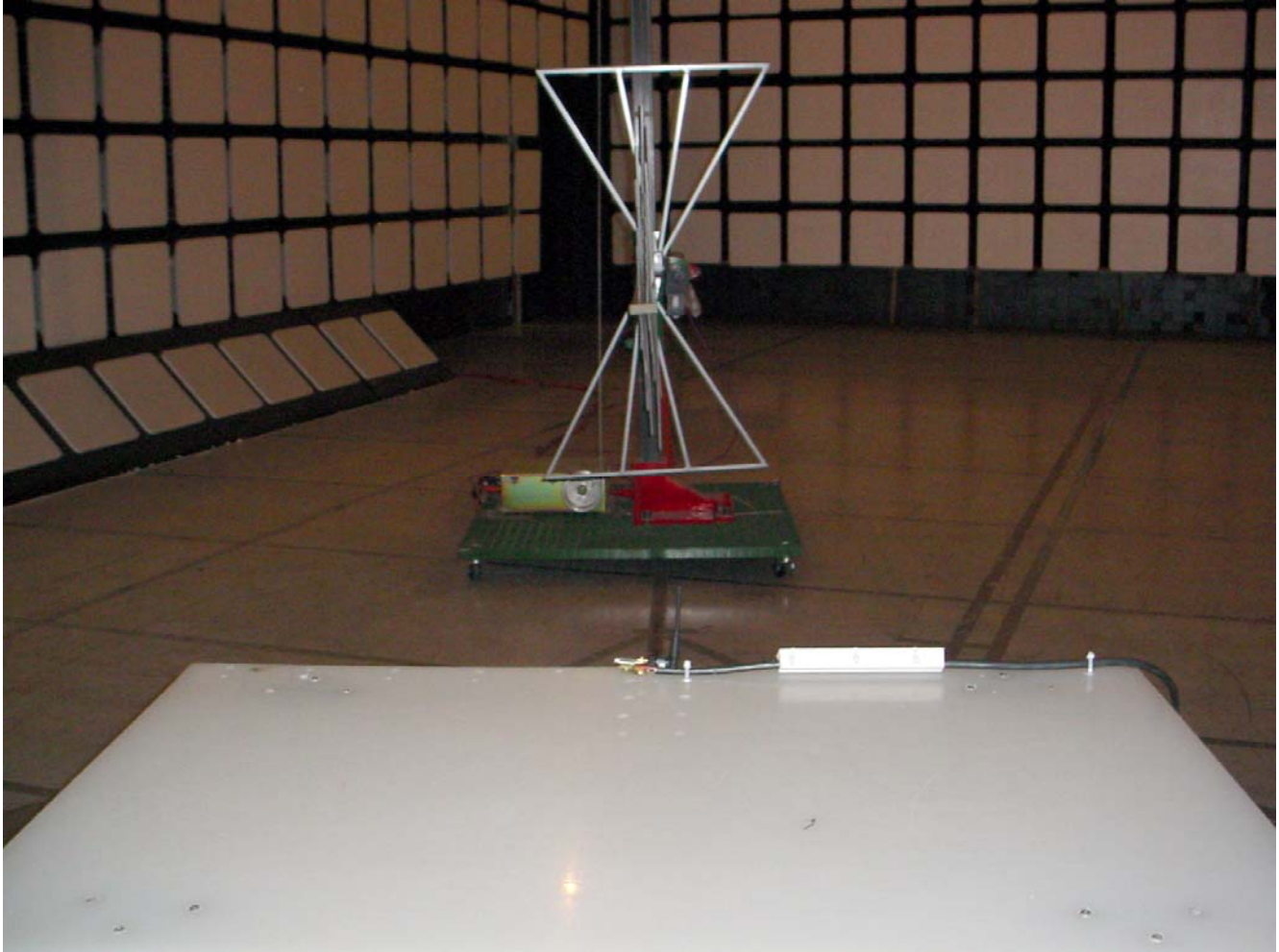
Radiated Emissions at 3 m EUT with 2.1 dBi Dipole Antenna
