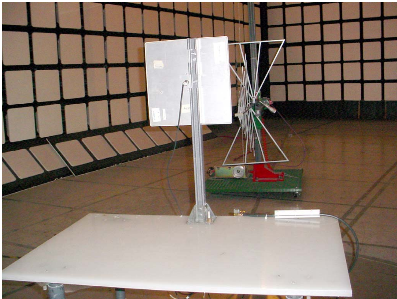
Radiated Emissions at 3 m EUT with 19 dBi Panel Antenna
