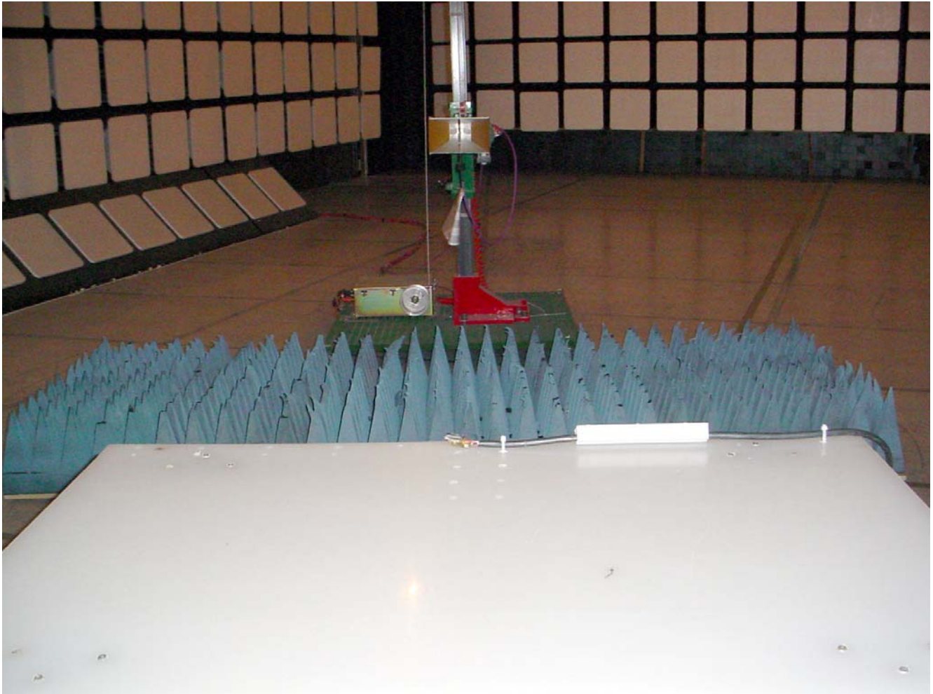
Radiated Emissions at 3 m EUT with 1.5 dBi Integrated Whip Monopole Antenna
