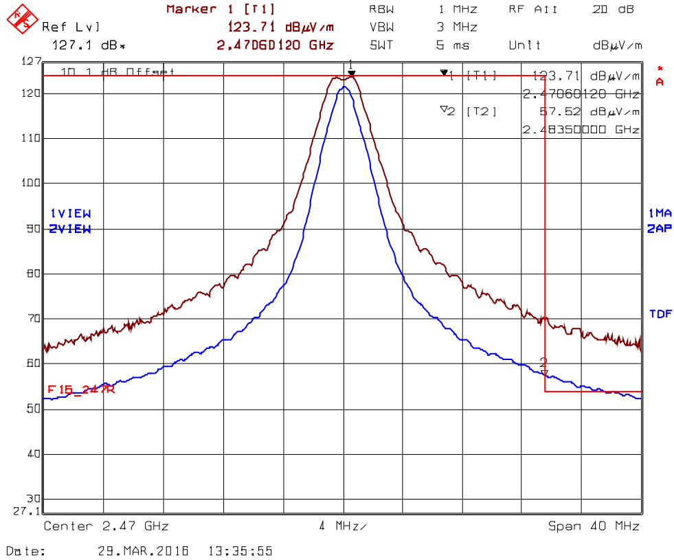
Plot 5.2.4.5.2.3. Band-Edge RF Radiated Emissions at 3 m, Horizontal Polarization High End of Frequency Band, Ch24- 2470 MHz, QPSK Modulation, Power 8 Mode 1 @ 66% Duty Cycle
