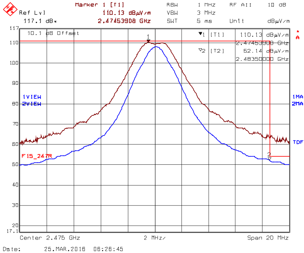
Plot 5.2.4.2.4. Band-Edge RF Radiated Emissions at 3 m, Vertical Polarization High End of Frequency Band, Ch25- 2475 MHz, QPSK Modulation, Power 8 Mode 1
