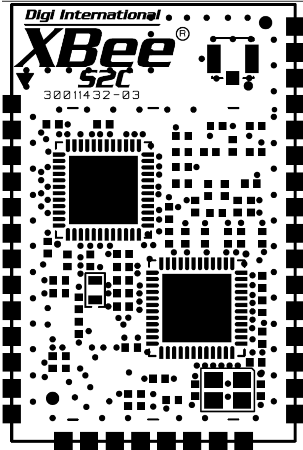
Top Silk mask for XBee S2C
