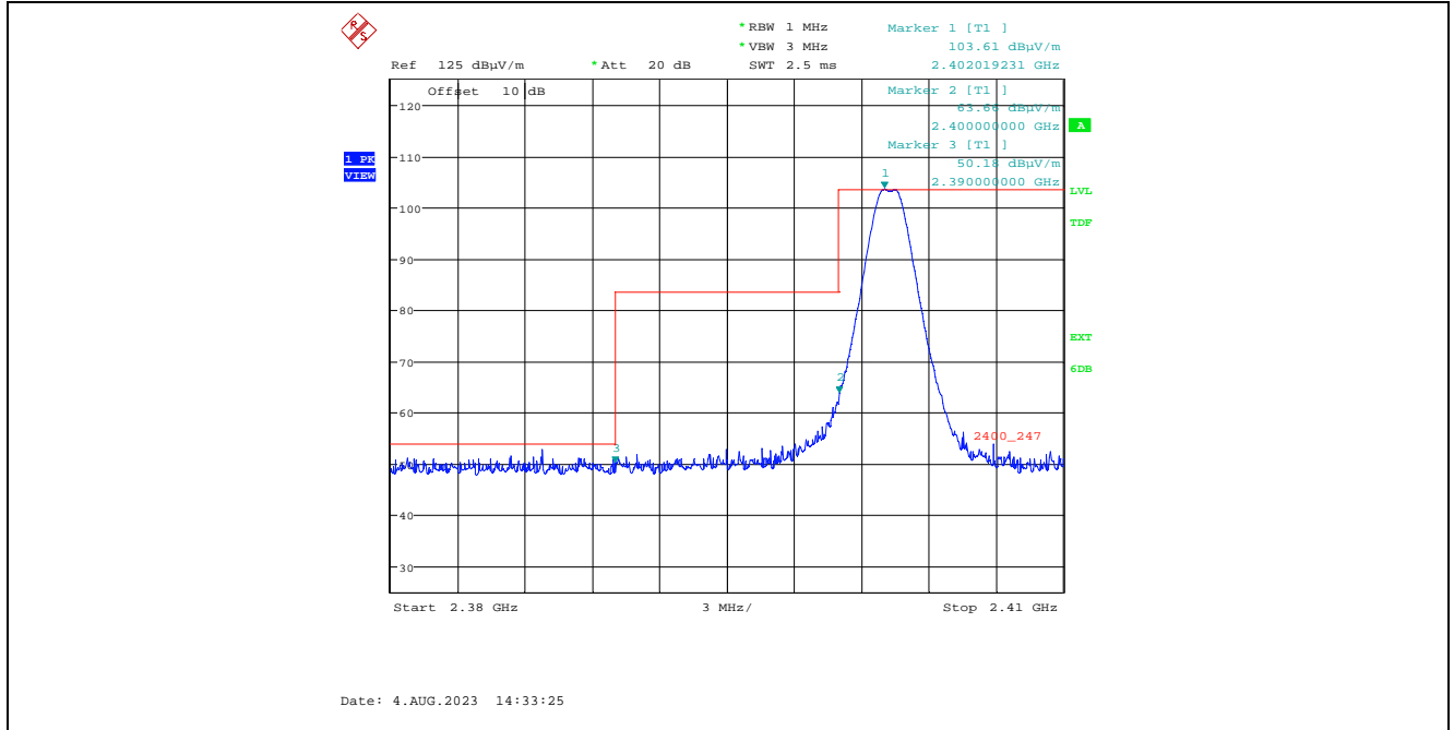
Plot 5.2.4.1.2.1. Band-Edge RF Radiated Emissions at 3 m, Vertical Polarization, Peak Low End of Frequency Band, 2402 MHz, 8 dBm Power Setting, 1 Mbps
