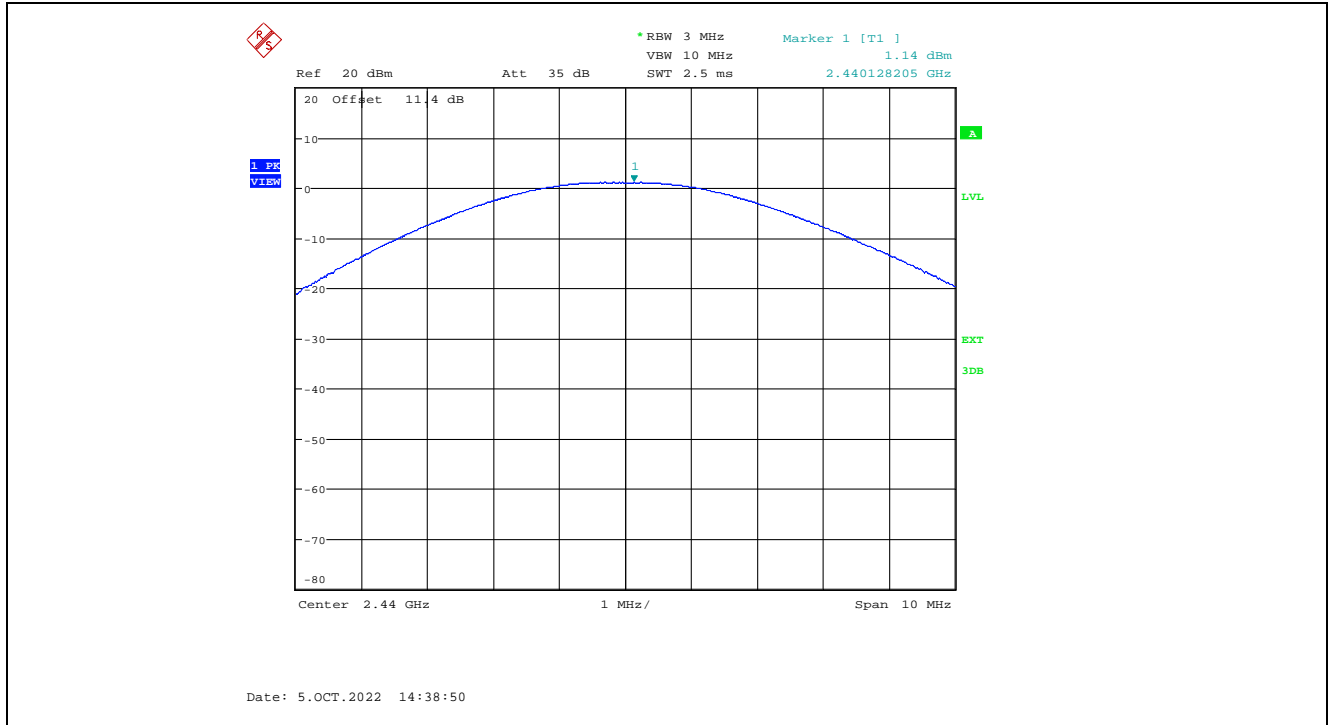
Plot 5.1.3.5. Maximum Peak Conducted Output Power, GFSK Modulation, 1 Mbps, -2 dBm Power Setting, 2440 MHz
