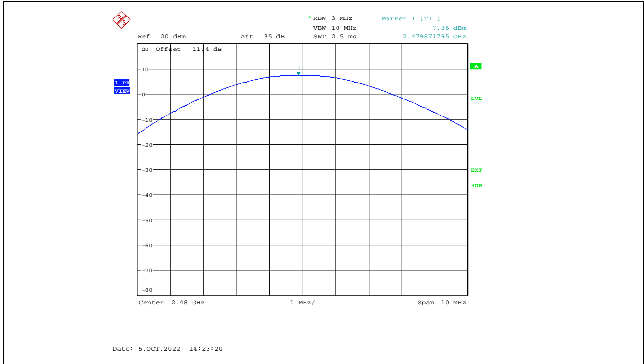
Plot 5.1.3.3. Maximum Peak Conducted Output Power, GFSK Modulation, 1 Mbps, 8 dBm Power Setting, 2480 MHz
