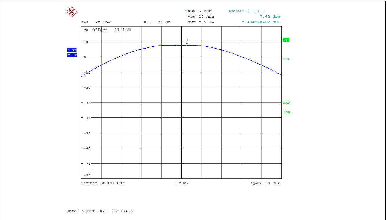
Plot 5.1.3.7. Maximum Peak Conducted Output Power, GFSK Modulation, 2 Mbps, 8 dBm Power Setting, 2404 MHz
