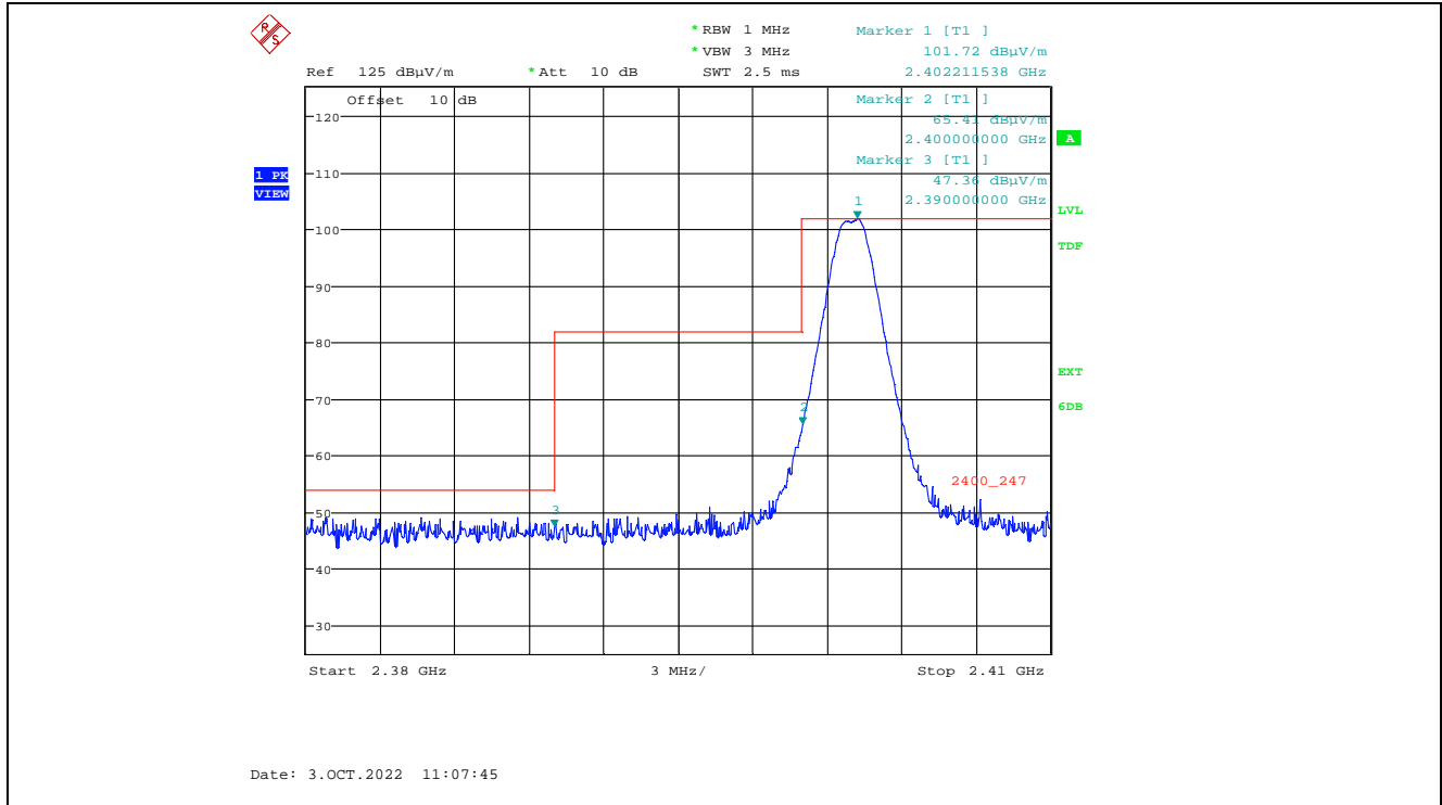
Plot 5.2.3.1.2.3. Band-Edge RF Radiated Emissions at 3 m, Horizontal Polarization, Peak Low End of Frequency Band, 2402 MHz, 8 dBm Power Setting, 1 Mbps
