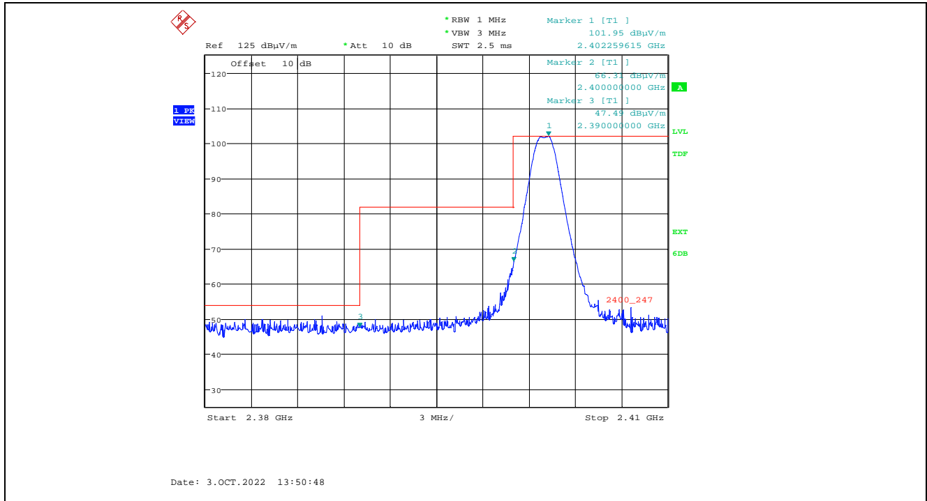
Plot 5.2.3.1.2.2. Band-Edge RF Radiated Emissions at 3 m, Vertical Polarization, Average Low End of Frequency Band, 2402 MHz, 8 dBm Power Setting, 1 Mbps
