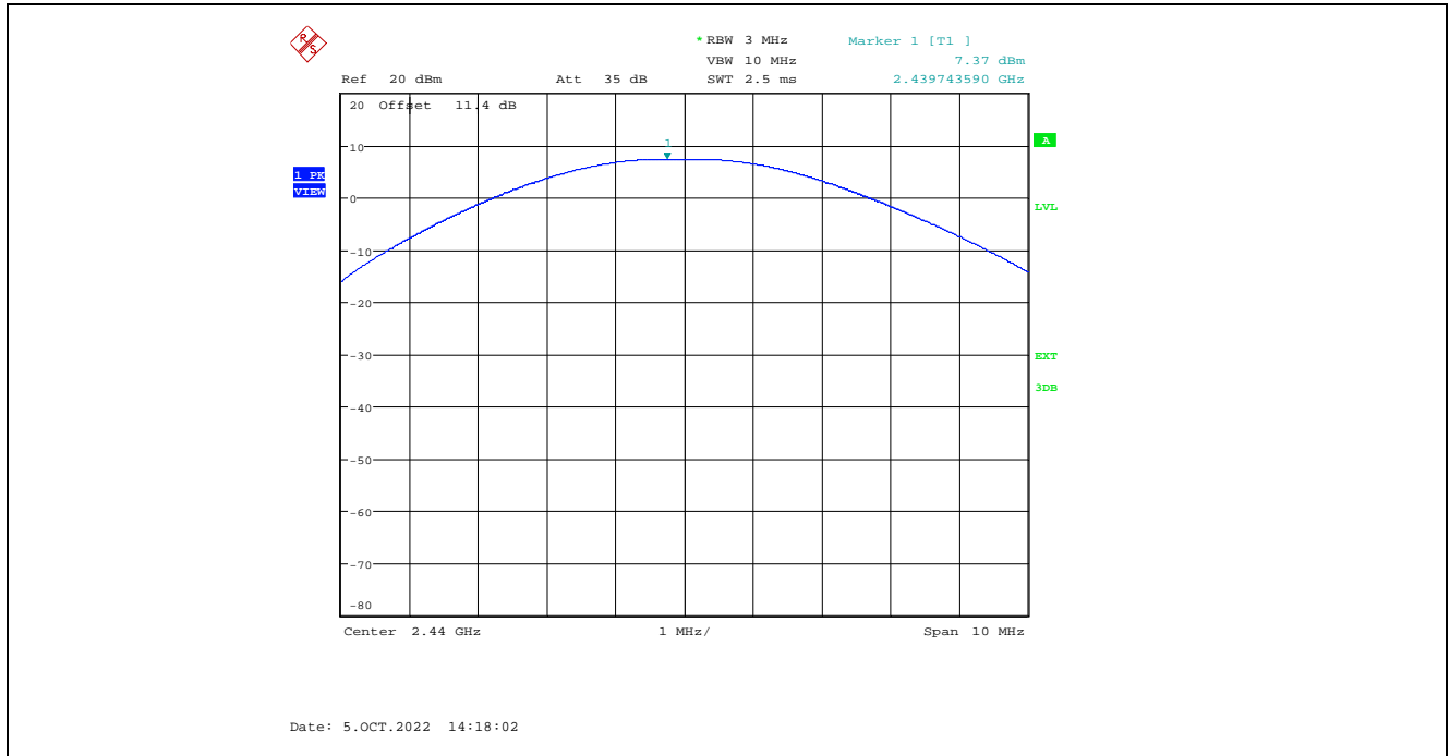
Plot 5.1.3.2. Maximum Peak Conducted Output Power, GFSK Modulation, 1 Mbps, 8 dBm Power Setting, 2440 MHz
