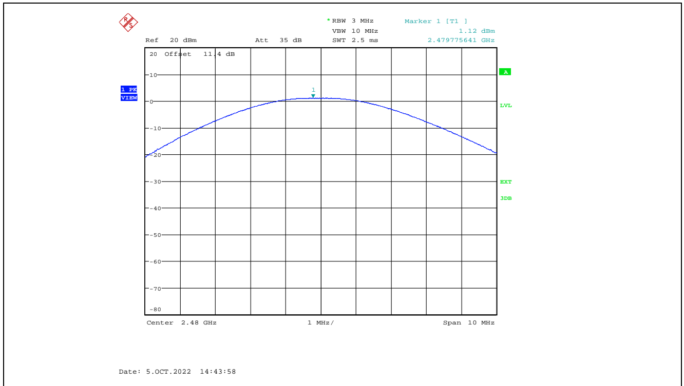
Plot 5.1.3.6. Maximum Peak Conducted Output Power, GFSK Modulation, 1 Mbps, -2 dBm Power Setting, 2480 MHz
