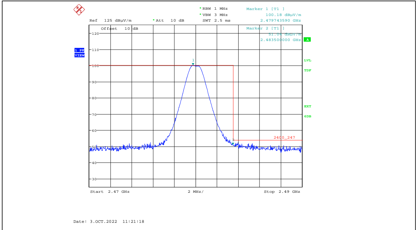
Plot 5.2.3.1.2.7. Band-Edge RF Radiated Emissions at 3 m, Horizontal Polarization, Peak High End of Frequency Band, 2480 MHz, 8 dBm Power Setting, 1 Mbps
