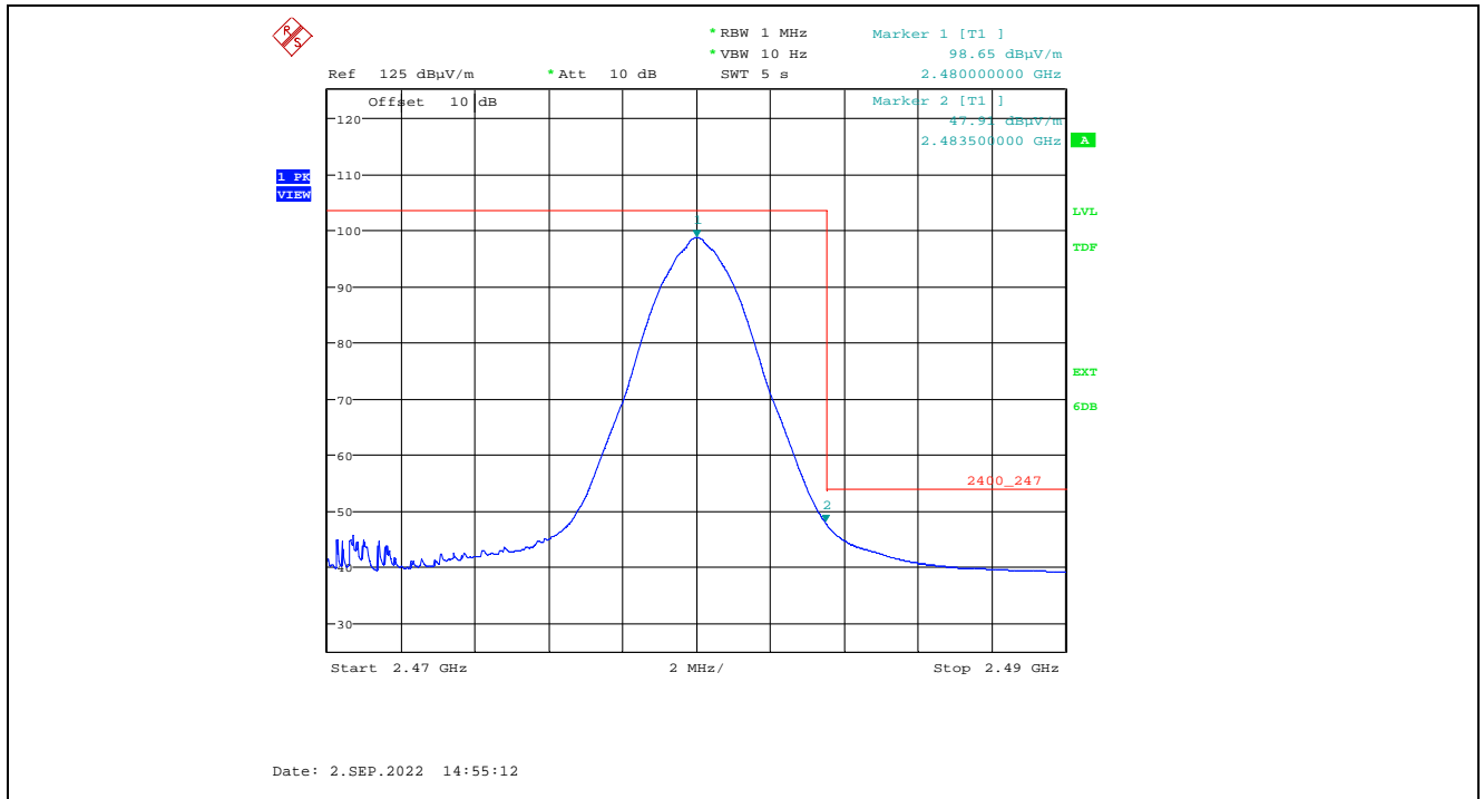
Plot 5.2.3.1.2.12. Band-Edge RF Radiated Emissions at 3 m, Horizontal Polarization, Average High End of Frequency Band, 2480 MHz, 3 dBm Power Setting
