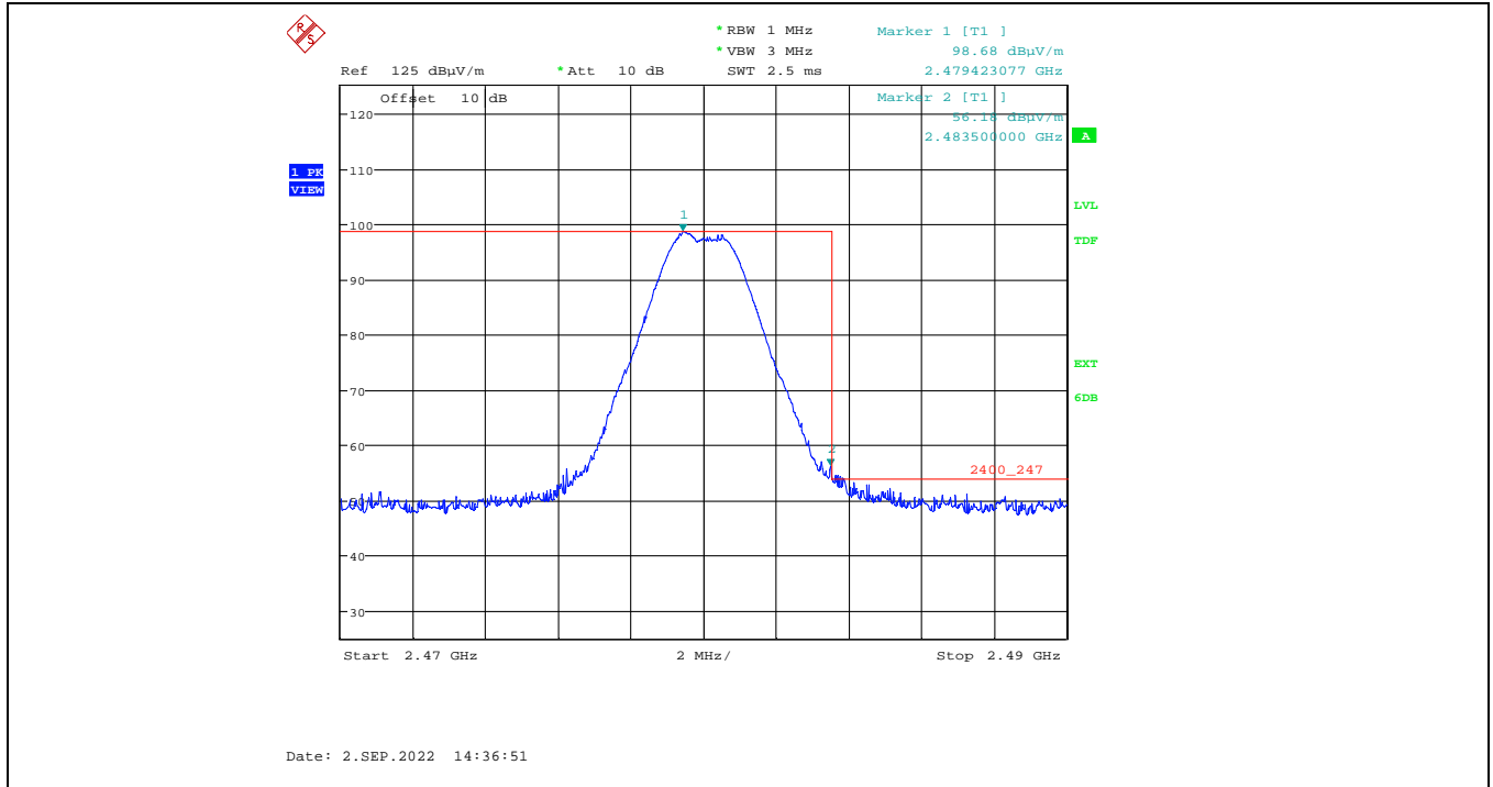
Plot 5.2.3.1.2.9. Band-Edge RF Radiated Emissions at 3 m, Vertical Polarization, Peak High End of Frequency Band, 2480 MHz, 3 dBm Power Setting
