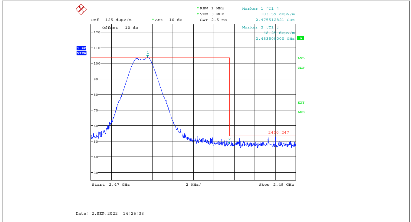
Plot 5.2.3.1.2.5. Band-Edge RF Radiated Emissions at 3 m, Vertical Polarization, Peak High End of Frequency Band, 2475 MHz, 7 dBm Power Setting
