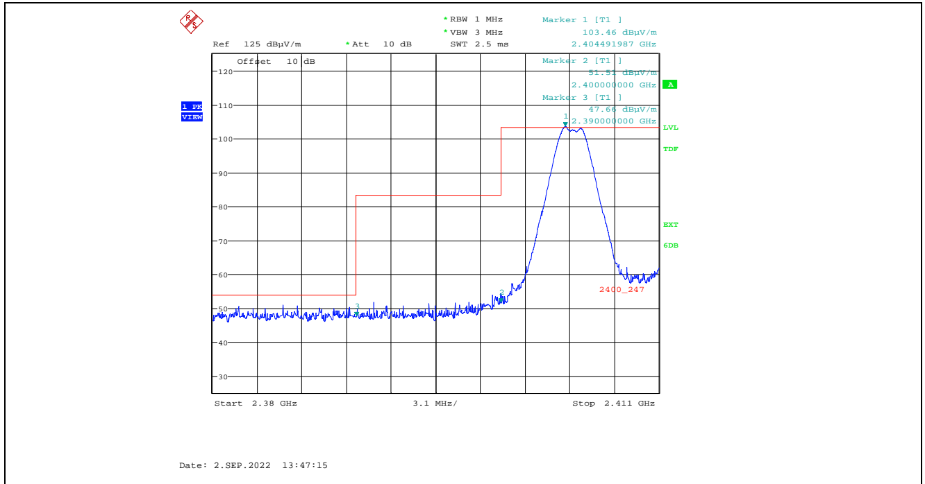
Plot 5.2.3.1.2.2. Band-Edge RF Radiated Emissions at 3 m, Vertical Polarization, Average Low End of Frequency Band, 2405 MHz, 7 dBm Power Setting
