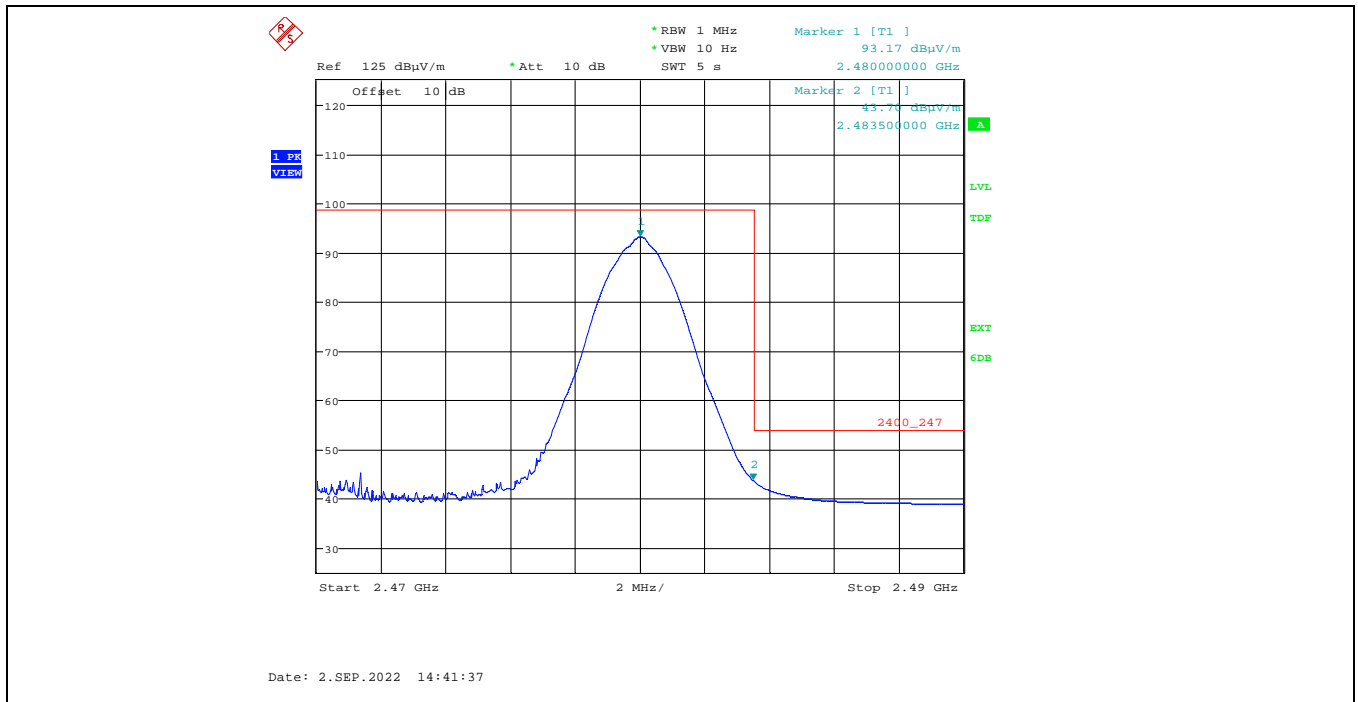
Plot 5.2.3.1.2.10. Band-Edge RF Radiated Emissions at 3 m, Vertical Polarization, Average High End of Frequency Band, 2480 MHz, 3 dBm Power Setting
