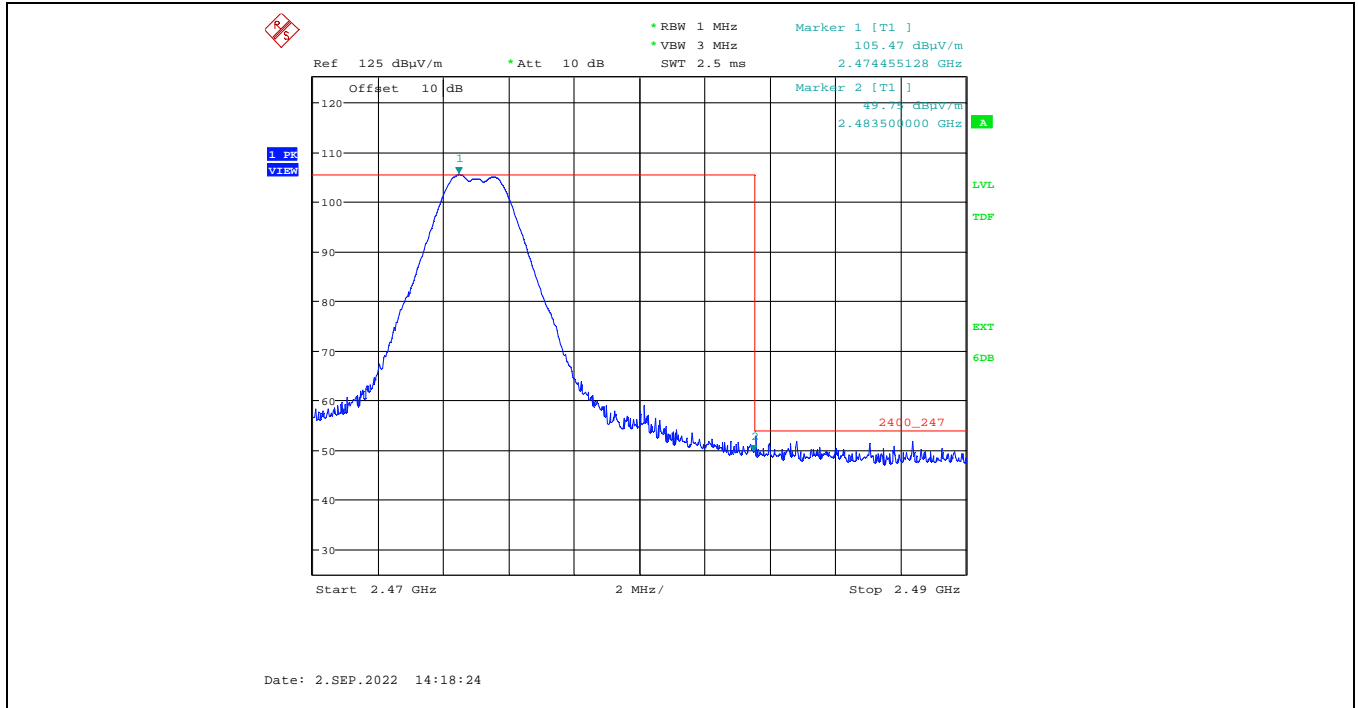
Plot 5.2.3.1.2.8. Band-Edge RF Radiated Emissions at 3 m, Horizontal Polarization, Average High End of Frequency Band, 2475 MHz, 7 dBm Power Setting
