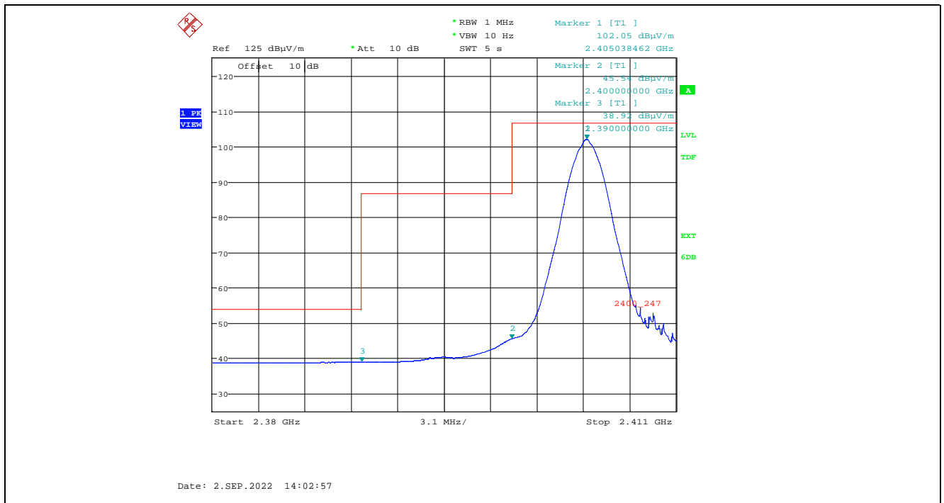
Plot 5.2.3.1.2.4. Band-Edge RF Radiated Emissions at 3 m, Horizontal Polarization, Average Low End of Frequency Band, 2405 MHz, 7 dBm Power Setting
