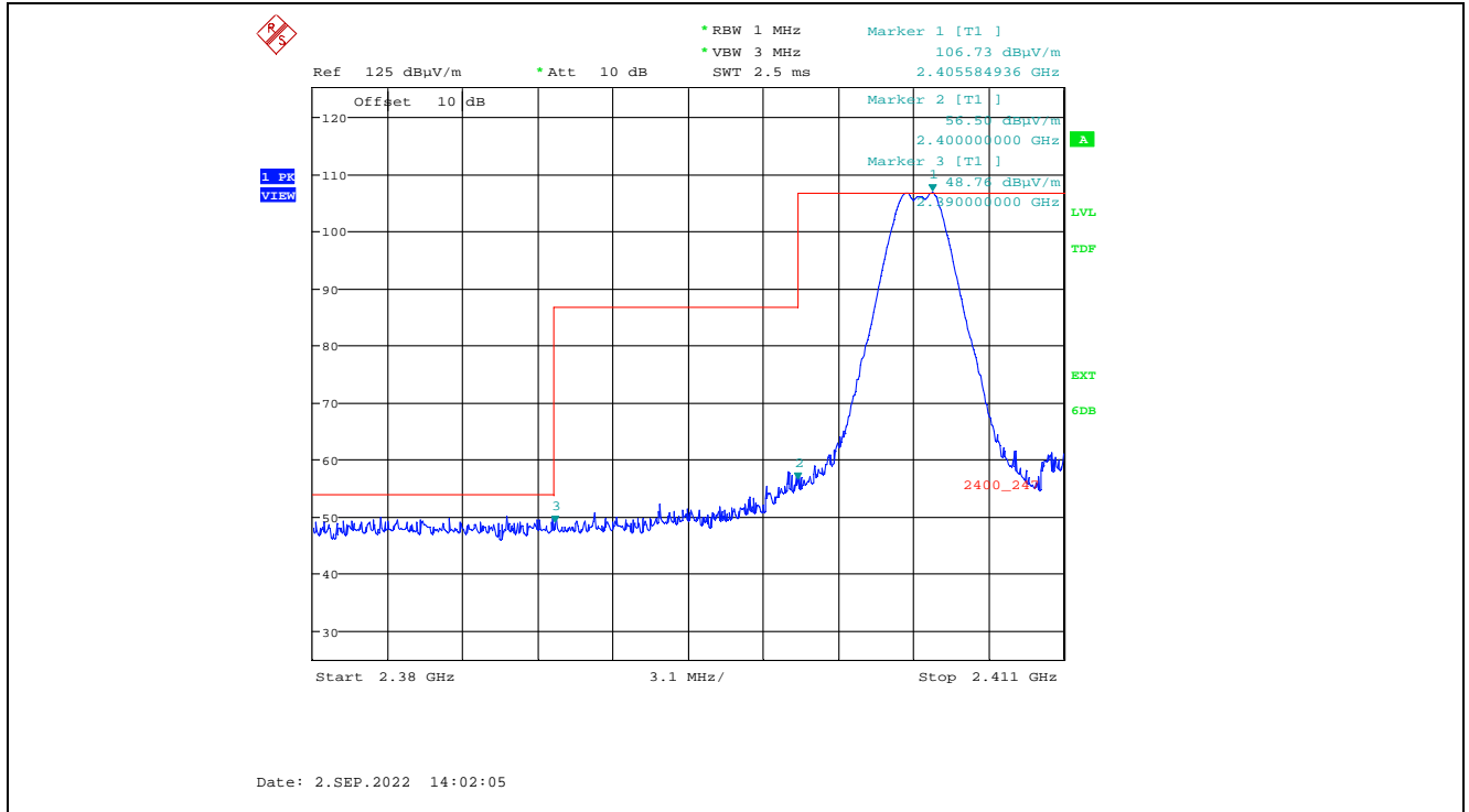
Plot 5.2.3.1.2.3. Band-Edge RF Radiated Emissions at 3 m, Horizontal Polarization, Peak Low End of Frequency Band, 2405 MHz, 7 dBm Power Setting
