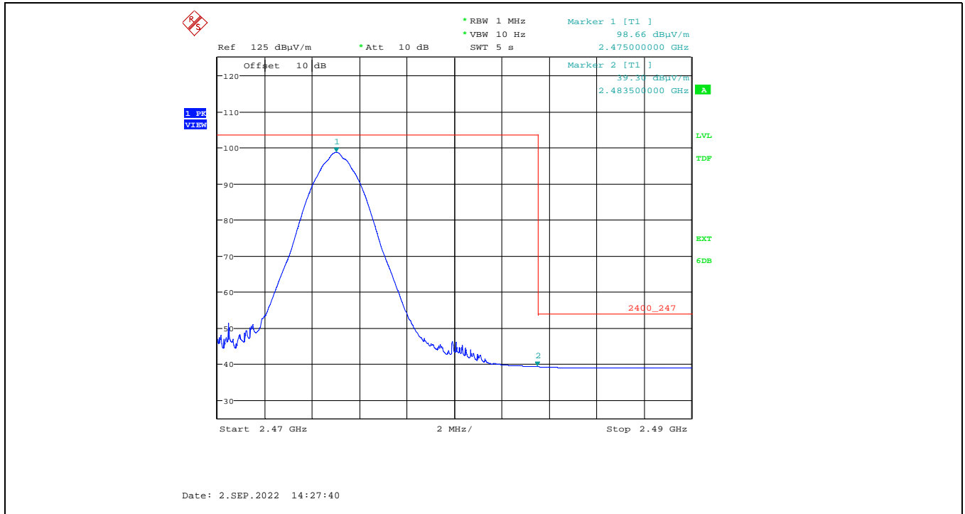
Plot 5.2.3.1.2.6. Band-Edge RF Radiated Emissions at 3 m, Vertical Polarization, Average High End of Frequency Band, 2475 MHz, 7 dBm Power Setting
