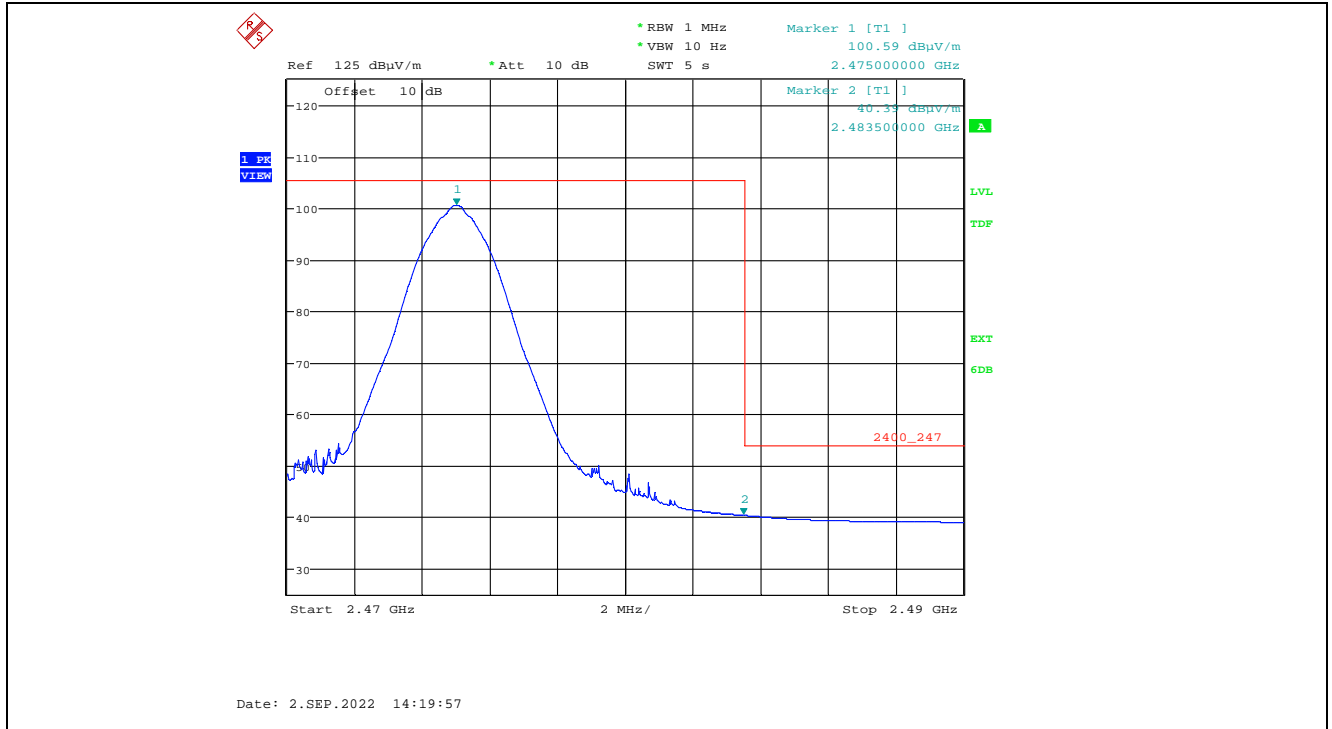
Plot 5.2.3.1.2.8. Band-Edge RF Radiated Emissions at 3 m, Horizontal Polarization, Average High End of Frequency Band, 2475 MHz, 7 dBm Power Setting
