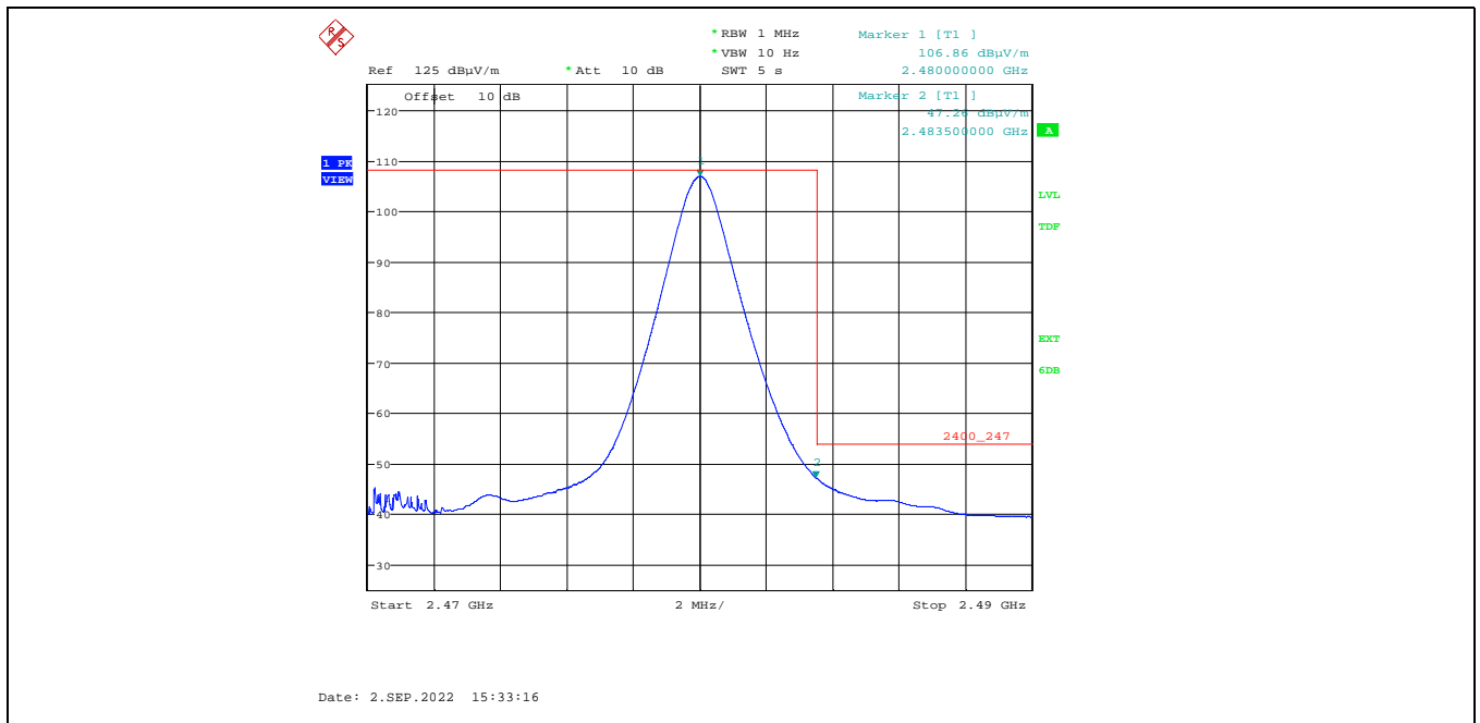
Plot 5.2.3.1.2.8. Band-Edge RF Radiated Emissions at 3 m, Horizontal Polarization, Average High End of Frequency Band, 2480 MHz, 8 dBm Power Setting, 1 Mbps
