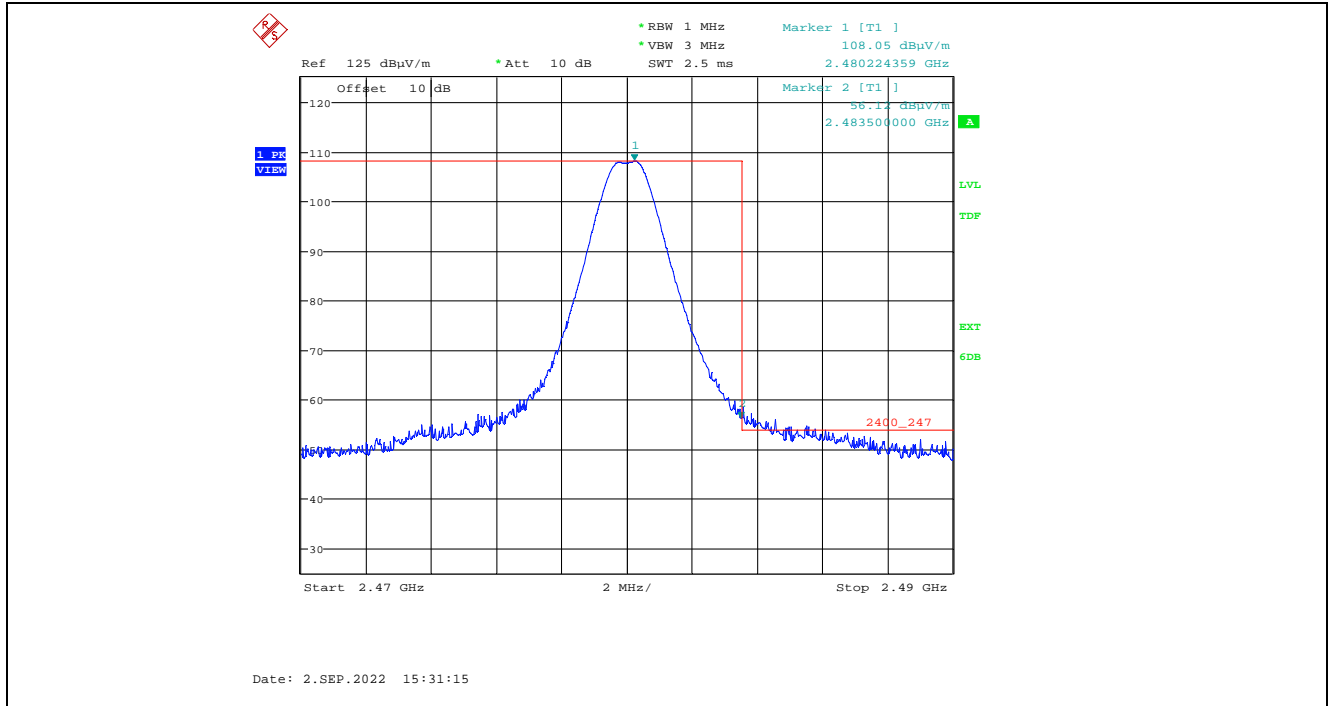
Plot 5.2.3.1.2.7. Band-Edge RF Radiated Emissions at 3 m, Horizontal Polarization, Peak High End of Frequency Band, 2480 MHz, 8 dBm Power Setting, 1 Mbps
