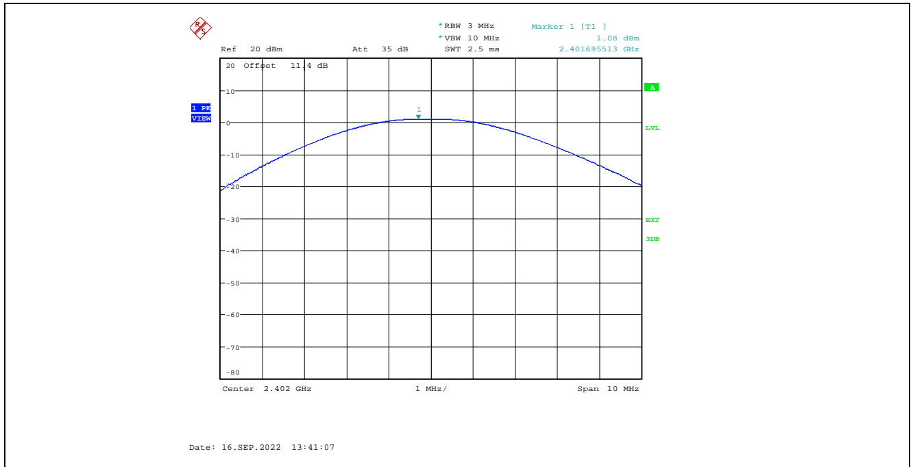
Plot 5.1.3.4. Maximum Peak Conducted Output Power, GFSK Modulation, 1 Mbps, -2 dBm Power Setting, 2402 MHz
