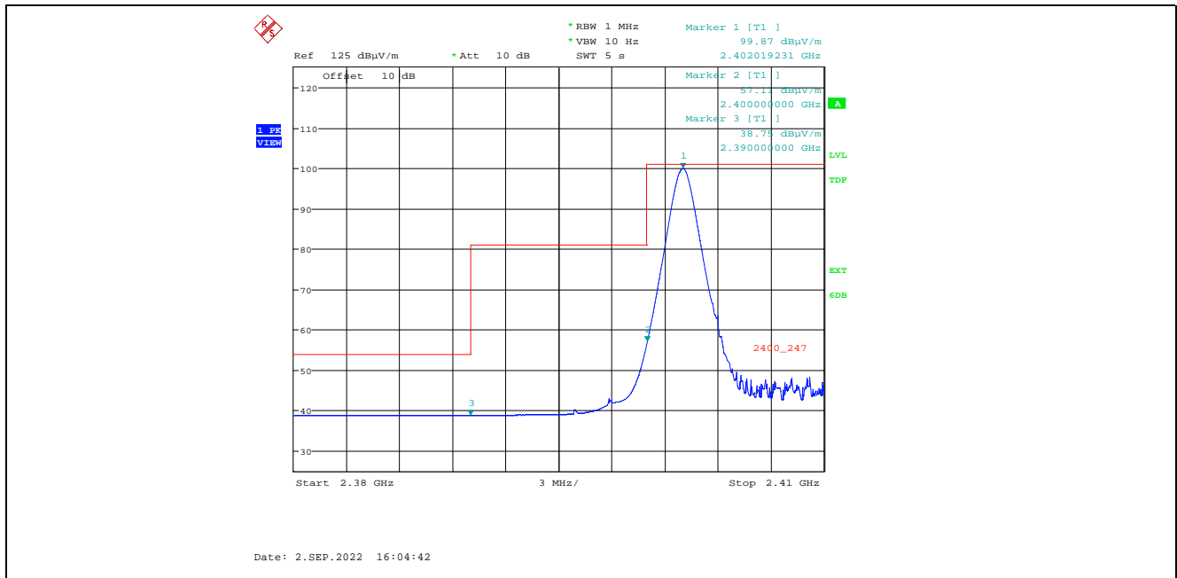
Plot 5.2.3.1.2.2. Band-Edge RF Radiated Emissions at 3 m, Vertical Polarization, Average Low End of Frequency Band, 2402 MHz, 8 dBm Power Setting, 1 Mbps
