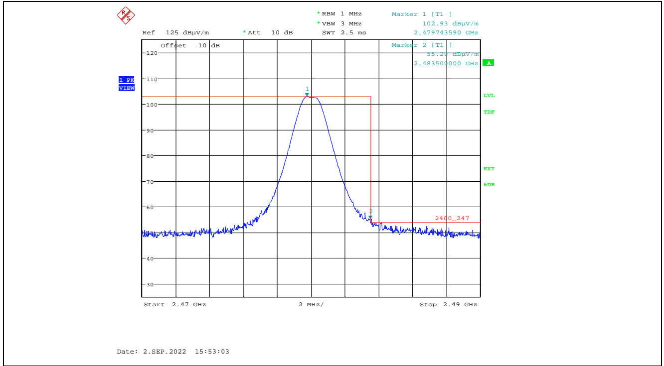
Plot 5.2.3.1.2.5. Band-Edge RF Radiated Emissions at 3 m, Vertical Polarization, Peak High End of Frequency Band, 2480 MHz, 8 dBm Power Setting, 1 Mbps
