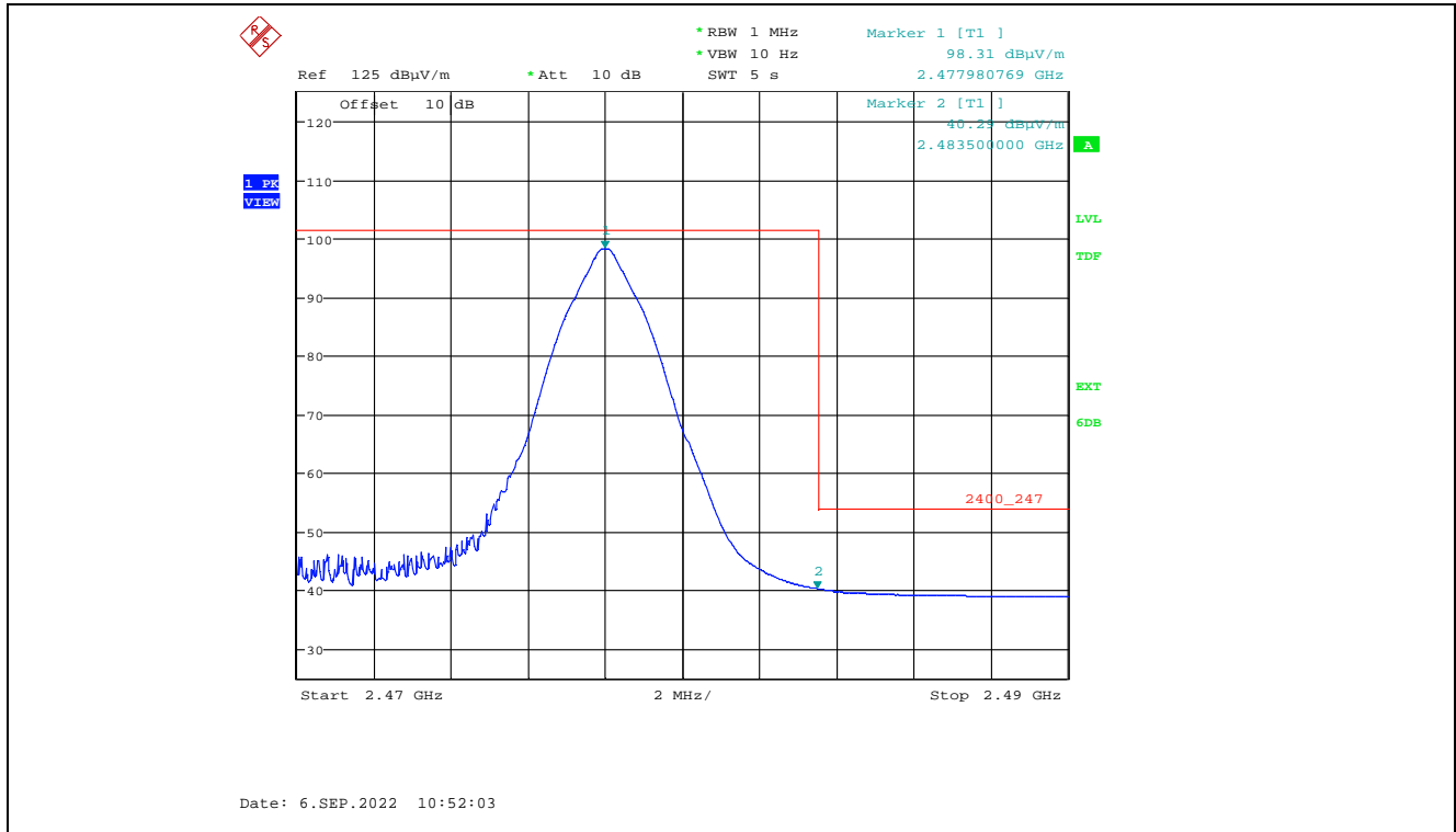
Plot 5.2.3.2.6. Band-Edge RF Radiated Emissions at 3 m, Vertical Polarization, Average High End of Frequency Band, 2478 MHz, 8 dBm Power Setting, 2 Mbps
