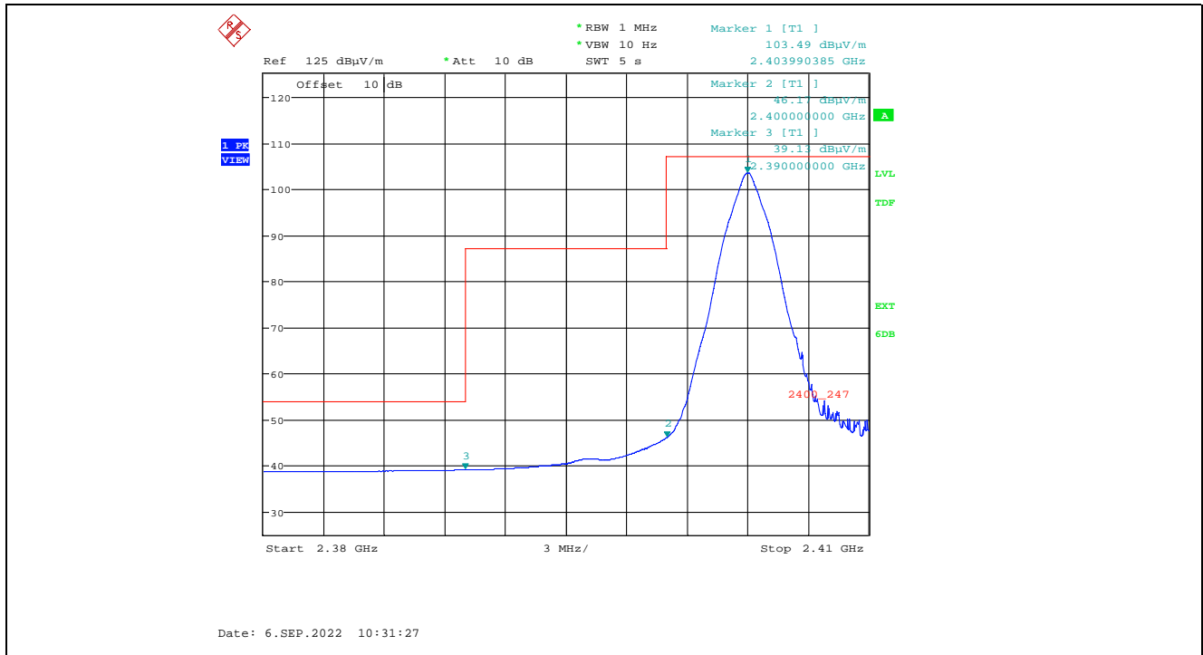
Plot 5.2.3.2.4. Band-Edge RF Radiated Emissions at 3 m, Horizontal Polarization, Average Low End of Frequency Band, 2404 MHz, 8 dBm Power Setting, 2 Mbps
