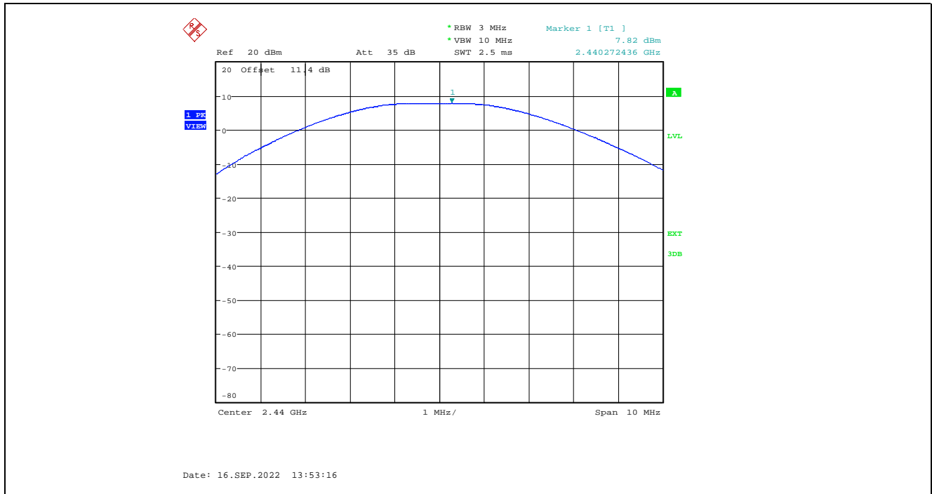
Plot 5.1.3.8. Maximum Peak Conducted Output Power, GFSK Modulation, 2 Mbps, 8 dBm Power Setting, 2440 MHz
