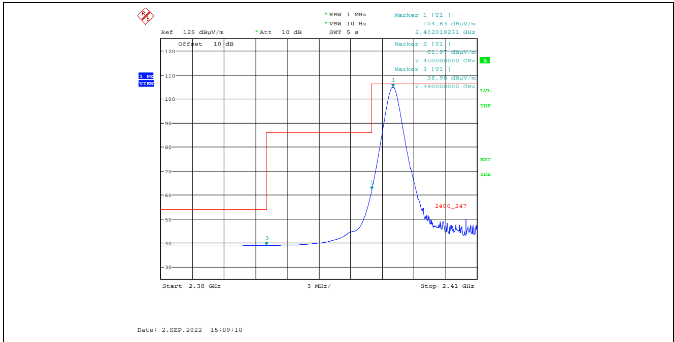
Plot 5.2.3.1.2.4. Band-Edge RF Radiated Emissions at 3 m, Horizontal Polarization, Average Low End of Frequency Band, 2402 MHz, 8 dBm Power Setting, 1 Mbps
