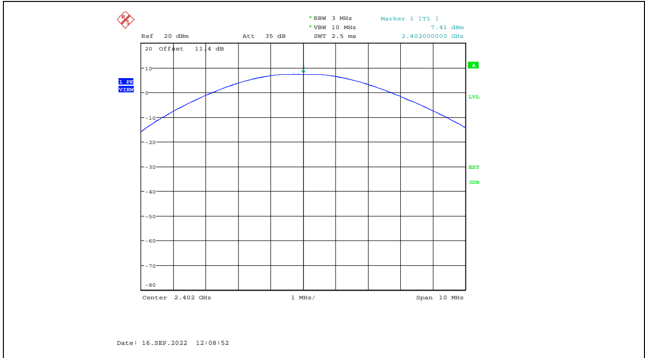
Plot 5.1.3.1. Maximum Peak Conducted Output Power, GFSK Modulation, 1 Mbps, 8 dBm Power Setting, 2402 MHz
