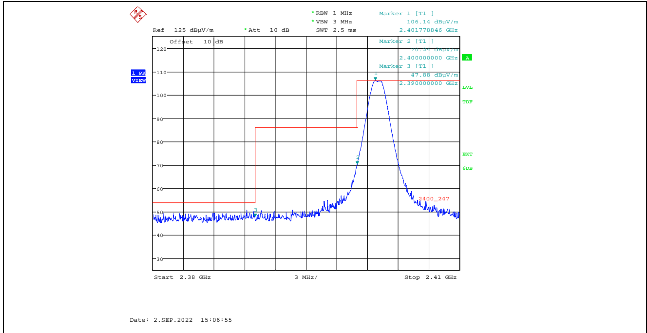
Plot 5.2.3.1.2.4. Band-Edge RF Radiated Emissions at 3 m, Horizontal Polarization, Average Low End of Frequency Band, 2402 MHz, 8 dBm Power Setting, 1 Mbps
