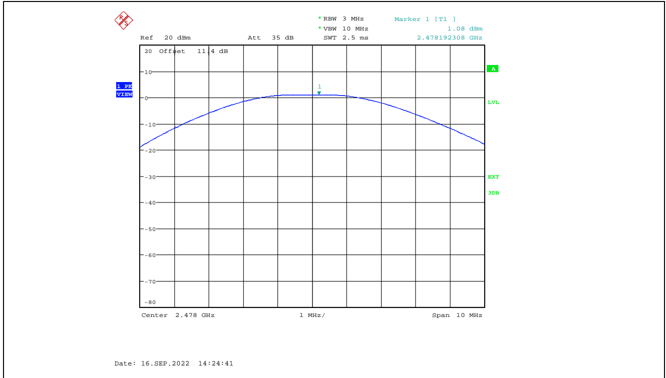
Plot 5.1.3.12. Maximum Peak Conducted Output Power, GFSK Modulation, 2 Mbps, -2 dBm Power Setting, 2478 MHz
