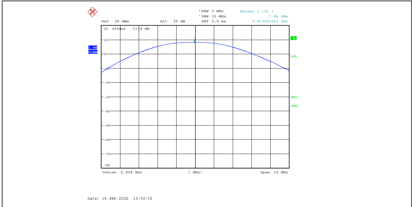
Plot 5.1.3.7. Maximum Peak Conducted Output Power, GFSK Modulation, 2 Mbps, 8 dBm Power Setting, 2404 MHz
