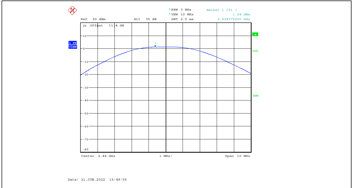
Plot 5.1.3.11. Maximum Peak Conducted Output Power, GFSK Modulation, 2 Mbps, -2 dBm Power Setting, 2440 MHz
