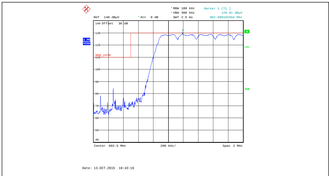
Plot 5.5.4.1.2.10. Band-Edge RF Radiated Emissions at 3 m, Horizontal Polarization Pseudorandom Hopping Mode, Low End of Frequency Band, 902.5 MHz, XB1, Data Rate at 110 kbps
