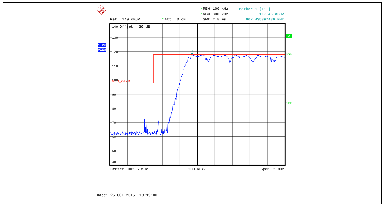
Plot 5.5.4.3.2.10. Band-Edge RF Radiated Emissions at 3 m, Horizontal Polarization Pseudorandom Hopping Mode, Low End of Frequency Band, 902.5 MHz, XB1, Data Rate at 110 kbps
