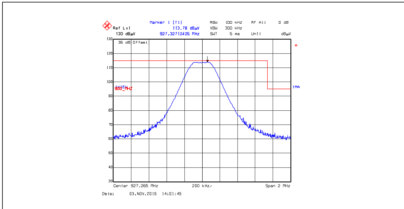
Plot 5.5.4.2.2.54. Band-Edge RF Radiated Emissions at 3 m, Horizontal Polarization Pseudorandom Hopping Mode, High End of Frequency Band, 927.265 MHz, XTCA1, Data Rate at 105kbps
