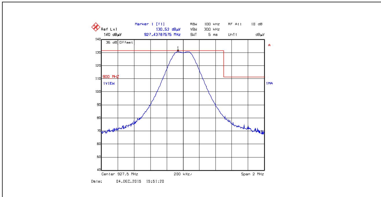
Plot 5.5.4.5.2.16. Band-Edge RF Radiated Emissions at 3 m, Vertical Polarization Pseudorandom Hopping Mode, High End of Frequency Band, 927.5 MHz, XBX1, Data Rate at 110 kbps
