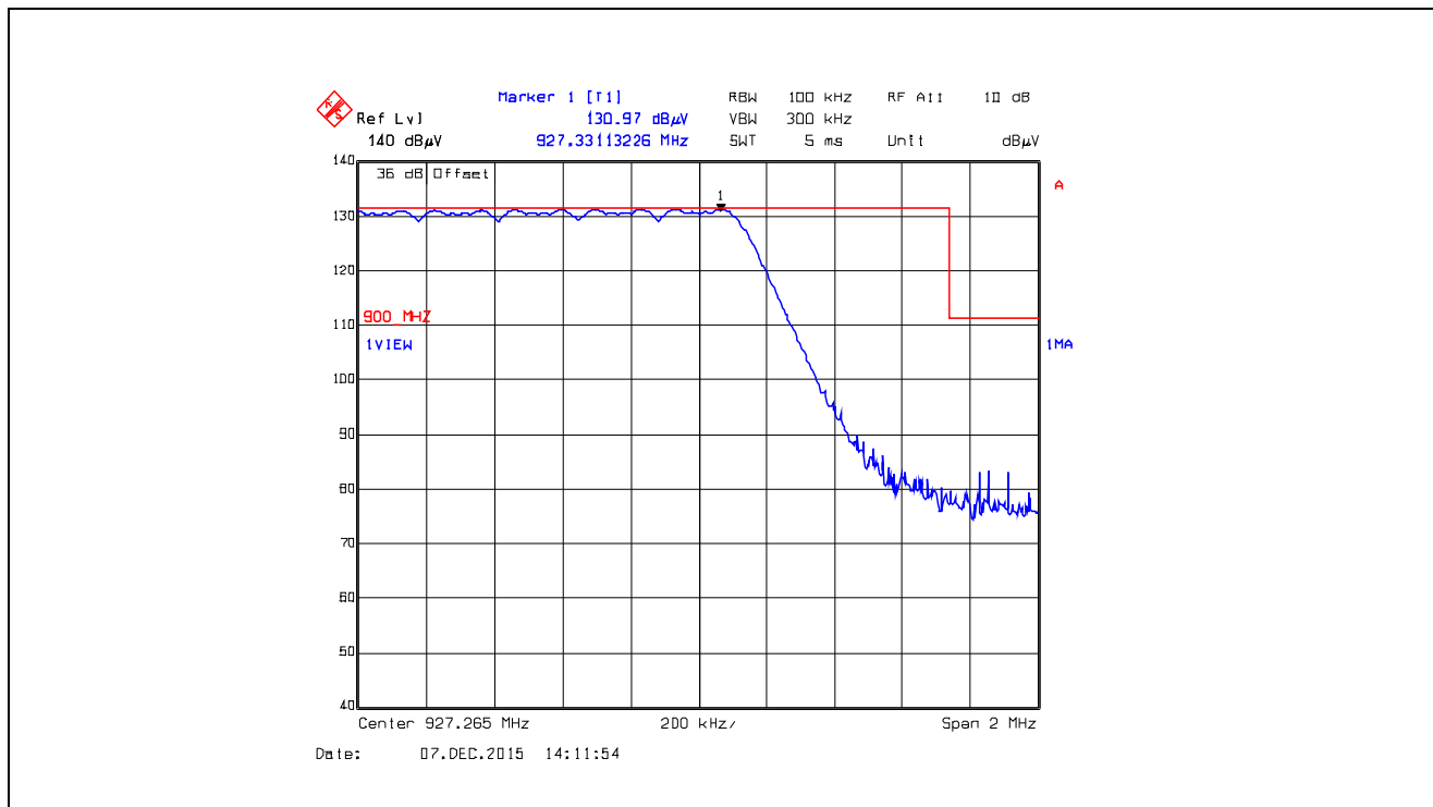
Plot 5.5.4.5.2.54. Band-Edge RF Radiated Emissions at 3 m, Horizontal Polarization Pseudorandom Hopping Mode, High End of Frequency Band, 927.265 MHz, XTCA1, Data Rate at 105kbps
