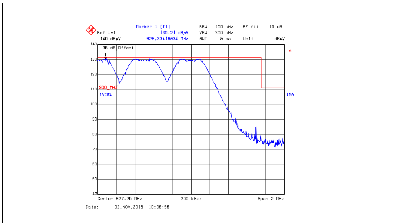
Plot 5.5.4.4.2.22. Band-Edge RF Radiated Emissions at 3 m, Horizontal Polarization Pseudorandom Hopping Mode, High End of Frequency Band, 927.25 MHz, XB2, Data Rate at 250 kbps
