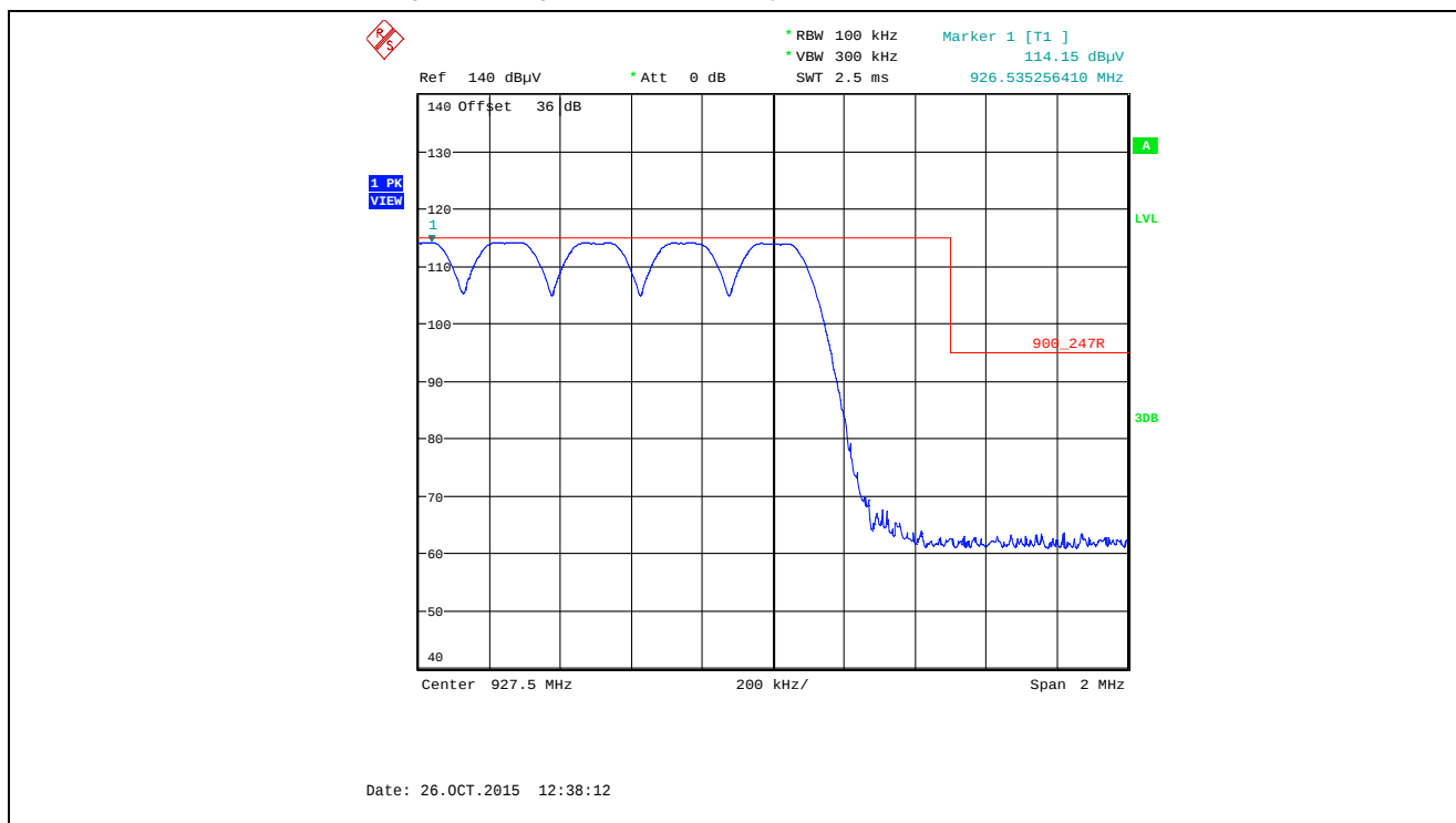
Plot 5.5.4.3.2.6. Band-Edge RF Radiated Emissions at 3 m, Horizontal Polarization Pseudorandom Hopping Mode, High End of Frequency Band, 927.5 MHz, XB0, Data Rate at 10 kbps
