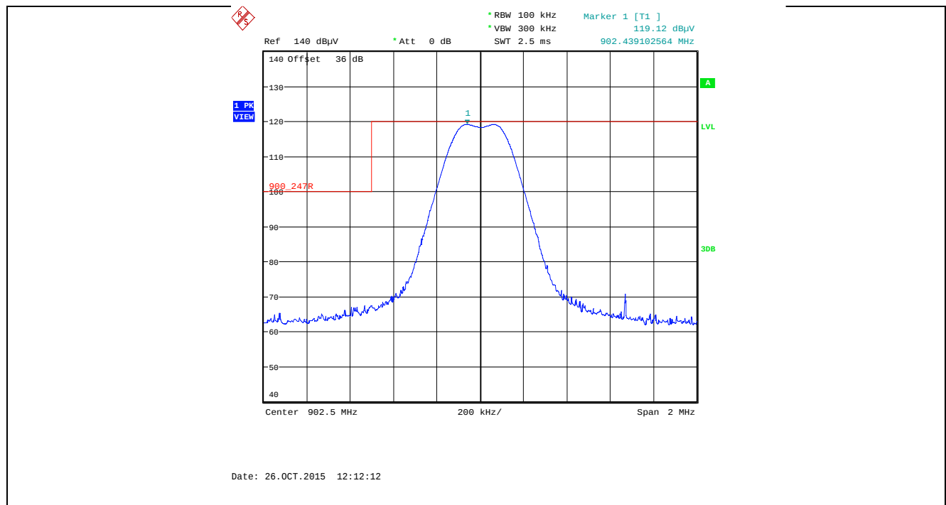
Plot 5.5.4.3.2.9. Band-Edge RF Radiated Emissions at 3 m, Horizontal Polarization Single Frequency Mode, Low End of Frequency Band, 902.5 MHz, XB1, Data Rate at 110 kbps
