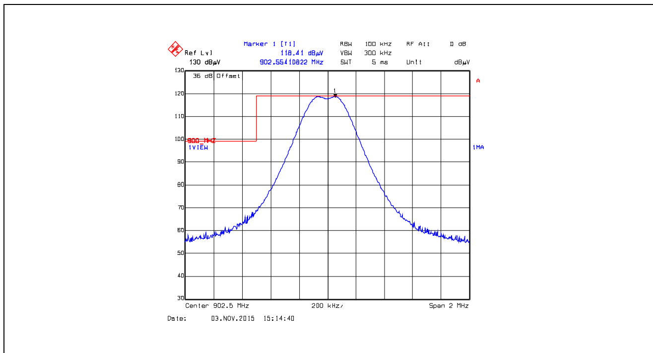
Plot 5.5.4.2.9. Band-Edge RF Radiated Emissions at 3 m, Horizontal Polarization Single Frequency Mode, Low End of Frequency Band, 902.5 MHz, XBX1, Data Rate at 110 kbps
