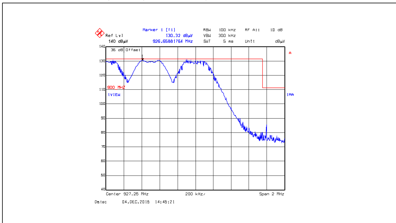
Plot 5.5.4.5.2.22. Band-Edge RF Radiated Emissions at 3 m, Horizontal Polarization Pseudorandom Hopping Mode, High End of Frequency Band, 927.25 MHz, XB2, Data Rate at 250 kbps
