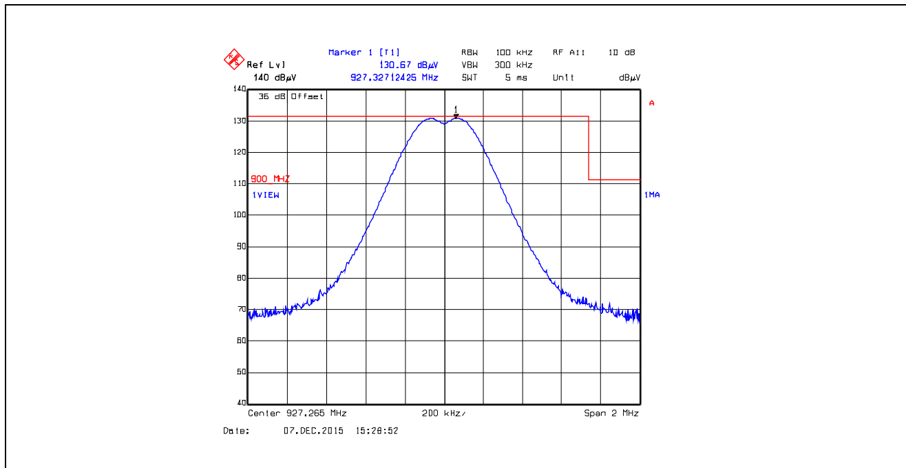
Plot 5.5.4.5.2.54. Band-Edge RF Radiated Emissions at 3 m, Horizontal Polarization Pseudorandom Hopping Mode, High End of Frequency Band, 927.265 MHz, XTCA1, Data Rate at 105kbps
