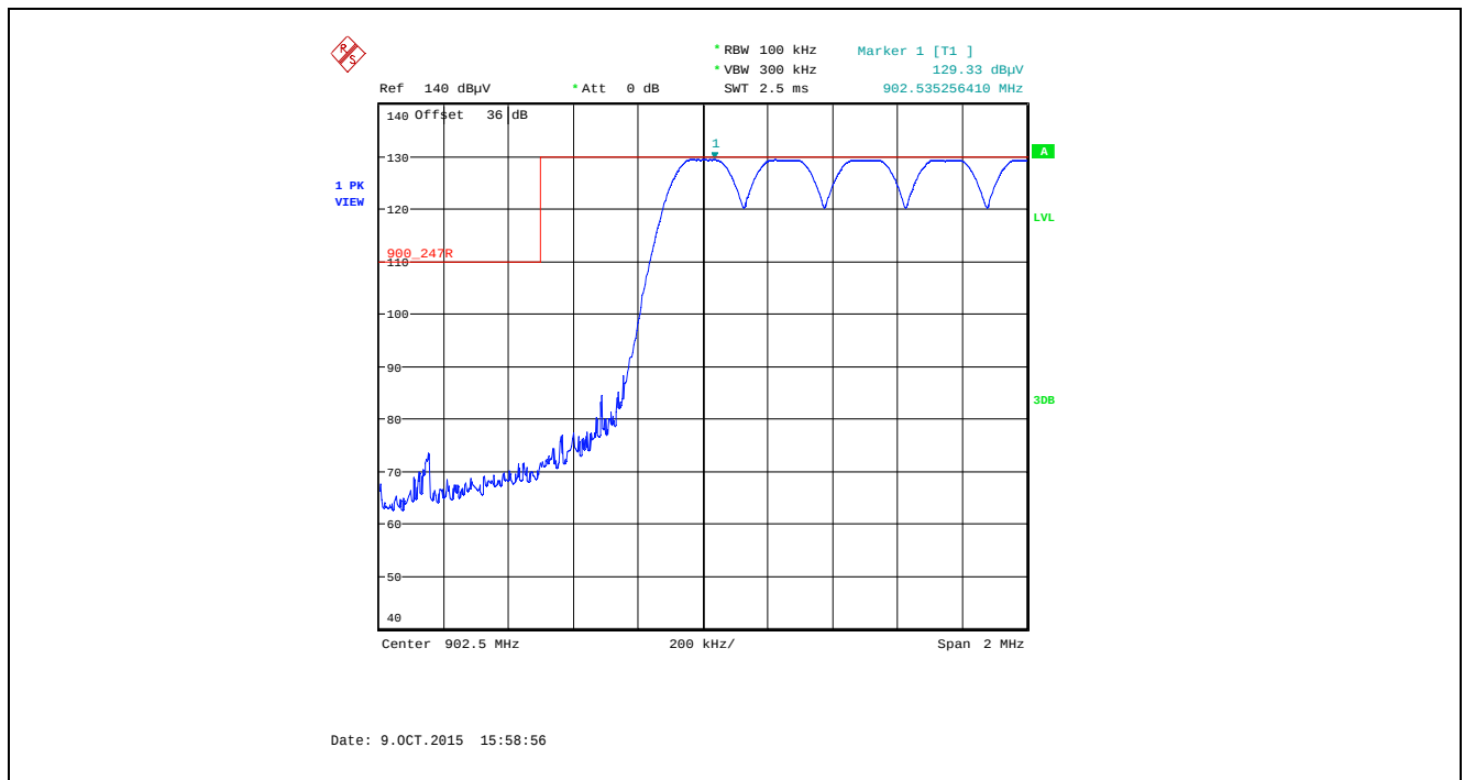
Plot 5.5.4.1.2.2. Band-Edge RF Radiated Emissions at 3 m, Horizontal Polarization Pseudorandom Hopping Mode, Low End of Frequency Band, 902.5 MHz, XB0, Data Rate at 10 kbps
