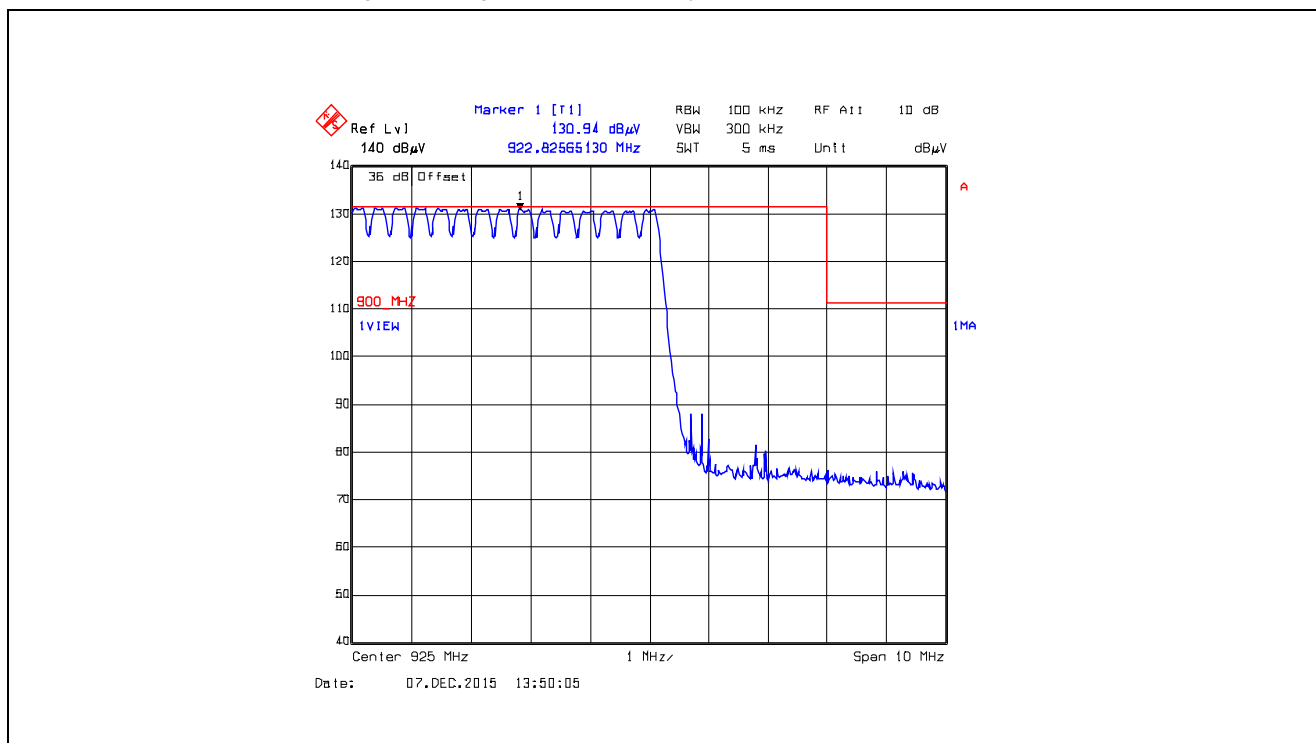
Plot 5.5.4.5.2.40. Band-Edge RF Radiated Emissions at 3 m, Vertical Polarization Pseudorandom Hopping Mode, High End of Frequency Band, 925.0 MHz, XTC1, Data Rate at 125 kbps
