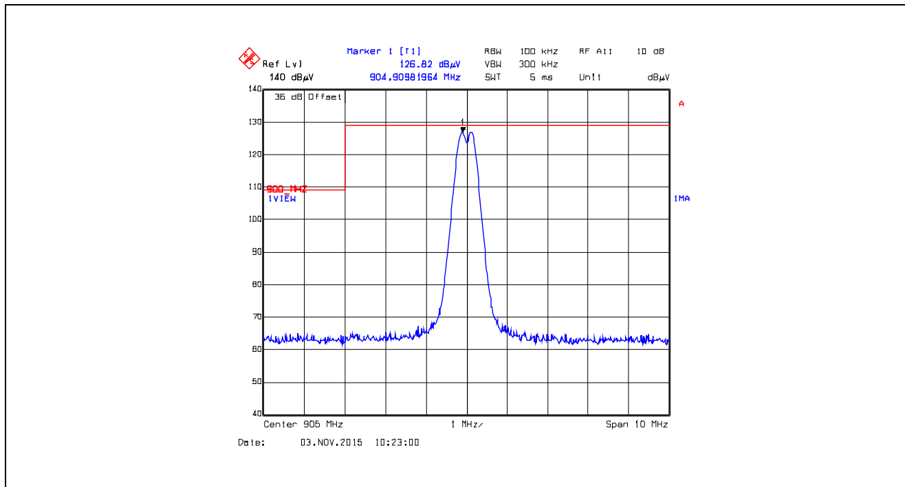
Plot 5.5.4.2.27. Band-Edge RF Radiated Emissions at 3 m, Vertical Polarization Single Frequency Mode, Low End of Frequency Band, 905.0 MHz, XTC0, Data Rate at 10 kbps
