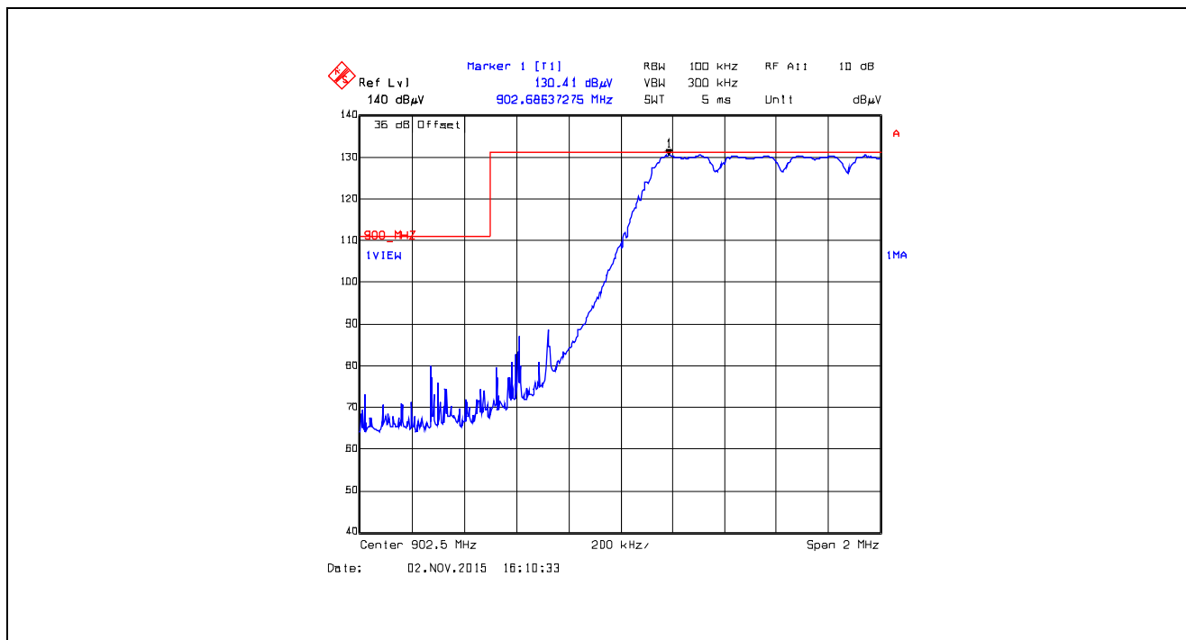
Plot 5.5.4.2.12. Band-Edge RF Radiated Emissions at 3 m, Vertical Polarization Pseudorandom Hopping Mode, Low End of Frequency Band, 902.5 MHz, XBX1, Data Rate at 110 kbps
