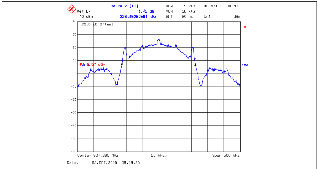
Plot 5.3.4.22. Carrier Frequency Separation, XB0, Data Rate at 10 kbps
