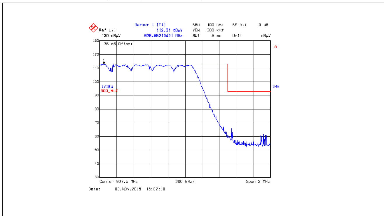
Plot 5.5.4.2.2.14. Band-Edge RF Radiated Emissions at 3 m, Horizontal Polarization Pseudorandom Hopping Mode, High End of Frequency Band, 927.5 MHz, XBX1, Data Rate at 110 kbps
