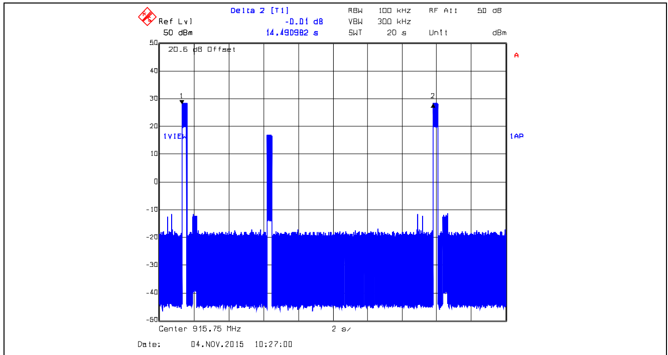
Plot 5.3.4.79. Time of Occupancy, 915.75 MHz XTCA0, Data Rate at 10 kbps Average time of occupancy = 20 \times (T_{\text{on}}) / (T_{\text{total}}) = 20 \times 0.2741483\text{s} / 14.4910\text{s} = 0.3783\text{s} < 0.4\text{s}
