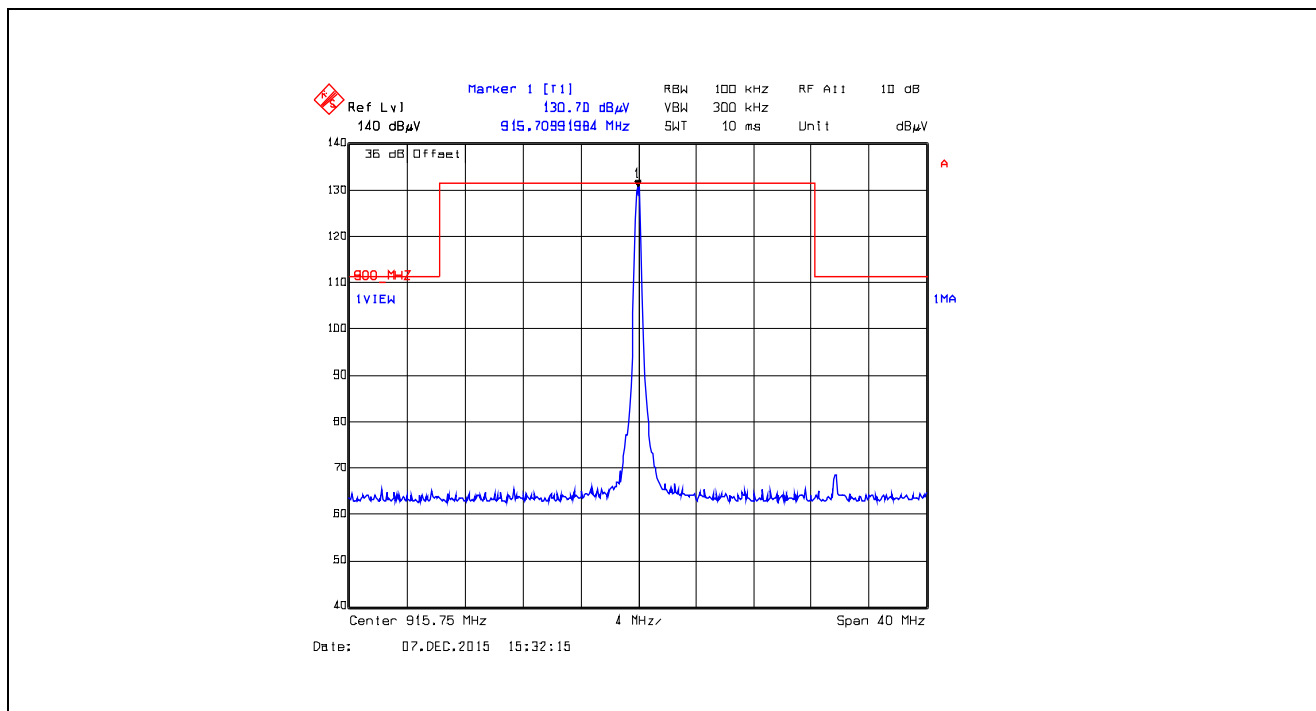
Plot 5.5.4.5.2.49. Band-Edge RF Radiated Emissions at 3 m, Horizontal Polarization Single Frequency Mode, Low End of Frequency Band, 915.75 MHz, XTCA1, Data Rate at 105kbps
