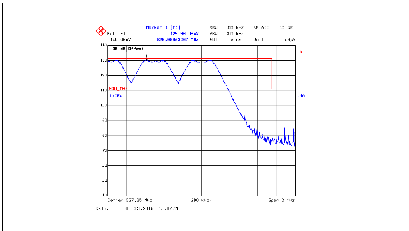
Plot 5.5.4.4.24. Band-Edge RF Radiated Emissions at 3 m, Vertical Polarization Pseudorandom Hopping Mode, High End of Frequency Band, 927.25 MHz, XB2, Data Rate at 250 kbps
