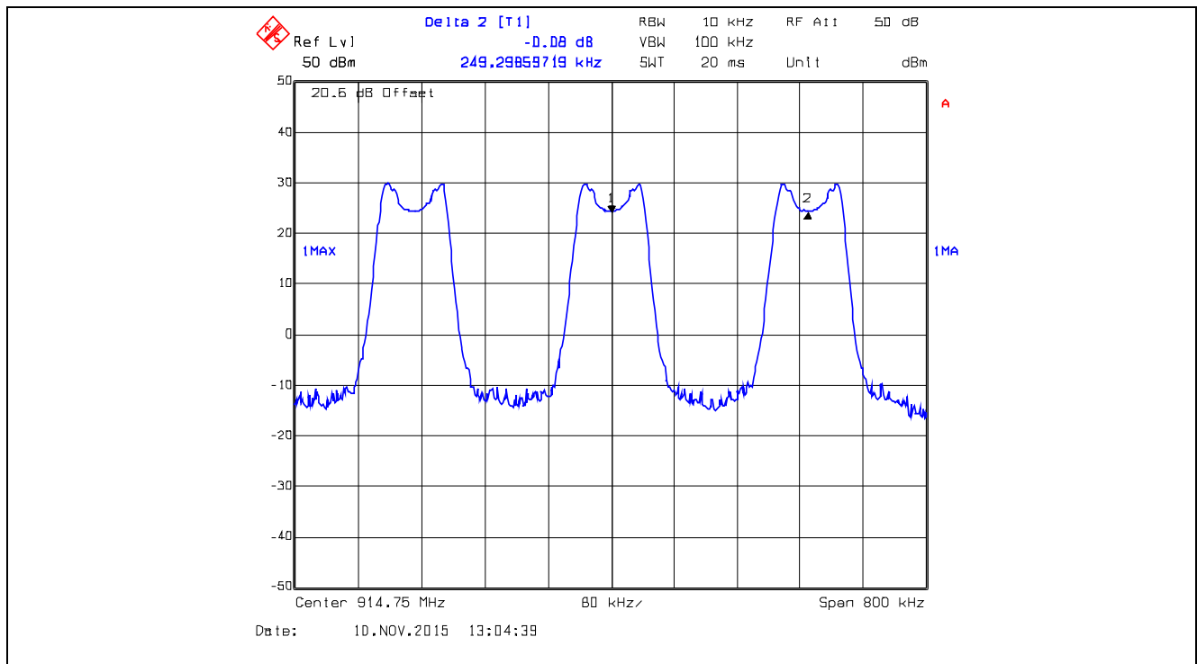
Plot 5.3.4.22. Carrier Frequency Separation, XB0, Data Rate at 10 kbps
