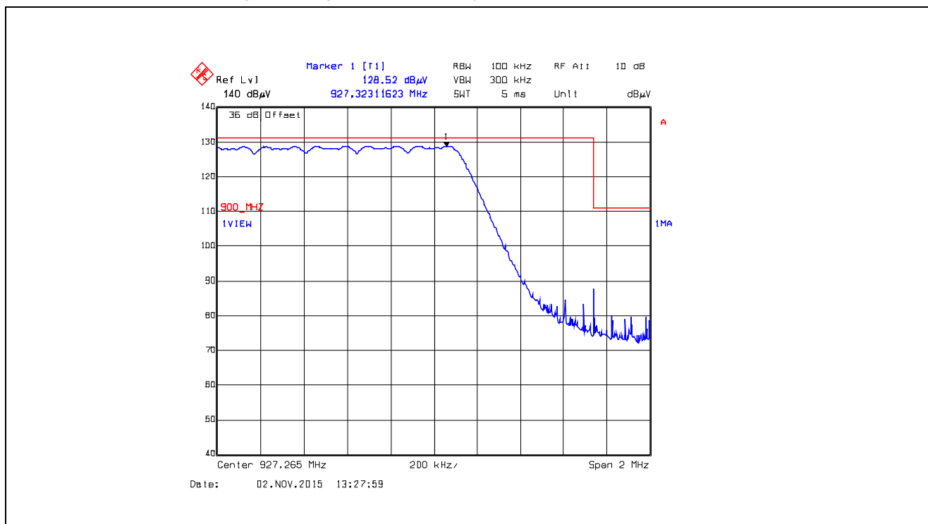
Plot 5.5.4.4.2.54. Band-Edge RF Radiated Emissions at 3 m, Horizontal Polarization Pseudorandom Hopping Mode, High End of Frequency Band, 927.265 MHz, XTCA1, Data Rate at 105kbps
