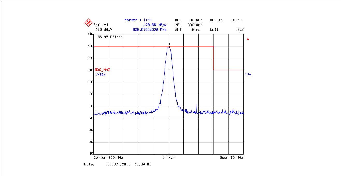
Plot 5.5.4.4.2.40. Band-Edge RF Radiated Emissions at 3 m, Vertical Polarization Pseudorandom Hopping Mode, High End of Frequency Band, 925.0 MHz, XTC1, Data Rate at 125 kbps
