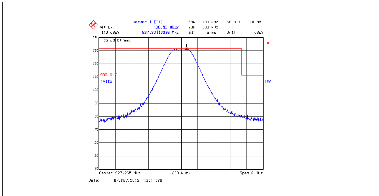
Plot 5.5.4.5.2.56. Band-Edge RF Radiated Emissions at 3 m, Vertical Polarization Pseudorandom Hopping Mode, High End of Frequency Band, 927.265 MHz, XTCA1, Data Rate at 105kbps
