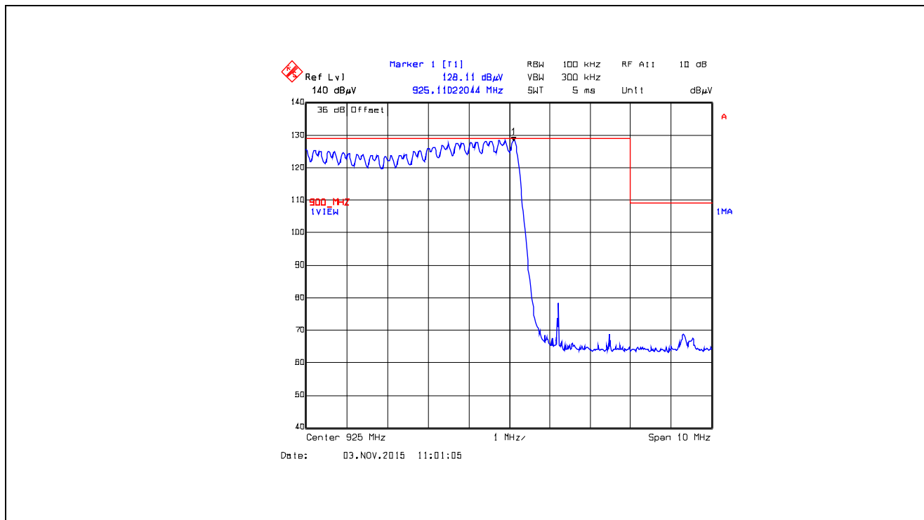
Plot 5.5.4.2.2.32. Band-Edge RF Radiated Emissions at 3 m, Vertical Polarization Pseudorandom Hopping Mode, High End of Frequency Band, 925.0 MHz, XTC0, Data Rate at 10 kbps
