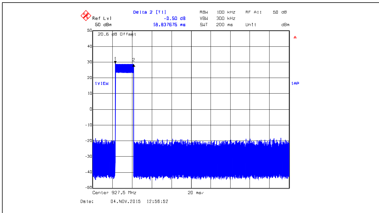
Plot 5.3.4.58. Time of Occupancy, 927.5 MHz, XBX1, Data Rate at 110 kbps Dwell Time @ 927.5 MHz = 18.8377 ms
