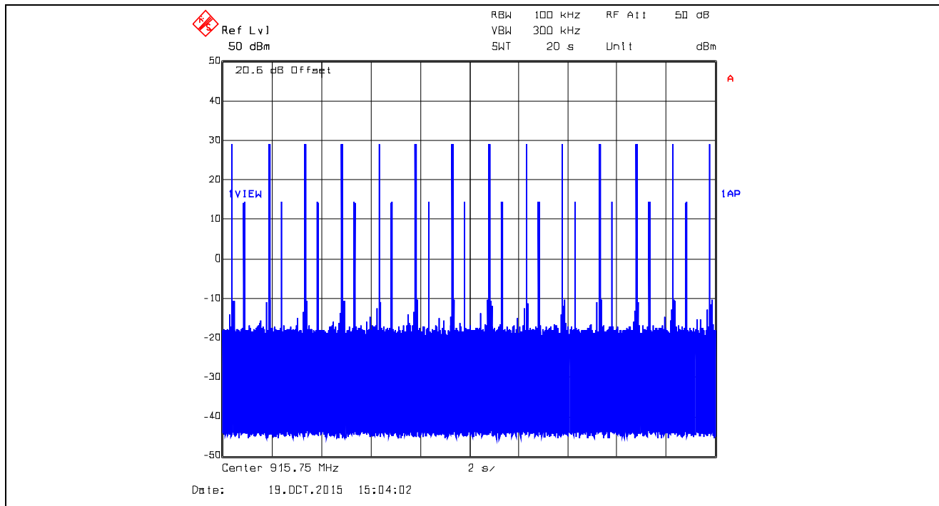
Plot 5.3.4.85. Time of Occupancy, 915.75 MHz XTCA1, Data Rate at 105 kbps Average time of occupancy = (Dwell Time) x (number of hops) = 27.6553 ms x 14 = 387.1742 ms < 0.4 sec within 20 sec
