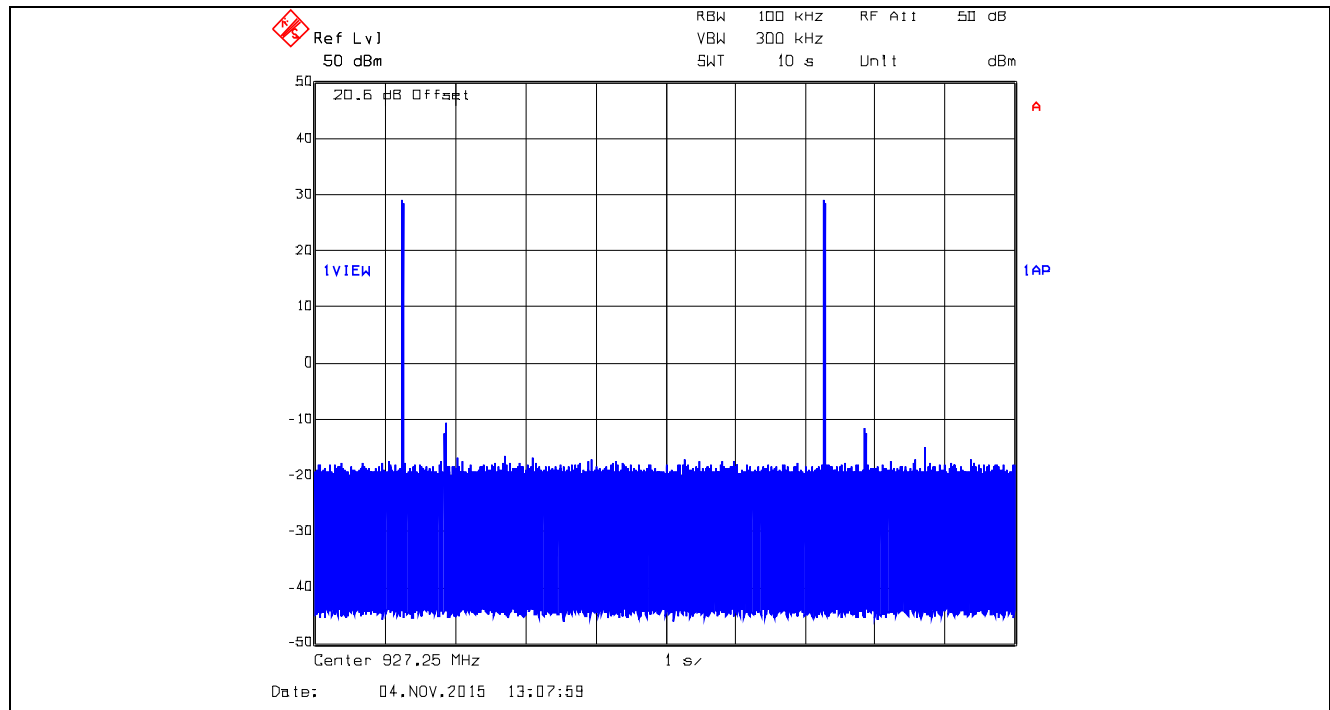
Plot 5.3.4.65. Time of Occupancy, 927.25 MHz, XB2, Data Rate at 250 kbps Average time of occupancy = (Dwell Time) x (number of hops) = 10.4208 ms x 2 = 20.8416 ms < 0.4 sec within 10 sec
