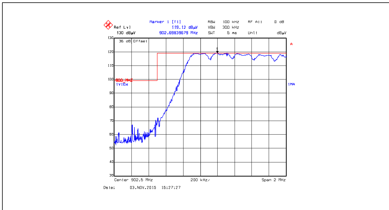
Plot 5.5.4.2.10. Band-Edge RF Radiated Emissions at 3 m, Horizontal Polarization Pseudorandom Hopping Mode, Low End of Frequency Band, 902.5 MHz, XBX1, Data Rate at 110 kbps
