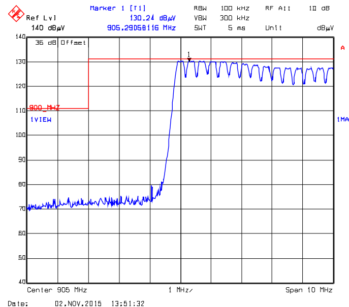
Plot 5.5.4.4.2.34. Band-Edge RF Radiated Emissions at 3 m, Horizontal Polarization Pseudorandom Hopping Mode, Low End of Frequency Band, 905.0 MHz, XTC1, Data Rate at 125 kbps
