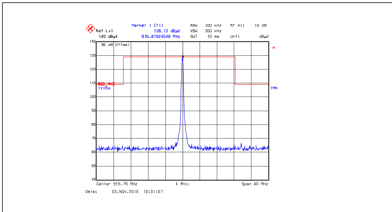
Plot 5.5.4.2.43. Band-Edge RF Radiated Emissions at 3 m, Vertical Polarization Single Frequency Mode, Low End of Frequency Band, 915.75 MHz, XTCA0, Data Rate at 10 kbps
