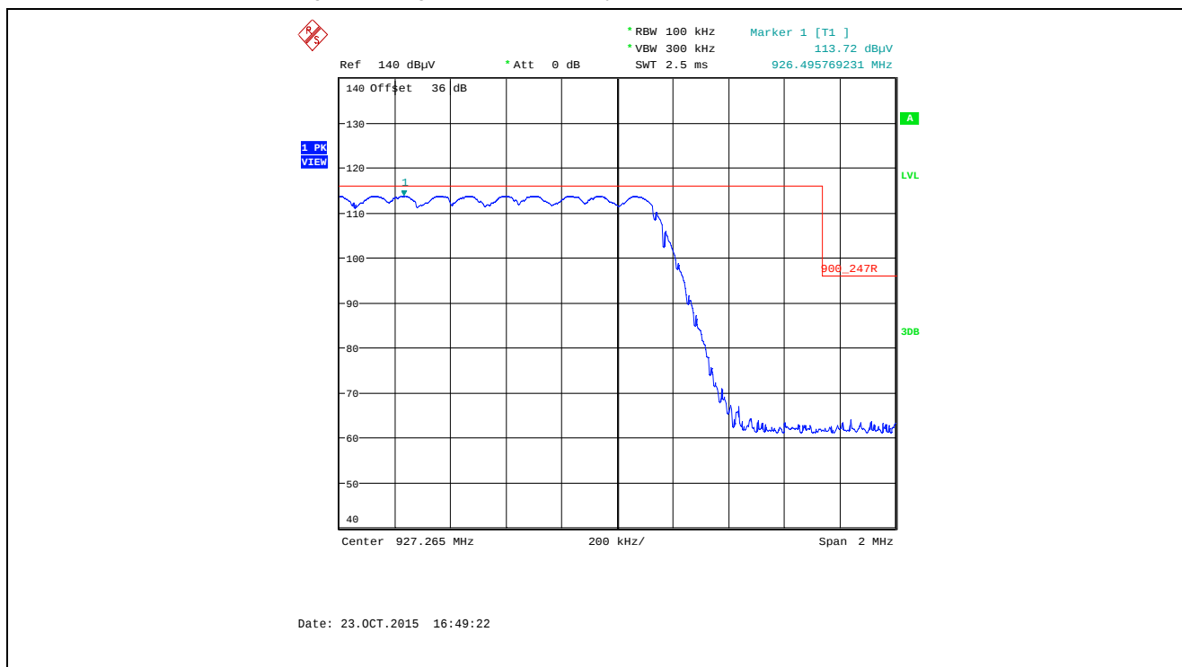
Plot 5.5.4.3.2.46. Band-Edge RF Radiated Emissions at 3 m, Horizontal Polarization Pseudorandom Hopping Mode, High End of Frequency Band, 927.265 MHz, XTCA0, Data Rate at 10 kbps
