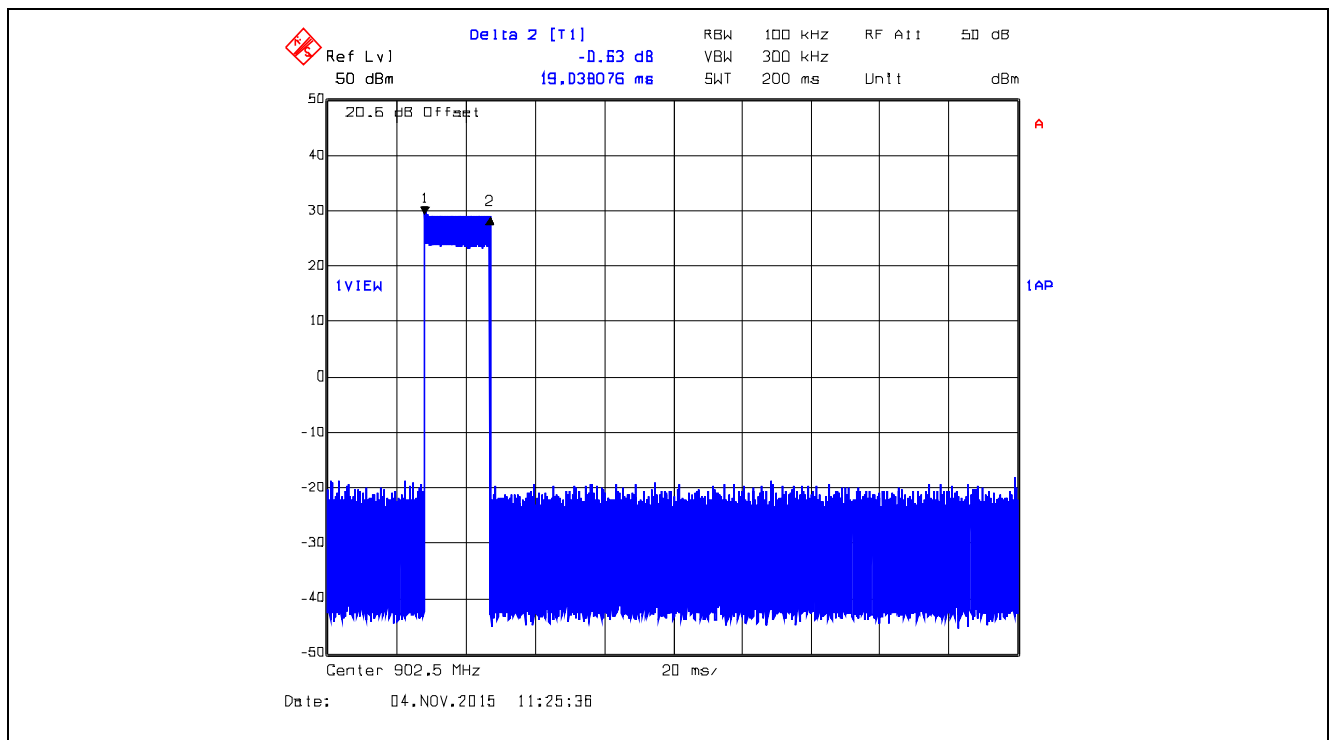
Plot 5.3.4.54. Time of Occupancy, 902.5 MHz, XB1, Data Rate at 110 kbps Dwell Time @ 902.5 MHz = 19.0381 ms
