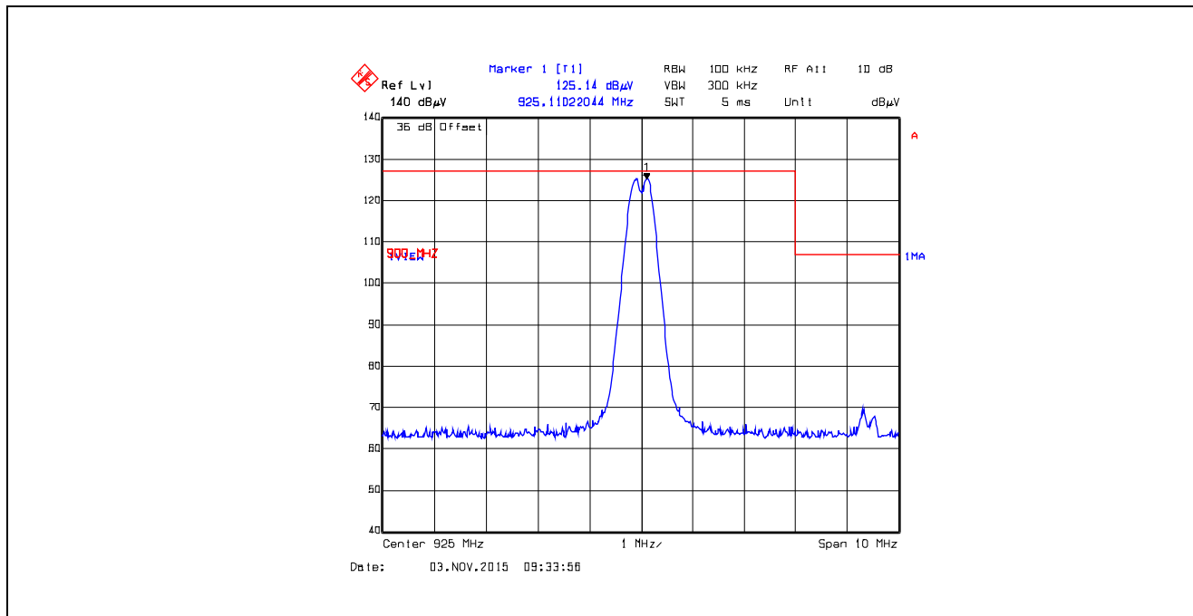
Plot 5.5.4.2.2.32. Band-Edge RF Radiated Emissions at 3 m, Vertical Polarization Pseudorandom Hopping Mode, High End of Frequency Band, 925.0 MHz, XTC0, Data Rate at 10 kbps
