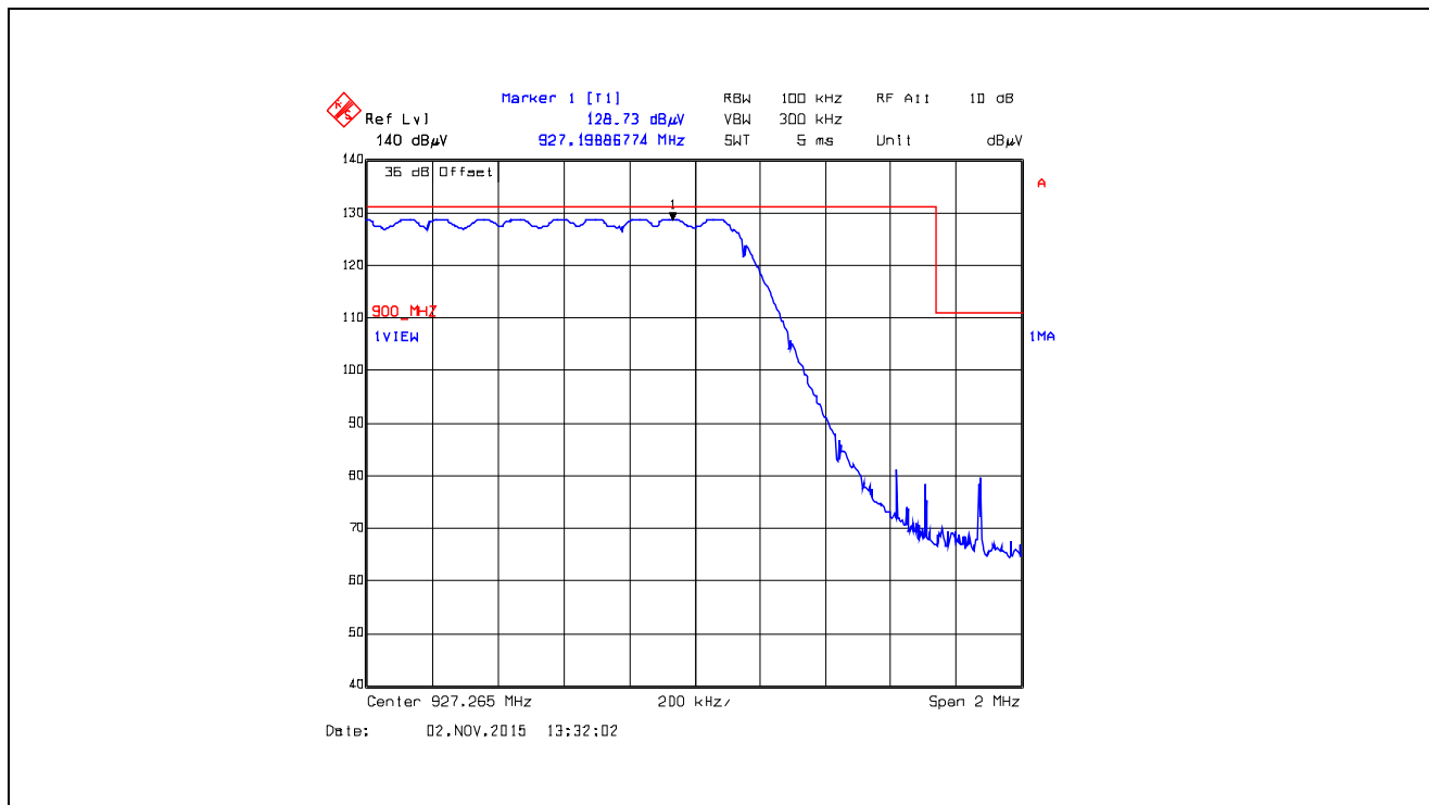
Plot 5.5.4.4.2.46. Band-Edge RF Radiated Emissions at 3 m, Horizontal Polarization Pseudorandom Hopping Mode, High End of Frequency Band, 927.265 MHz, XTCA0, Data Rate at 10 kbps
