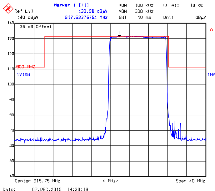
Plot 5.5.4.5.2.42. Band-Edge RF Radiated Emissions at 3 m, Horizontal Polarization Pseudorandom Hopping Mode, Low End of Frequency Band, 915.75 MHz, XTCA0, Data Rate at 10 kbps
