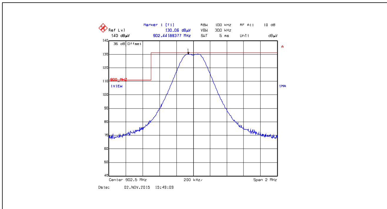
Plot 5.5.4.2.11. Band-Edge RF Radiated Emissions at 3 m, Vertical Polarization Single Frequency Mode, Low End of Frequency Band, 902.5 MHz, XBX1, Data Rate at 110 kbps
