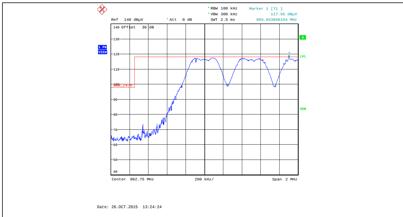
Plot 5.5.4.3.2.18. Band-Edge RF Radiated Emissions at 3 m, Horizontal Polarization Pseudorandom Hopping Mode, Low End of Frequency Band, 902.75 MHz, XB2, Data Rate at 250 kbps
