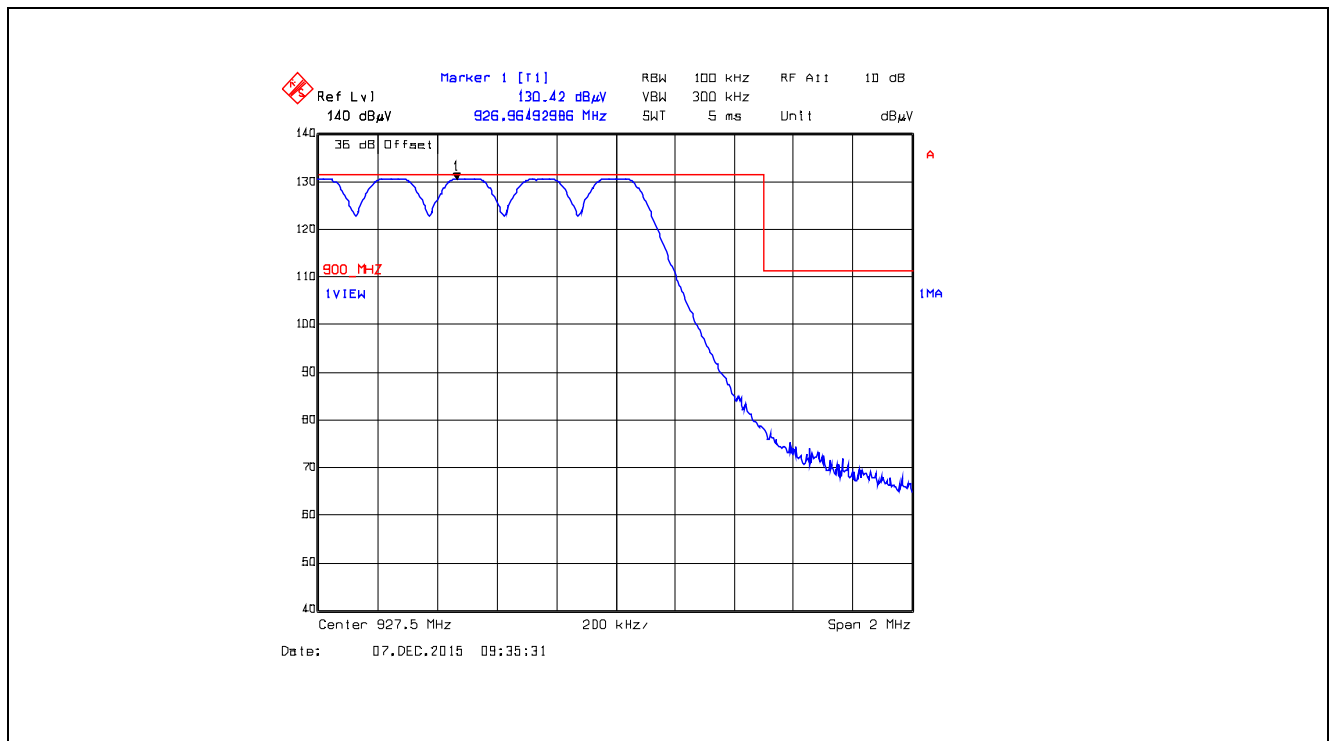
Plot 5.5.4.5.2.8. Band-Edge RF Radiated Emissions at 3 m, Vertical Polarization Pseudorandom Hopping Mode, High End of Frequency Band, 927.5 MHz, XB0, Data Rate at 10 kbps
