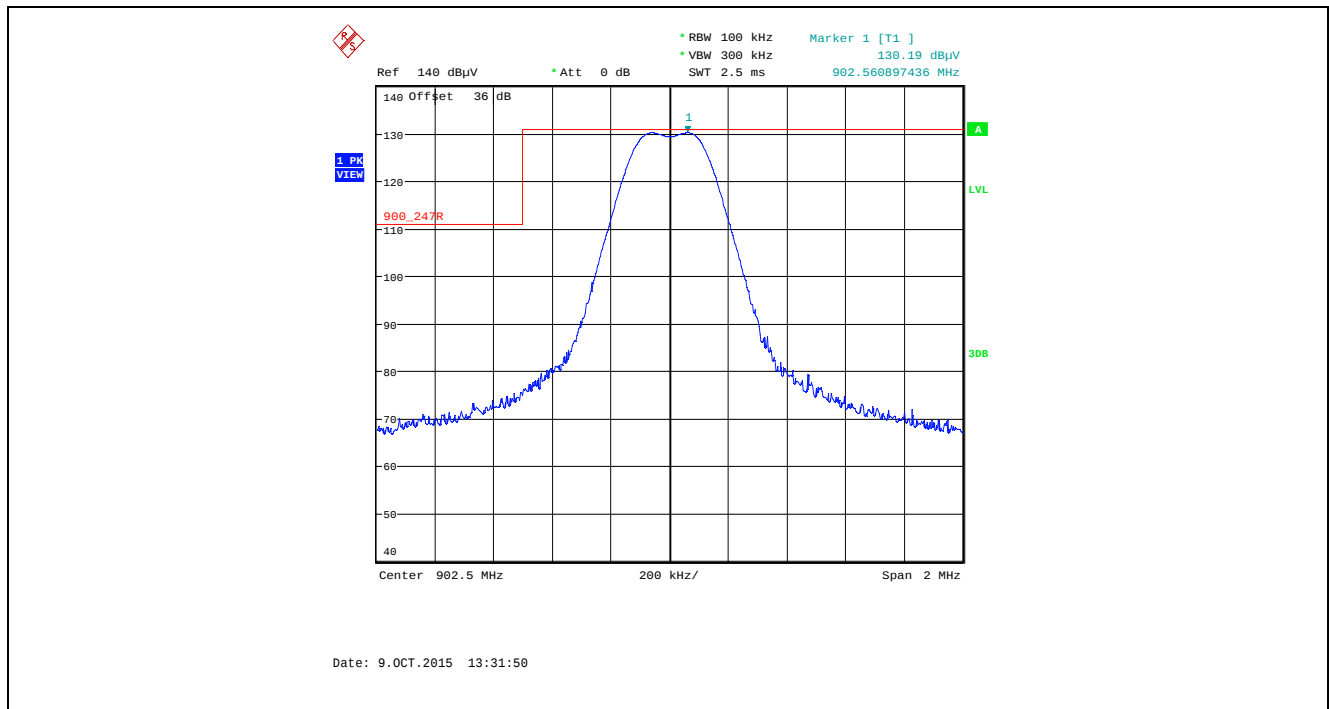
Plot 5.5.4.1.2.9. Band-Edge RF Radiated Emissions at 3 m, Horizontal Polarization Single Frequency Mode, Low End of Frequency Band, 902.5 MHz, XB1, Data Rate at 110 kbps
