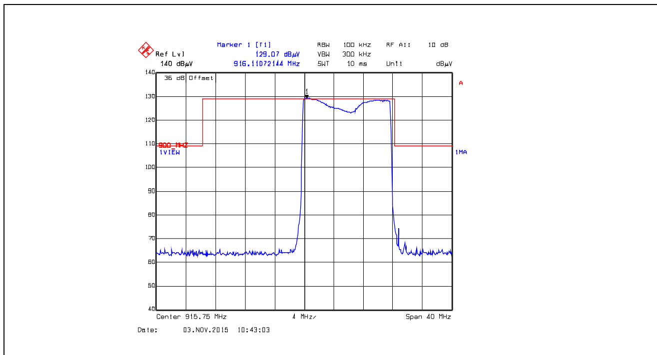
Plot 5.5.4.2.44. Band-Edge RF Radiated Emissions at 3 m, Vertical Polarization Pseudorandom Hopping Mode, Low End of Frequency Band, 915.75 MHz, XTCA0, Data Rate at 10 kbps
