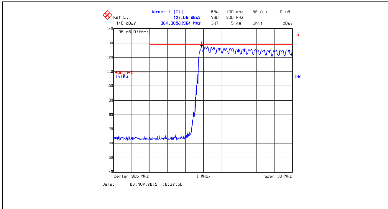
Plot 5.5.4.2.28. Band-Edge RF Radiated Emissions at 3 m, Vertical Polarization Pseudorandom Hopping Mode, Low End of Frequency Band, 905.0 MHz, XTC0, Data Rate at 10 kbps
