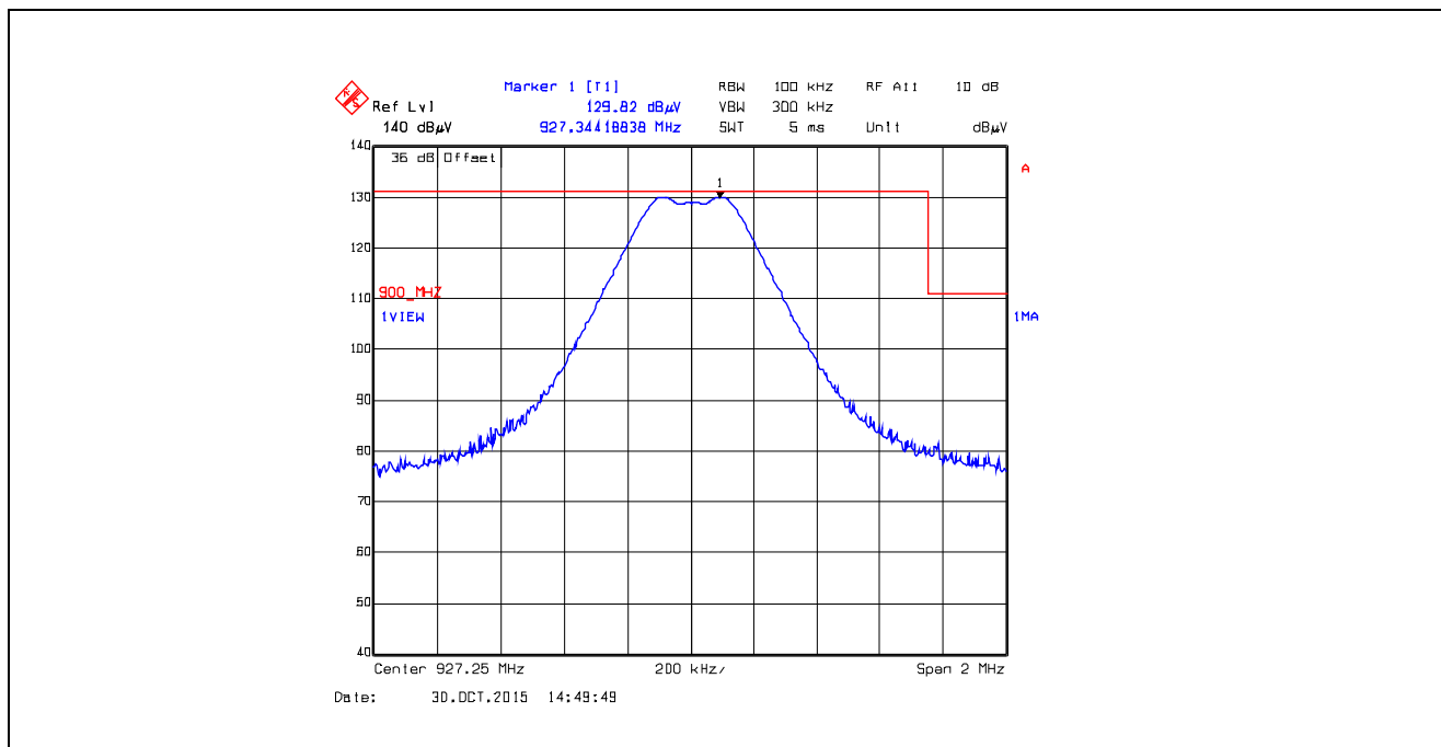
Plot 5.5.4.4.23. Band-Edge RF Radiated Emissions at 3 m, Vertical Polarization Single Frequency Mode, High End of Frequency Band, 927.25 MHz, XB2, Data Rate at 250 kbps
