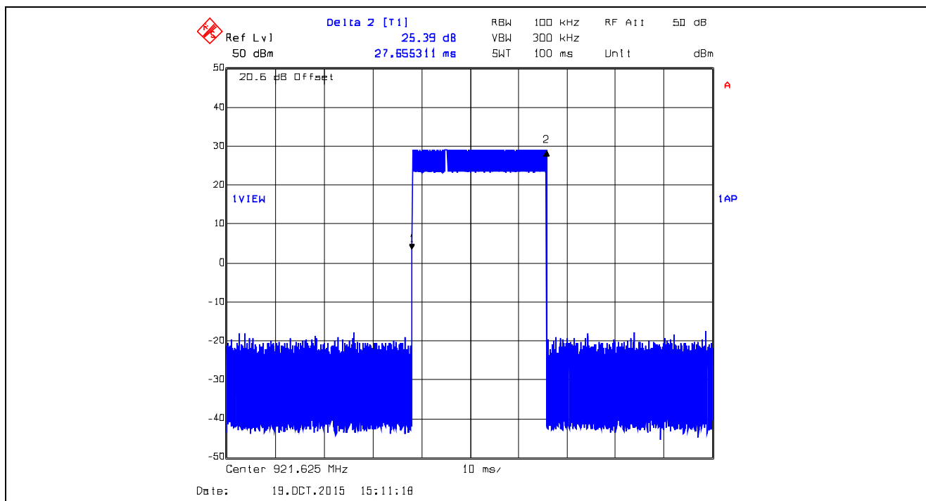
Plot 5.3.4.86. Time of Occupancy, 921.625 MHz, XTCA1, Data Rate at 105 kbps Dwell Time @ 921.625 MHz = 27.6553 ms
