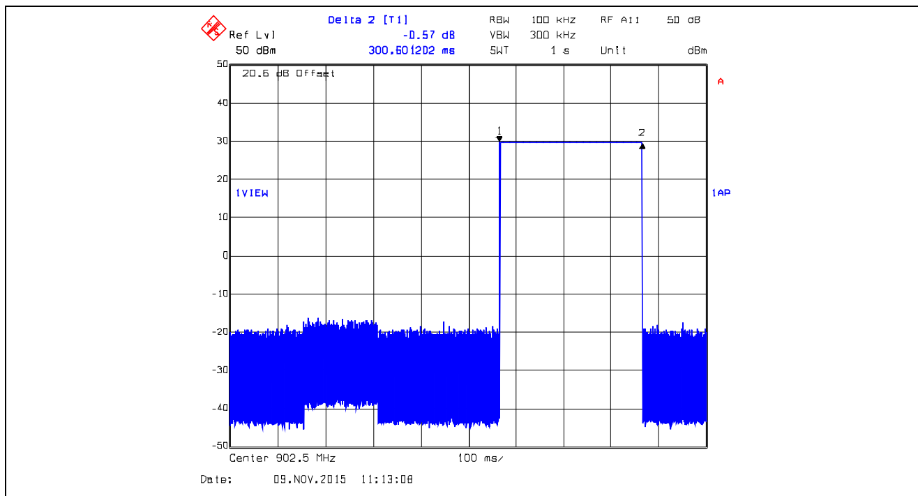
Plot 5.3.4.48. Time of Occupancy, 902.5 MHz, XB0, Data Rate at 10 kbps Dwell Time @ 902.5 MHz = 300.601202 ms
