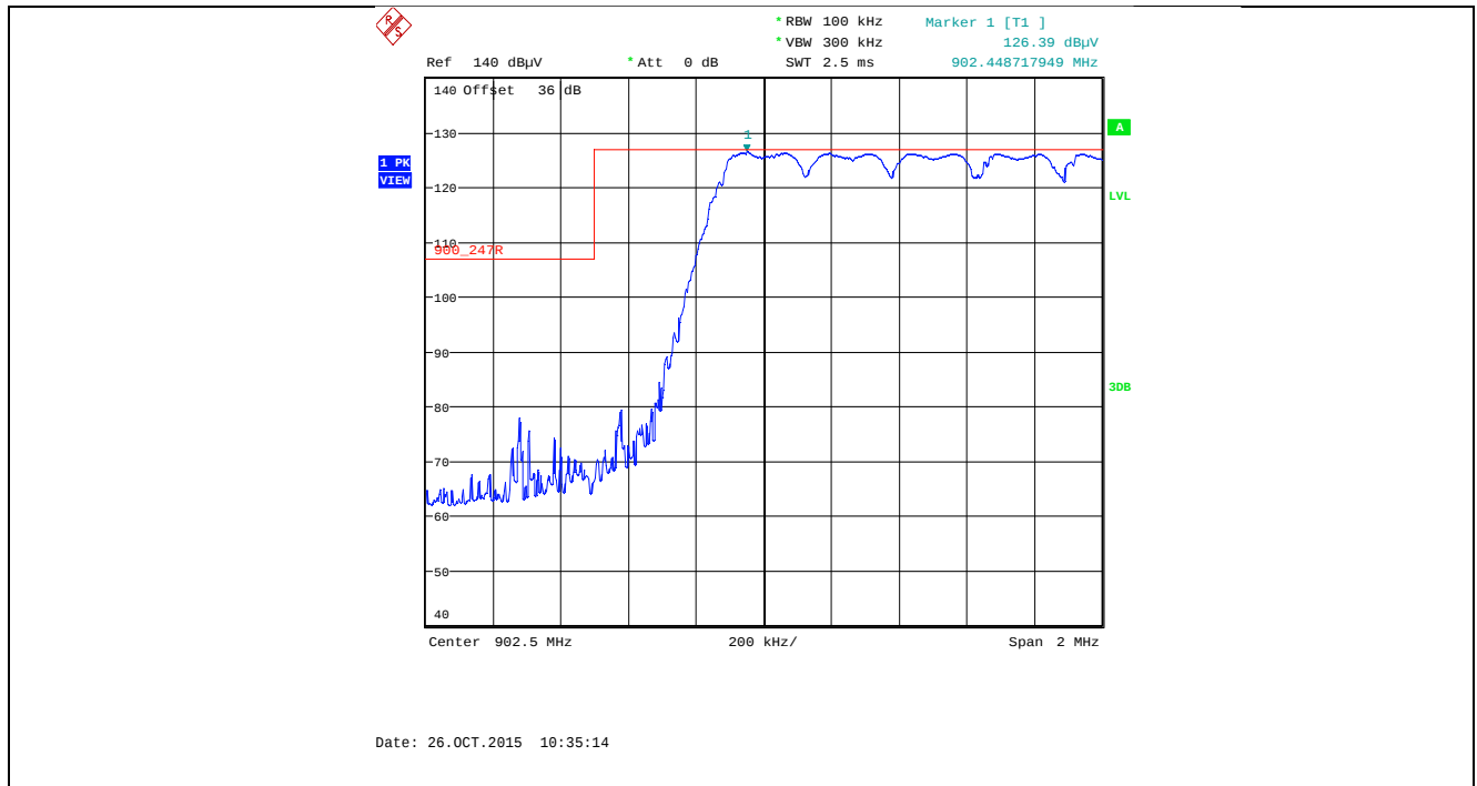
Plot 5.5.4.3.2.12. Band-Edge RF Radiated Emissions at 3 m, Vertical Polarization Pseudorandom Hopping Mode, Low End of Frequency Band, 902.5 MHz, XB1, Data Rate at 110 kbps
