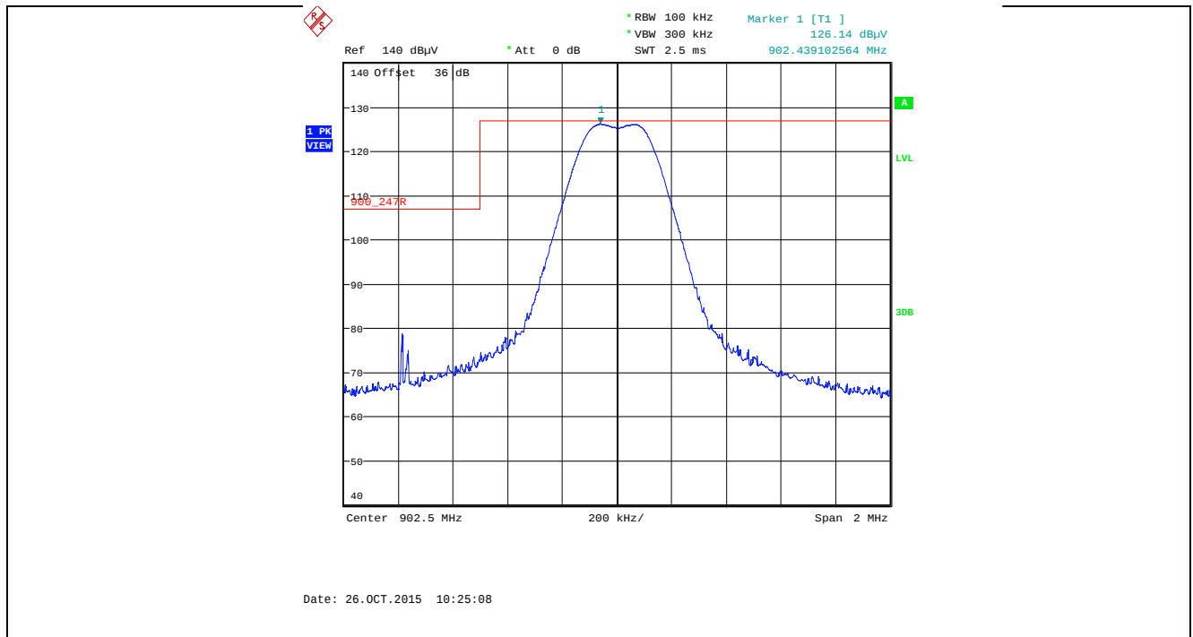
Plot 5.5.4.3.2.11. Band-Edge RF Radiated Emissions at 3 m, Vertical Polarization Single Frequency Mode, Low End of Frequency Band, 902.5 MHz, XB1, Data Rate at 110 kbps
