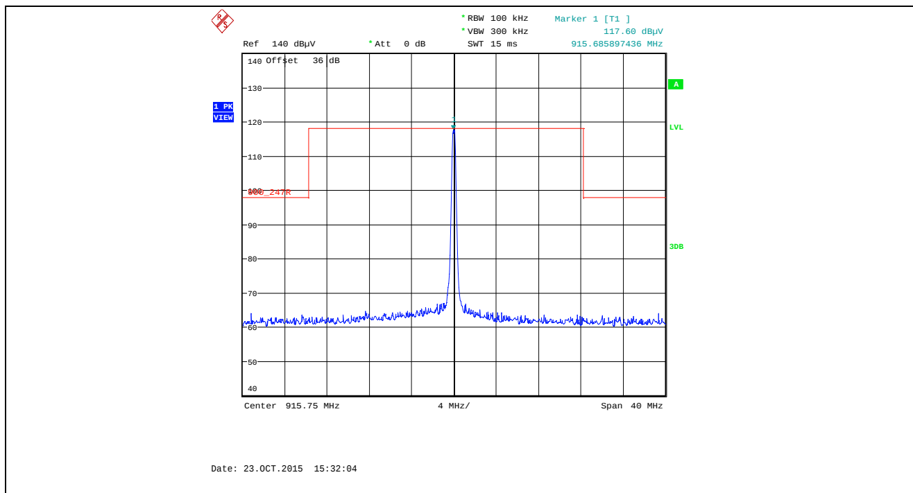
Plot 5.5.4.3.2.49. Band-Edge RF Radiated Emissions at 3 m, Horizontal Polarization Single Frequency Mode, Low End of Frequency Band, 915.75 MHz, XTCA1, Data Rate at 105kbps
