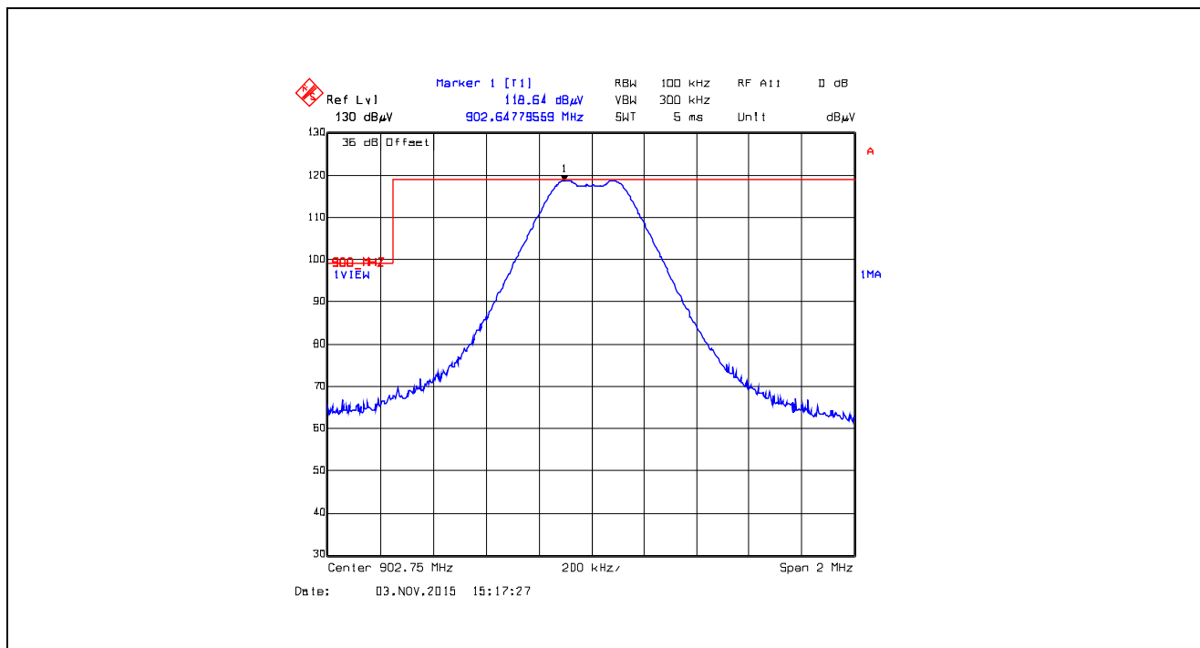
Plot 5.5.4.2.2.17. Band-Edge RF Radiated Emissions at 3 m, Horizontal Polarization Single Frequency Mode, Low End of Frequency Band, 902.75 MHz, XBX2, Data Rate at 250 kbps
