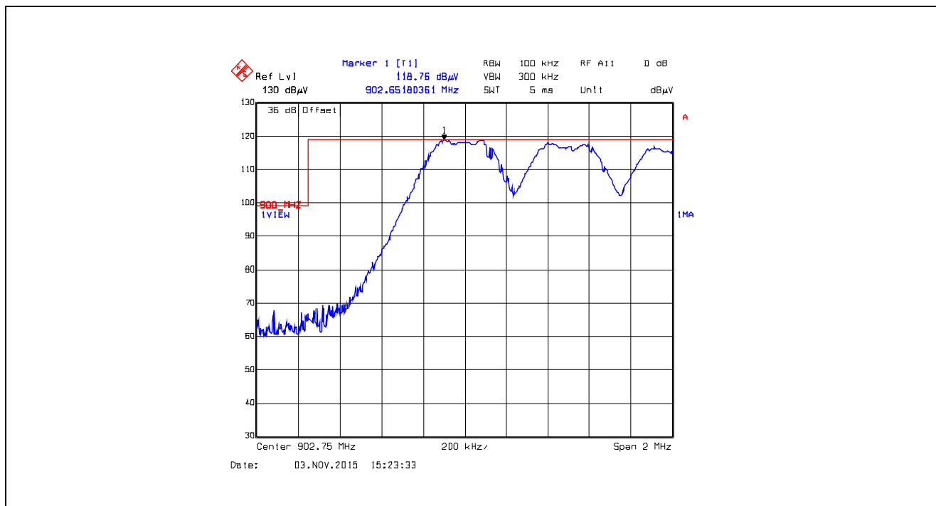
Plot 5.5.4.2.2.18. Band-Edge RF Radiated Emissions at 3 m, Horizontal Polarization Pseudorandom Hopping Mode, Low End of Frequency Band, 902.75 MHz, XBX2, Data Rate at 250 kbps
