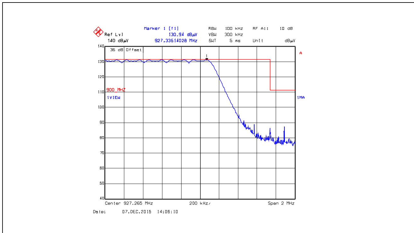
Plot 5.5.4.5.2.56. Band-Edge RF Radiated Emissions at 3 m, Vertical Polarization Pseudorandom Hopping Mode, High End of Frequency Band, 927.265 MHz, XTCA1, Data Rate at 105kbps
