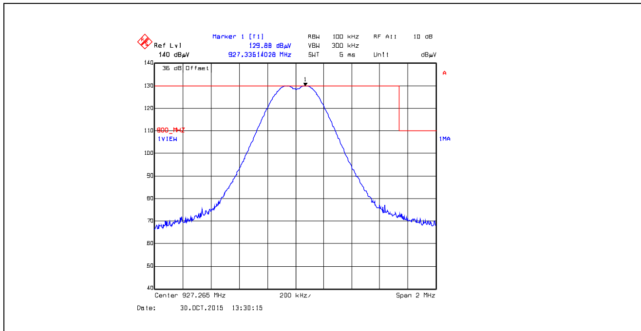
Plot 5.5.4.4.2.48. Band-Edge RF Radiated Emissions at 3 m, Vertical Polarization Pseudorandom Hopping Mode, High End of Frequency Band, 927.265 MHz, XTCA0, Data Rate at 10 kbps
