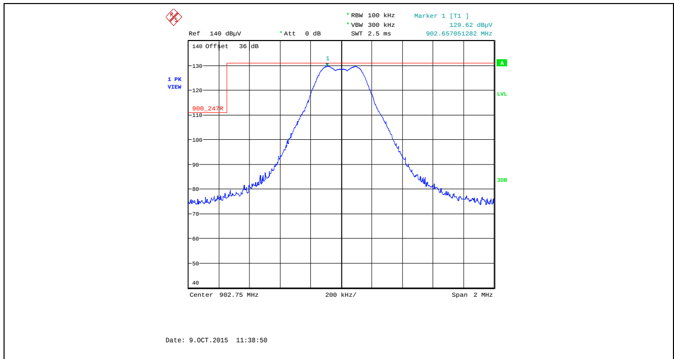
Plot 5.5.4.1.2.19. Band-Edge RF Radiated Emissions at 3 m, Vertical Polarization Single Frequency Mode, Low End of Frequency Band, 902.75 MHz, XB2, Data Rate at 250 kbps
