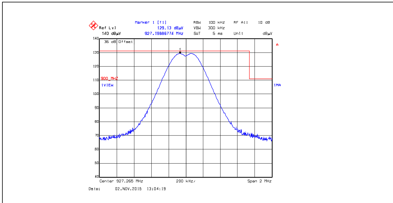
Plot 5.5.4.4.2.46. Band-Edge RF Radiated Emissions at 3 m, Horizontal Polarization Pseudorandom Hopping Mode, High End of Frequency Band, 927.265 MHz, XTCA0, Data Rate at 10 kbps
