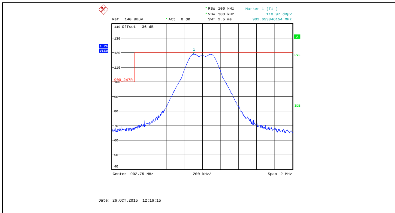
Plot 5.5.4.3.2.17. Band-Edge RF Radiated Emissions at 3 m, Horizontal Polarization Single Frequency Mode, Low End of Frequency Band, 902.75 MHz, XB2, Data Rate at 250 kbps
