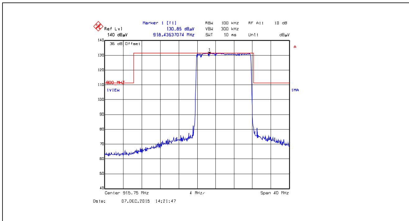
Plot 5.5.4.5.2.50. Band-Edge RF Radiated Emissions at 3 m, Horizontal Polarization Pseudorandom Hopping Mode, Low End of Frequency Band, 915.75 MHz, XTCA1, Data Rate at 105kbps
