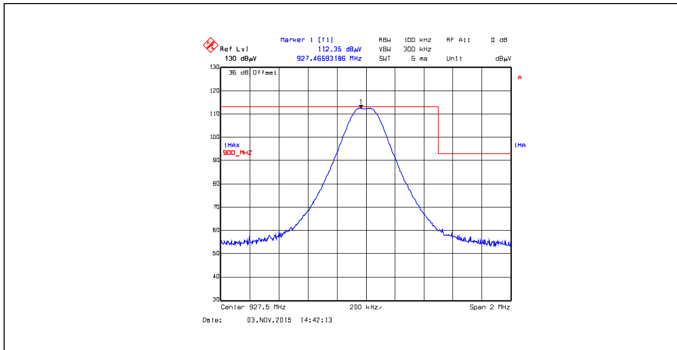
Plot 5.5.4.2.6. Band-Edge RF Radiated Emissions at 3 m, Horizontal Polarization Pseudorandom Hopping Mode, High End of Frequency Band, 927.5 MHz, XB0, Data Rate at 10 kbps
