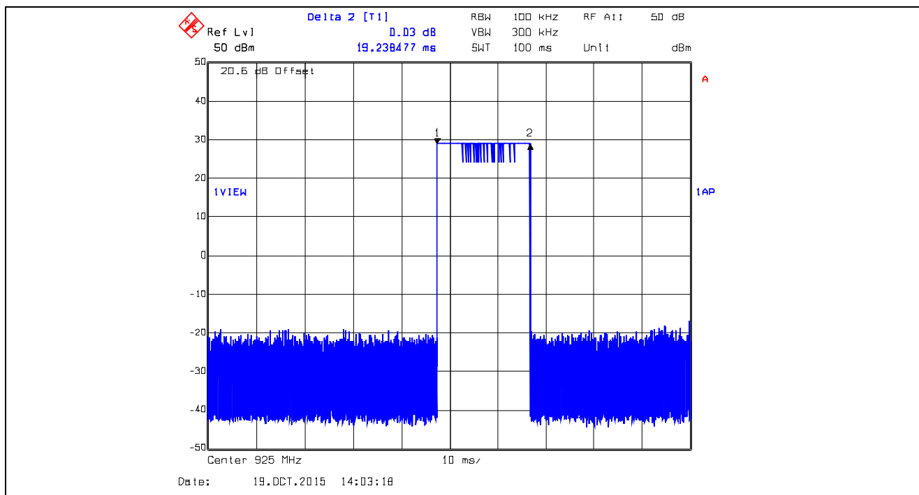
Plot 5.3.4.76. Time of Occupancy, 925.0 MHz, XTC1, Data Rate at 125 kbps Dwell Time @ 925.0 MHz = 19.2385 ms
