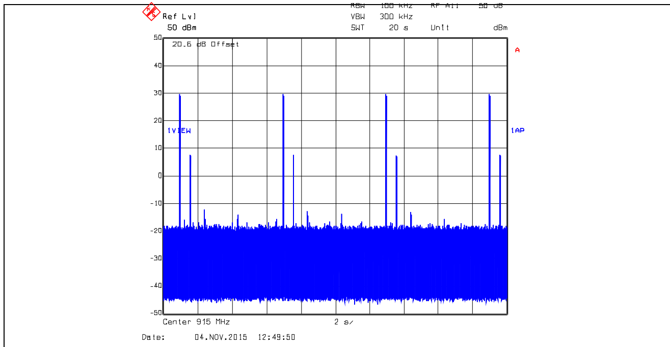
Plot 5.3.4.57. Time of Occupancy, 915.0 MHz, XBX1, Data Rate at 110 kbps Average time of occupancy = (Dwell Time) x (number of hops) = 18.8377 ms x 4 = 75.3508 ms < 0.4 sec within 20 sec
