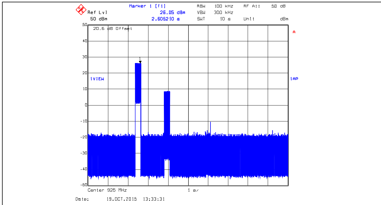
Plot 5.3.4.71. Time of Occupancy, 925.0 MHz, XTC0, Data Rate at 10 kbps Average time of occupancy = (Dwell Time) x (number of hops) = 274.55 ms x 1 = 274.55 ms < 0.4 sec within 10 sec
