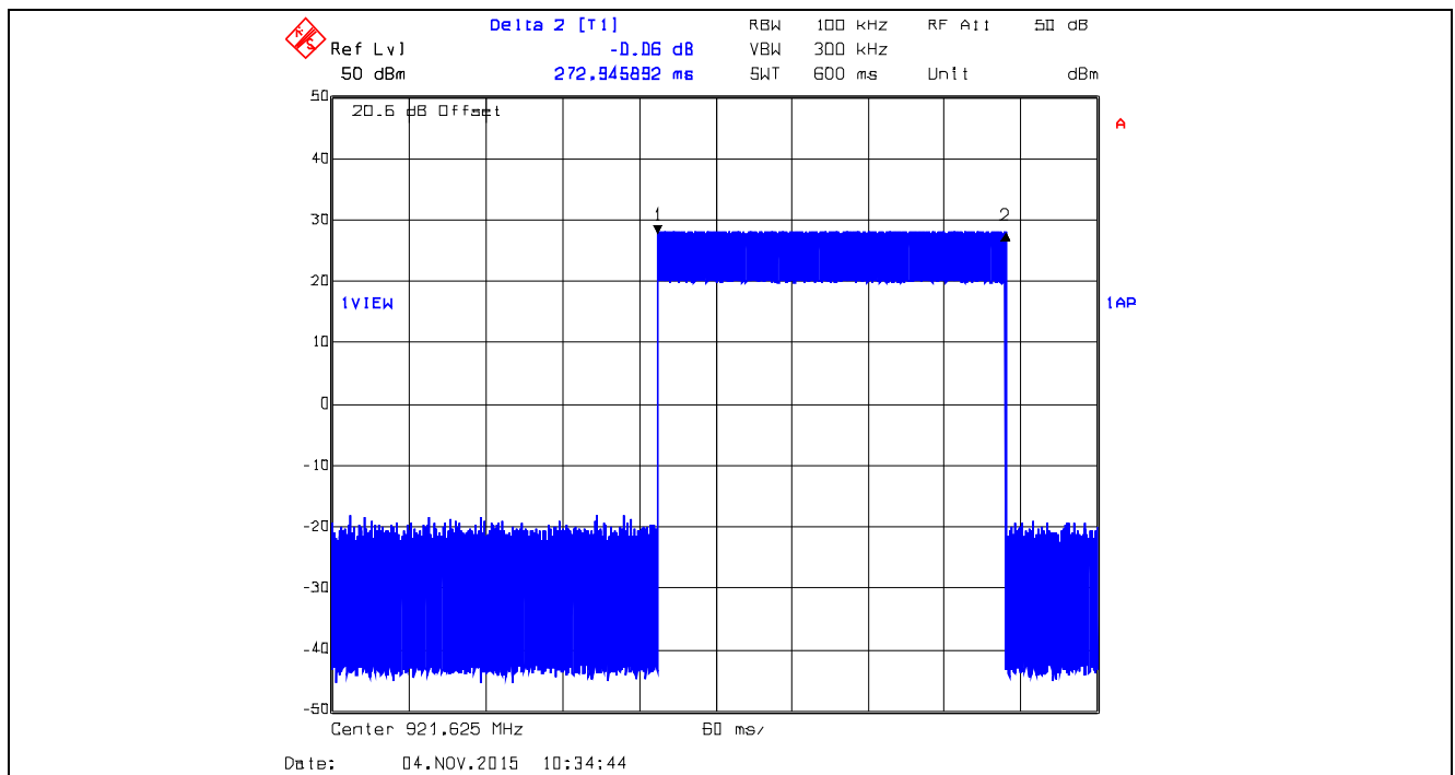
Plot 5.3.4.80. Time of Occupancy, 921.625 MHz, XTCA0, Data Rate at 10 kbps Dwell Time @ 921.625 MHz = 272.9459 ms
