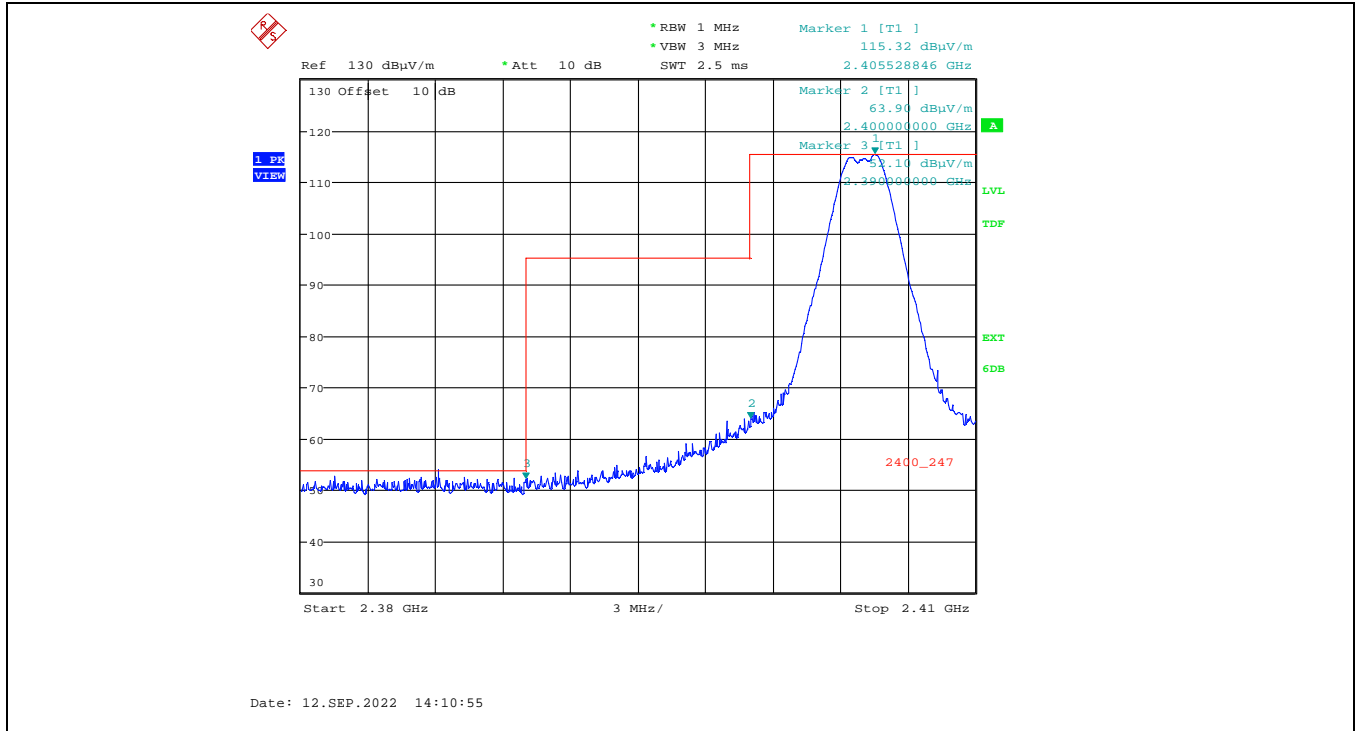
Plot 5.2.3.1.2.3. Band-Edge RF Radiated Emissions at 3 m, Horizontal Polarization, Peak Low End of Frequency Band, 2405 MHz, 20 dBm Power Setting
