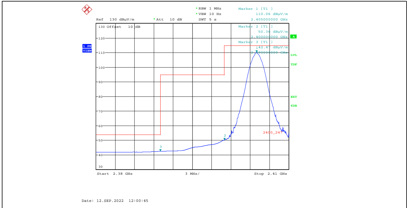
Plot 5.2.3.1.2.2. Band-Edge RF Radiated Emissions at 3 m, Vertical Polarization, Average Low End of Frequency Band, 2405 MHz, 20 dBm Power Setting
