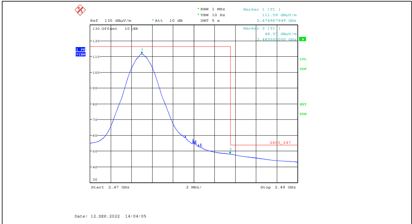
Plot 5.2.3.1.2.8. Band-Edge RF Radiated Emissions at 3 m, Horizontal Polarization, Average High End of Frequency Band, 2475 MHz, 20 dBm Power Setting
