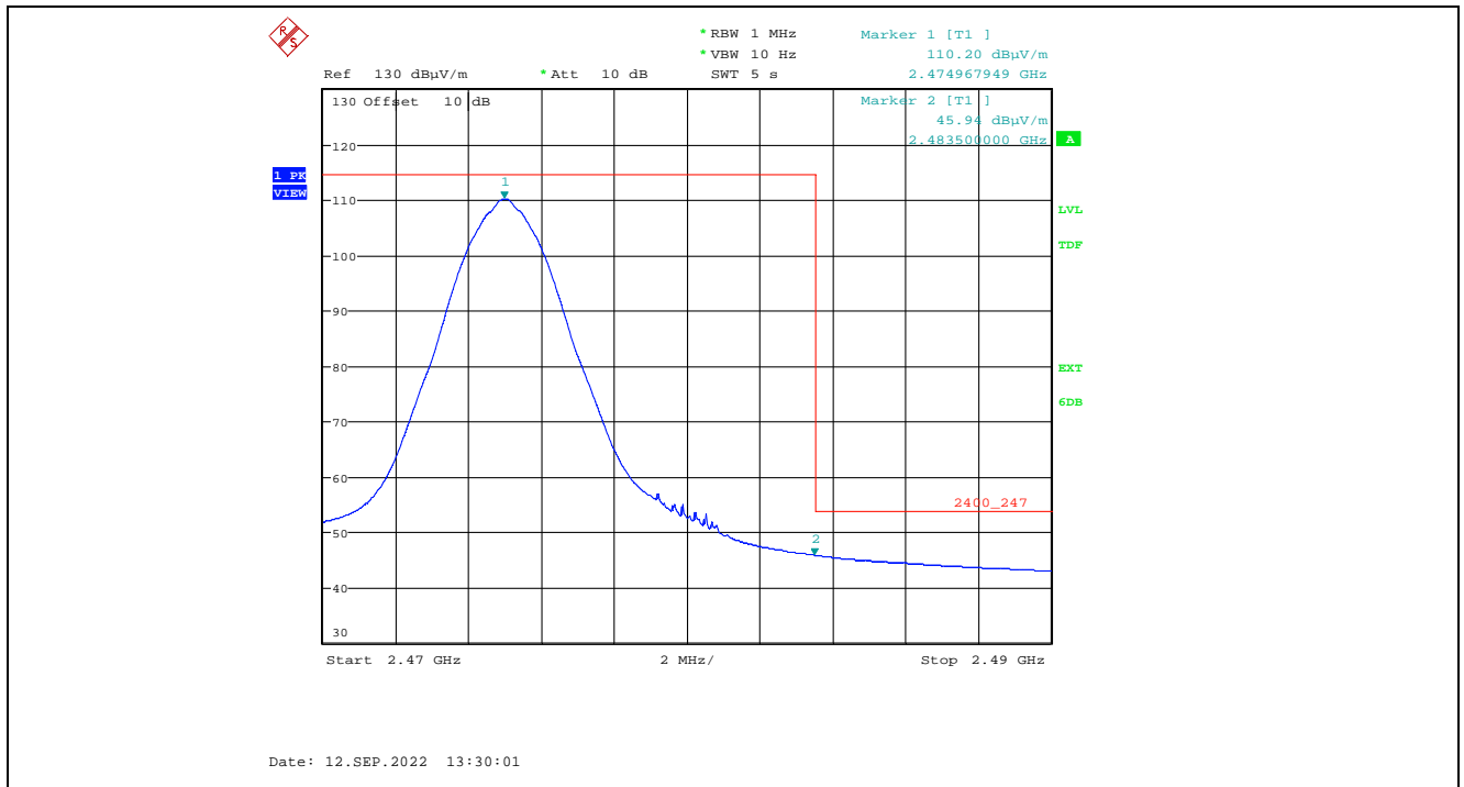
Plot 5.2.3.1.2.6. Band-Edge RF Radiated Emissions at 3 m, Vertical Polarization, Average High End of Frequency Band, 2475 MHz, 20 dBm Power Setting
