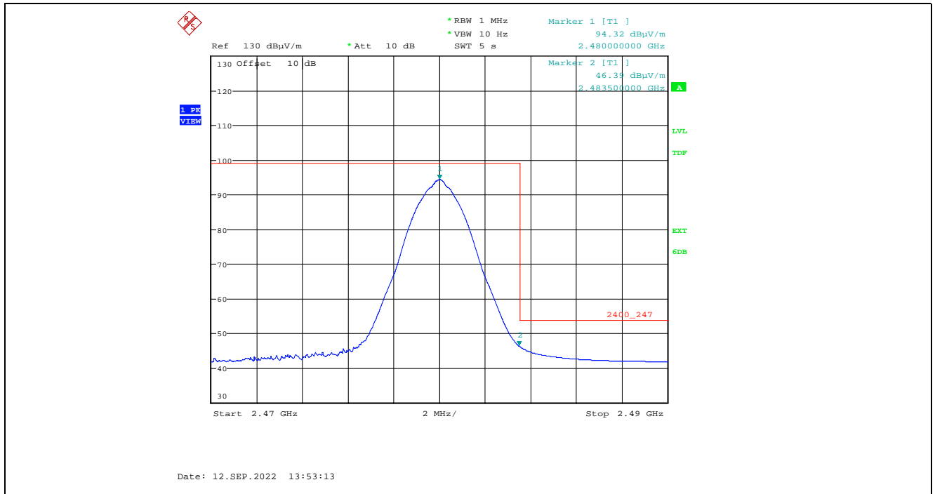
Plot 5.2.3.1.2.12. Band-Edge RF Radiated Emissions at 3 m, Horizontal Polarization, Average High End of Frequency Band, 2480 MHz, 3 dBm Power Setting
