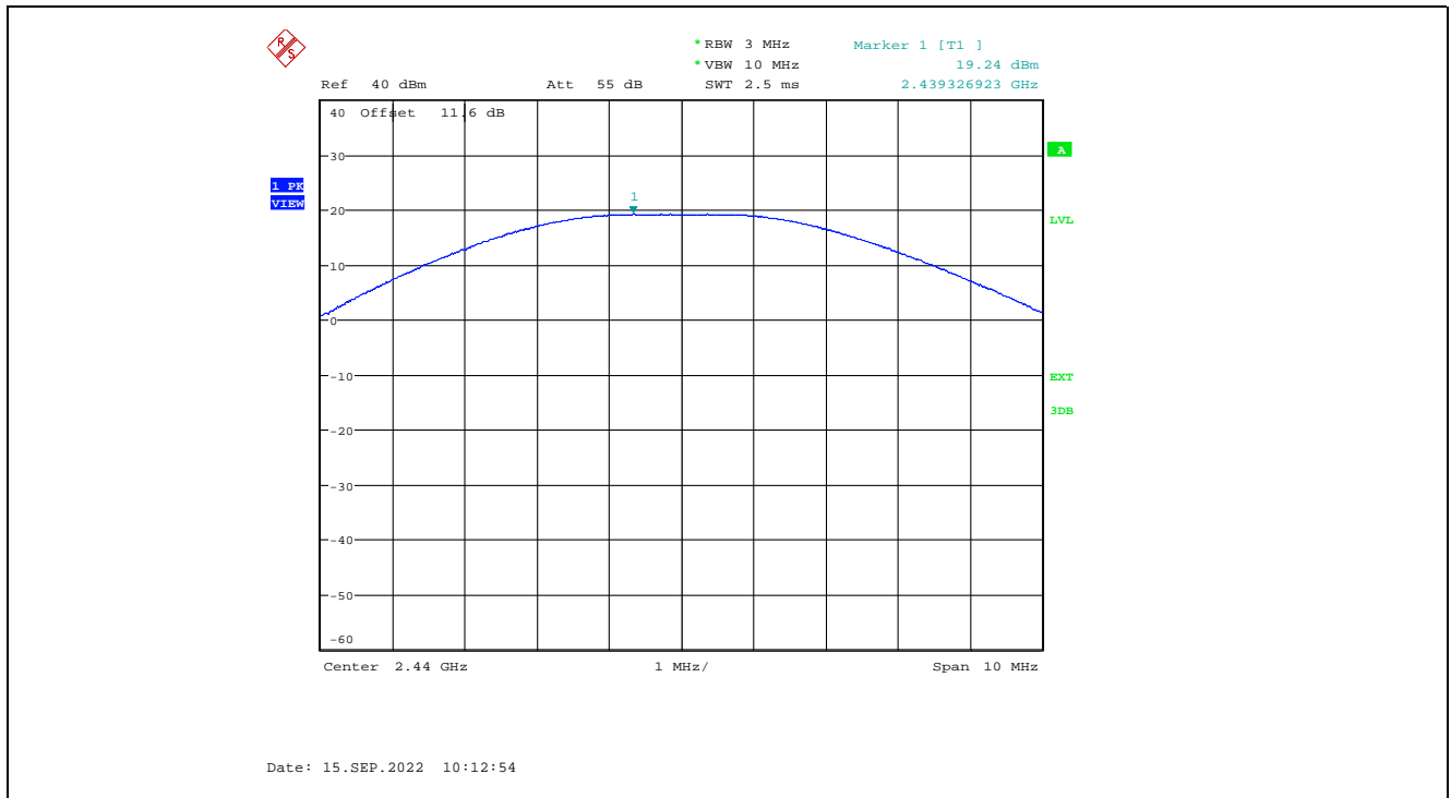
Plot 5.1.3.2. Maximum Peak Conducted Output Power, QPSK Modulation, 20 dBm Power Setting, 2440 MHz
