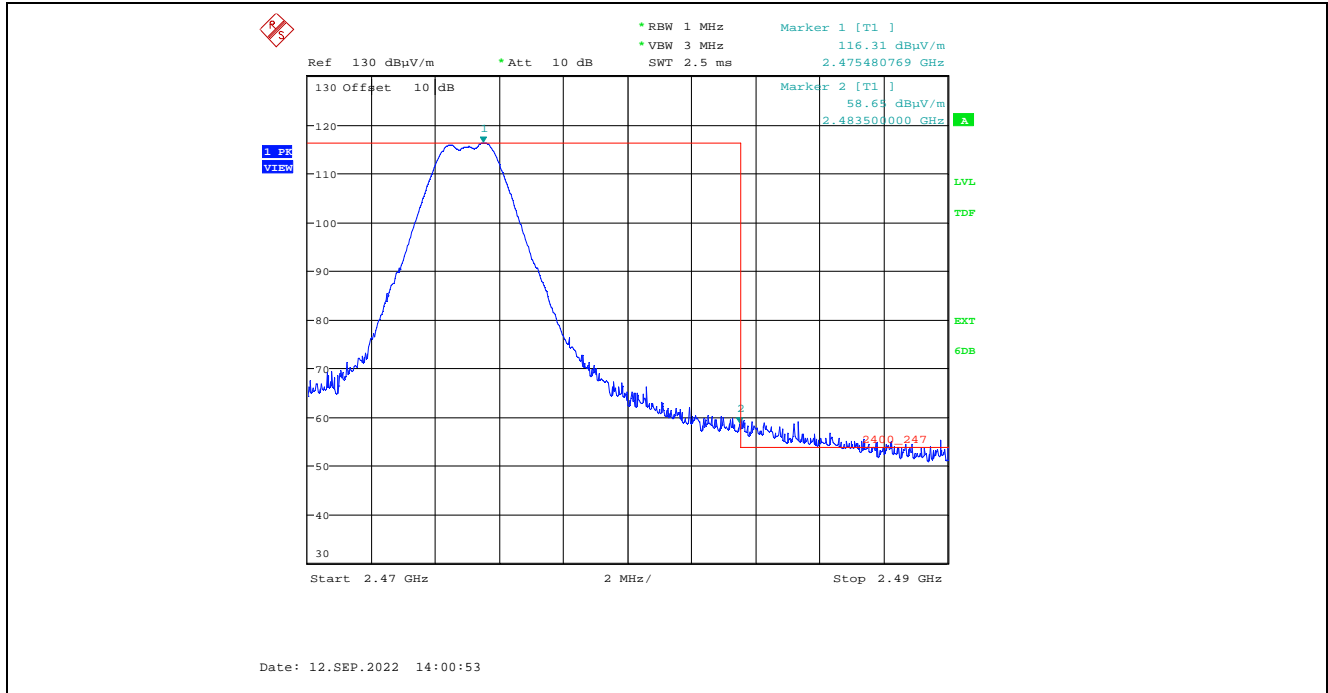
Plot 5.2.3.1.2.7. Band-Edge RF Radiated Emissions at 3 m, Horizontal Polarization, Peak High End of Frequency Band, 2475 MHz, 20 dBm Power Setting
