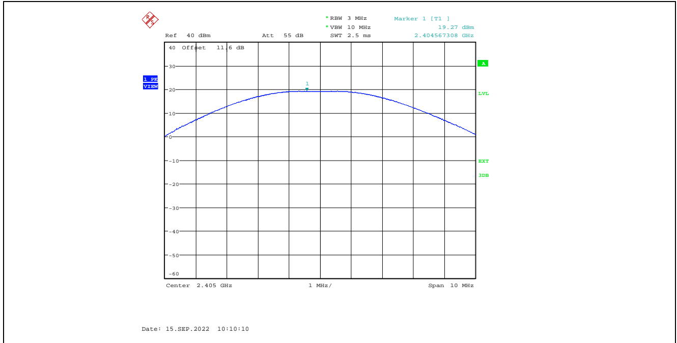
Plot 5.1.3.1. Maximum Peak Conducted Output Power, QPSK Modulation, 20 dBm Power Setting, 2405 MHz
