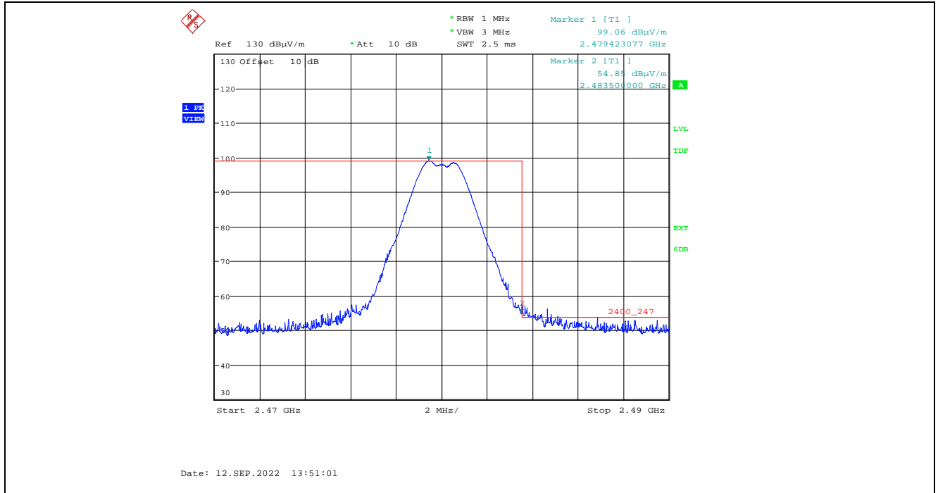
Plot 5.2.3.1.2.11. Band-Edge RF Radiated Emissions at 3 m, Horizontal Polarization, Peak High End of Frequency Band, 2480 MHz, 3 dBm Power Setting
