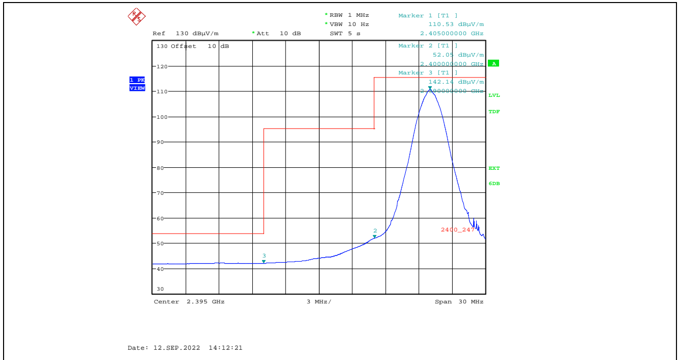
Plot 5.2.3.1.2.4. Band-Edge RF Radiated Emissions at 3 m, Horizontal Polarization, Average Low End of Frequency Band, 2405 MHz, 20 dBm Power Setting
