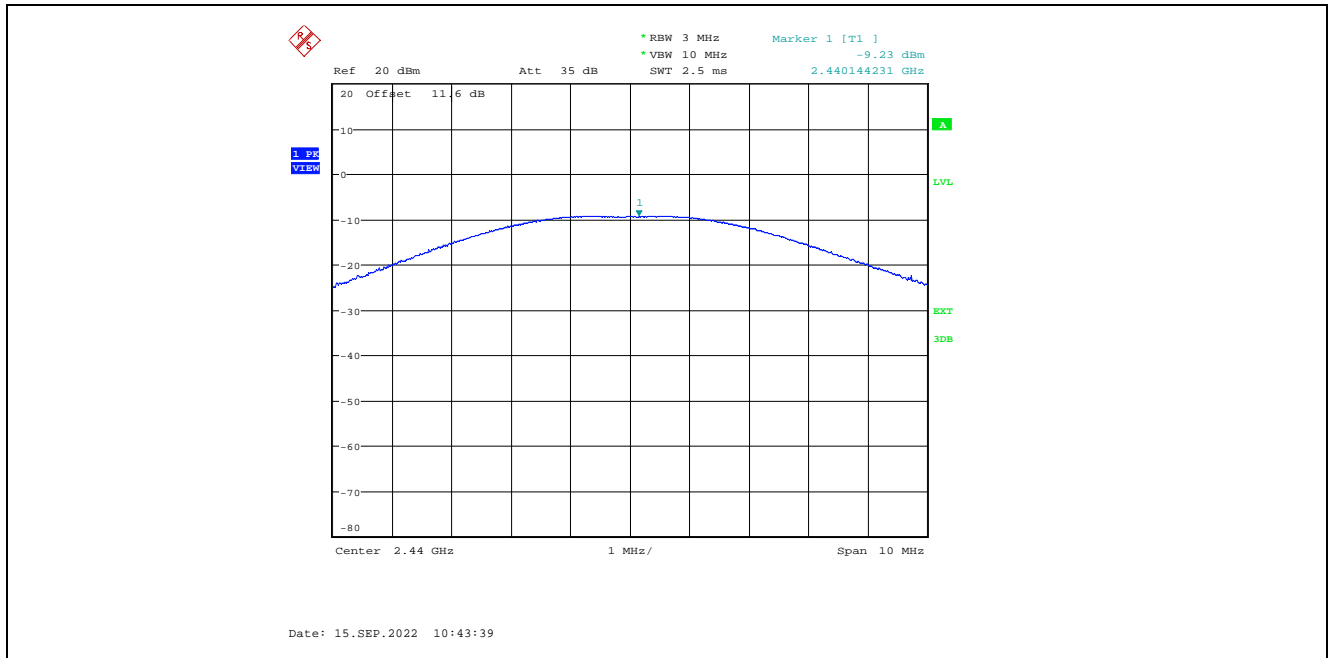
Plot 5.1.3.6. Maximum Peak Conducted Output Power, QPSK Modulation, -10 dBm Power Setting, 2440 MHz
