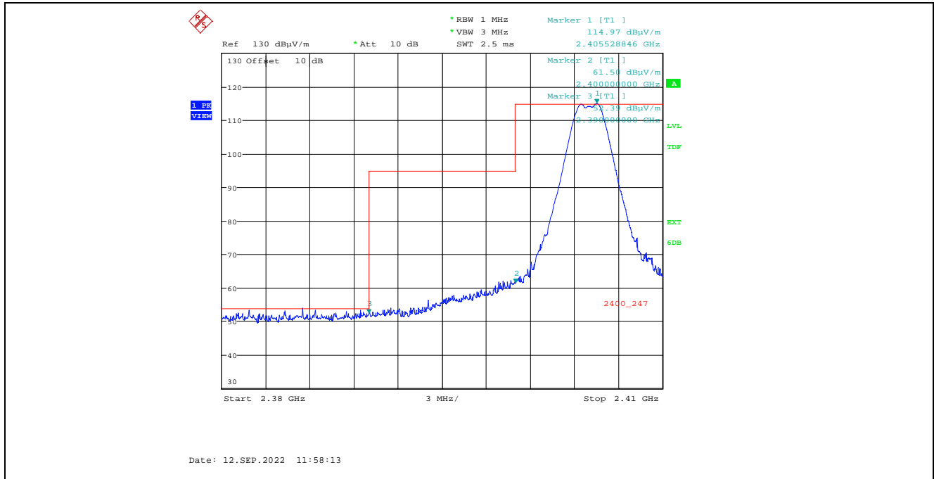
Plot 5.2.3.1.2.1. Band-Edge RF Radiated Emissions at 3 m, Vertical Polarization, Peak Low End of Frequency Band, 2405 MHz, 20 dBm Power Setting
