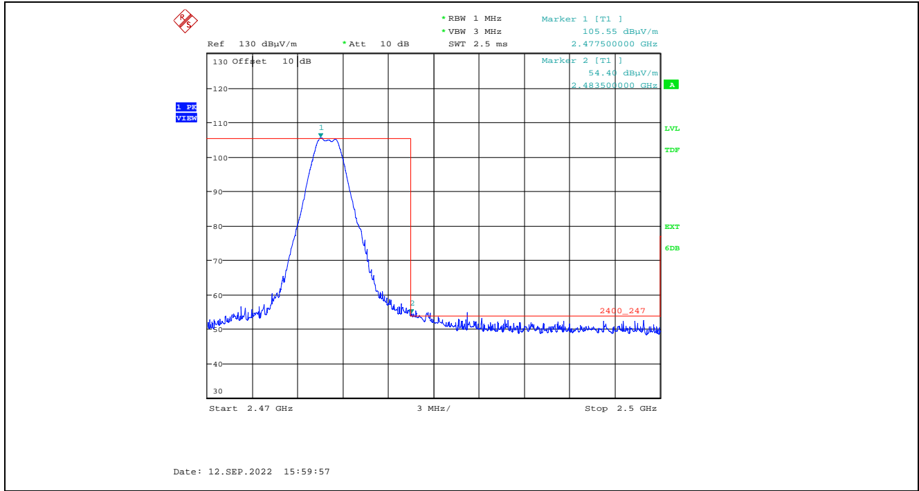
Plot 5.2.3.2.2.7. Band-Edge RF Radiated Emissions at 3 m, Horizontal Polarization, Peak High End of Frequency Band, 2478 MHz, 8 dBm Power Setting, 2 Mbps
