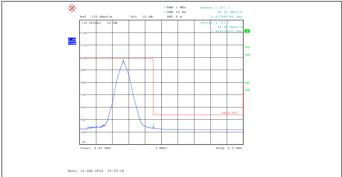
Plot 5.2.3.2.2.6. Band-Edge RF Radiated Emissions at 3 m, Vertical Polarization, Average High End of Frequency Band, 2478 MHz, 8 dBm Power Setting, 2 Mbps
