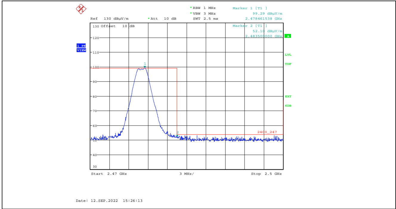
Plot 5.2.3.2.2.5. Band-Edge RF Radiated Emissions at 3 m, Vertical Polarization, Peak High End of Frequency Band, 2478 MHz, 8 dBm Power Setting, 2 Mbps
