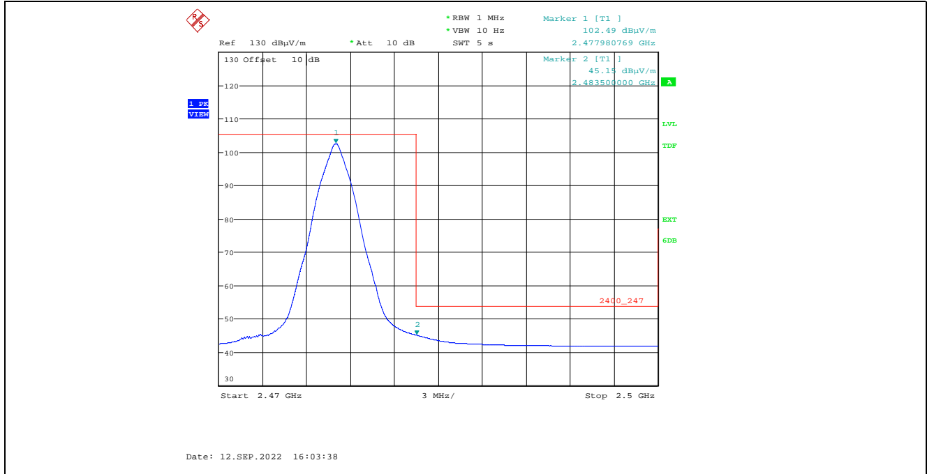
Plot 5.2.3.2.2.8. Band-Edge RF Radiated Emissions at 3 m, Horizontal Polarization, Average High End of Frequency Band, 2478 MHz, 8 dBm Power Setting, 2 Mbps
