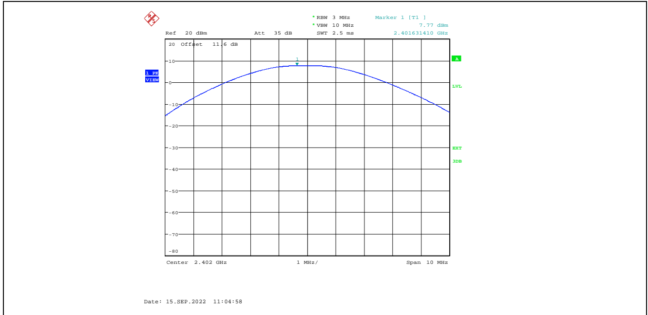
Plot 5.1.3.1. Maximum Peak Conducted Output Power, GFSK Modulation, 1 Mbps, 8 dBm Power Setting, 2402 MHz
