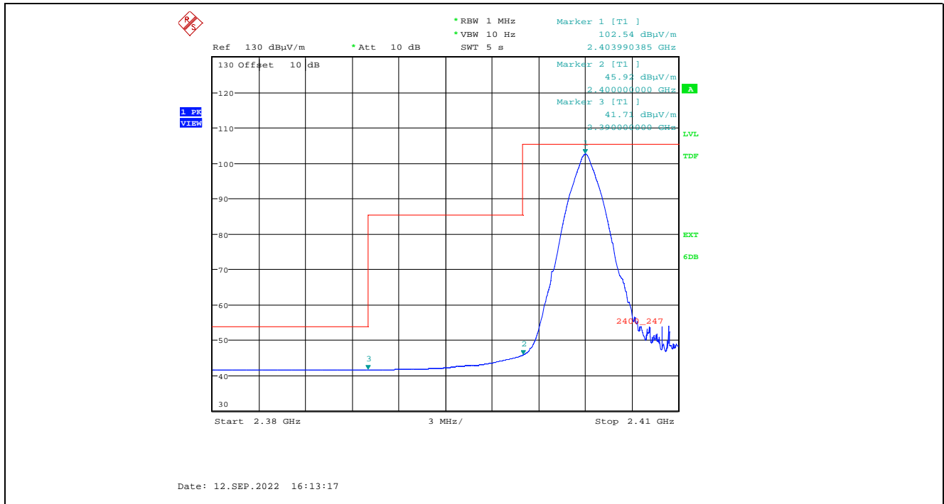
Plot 5.2.3.2.2.4. Band-Edge RF Radiated Emissions at 3 m, Horizontal Polarization, Average Low End of Frequency Band, 2404 MHz, 8 dBm Power Setting, 2 Mbps
