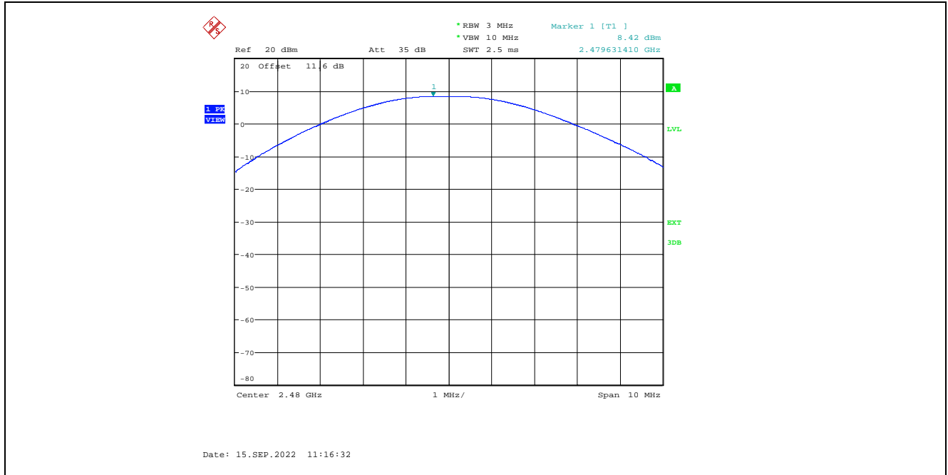
Plot 5.1.3.3. Maximum Peak Conducted Output Power, GFSK Modulation, 1 Mbps, 8 dBm Power Setting, 2480 MHz
