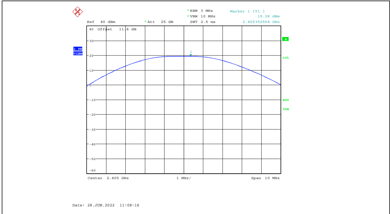
Plot 5.1.3.1. Maximum Peak Conducted Output Power, QPSK Modulation, 20 dBm Power Setting, 2405 MHz
