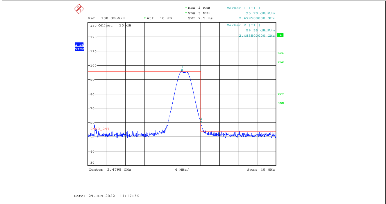
Plot 5.2.3.1.2.9. Band-Edge RF Radiated Emissions at 3 m, Horizontal Polarization, Peak High End of Frequency Band, 2480 MHz, 3 dBm Power Setting
