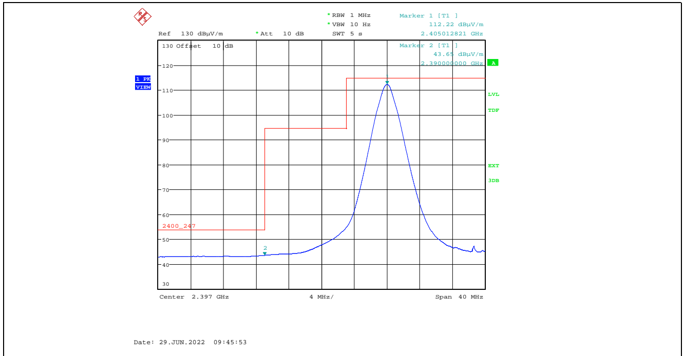
Plot 5.2.3.1.2.2. Band-Edge RF Radiated Emissions at 3 m, Horizontal Polarization, Average Low End of Frequency Band, 2405 MHz, 20 dBm Power Setting
