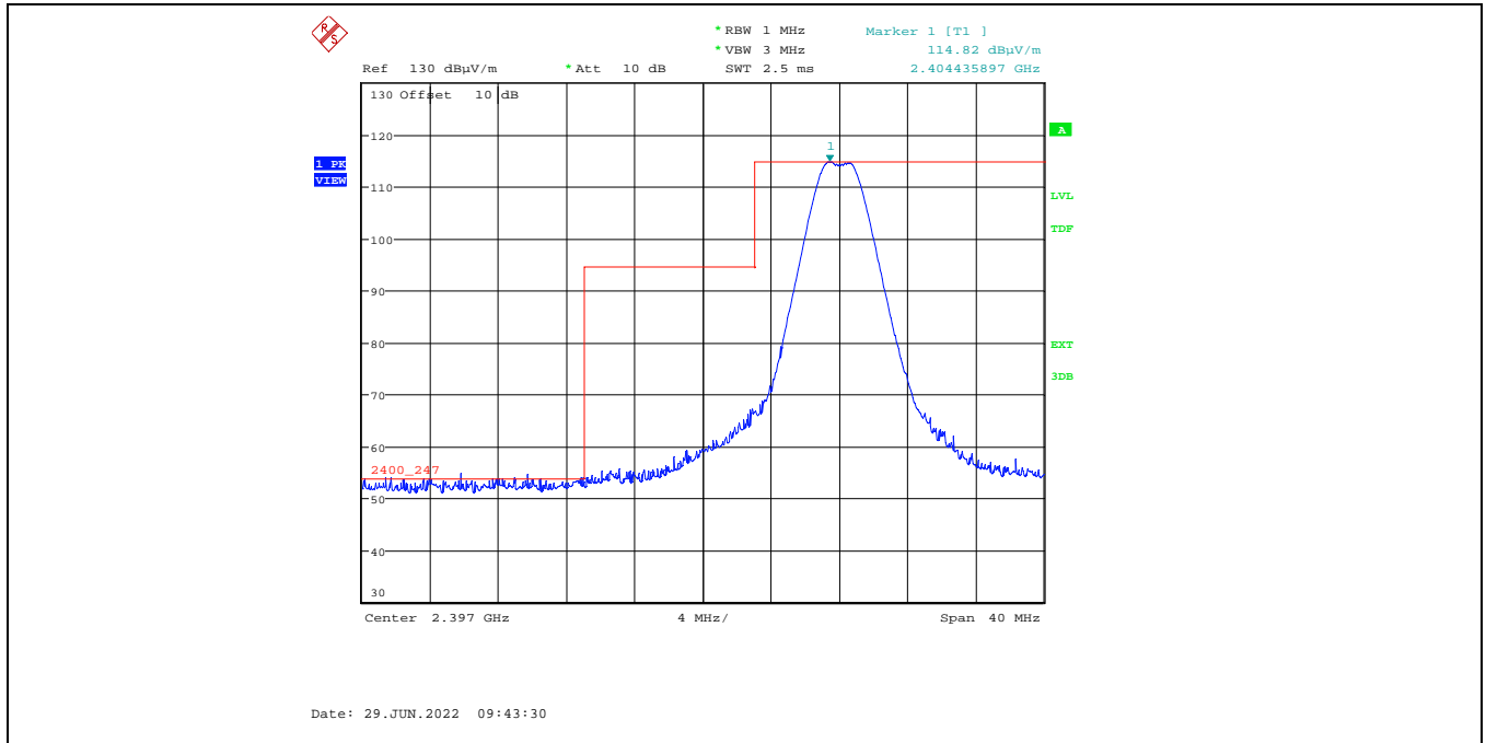
Plot 5.2.3.1.2.2. Band-Edge RF Radiated Emissions at 3 m, Horizontal Polarization, Average Low End of Frequency Band, 2405 MHz, 20 dBm Power Setting
