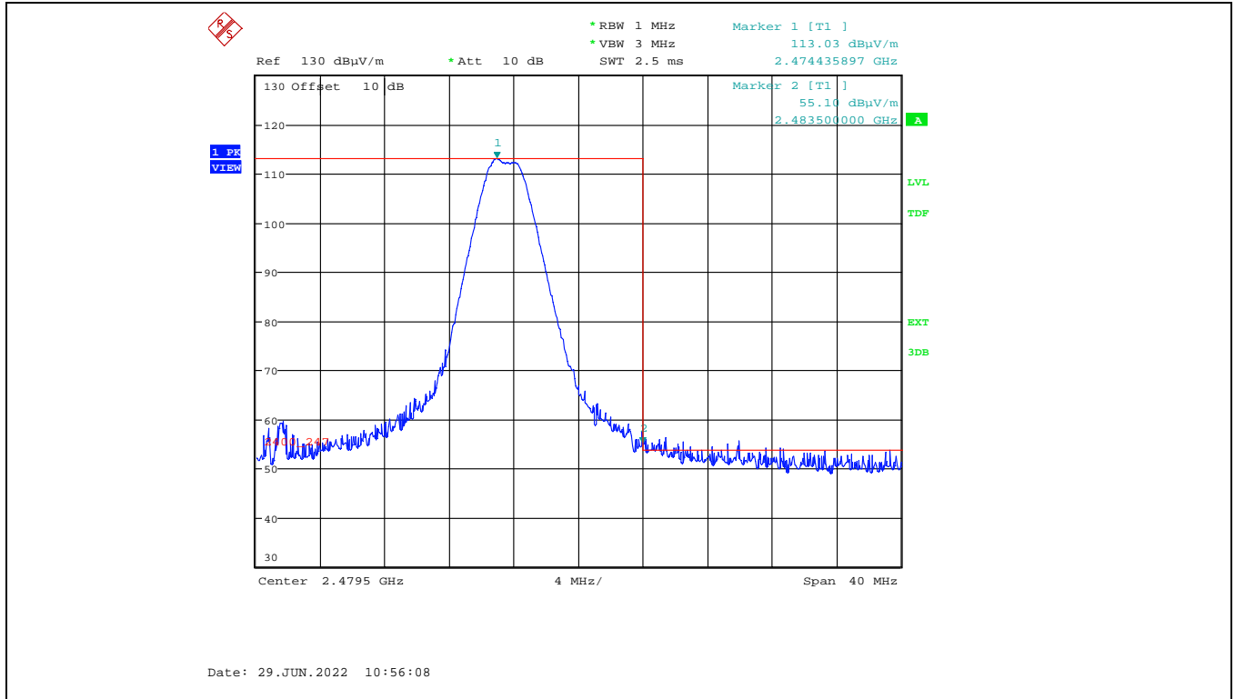
Plot 5.2.3.1.2.8. Band-Edge RF Radiated Emissions at 3 m, Vertical Polarization, Average High End of Frequency Band, 2475 MHz, 20 dBm Power Setting
