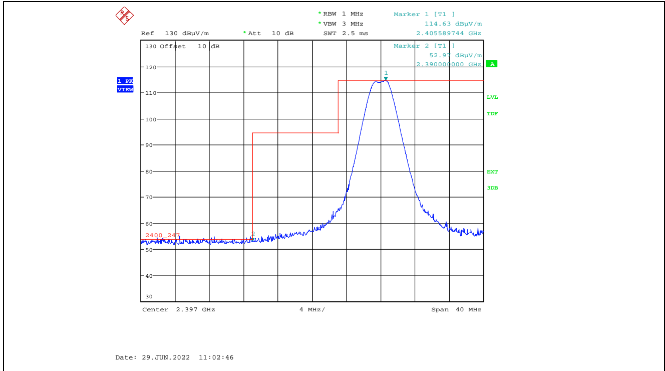
Plot 5.2.3.1.2.3. Band-Edge RF Radiated Emissions at 3 m, Vertical Polarization, Peak Low End of Frequency Band, 2405 MHz, 20 dBm Power Setting
