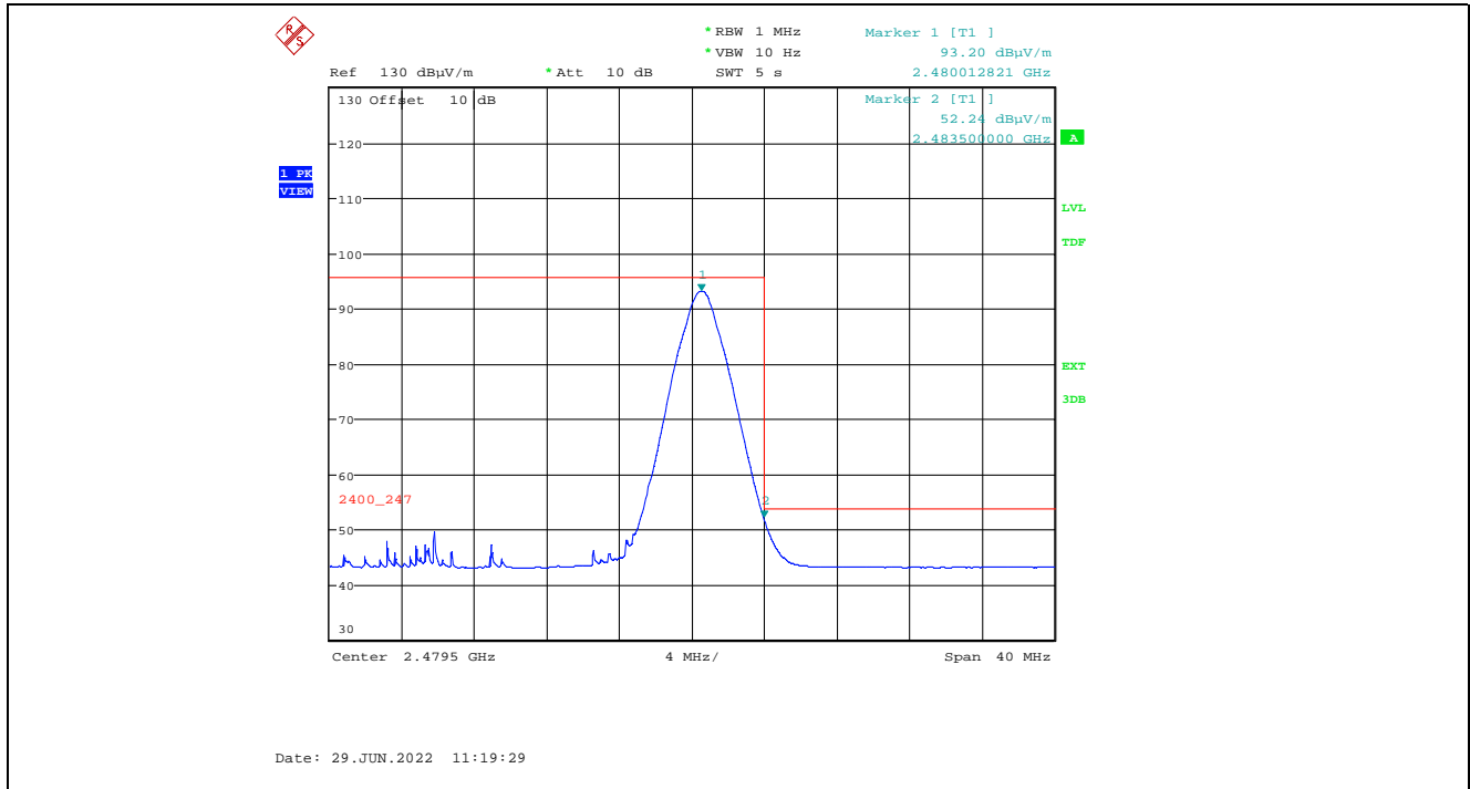
Plot 5.2.3.1.2.10. Band-Edge RF Radiated Emissions at 3 m, Horizontal Polarization, Average High End of Frequency Band, 2480 MHz, 3 dBm Power Setting
