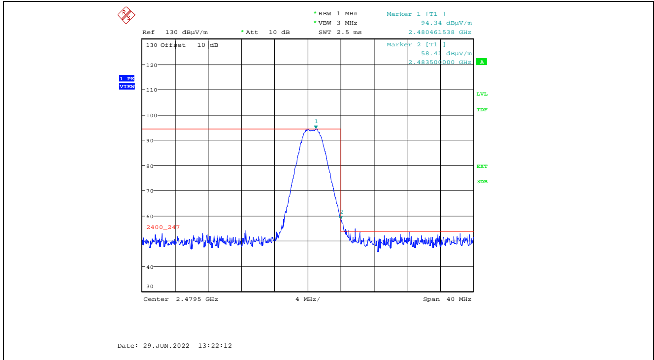
Plot 5.2.3.1.2.11. Band-Edge RF Radiated Emissions at 3 m, Vertical Polarization, Peak High End of Frequency Band, 2480 MHz, 3 dBm Power Setting
