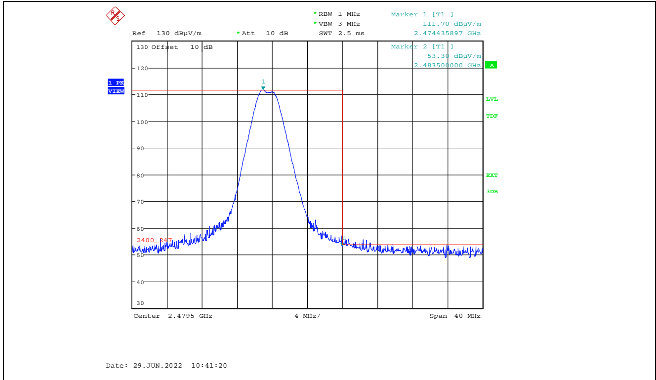
Plot 5.2.3.1.2.6. Band-Edge RF Radiated Emissions at 3 m, Horizontal Polarization, Average High End of Frequency Band, 2475 MHz, 20 dBm Power Setting
