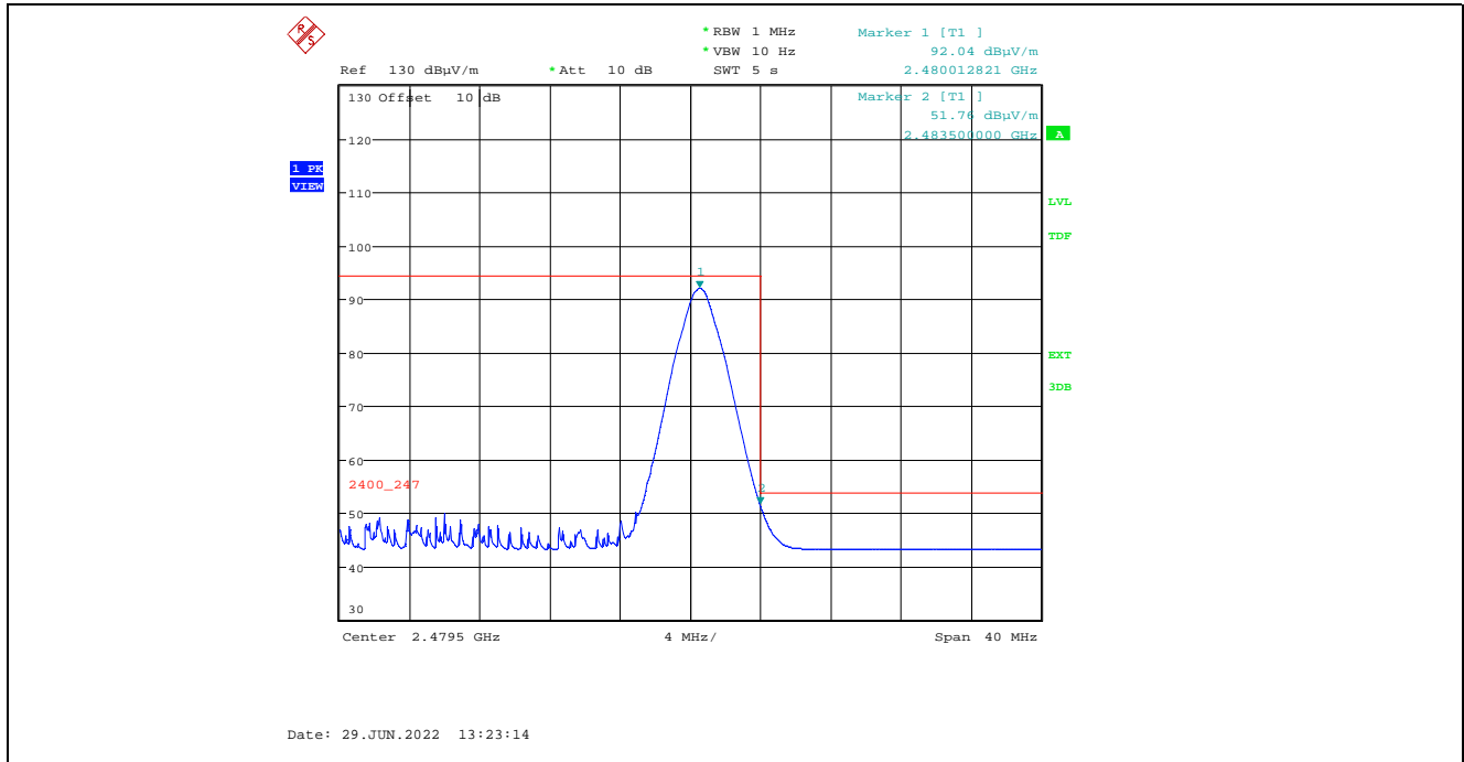
Plot 5.2.3.1.2.12. Band-Edge RF Radiated Emissions at 3 m, Vertical Polarization, Average High End of Frequency Band, 2480 MHz, 3 dBm Power Setting
