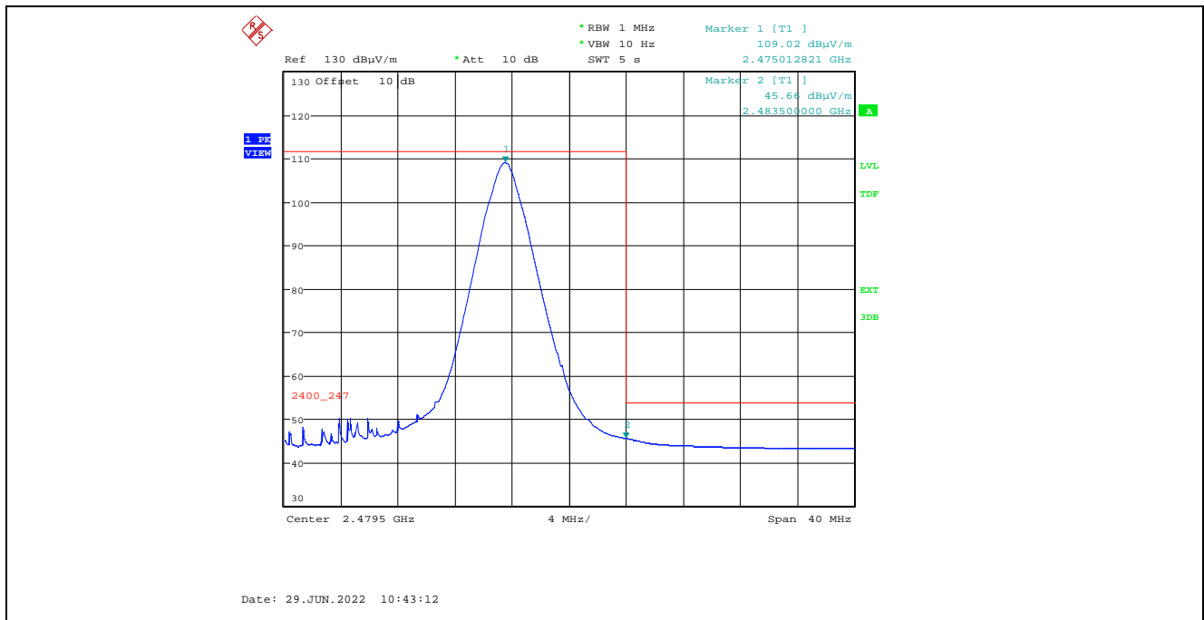
Plot 5.2.3.1.2.6. Band-Edge RF Radiated Emissions at 3 m, Horizontal Polarization, Average High End of Frequency Band, 2475 MHz, 20 dBm Power Setting
