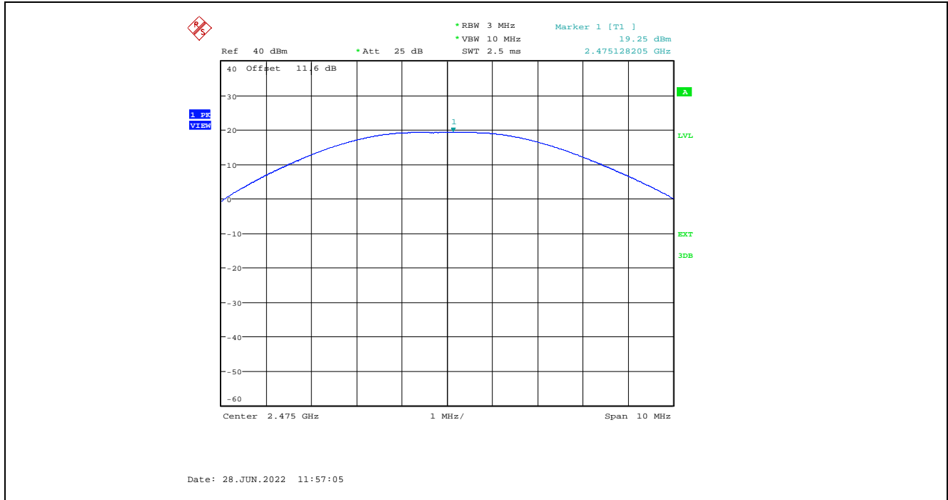
Plot 5.1.3.3. Maximum Peak Conducted Output Power, QPSK Modulation, 20 dBm Power Setting, 2475 MHz
