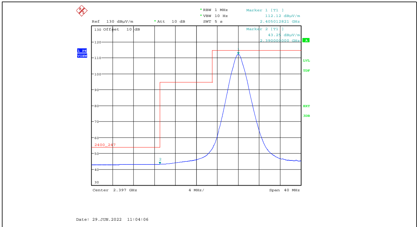
Plot 5.2.3.1.2.4. Band-Edge RF Radiated Emissions at 3 m, Vertical Polarization, Average Low End of Frequency Band, 2405 MHz, 20 dBm Power Setting
