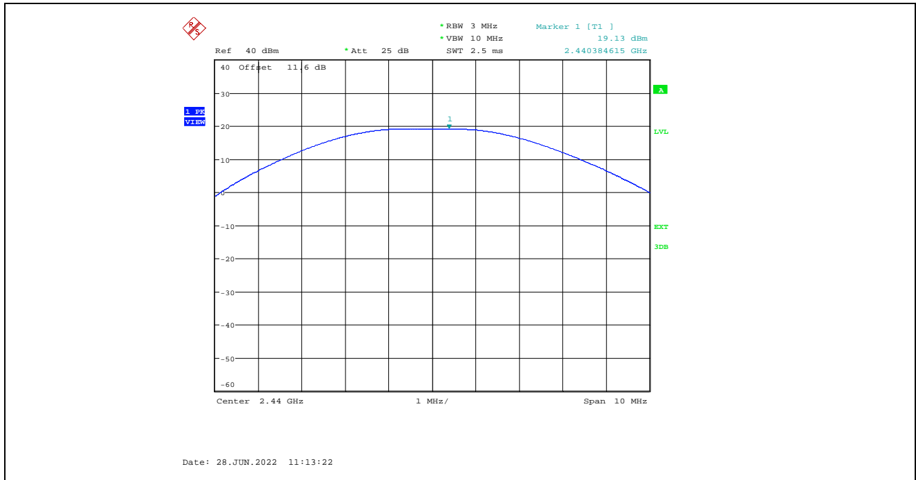
Plot 5.1.3.2. Maximum Peak Conducted Output Power, QPSK Modulation, 20 dBm Power Setting, 2440 MHz
