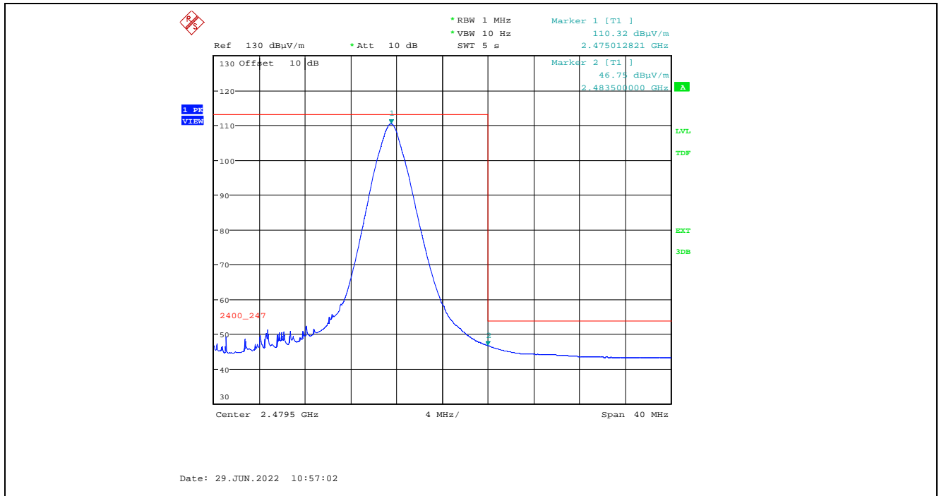
Plot 5.2.3.1.2.8. Band-Edge RF Radiated Emissions at 3 m, Vertical Polarization, Average High End of Frequency Band, 2475 MHz, 20 dBm Power Setting
