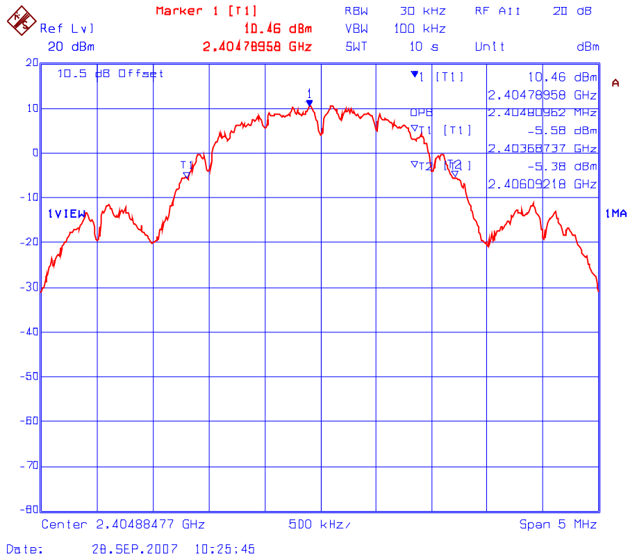
Plot 6.6.5.4 99% Occupied Bandwidth Frequency: 2405 MHz
