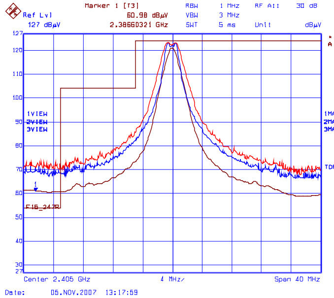
Plot 6.9.5.3.2(ii) Band-Edge RF Radiated Emissions @ 3 m Low End of Frequency Band Rx Antenna Orientation: Vertical
