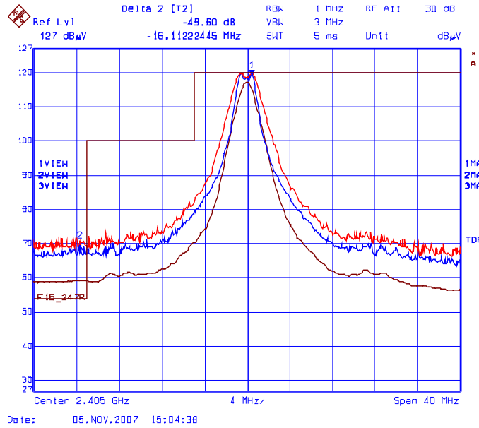
Plot 6.9.5.2.1(ii) Band-Edge RF Radiated Emissions @ 3 m Low End of Frequency Band Rx Antenna Orientation: Horizontal
