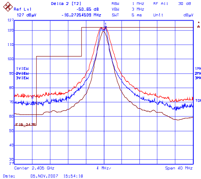
Plot 6.9.5.1.1(ii) Band-Edge RF Radiated Emissions @ 3 m Low End of Frequency Band Rx Antenna Orientation: Horizontal
