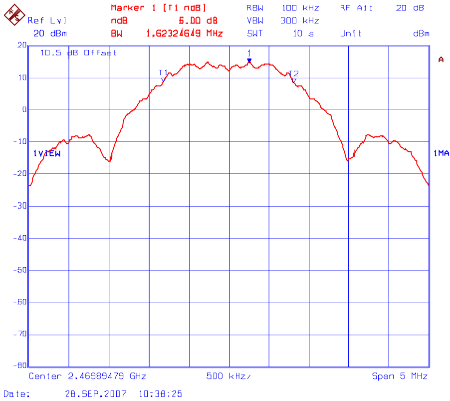
Plot 6.6.5.3 6 dB Bandwidth Frequency: 2470 MHz
