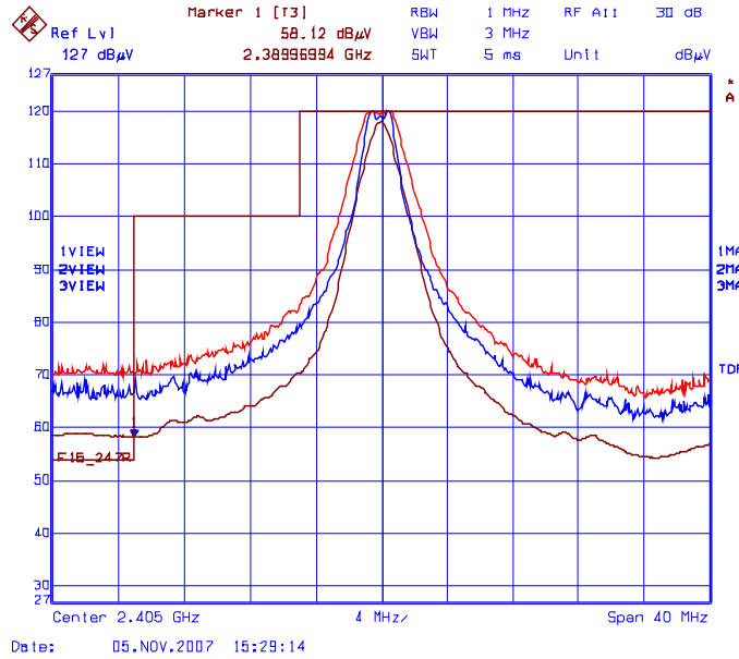
Plot 6.9.5.2.2(ii) Band-Edge RF Radiated Emissions @ 3 m Low End of Frequency Band Rx Antenna Orientation: Vertical
