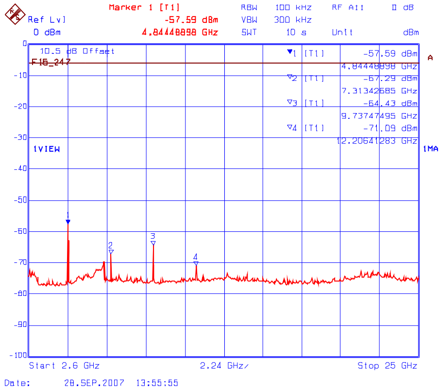
Plot 6.8.5.2.4 Spurious RF Conducted Emissions Transmitter Frequency: 2440 MHz
