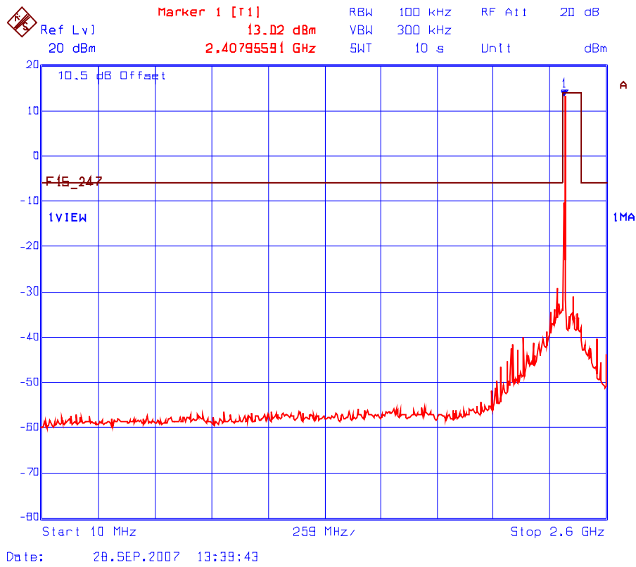
Plot 6.8.5.2.1 Spurious RF Conducted Emissions Transmitter Frequency: 2405 MHz
