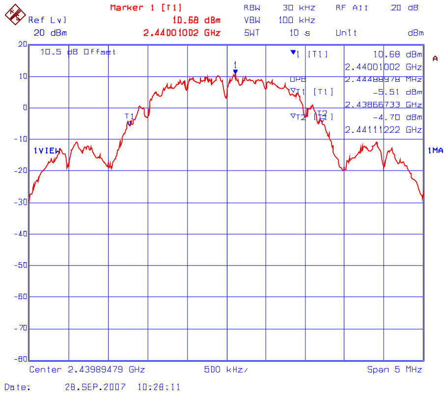
Plot 6.6.5.5 99% Occupied Bandwidth Frequency: 2440 MHz
