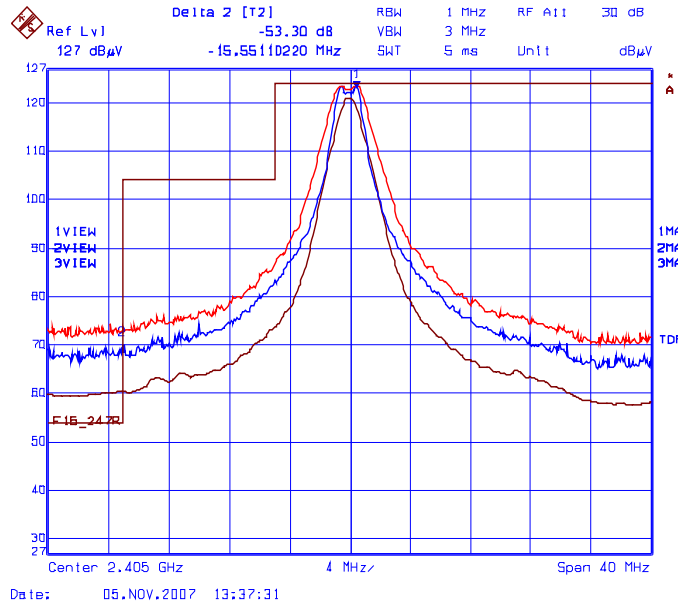
Plot 6.9.5.3.1(ii) Band-Edge RF Radiated Emissions @ 3 m Low End of Frequency Band Rx Antenna Orientation: Horizontal
