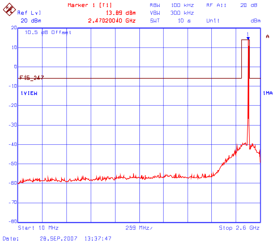
Plot 6.8.5.2.5 Spurious RF Conducted Emissions Transmitter Frequency: 2470 MHz
