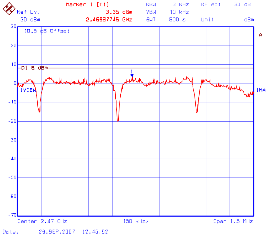
Plot 6.10.5.3 Power Spectral Density Frequency: 2470 MHz
