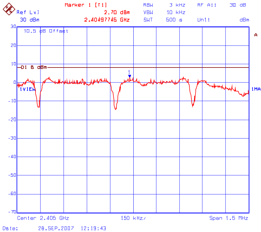
Plot 6.10.5.1 Power Spectral Density Frequency: 2405 MHz
