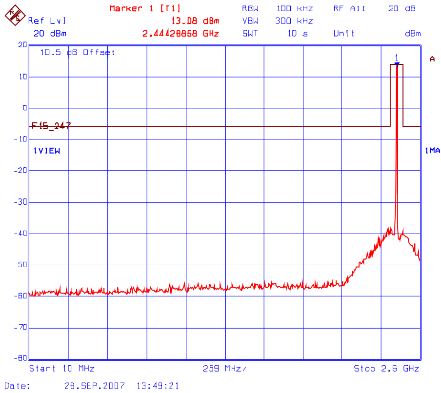
Plot 6.8.5.2.3 Spurious RF Conducted Emissions Transmitter Frequency: 2440 MHz
