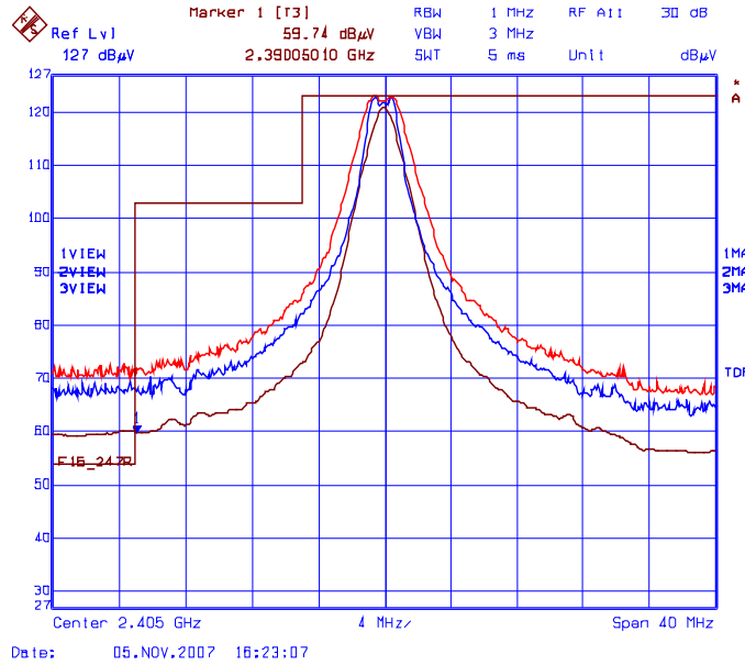
Plot 6.9.5.1.2(ii) Band-Edge RF Radiated Emissions @ 3 m Low End of Frequency Band Rx Antenna Orientation: Vertical
