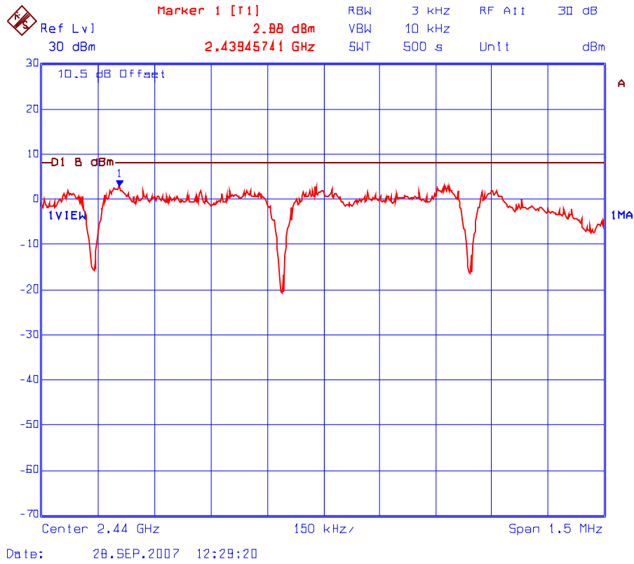
Plot 6.10.5.2 Power Spectral Density Frequency: 2440 MHz
