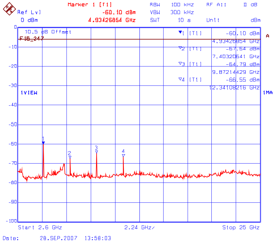
Plot 6.8.5.2.6 Spurious RF Conducted Emissions Transmitter Frequency: 2470 MHz
