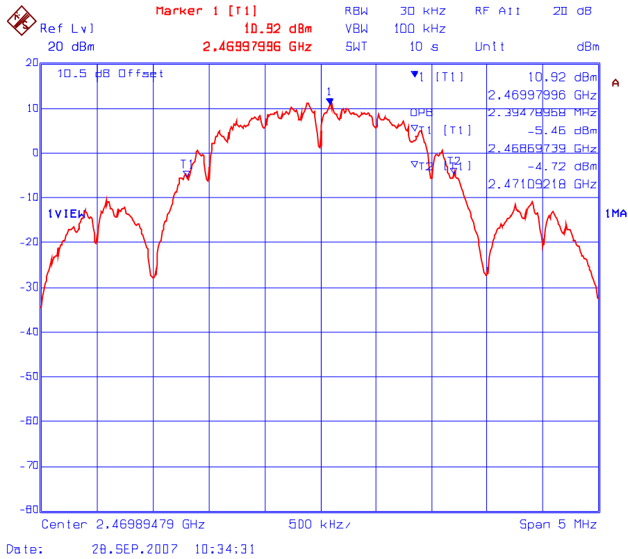
Plot 6.6.5.6 99% Occupied Bandwidth Frequency: 2470 MHz
