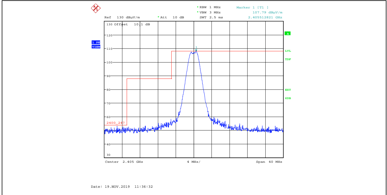
Plot 5.2.4.2.1. Band-Edge Radiated Emissions, Lower Band-edge, Peak Detector Rx Antenna in Vertical Polarization, QPSK Modulation, Power Setting 20, 2405 MHz
