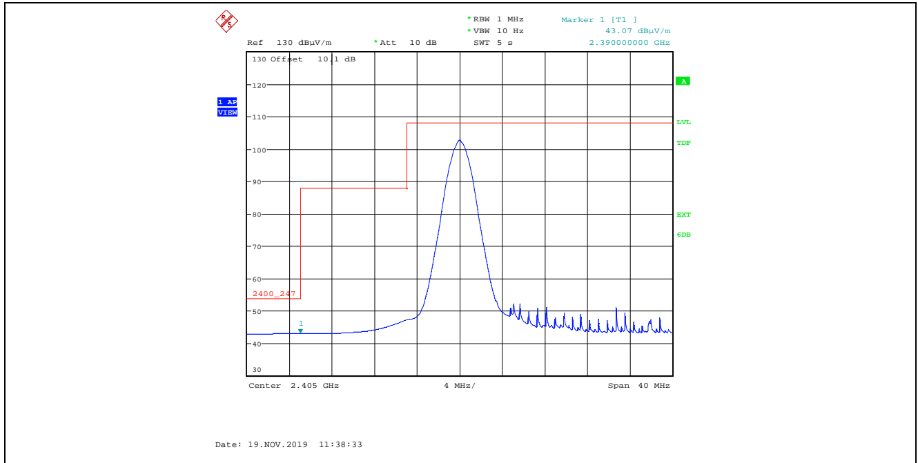
Plot 5.2.4.2.2. Band-Edge Radiated Emissions, Lower Band-edge, Average Detector Rx Antenna in Vertical Polarization, QPSK Modulation, Power Setting 20, 2405 MHz
