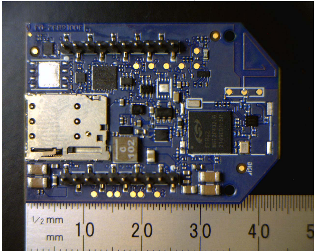
Bottom Side: Hardware Version 55002112-02 and 55002112-03 (Shield Removed)
