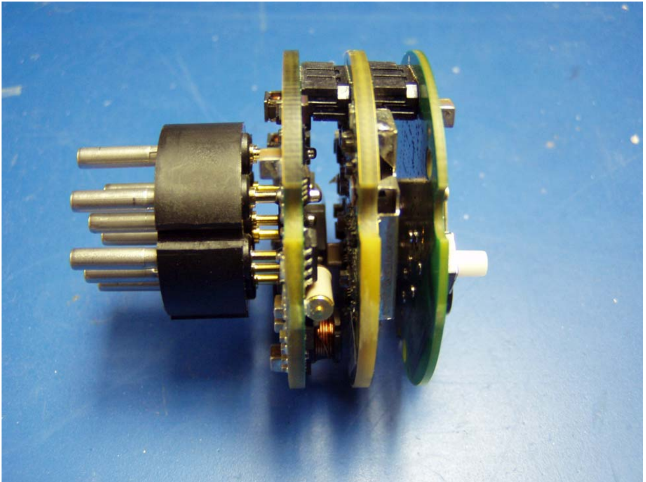
All three boards minus mechanicals - Assembled
