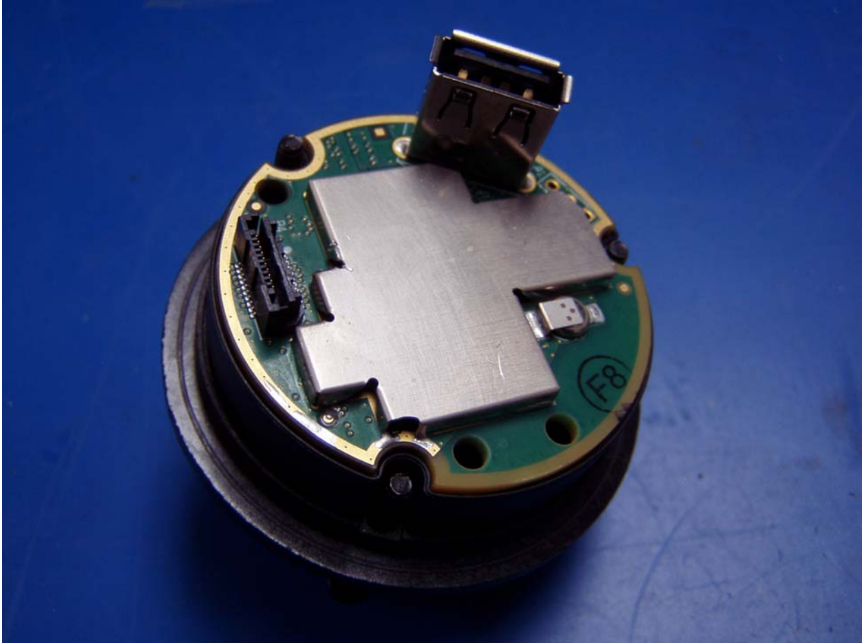
Assembly minus top, RF board, heatsink
