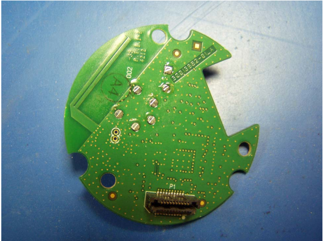
RF Board bottomside
