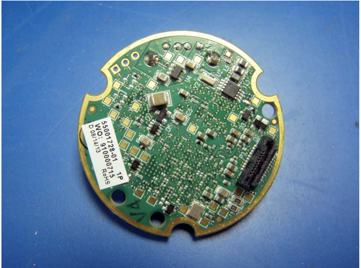
Processor board bottomside
