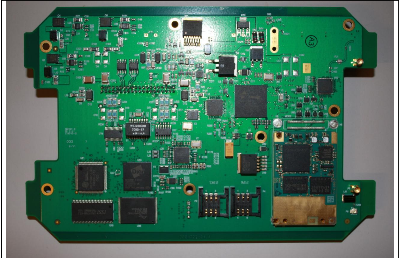
Figure 3. Internal circuit board back side
