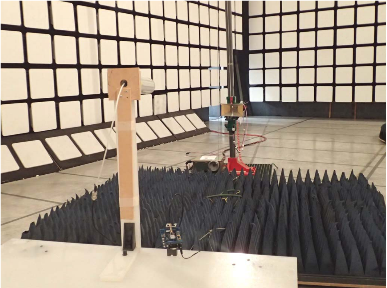
Radiated Emissions @ 3 m, Orthogonal Position 3 EUT with 15.0 dBi Yagi Antenna
