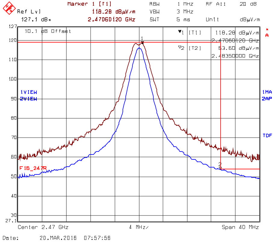
Plot 5.2.4.4.2.3. Band-Edge RF Radiated Emissions at 3 m, Horizontal Polarization High End of Frequency Band, Ch24- 2470 MHz, QPSK Modulation, Power 8 Mode 1
