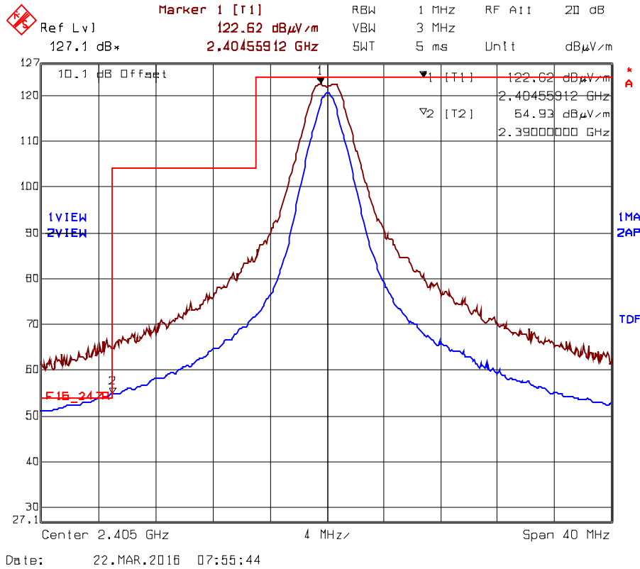
Plot 5.2.4.5.2.1. Band-Edge RF Radiated Emissions at 3 m, Horizontal Polarization Low End of Frequency Band, Ch11- 2405 MHz, QPSK Modulation, Power 8 Mode 1 @ 66% Duty Cycle
