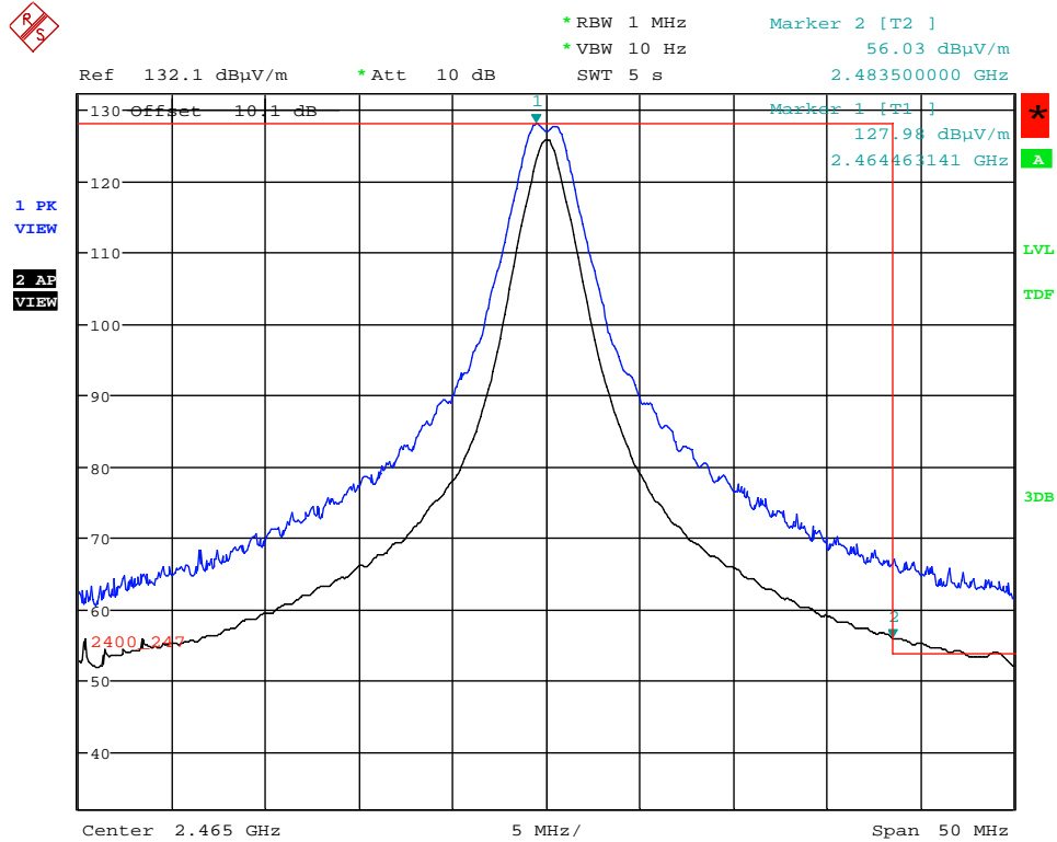
Plot 5.2.4.4.2.3. Band-Edge RF Radiated Emissions at 3 m, Horizontal Polarization Higher End of Frequency Band, Ch23- 2465 MHz, QPSK Modulation, Power -8 Mode 3 @ 66% Duty Cycle
