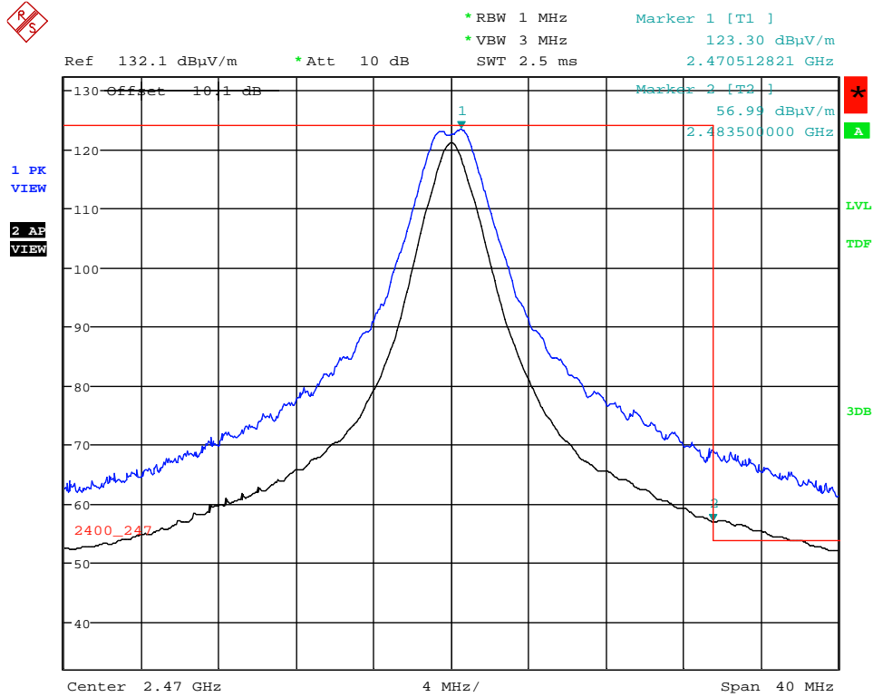
Plot 5.2.4.4.2.5. Band-Edge RF Radiated Emissions at 3 m, Horizontal Polarization Highest End of Frequency Band, Ch24- 2470 MHz, QPSK Modulation, Power -8 Mode 3 @ 66% Duty Cycle
