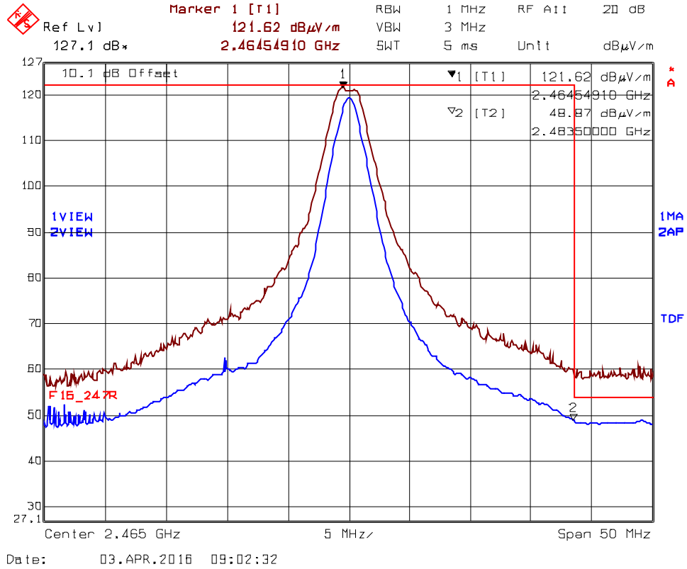
Plot 5.2.4.2.4. Band-Edge RF Radiated Emissions at 3 m, Vertical Polarization High End of Frequency Band, Ch23- 2465 MHz, QPSK Modulation, Power -8 Mode 3
