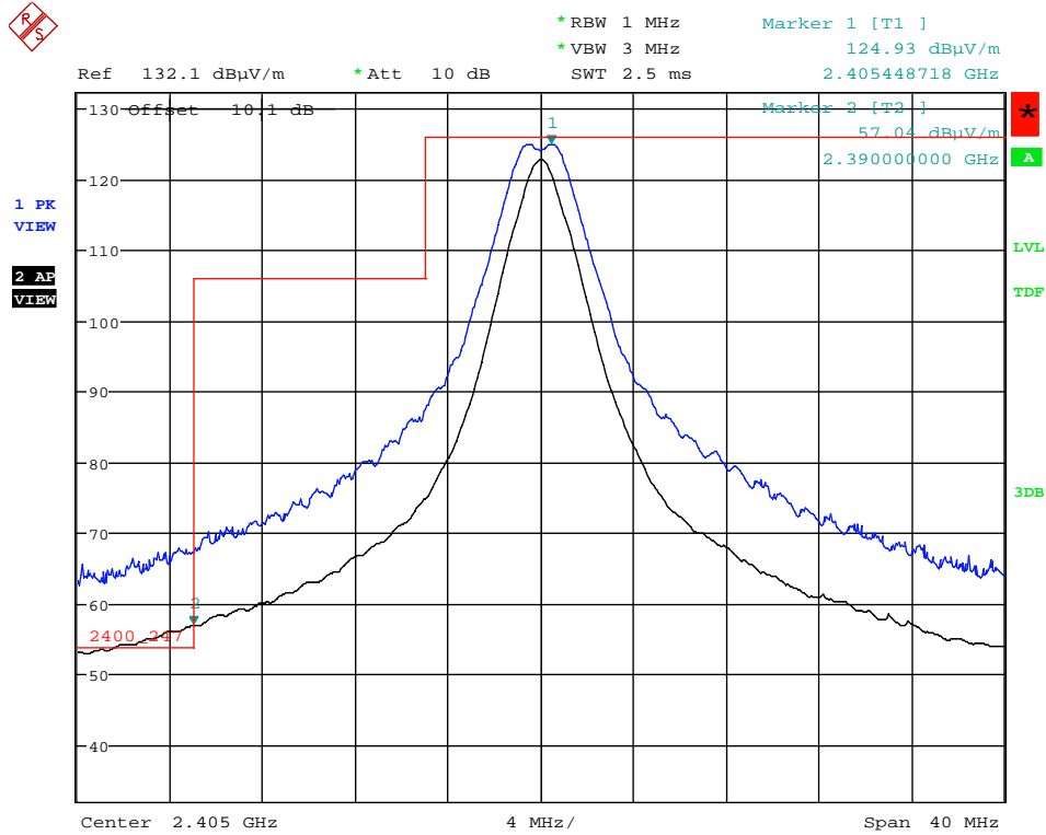
Plot 5.2.4.4.2.1. Band-Edge RF Radiated Emissions at 3 m, Horizontal Polarization Low End of Frequency Band, Ch11- 2405 MHz, QPSK Modulation, Power -8 Mode 3 @ 66% Duty Cycle
