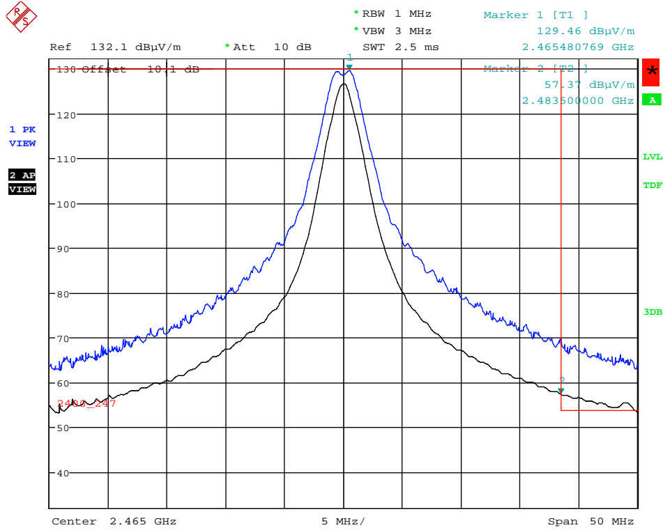
Plot 5.2.4.5.2.3. Band-Edge RF Radiated Emissions at 3 m, Horizontal Polarization Higher End of Frequency Band, Ch23- 2465 MHz, QPSK Modulation, Power -8 Mode 3 @ 66% Duty Cycle
