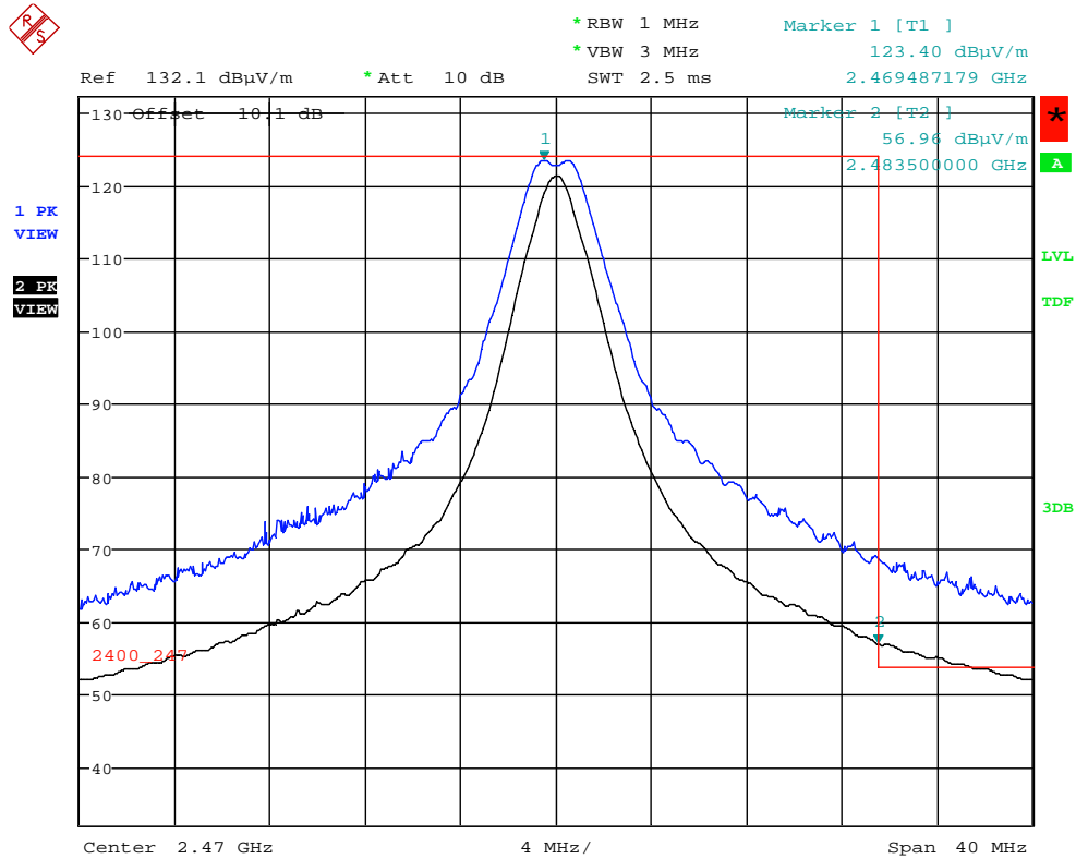
Plot 5.2.4.5.2.5. Band-Edge RF Radiated Emissions at 3 m, Horizontal Polarization Highest End of Frequency Band, Ch24- 2470 MHz, QPSK Modulation, Power -8 Mode 3 @ 66% Duty Cycle
