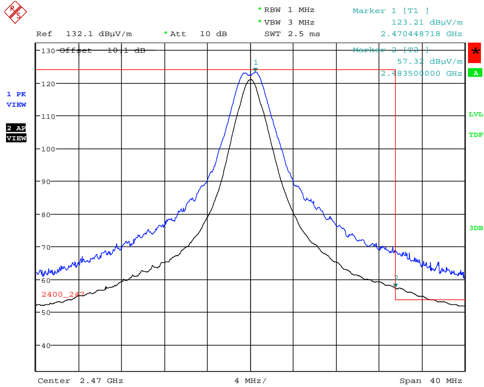
Plot 5.2.4.4.2.6. Band-Edge RF Radiated Emissions at 3 m, Vertical Polarization Highest End of Frequency Band, Ch24- 2470 MHz, QPSK Modulation, Power -8 Mode 3 @ 66% Duty Cycle
