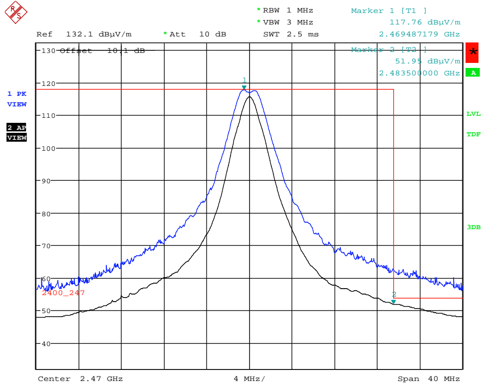
Plot 5.2.4.3.2.5. Band-Edge RF Radiated Emissions at 3 m, Horizontal Polarization Highest End of Frequency Band, Ch24- 2470 MHz, QPSK Modulation, Power -8 Mode 3 @ 66% Duty Cycle
