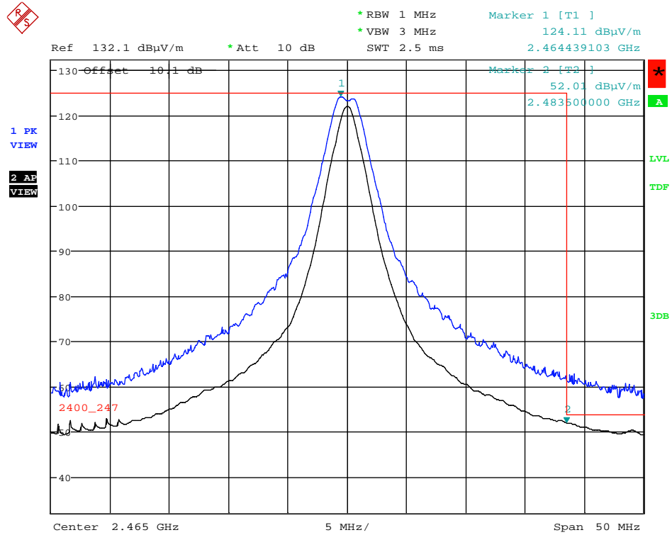
Plot 5.2.4.3.2.3. Band-Edge RF Radiated Emissions at 3 m, Horizontal Polarization High End of Frequency Band, Ch23- 2465 MHz, QPSK Modulation, Power -8 Mode 3 @ 66% Duty Cycle
