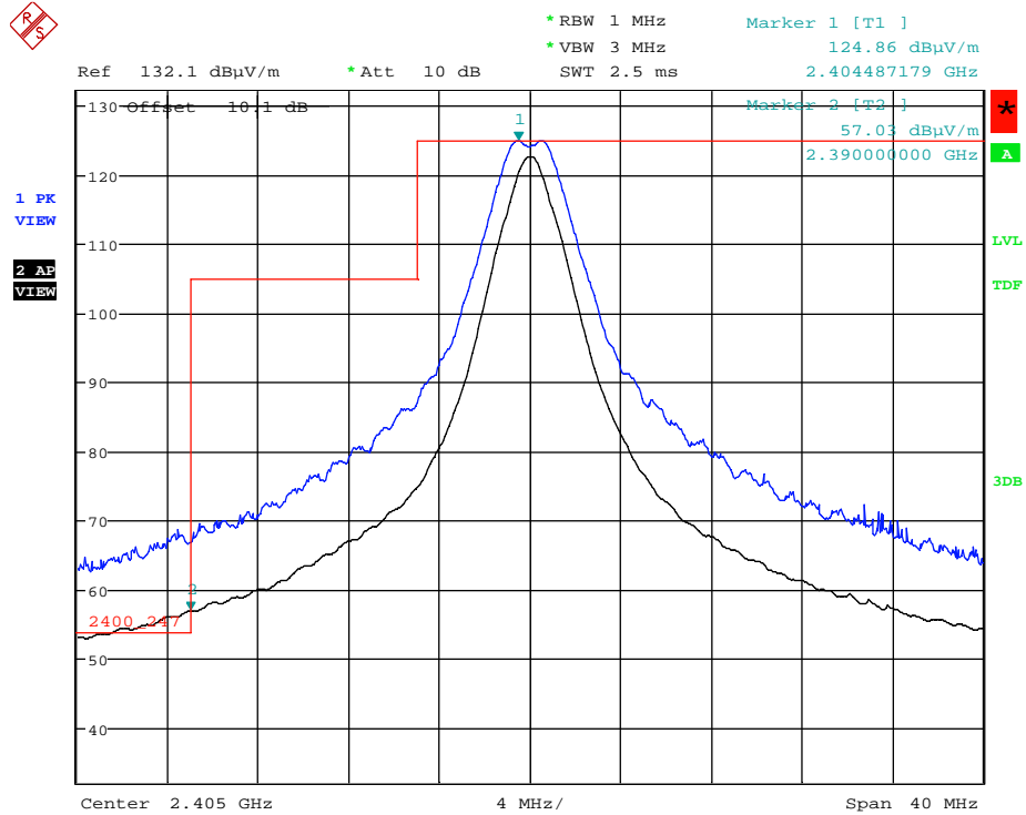
Plot 5.2.4.5.2.1. Band-Edge RF Radiated Emissions at 3 m, Horizontal Polarization Low End of Frequency Band, Ch11- 2405 MHz, QPSK Modulation, Power -8 Mode 3 @ 66% Duty Cycle
