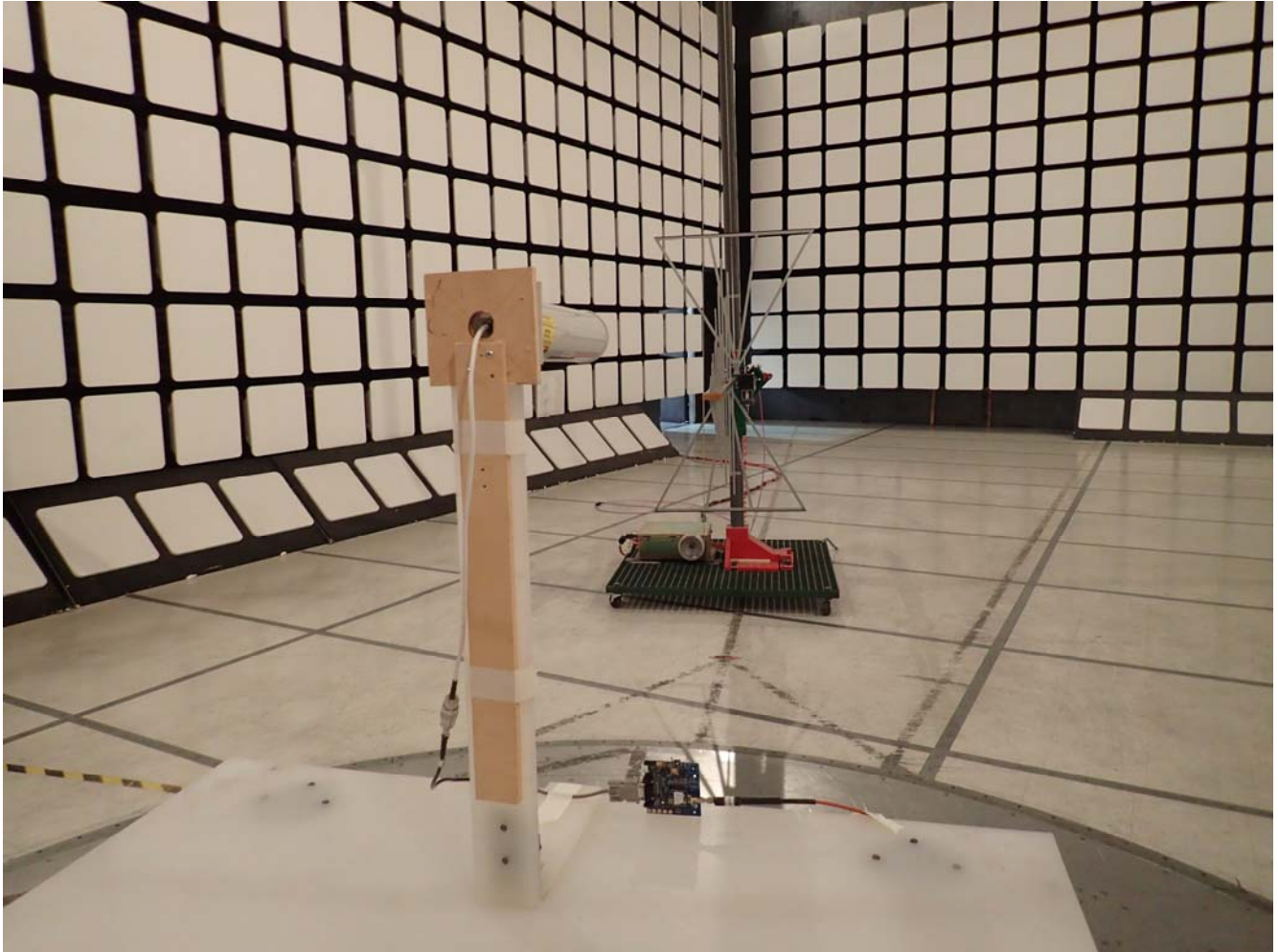
Radiated Emissions @ 3 m, Orthogonal Position 2 EUT with 15.0 dBi Yagi Antenna and 6.04 dB Assembly Cable Loss
