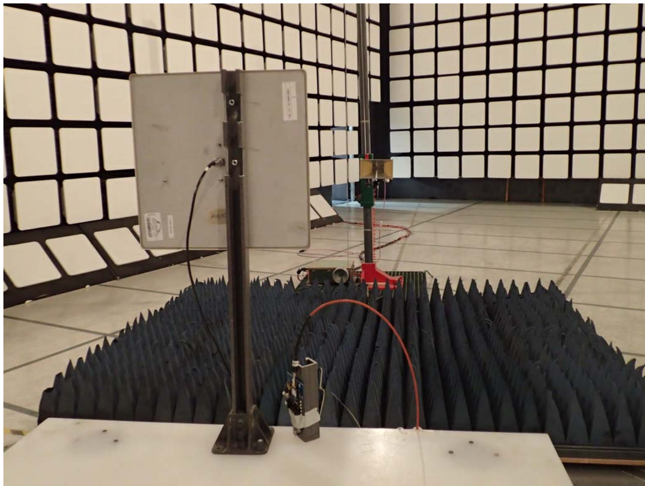
Radiated Emissions @ 3 m, Orthogonal Position 3 EUT with 19.0 dBi Flat Panel Antenna and 12.12 dB Assembly Cable Loss
