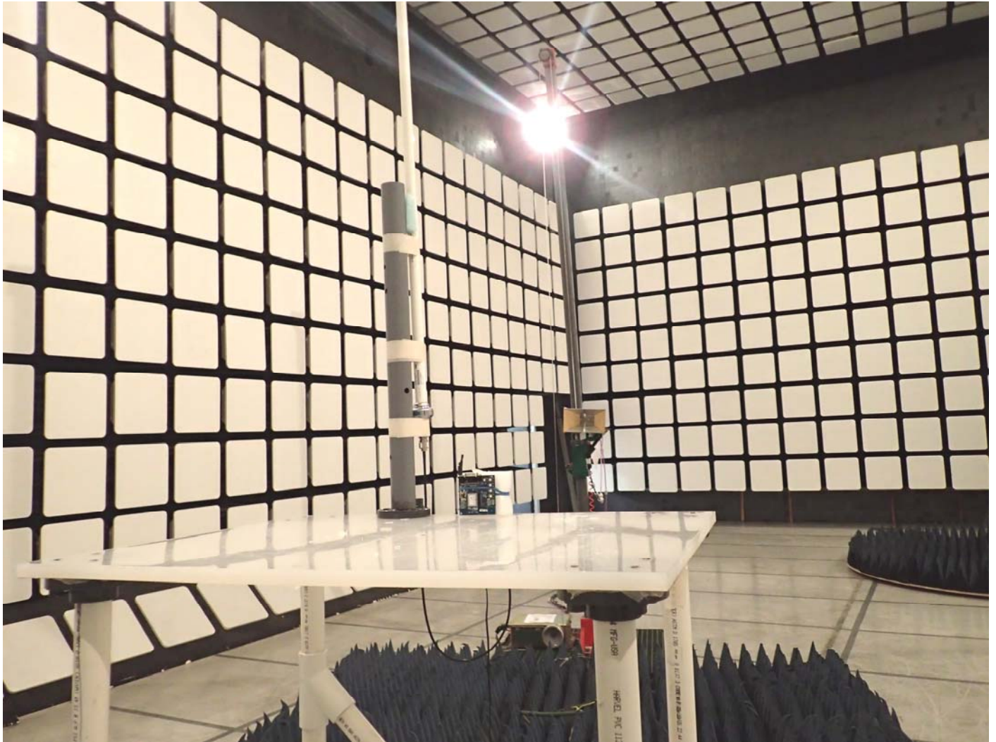
Radiated Emissions @ 3 m, Orthogonal Position 3 EUT with 15 dBi Omni-directional Antenna
