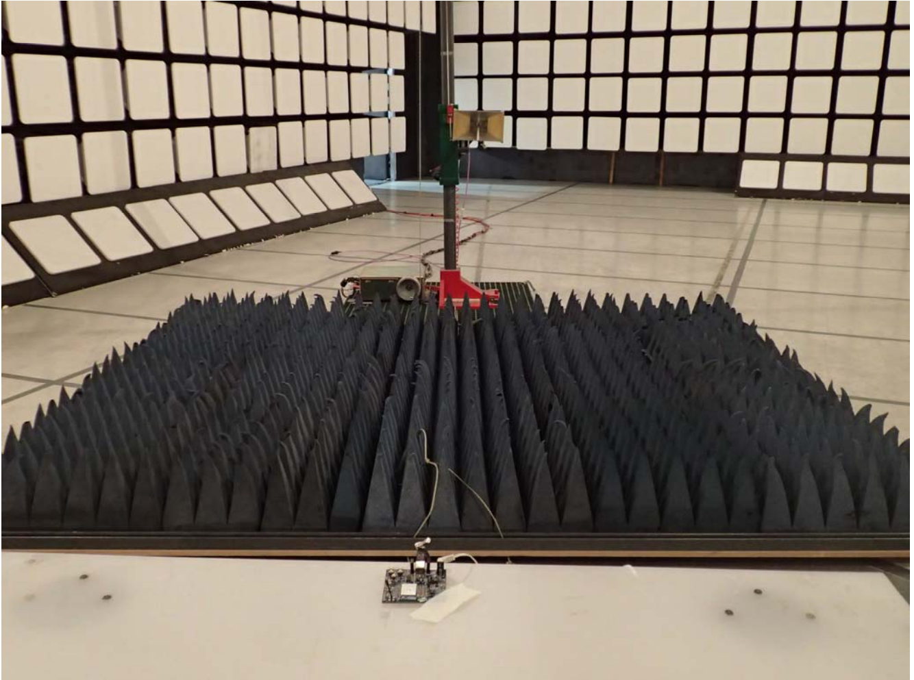
Radiated Emissions @ 3 m EUT with 1.5 dBi Monopole (Integrated Whip) Antenna
