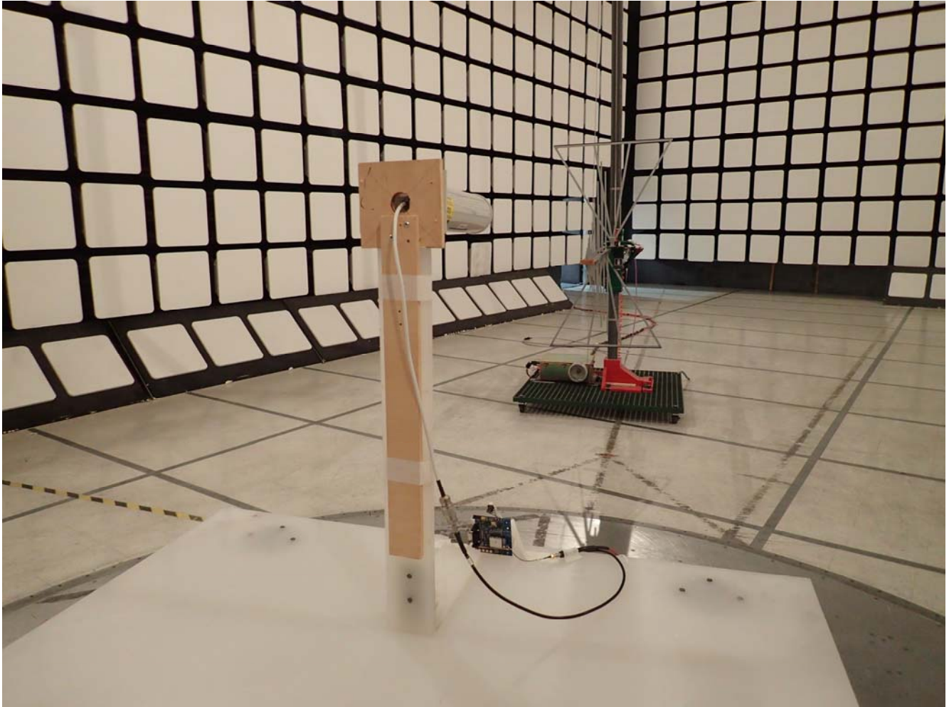
Radiated Emissions @ 3 m, Orthogonal Position 2 EUT with 15.0 dBi Yagi Antenna and 10.08 dB Assembly Cable Loss
