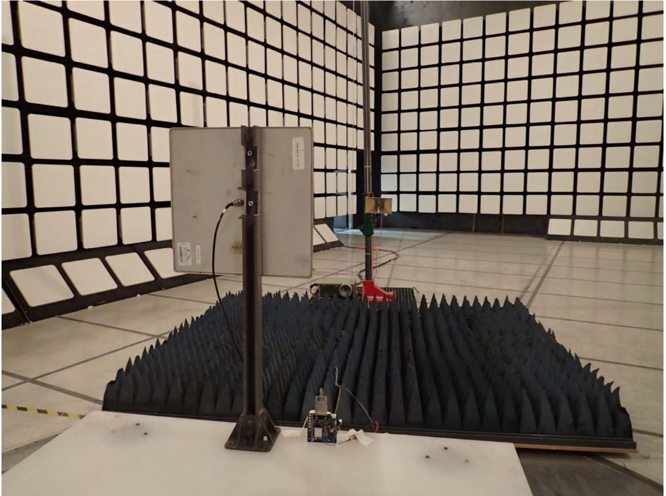
Radiated Emissions @ 3 m, Orthogonal Position 3 EUT with 19.0 dBi Flat Panel Antenna and 14.66 dB Assembly Cable Loss
