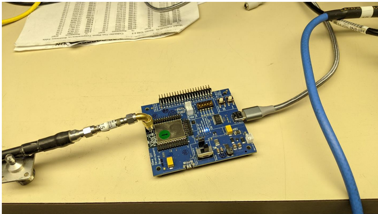
Conducted RF Test Setup
