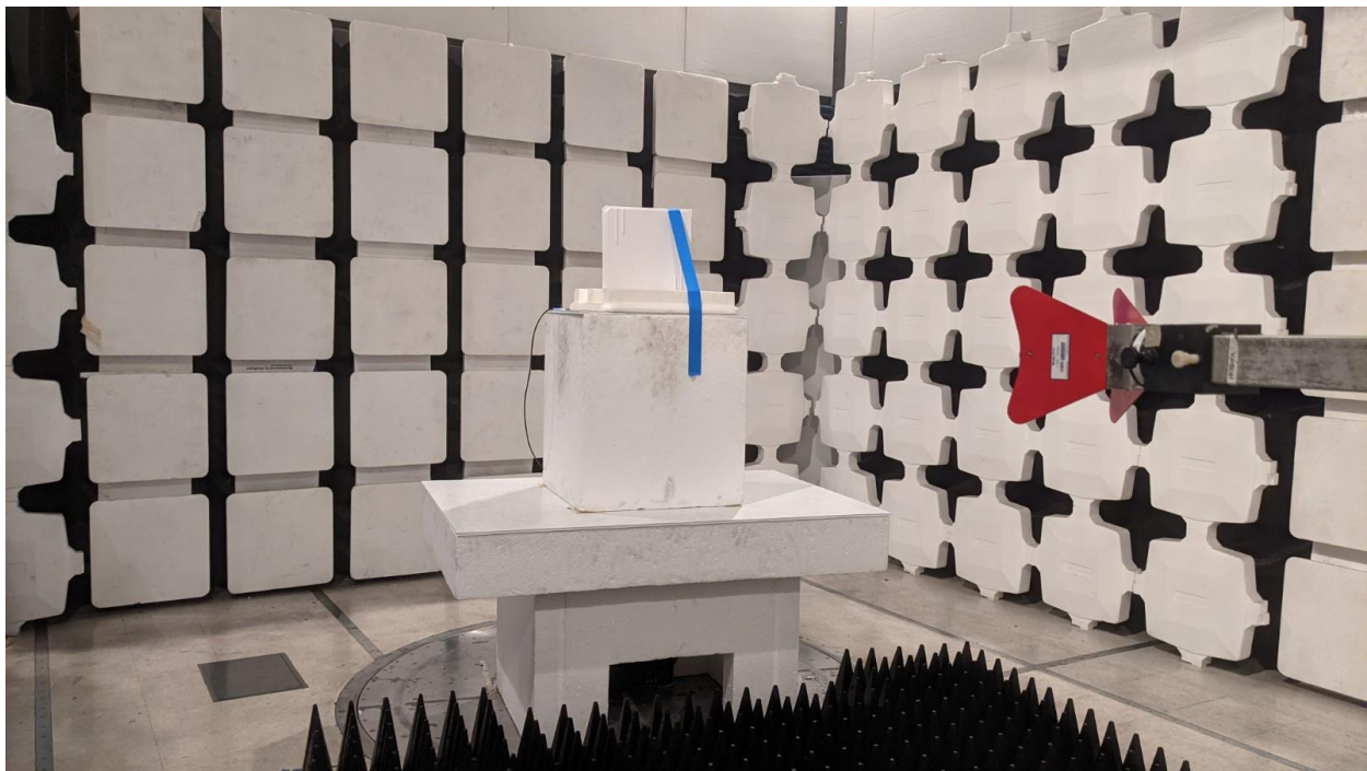
Spurious Emissions PAT2419
