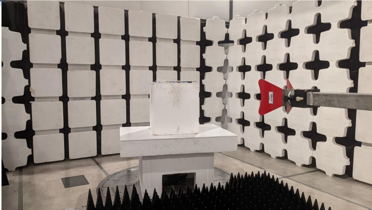
Spurious Emissions STKA-YA24-18SM
