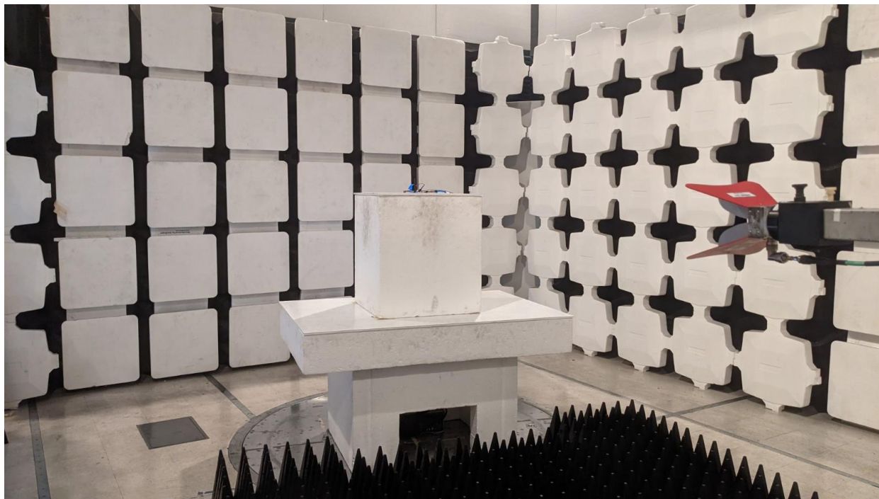
Spurious Emissions A24-HASM-450
