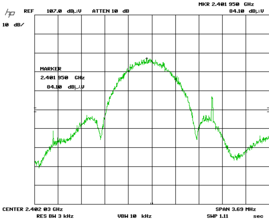
Low Channel Vertical Antenna Polarity
