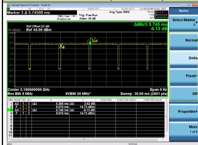
802.11ac-VHT40 (T = 5.385ms)
