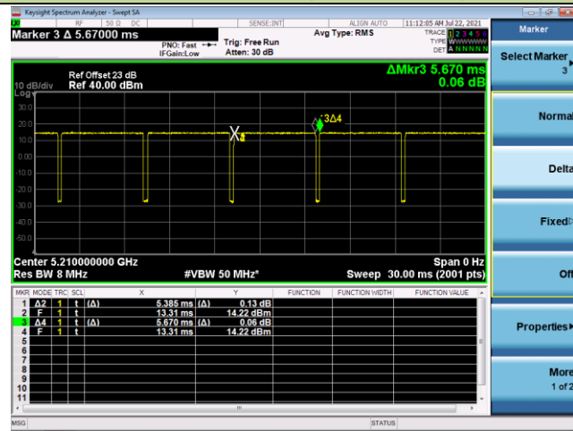
802.11ax-HE80 (T = 5.385ms)
