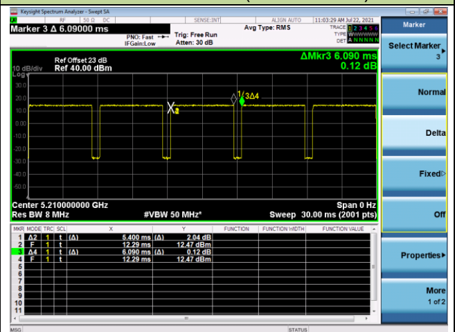
802.11ac-VHT80 (T = 5.400ms)
