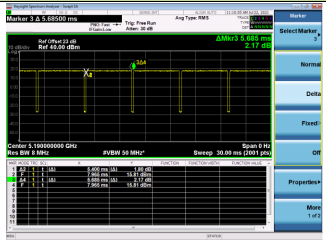
802.11ax-HE40 (T = 5.400ms)
