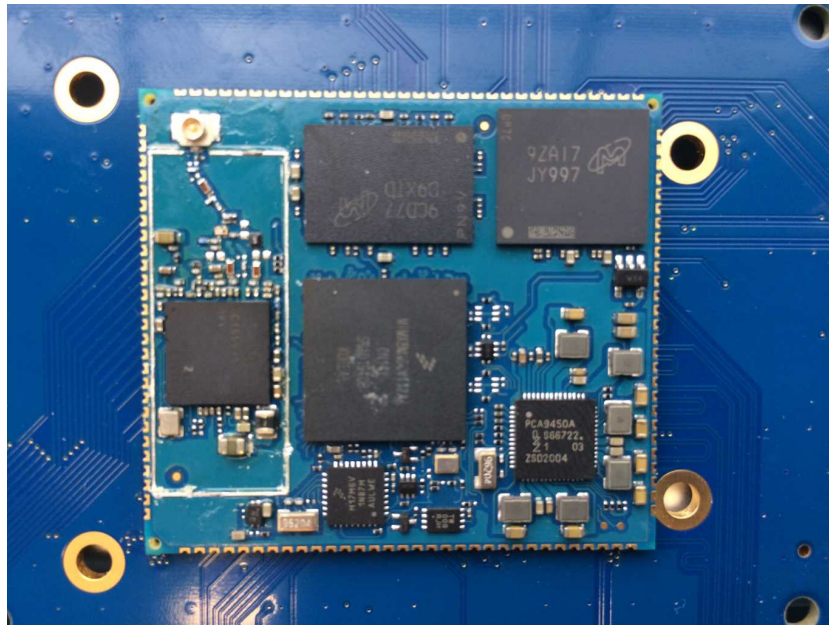
Photo 1: Module top side view with shielding removed
