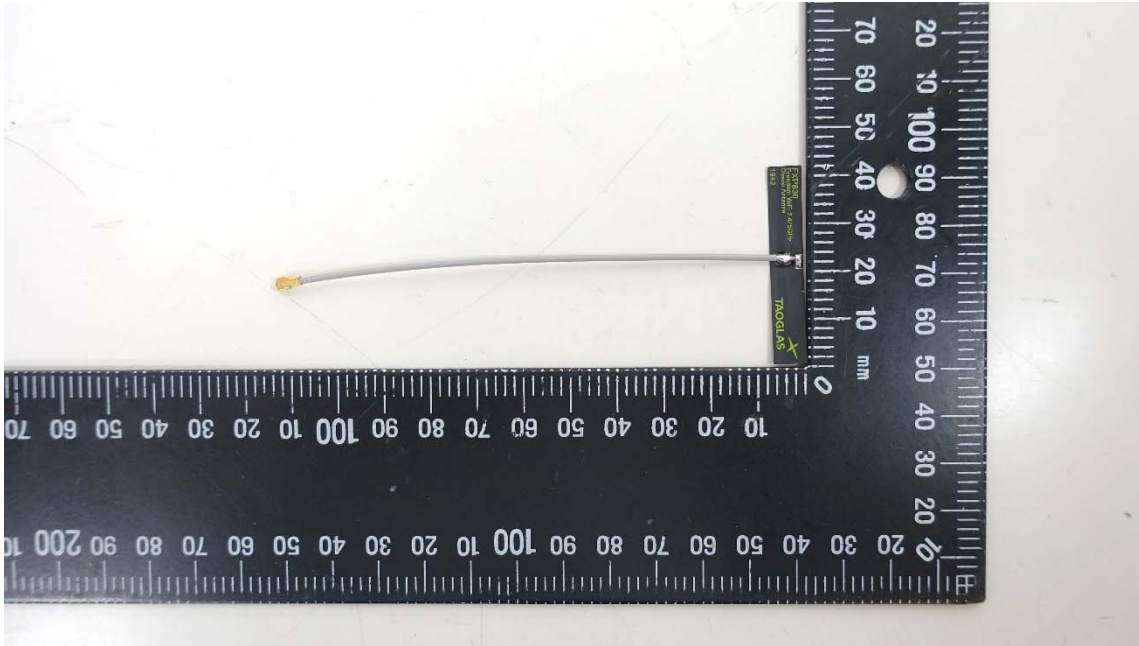
Antenna-6 (Model No.: FXP831.07.0100C)
