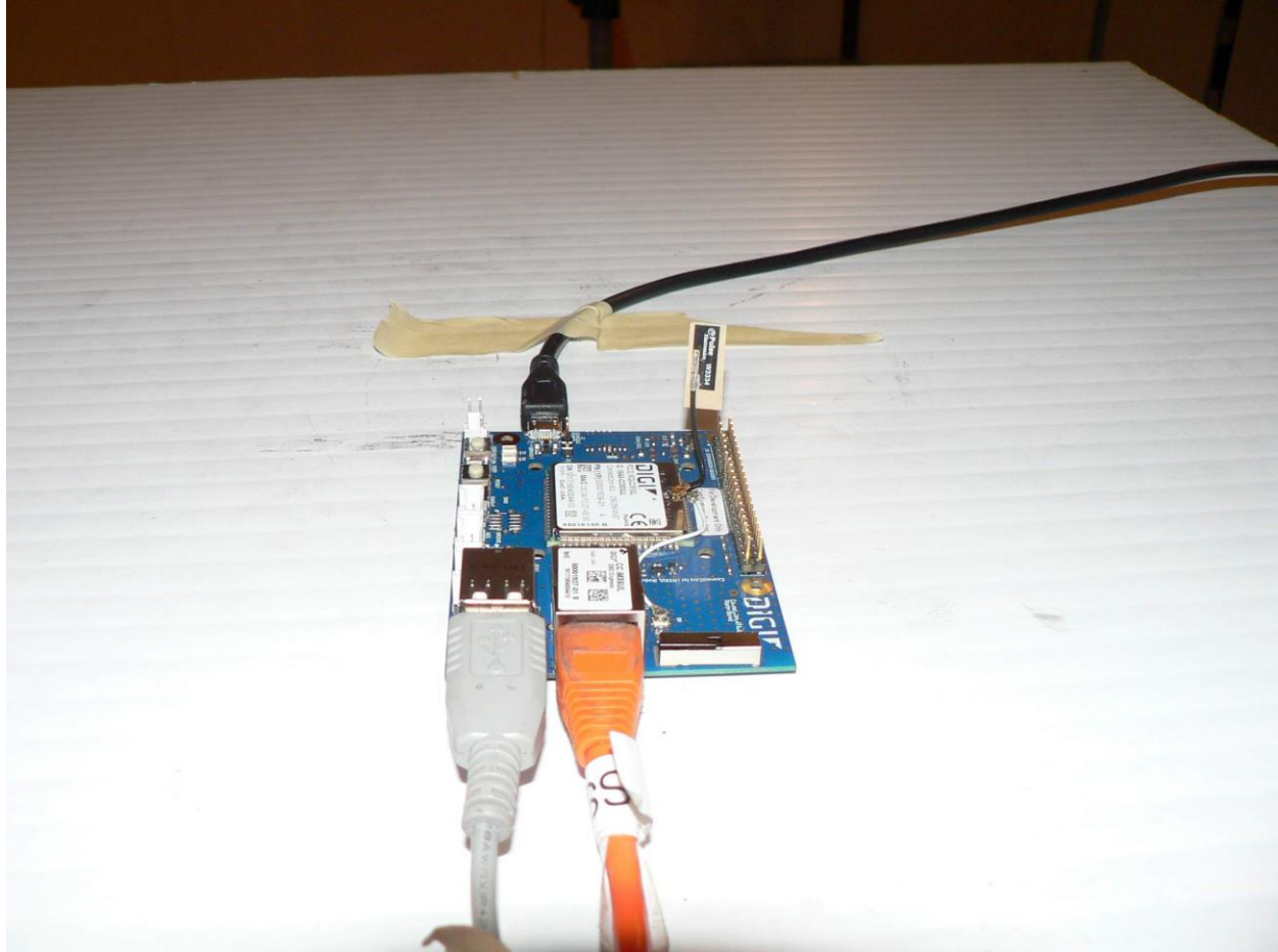
DIGI79 Transmitter Spurious Setup -Closeup with Patch Antenna
