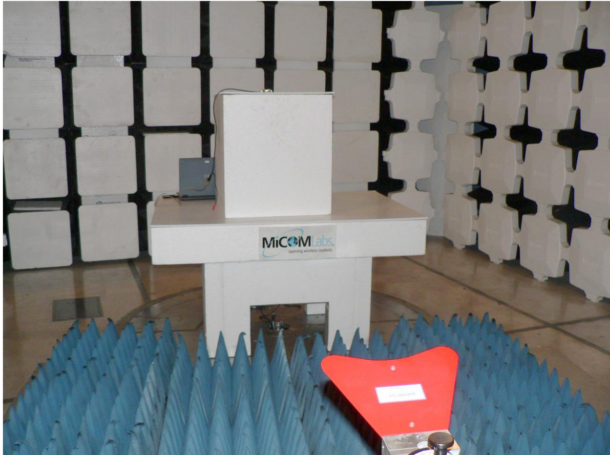
DIGI79 Transmitter Spurious 1-18GHz
